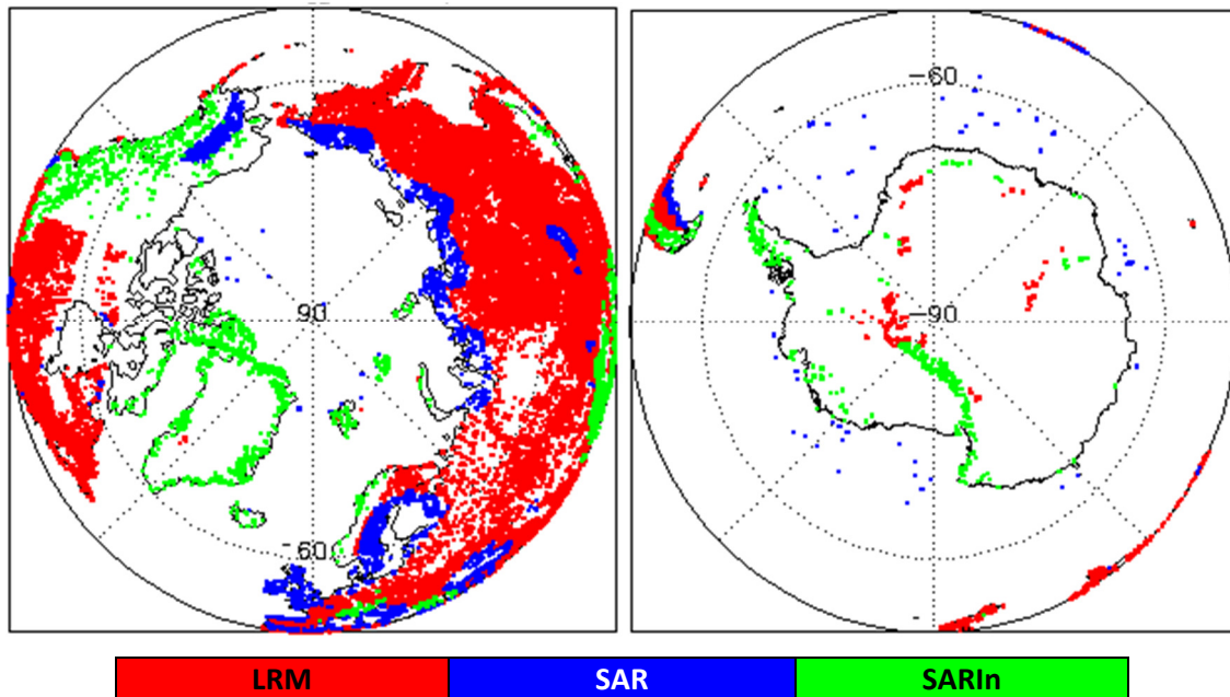
Figure 2 - Polar plots showing areas of loss of track in all SIRAL modes L0 data during August 2019.
