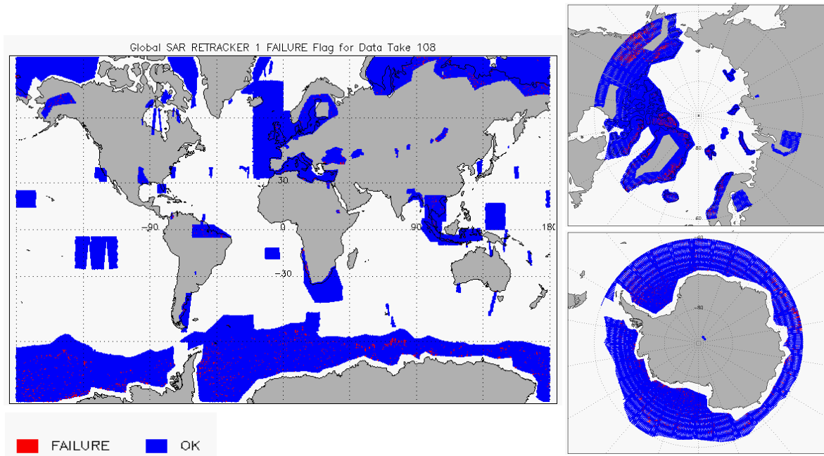
Figure 10 – Global plots showing Retracker Failure Flags for SAR mode for cycle #108
