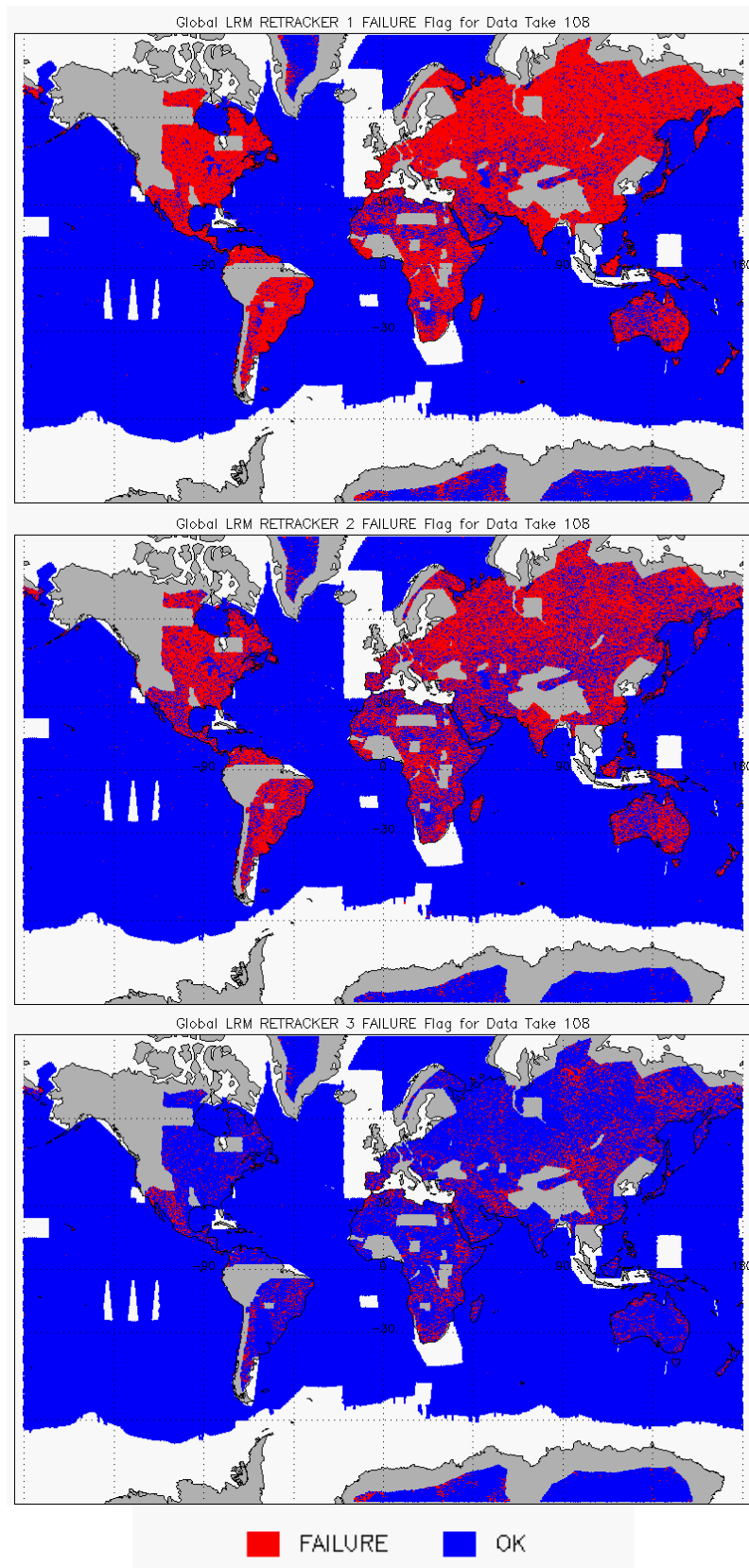
Figure 9 – Global plots showing Retracker Failure Flags for LRM mode for cycle #108:
