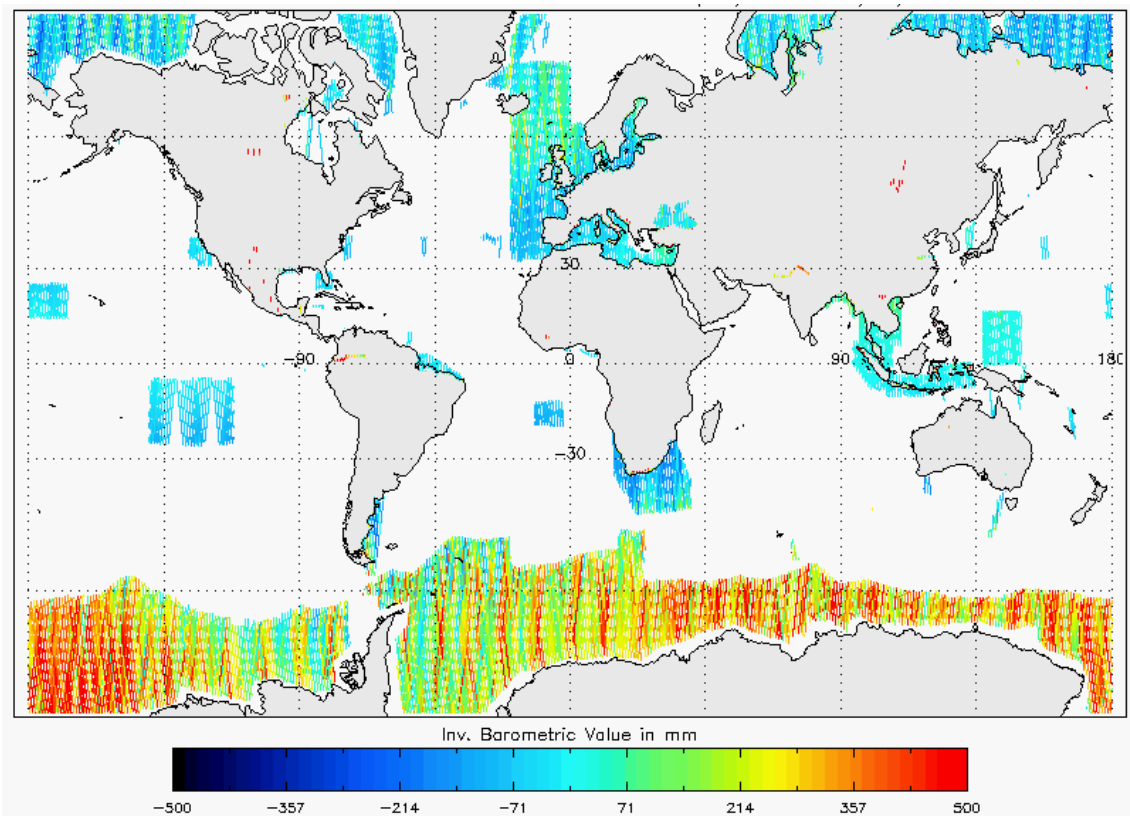
Figure 20 - Global plot of Inverse Barometric Correction for cycle #108
