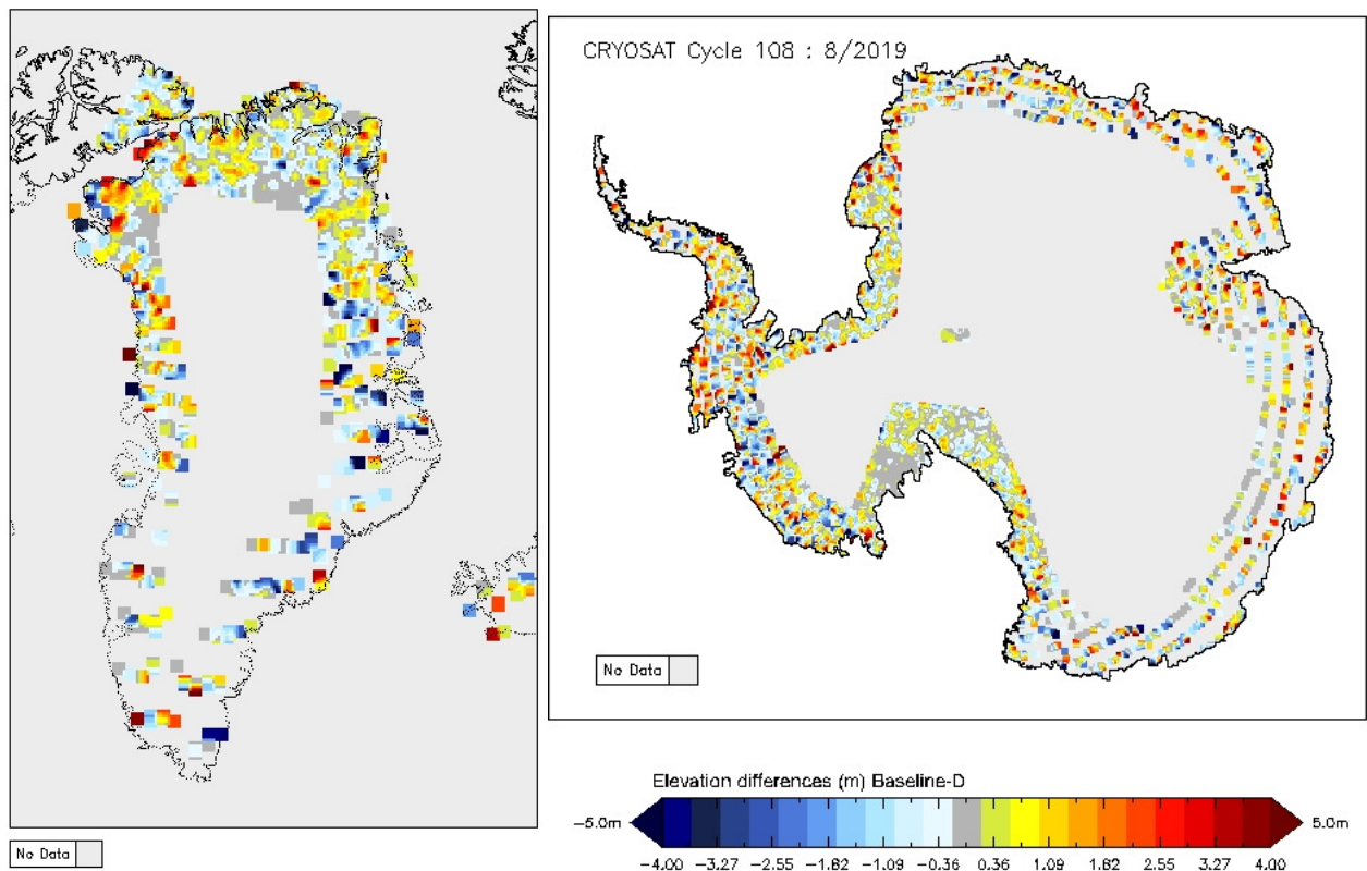
Figure 15 - Greenland and Antarctica maps of SARIn elevation differences for cycle #108
