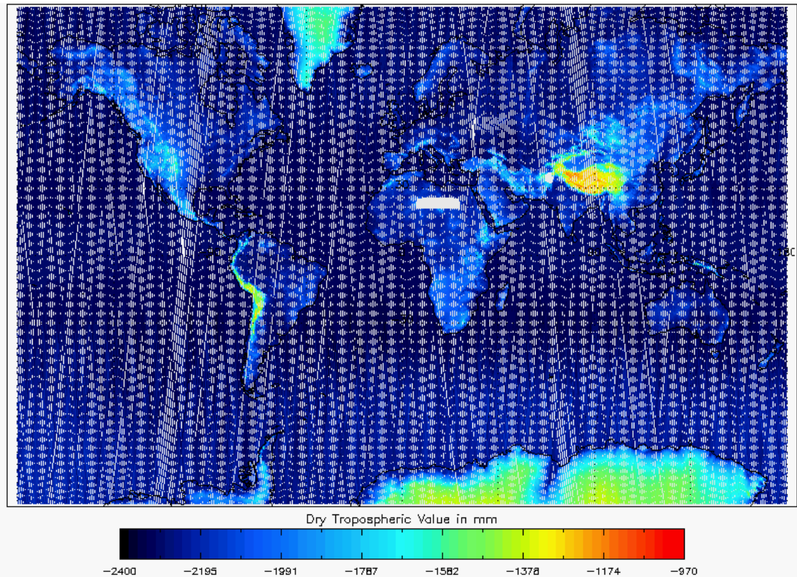
Figure 16 - Global plot of Dry Tropospheric Correction for cycle #108
