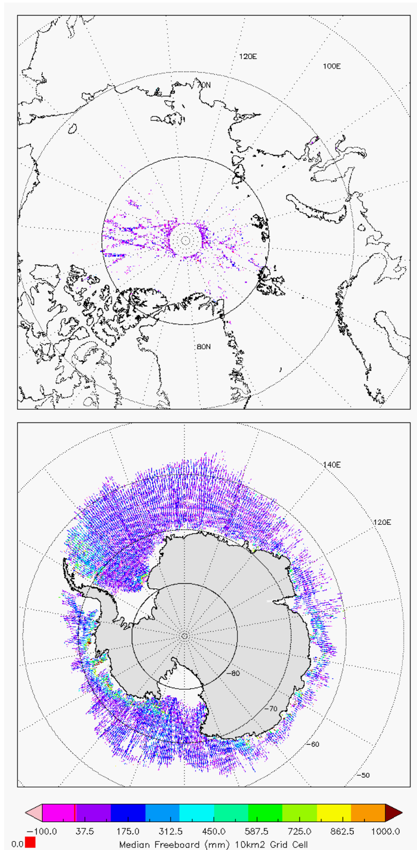
Figure 6 - Polar plots of 10km Gridded Freeboard values from L2 SAR products in cycle #108.
