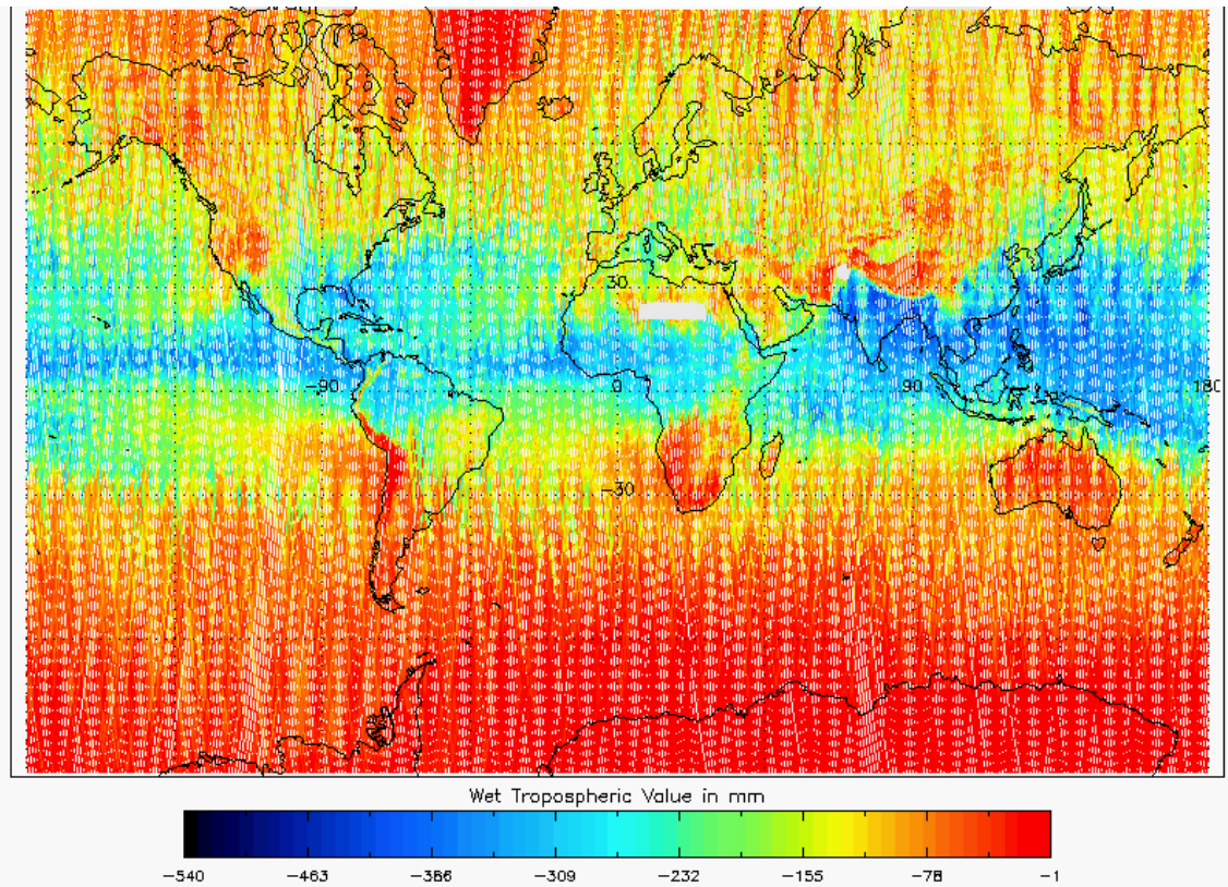
Figure 18 - Global plot of Wet Tropospheric Correction for cycle #108
