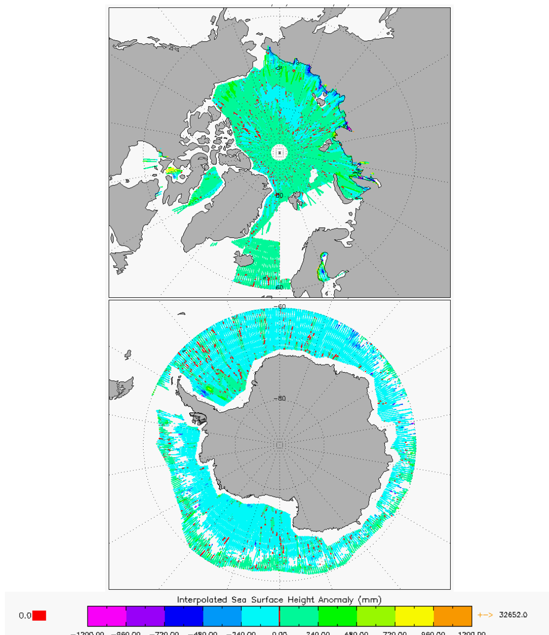
Figure 7 –Polar plots of SSHA for cycle #108.
