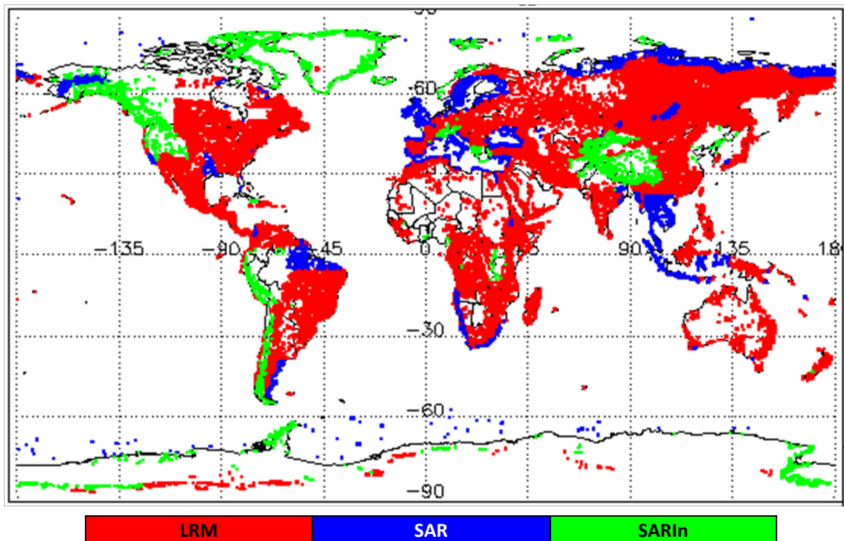
Figure 1 - Global plot showing areas of loss of track in all SIRAL modes L0 data during August 2019.
