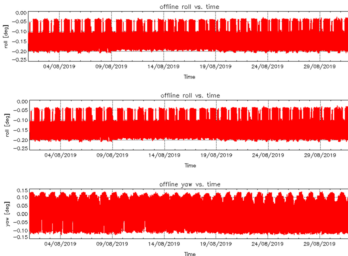
Figure 4 – Roll (top), Pitch (middle) and Yaw (bottom) values for L1B Products during cycle #108.
