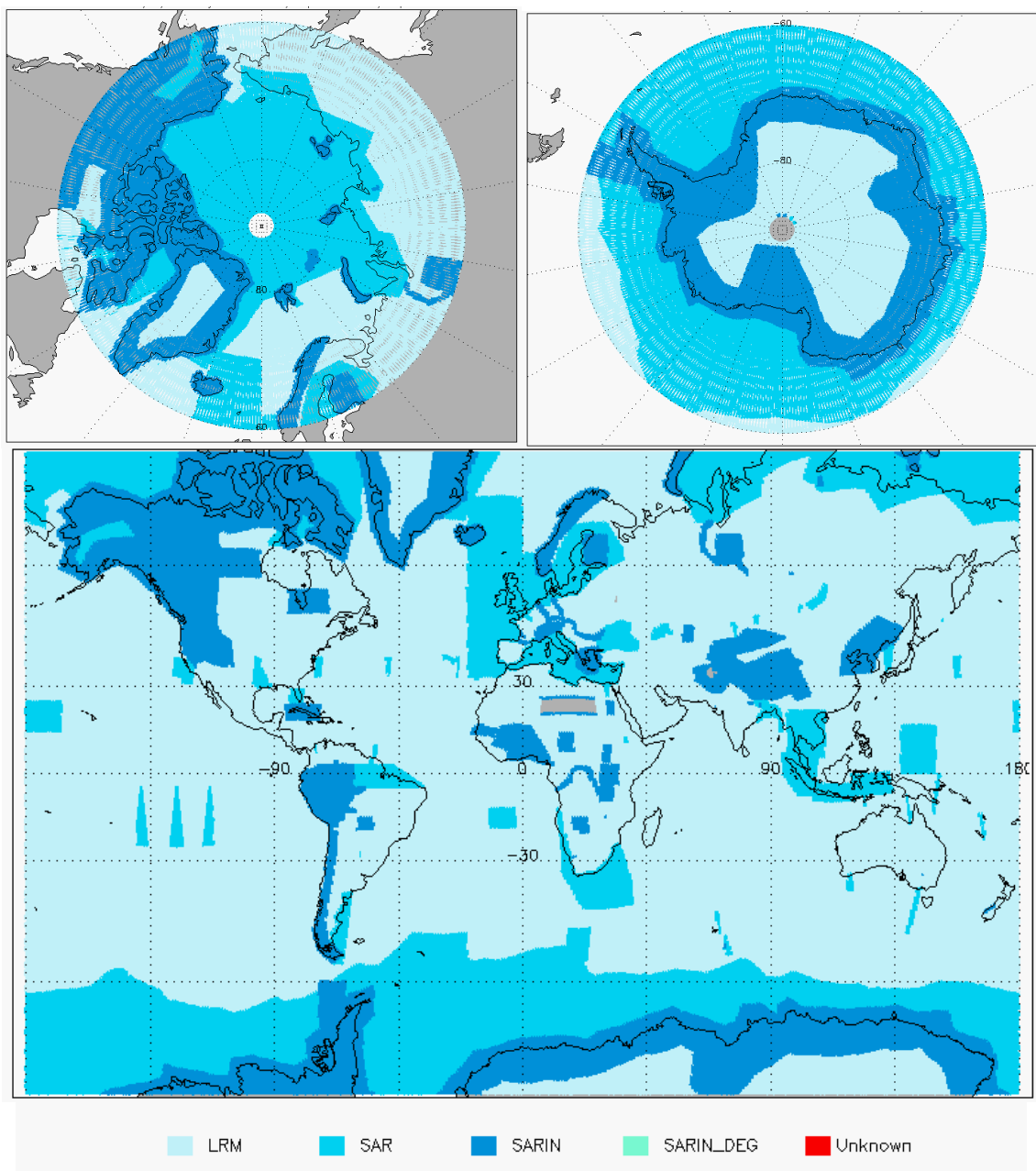
Figure 3 - Global and Polar plots of SIRAL Modes for cycle #108.
