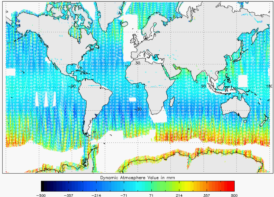
Figure 22 - Global plot of Dynamic Atmospheric Correction for cycle #108
