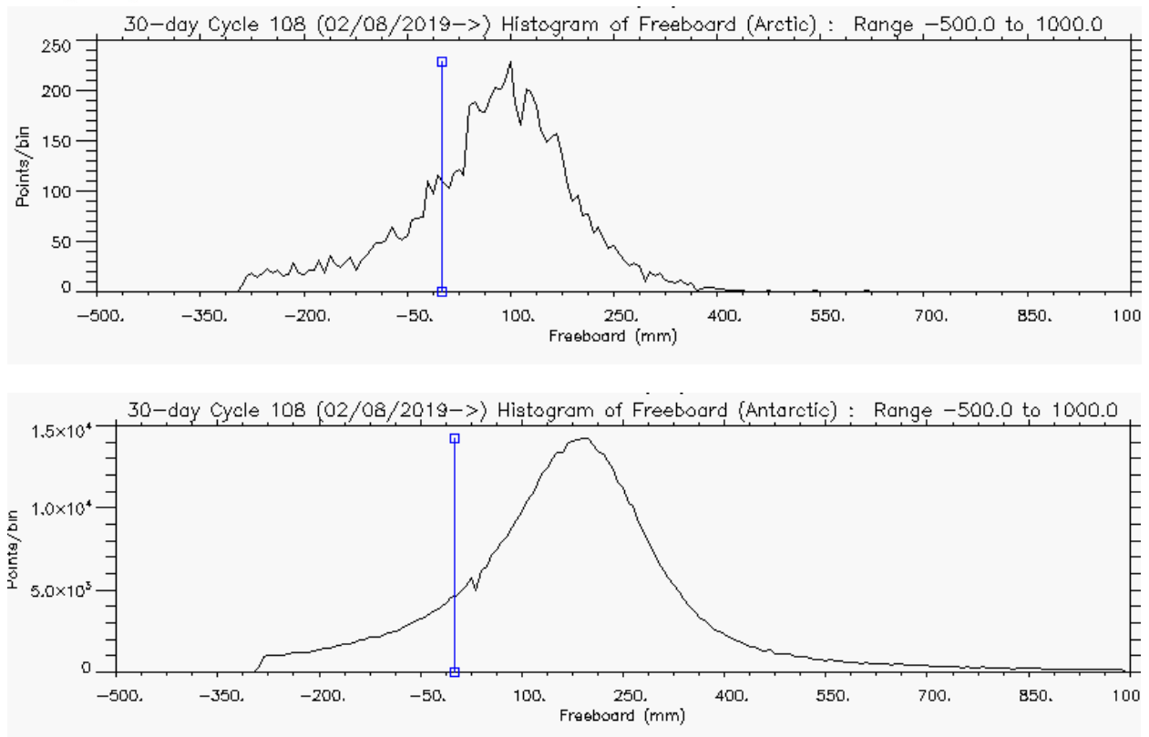
Figure 5 – Histogram of Freeboard for Arctic (above) and Antarctic (below) for cycle #108
