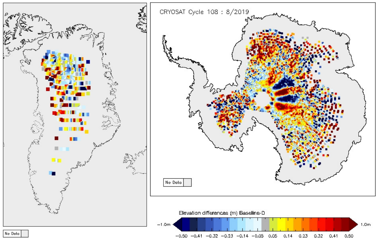
Figure 14 - Greenland and Antarctica maps of LRM elevation differences for cycle #108.
