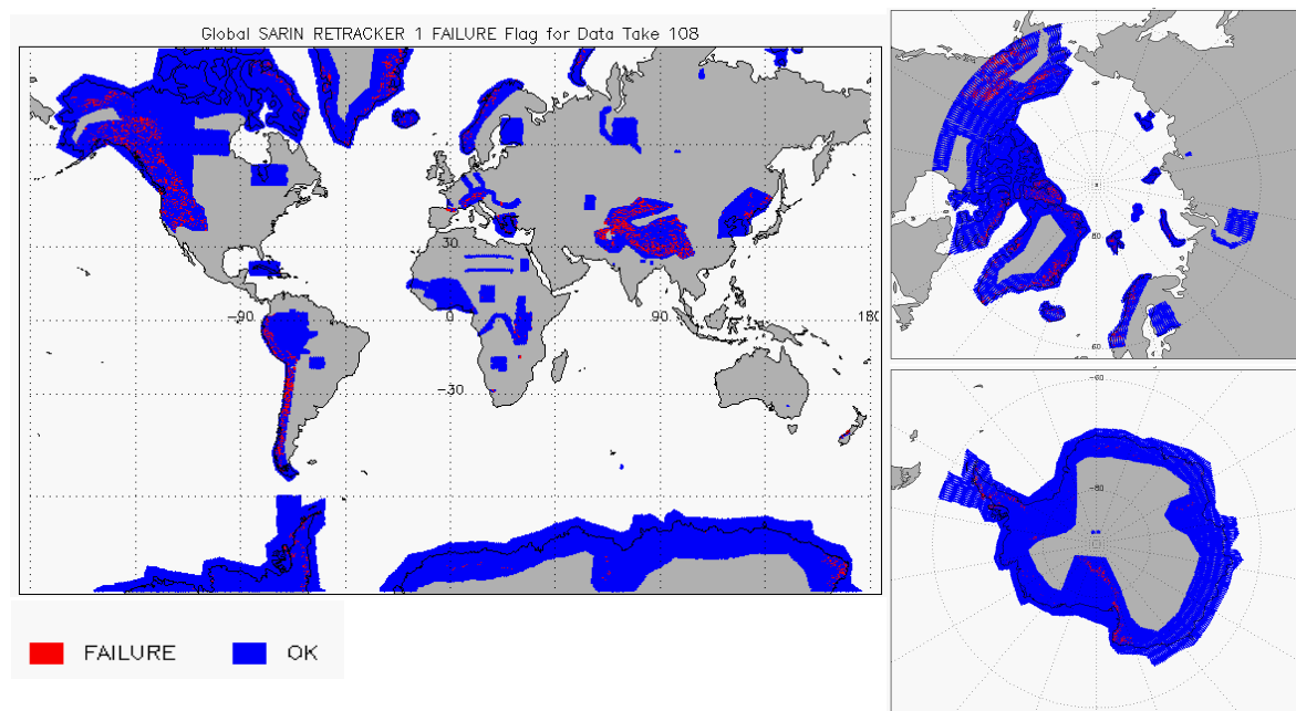
Figure 11 – Global plots showing Retracker Failure Flags for SARIn mode for cycle #108
