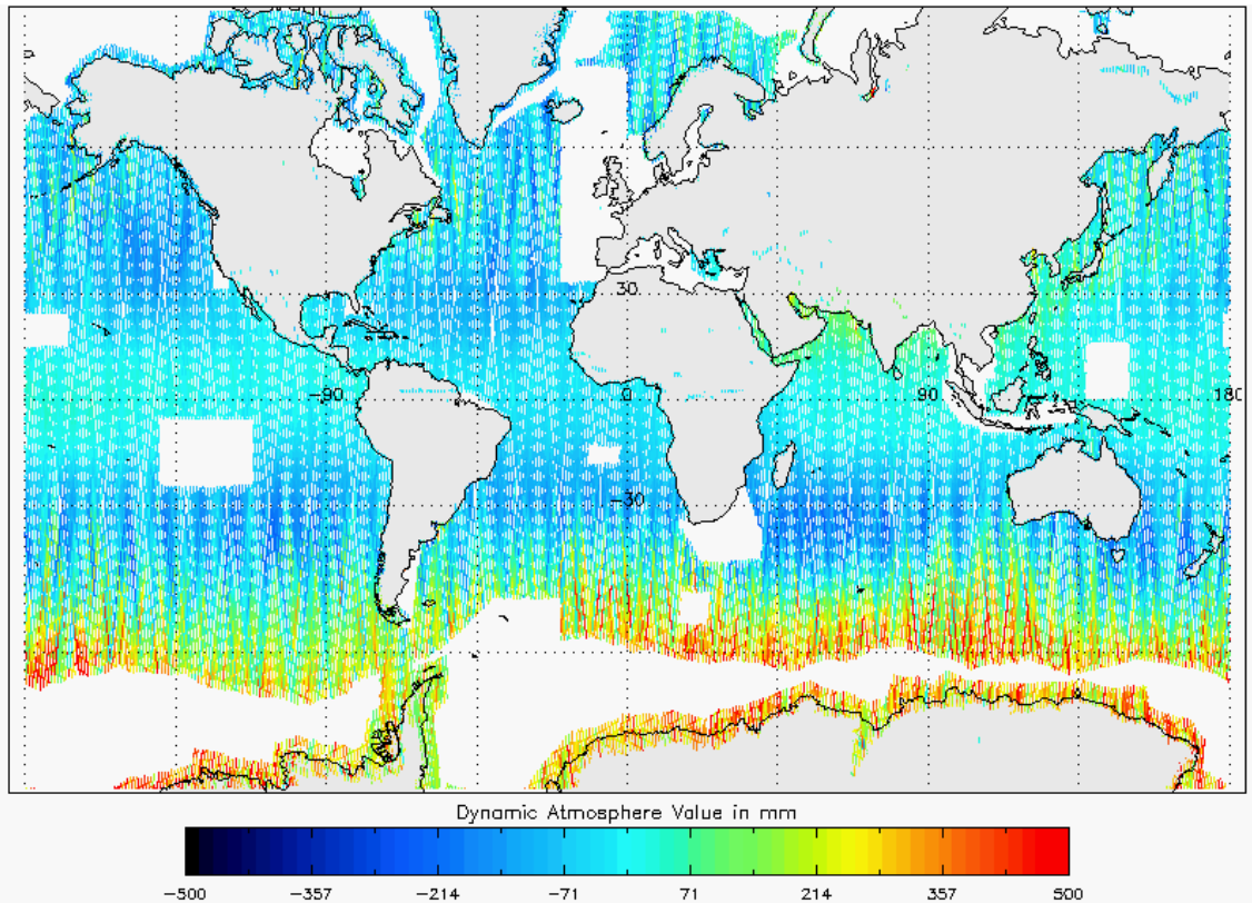
Figure 22 - Global plot of Dynamic Atmospheric Correction for cycle #106
