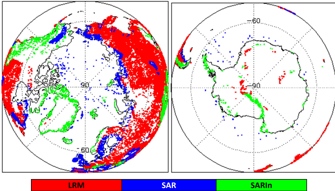
Figure 2 - Polar plots showing areas of loss of track in all SIRAL modes L0 data during June 2019.
