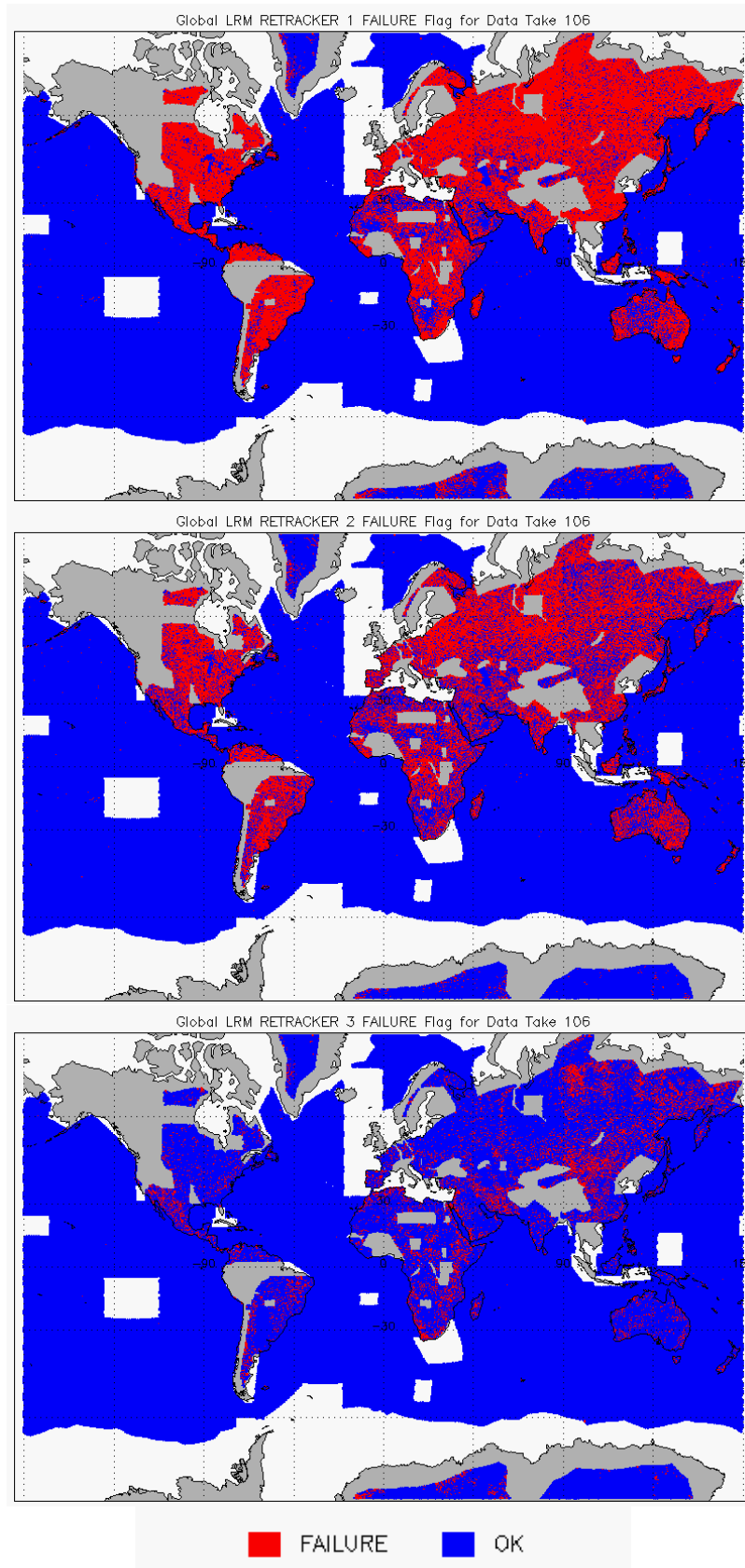
Figure 9 – Global plots showing Retracker Failure Flags for LRM mode for cycle #106: LRM CFI (top), LRM LIRT (middle), LRM OCOG (bottom)
