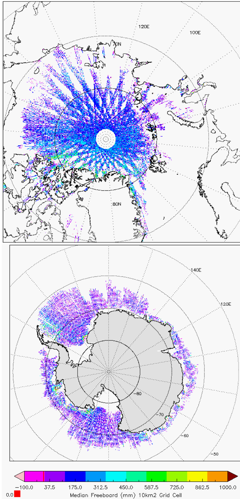
Figure 6 - Polar plots of 10km Gridded Freeboard values from L2 SAR products in cycle #106.
