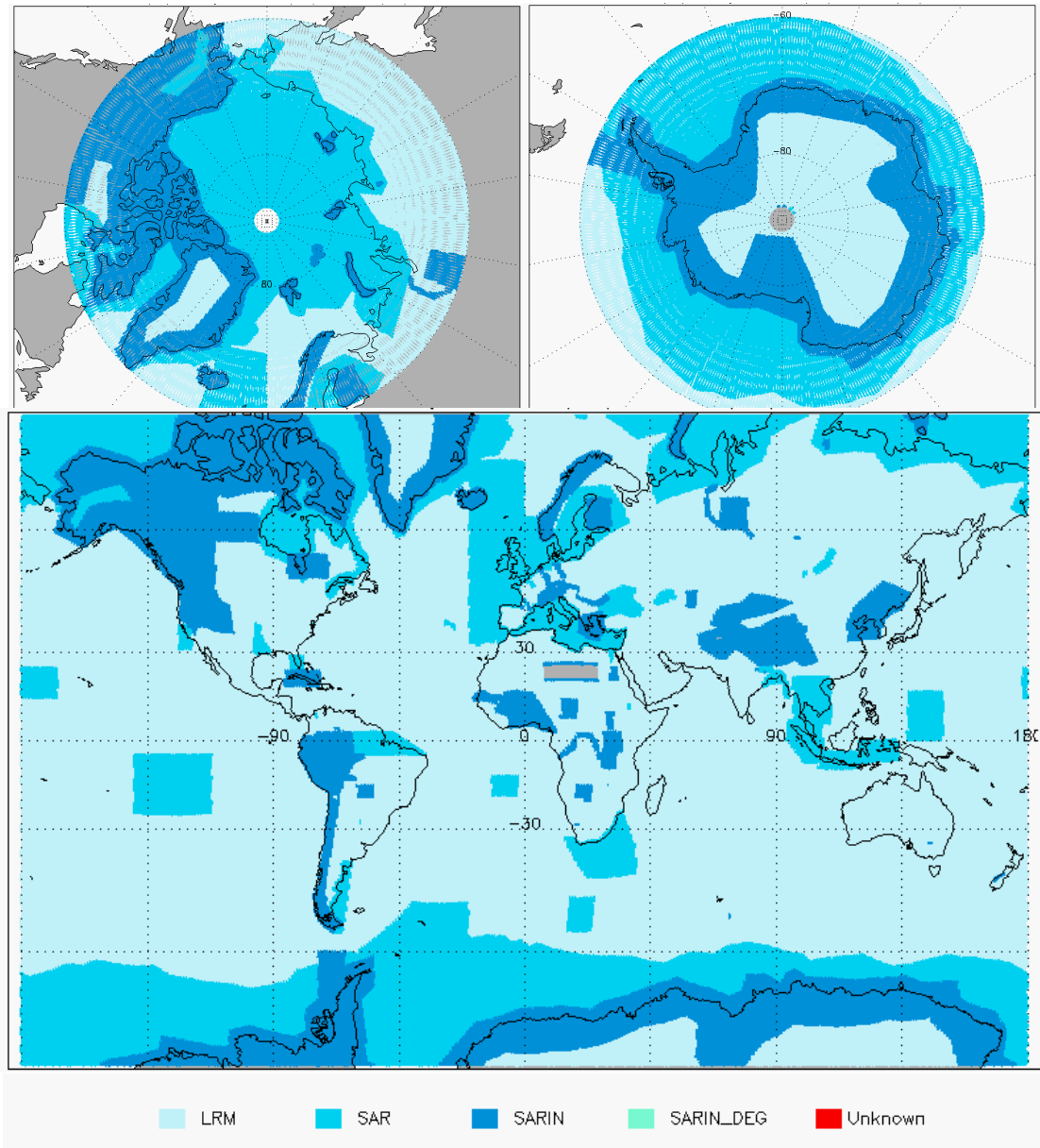
Figure 3 - Global and Polar plots of SIRAL Modes for cycle #106.
