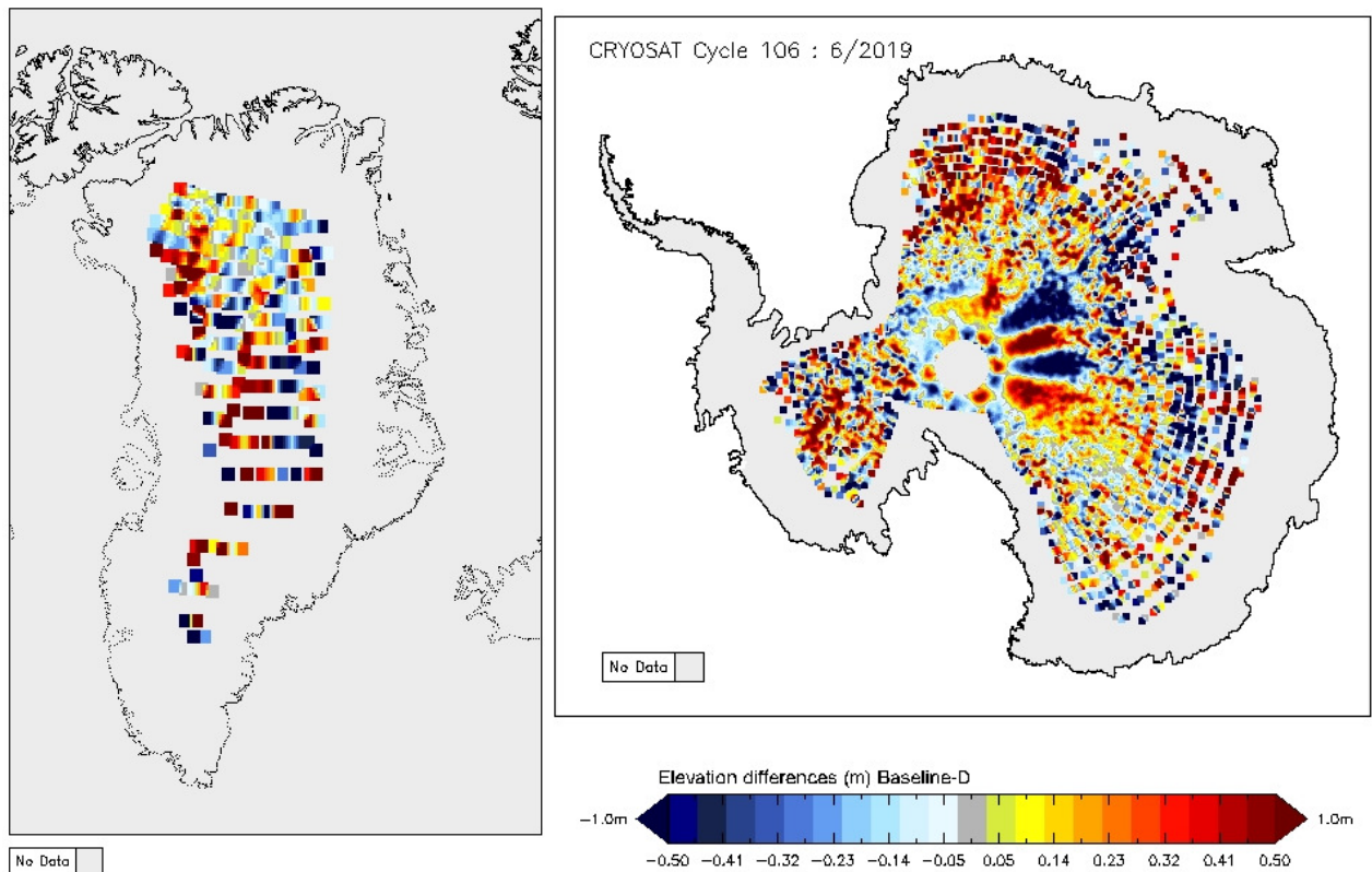
Figure 14 - Greenland and Antarctica maps of LRM elevation differences for cycle #106.
