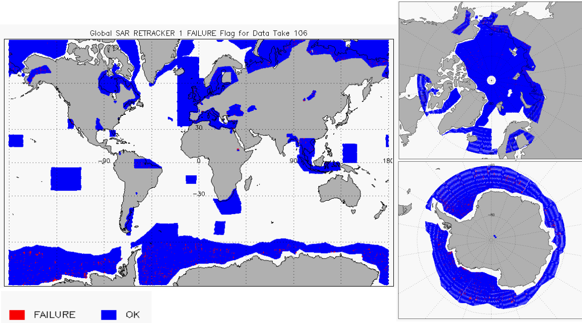
Figure 10 – Global plots showing Retracker Failure Flags for SAR mode for cycle #106
