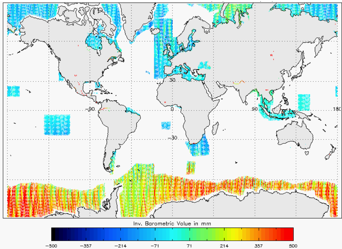
Figure 20 - Global plot of Inverse Barometric Correction for cycle #106
