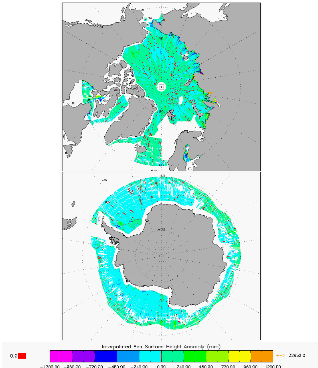
Figure 7 –Polar plots of SSHA for cycle #106.
