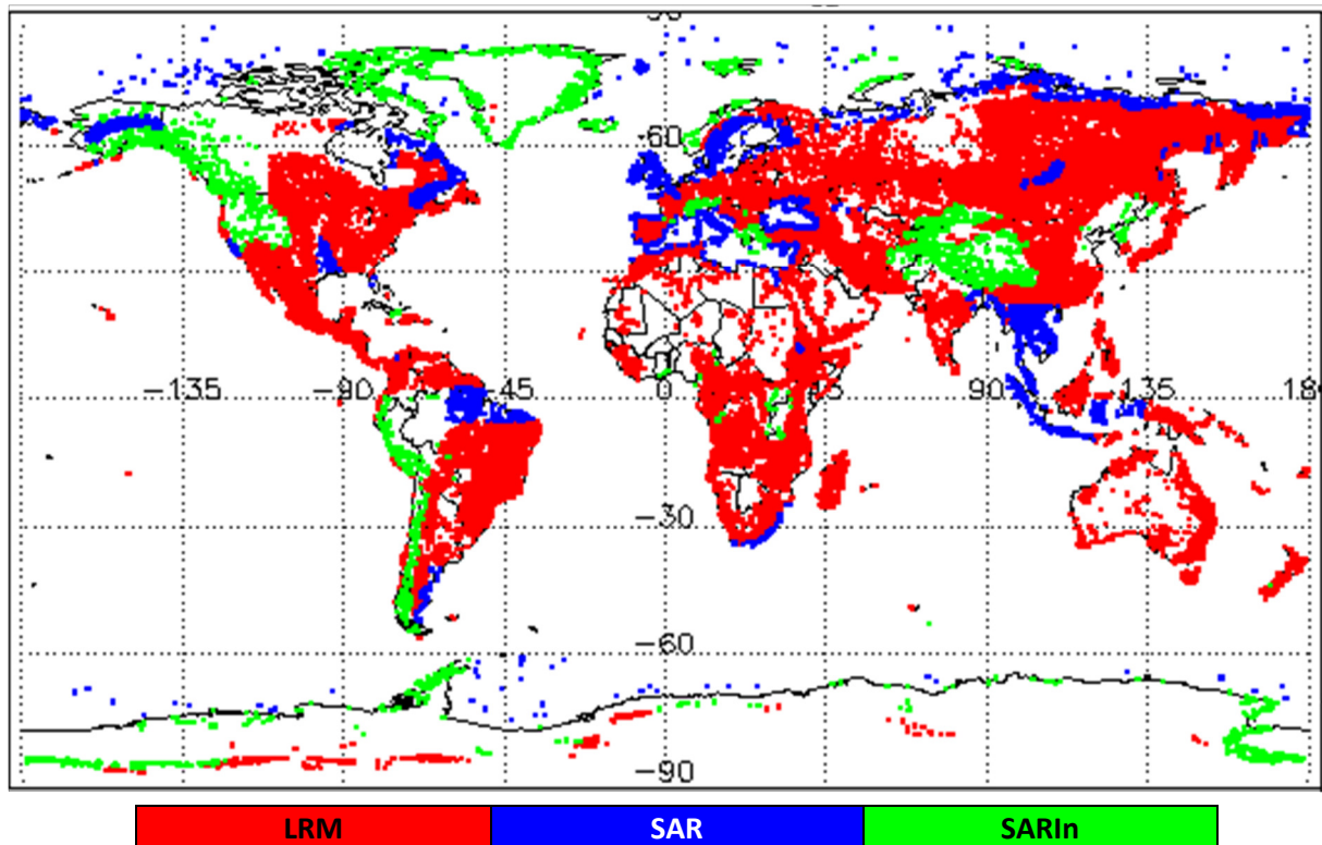
Figure 1 - Global plot showing areas of loss of track in all SIRAL modes L0 data during June 2019.
