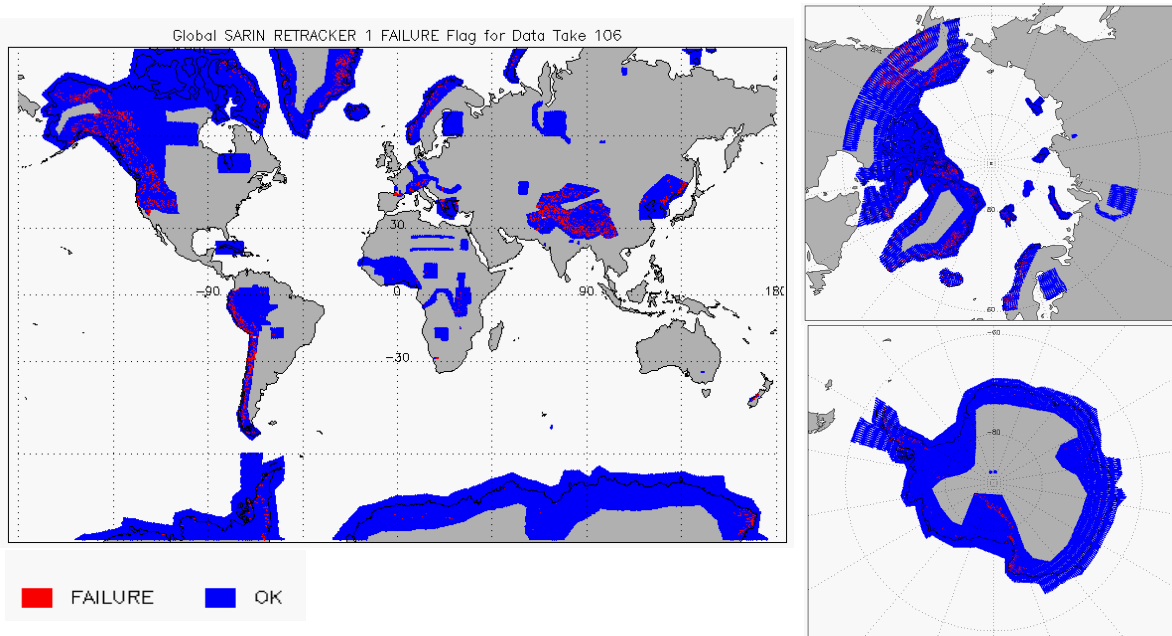
Figure 11 – Global plots showing Retracker Failure Flags for SARIn mode for cycle #106
