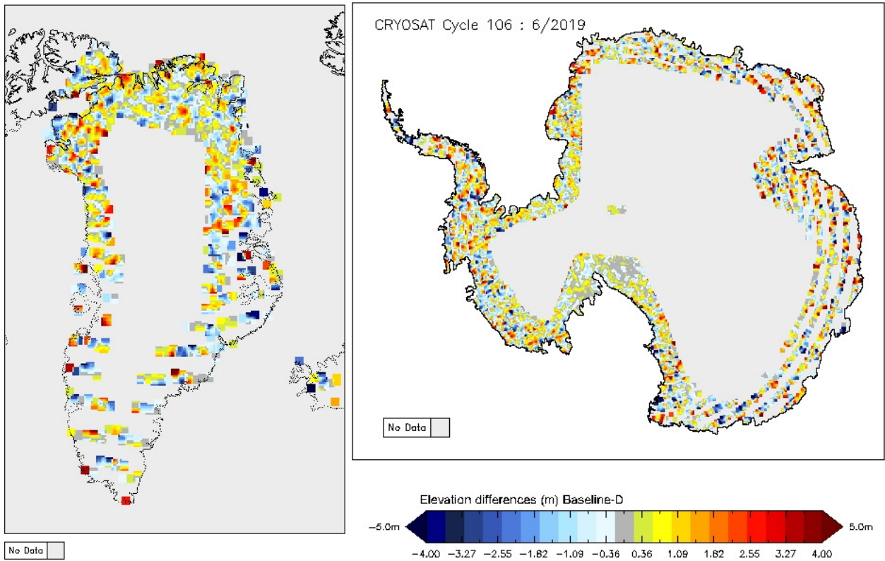
Figure 15 - Greenland and Antarctica maps of SARIn elevation differences for cycle #106
