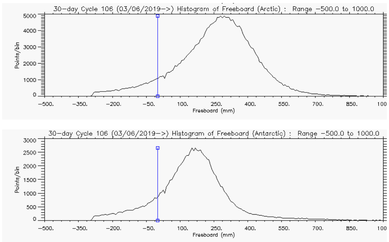
Figure 5 – Histogram of Freeboard for Arctic (above) and Antarctic (below) for cycle #106
