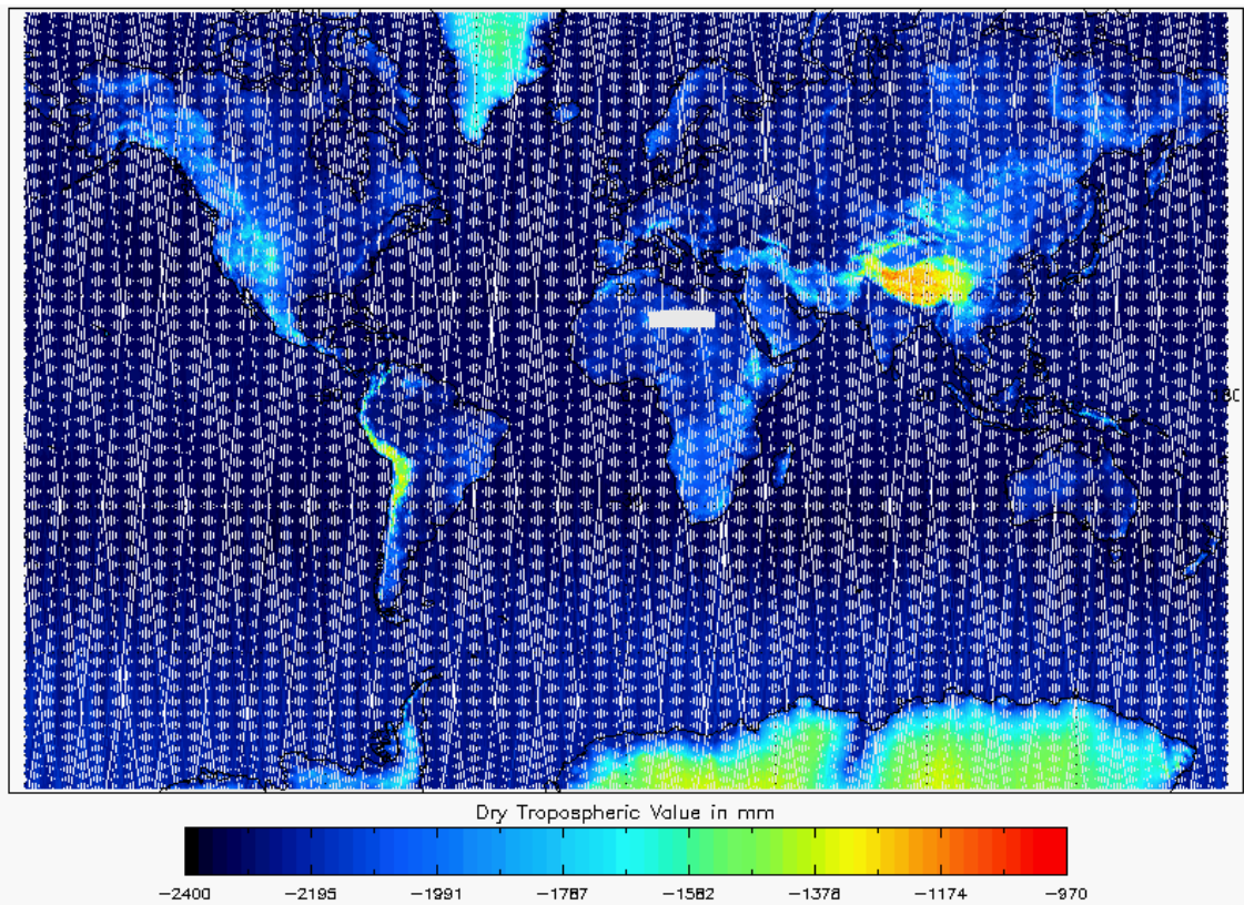
Figure 16 - Global plot of Dry Tropospheric Correction for cycle #106
