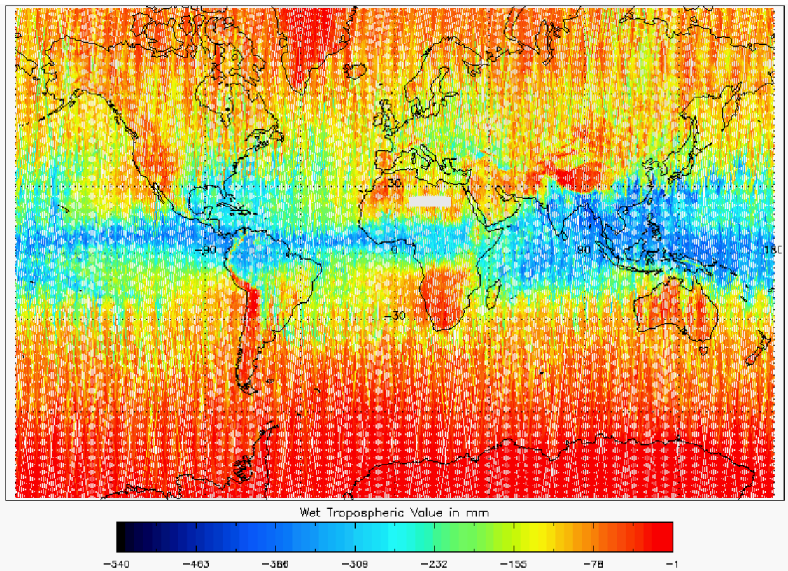
Figure 18 - Global plot of Wet Tropospheric Correction for cycle #106
