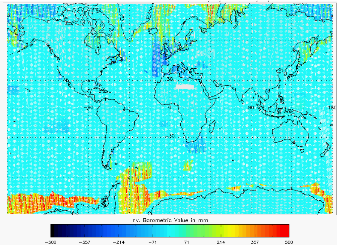
Figure 20 - Global plot of Inverse Barometric Correction for cycle #103
