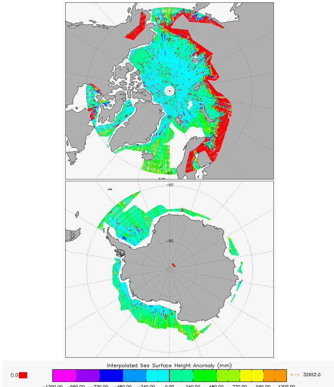
Figure 7 –Polar plots of SSHA for cycle #103.
