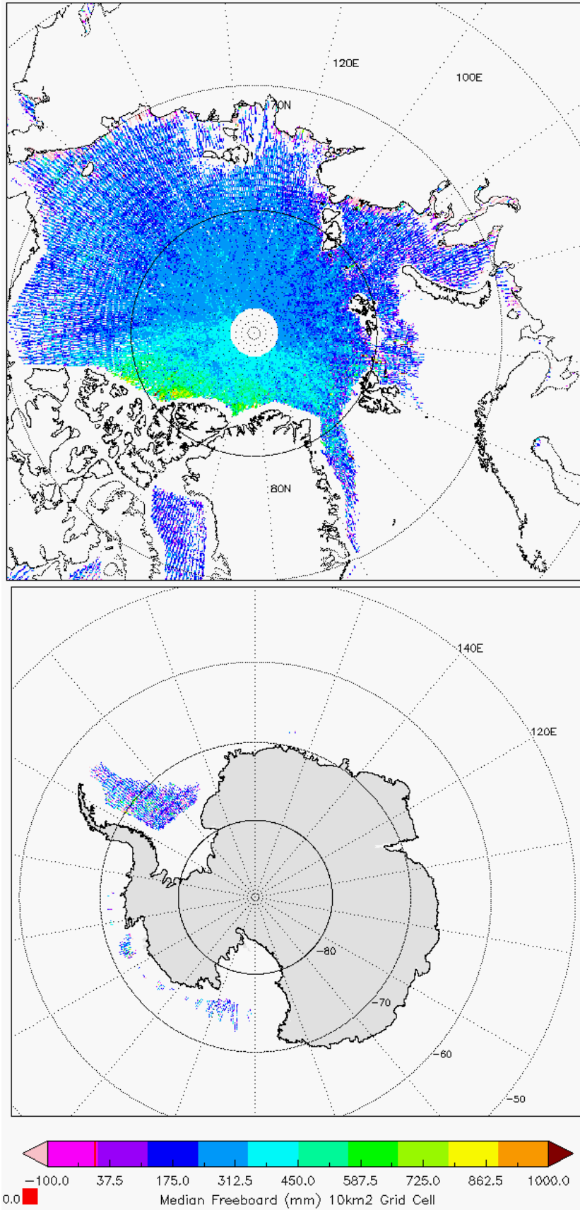
Figure 6 - Polar plots of 10km Gridded Freeboard values from L2 SAR products in cycle #103.
