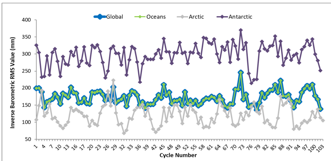
Figure 23 – Dynamic Atmospheric Correction RMS value trend from beginning of mission
