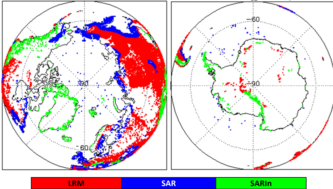
Figure 2 - Polar plots showing areas of loss of track in all SIRAL modes L0 data during March 2019.
