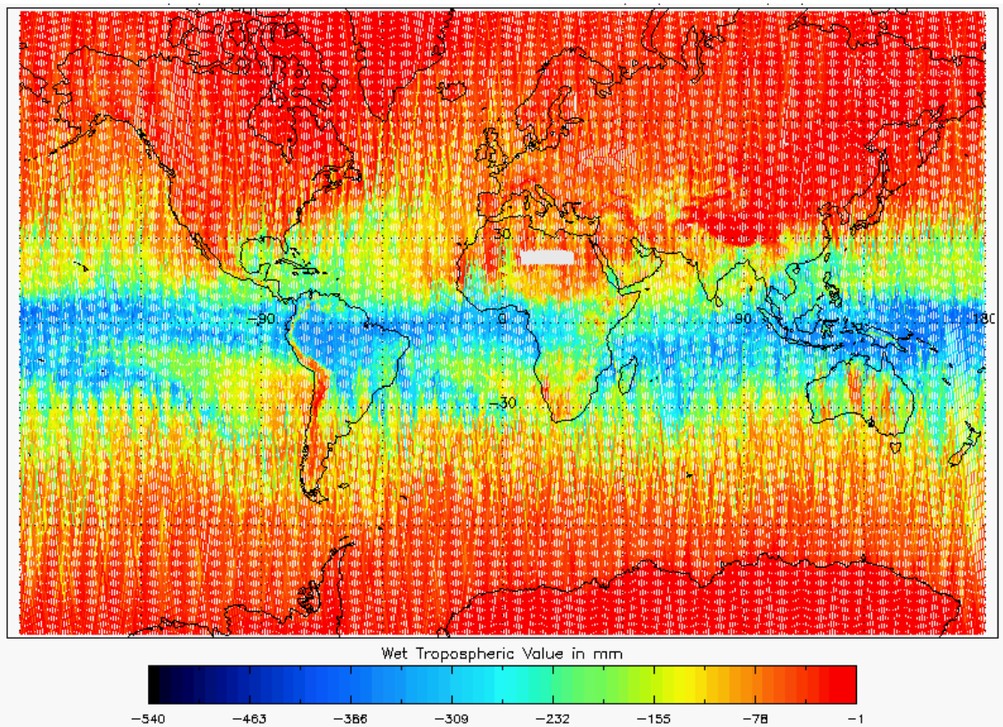
Figure 18 - Global plot of Wet Tropospheric Correction for cycle #103
