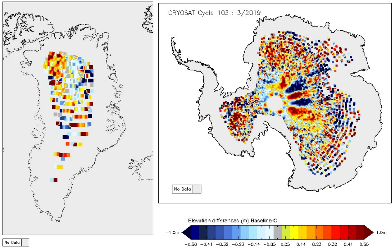
Figure 14 - Greenland and Antarctica maps of LRM elevation differences for cycle #103.
