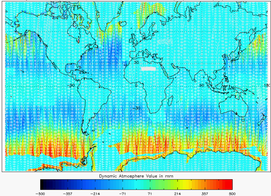
Figure 22 - Global plot of Dynamic Atmospheric Correction for cycle #103
