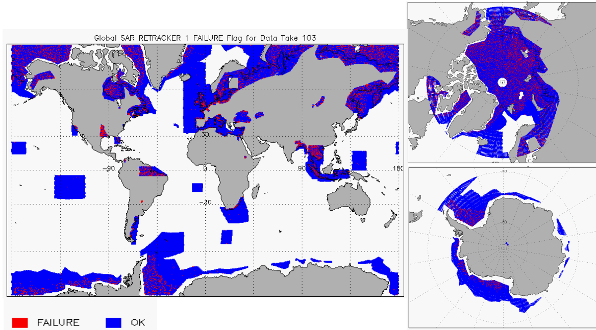
Figure 10 – Global plots showing Retracker Failure Flags for SAR mode for cycle #103
