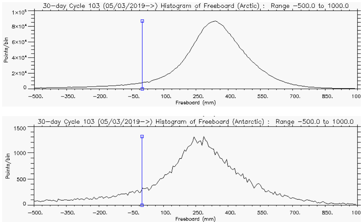
Figure 5 – Histogram of Freeboard for Arctic (above) and Antarctic (below) for cycle #103
