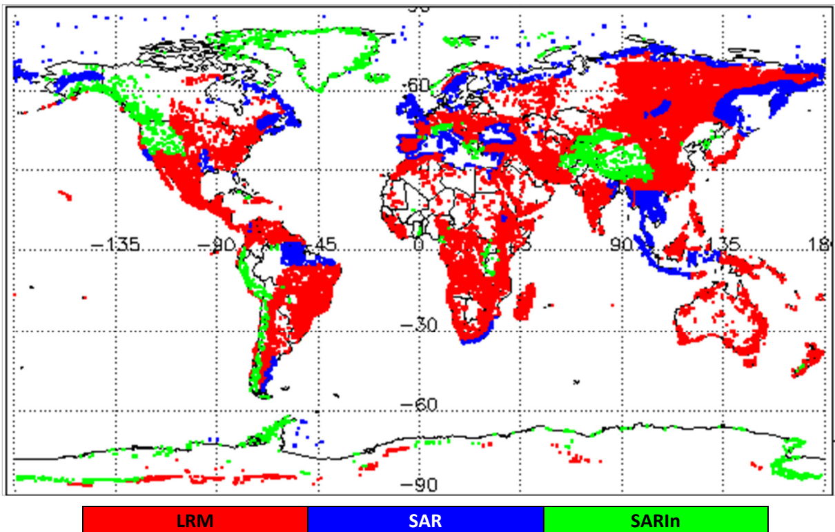
Figure 1 - Global plot showing areas of loss of track in all SIRAL modes L0 data during March 2019.
