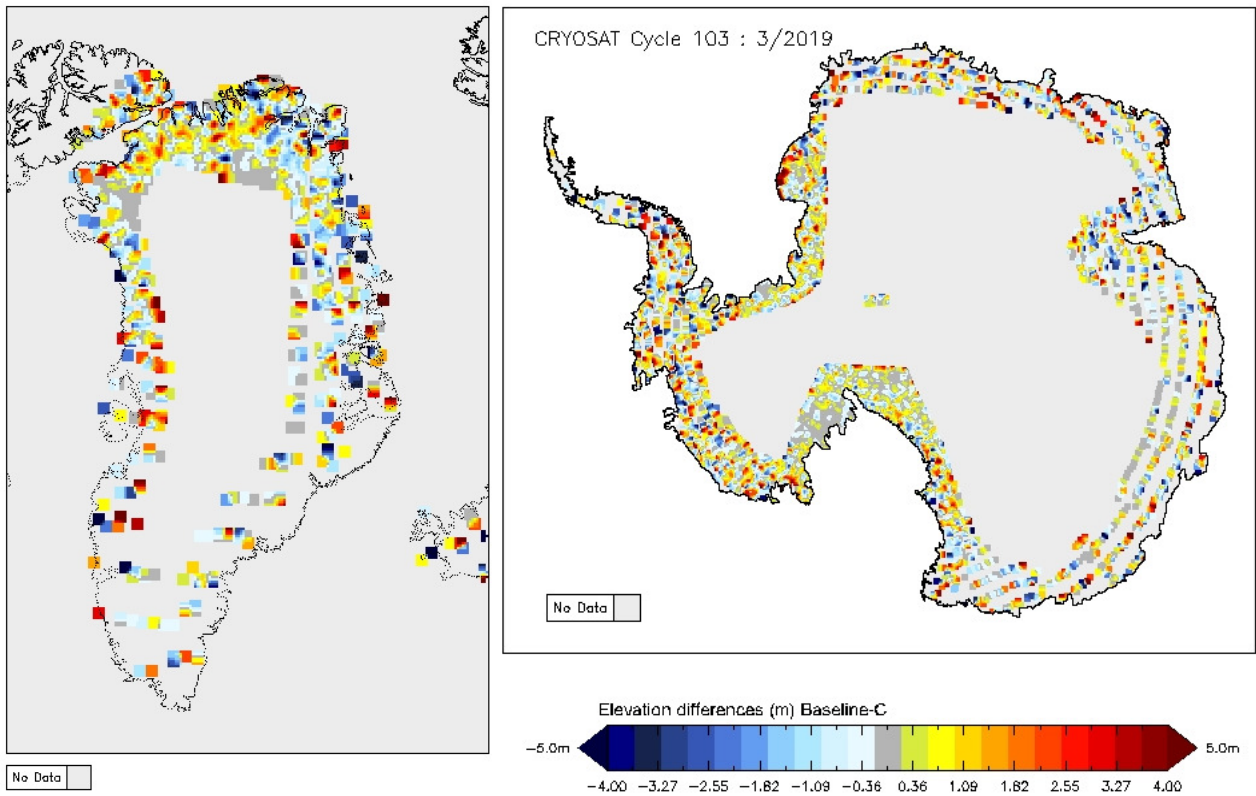
Figure 15 - Greenland and Antarctica maps of SARIn elevation differences for cycle #103
