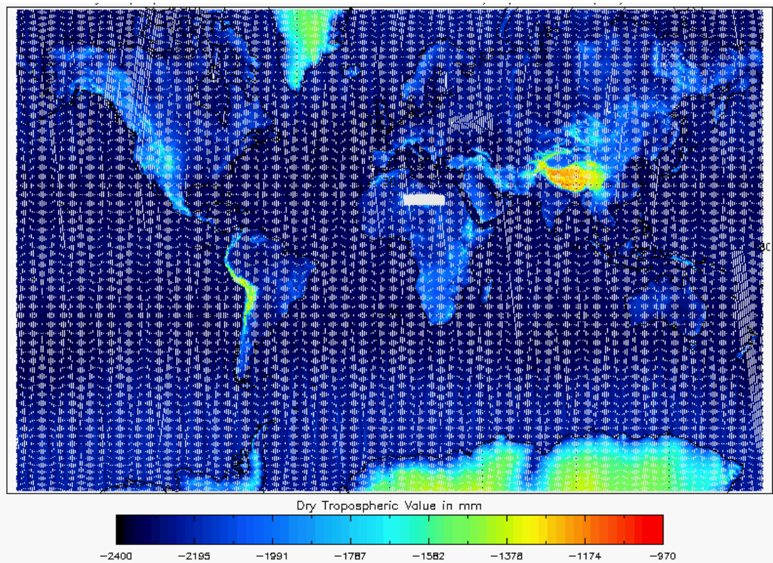
Figure 16 - Global plot of Dry Tropospheric Correction for cycle #103
