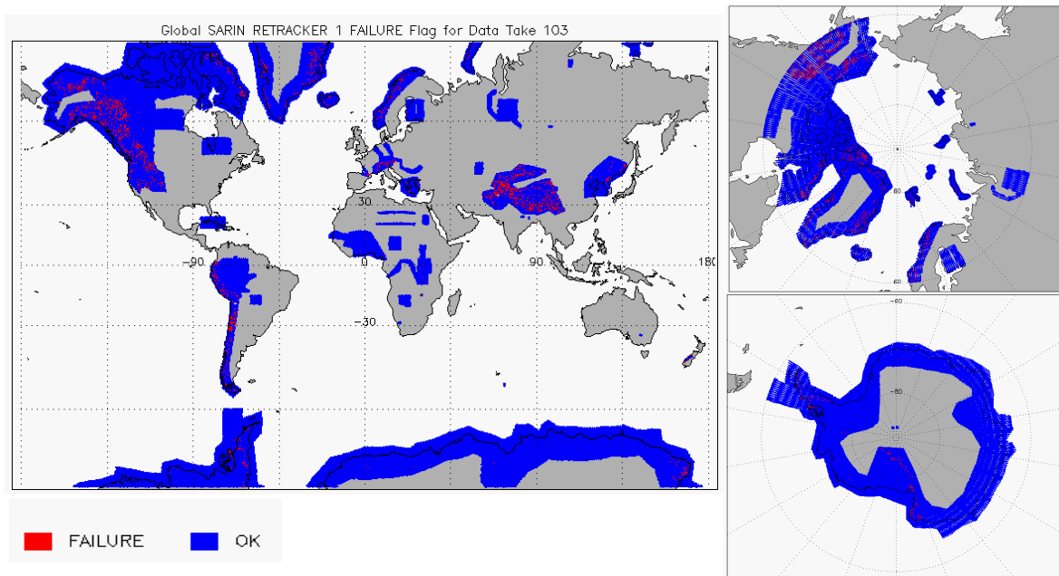
Figure 11 – Global plots showing Retracker Failure Flags for SARIn mode for cycle #103
