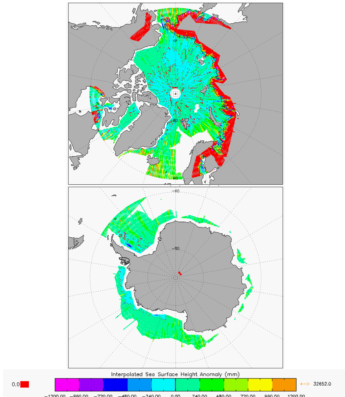
Figure 7 –Polar plots of SSHA for cycle #102.
