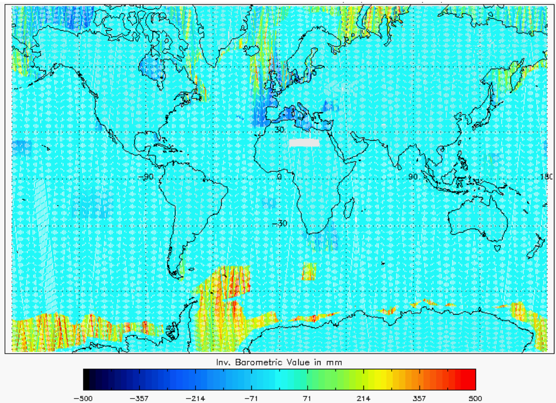
Figure 20 - Global plot of Inverse Barometric Correction for cycle #102
