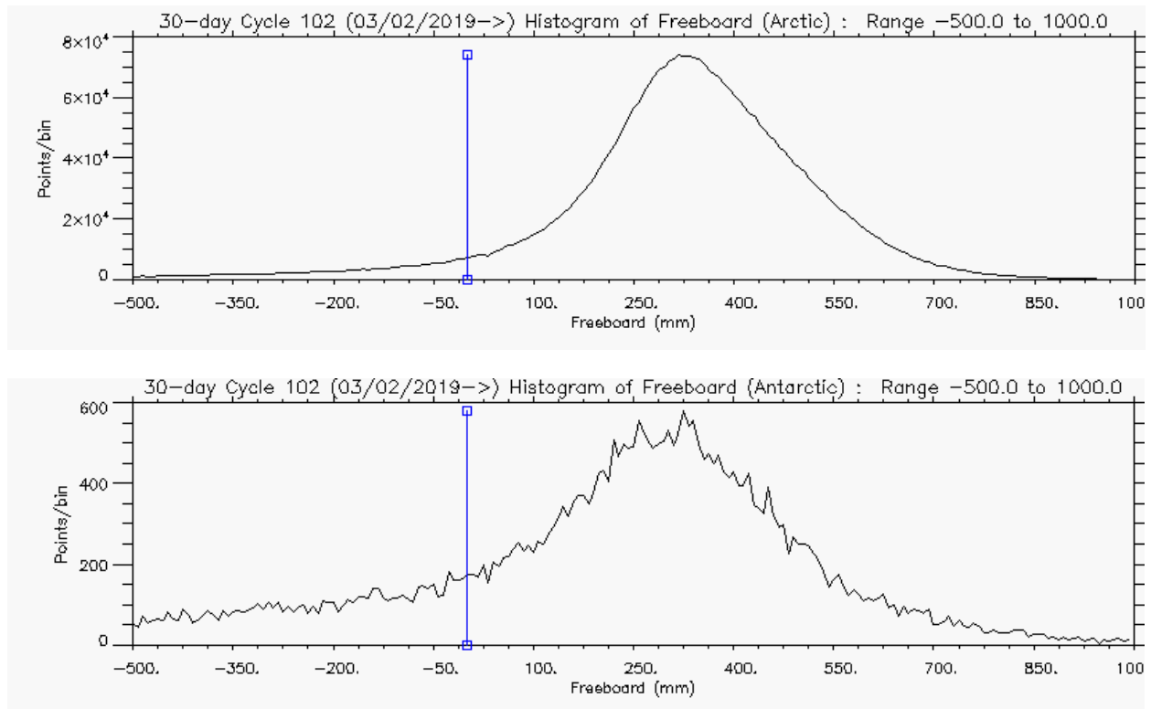
Figure 5 – Histogram of Freeboard for Arctic (above) and Antarctic (below) for cycle #102
