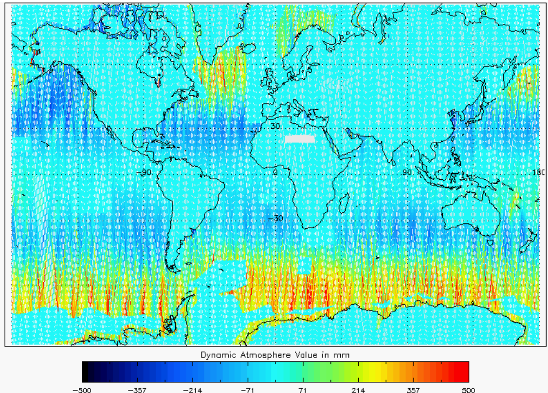
Figure 22 - Global plot of Dynamic Atmospheric Correction for cycle #102
