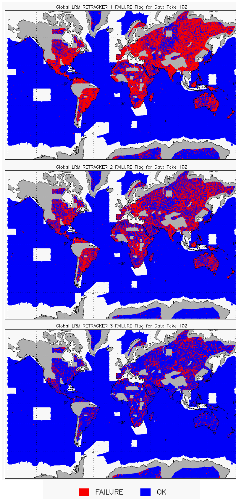
Figure 9 – Global plots showing Retracker Failure Flags for LRM mode for cycle #102:
