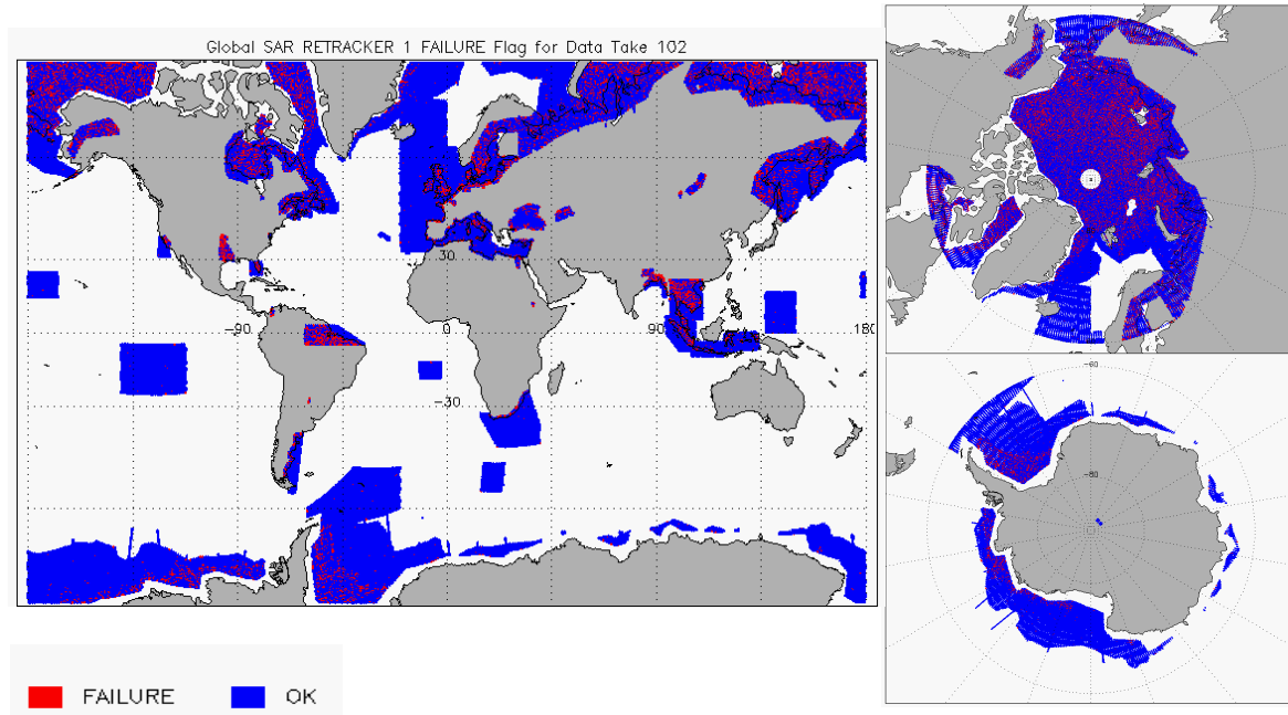
Figure 10 – Global plots showing Retracker Failure Flags for SAR mode for cycle #102
