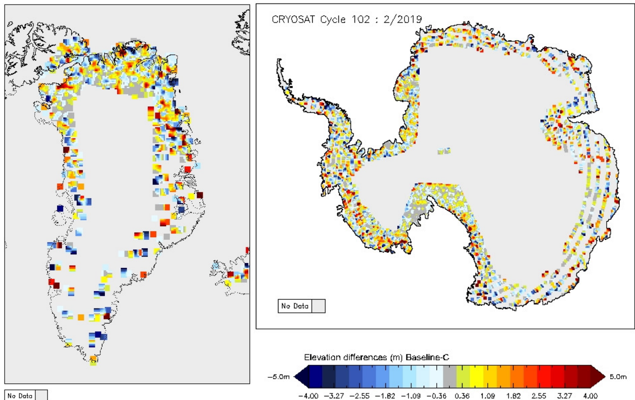
Figure 15 - Greenland and Antarctica maps of SARIn elevation differences for cycle #102
