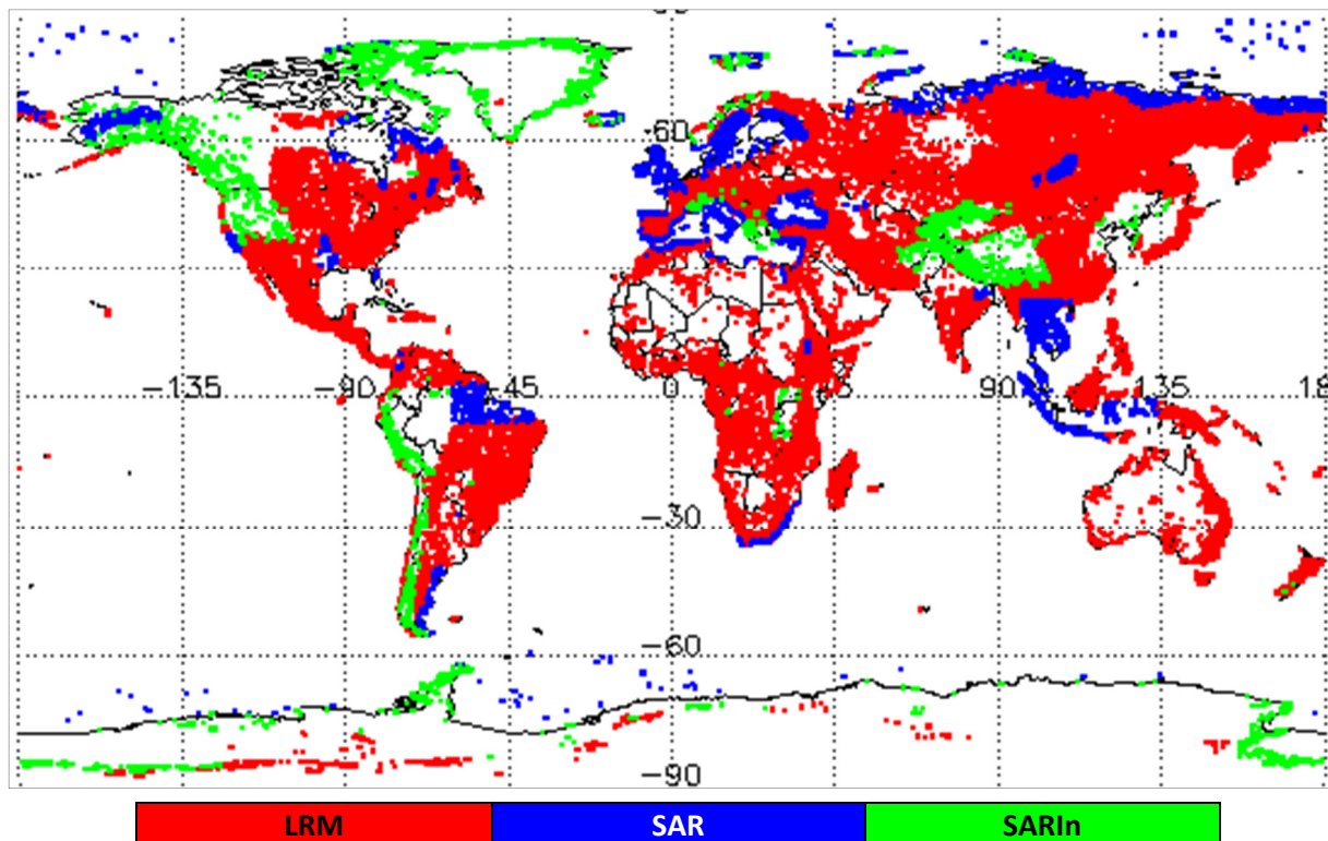
Figure 1 - Global plot showing areas of loss of track in all SIRAL modes L0 data during February 2019.
