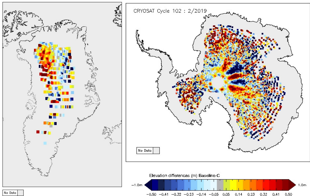
Figure 14 - Greenland and Antarctica maps of LRM elevation differences for cycle #102.
