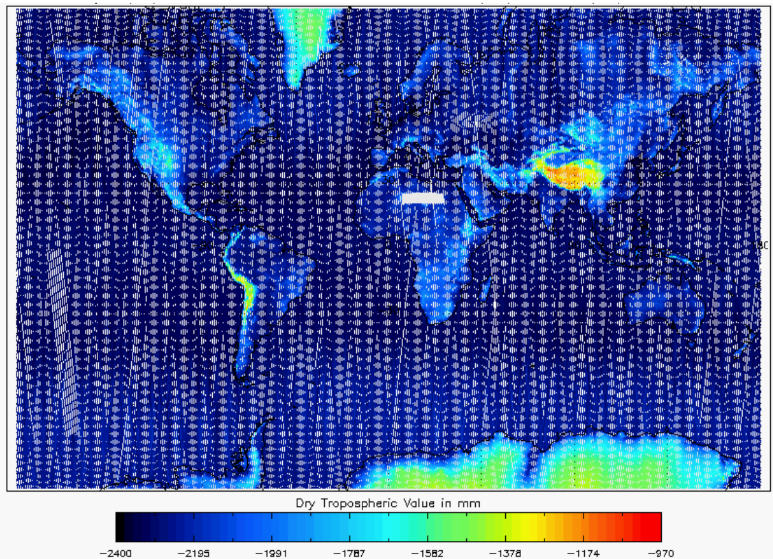
Figure 16 - Global plot of Dry Tropospheric Correction for cycle #102
