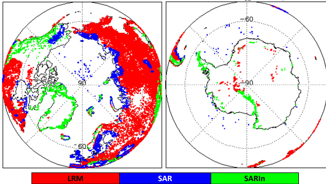
Figure 2 - Polar plots showing areas of loss of track in all SIRAL modes L0 data during February 2019.
