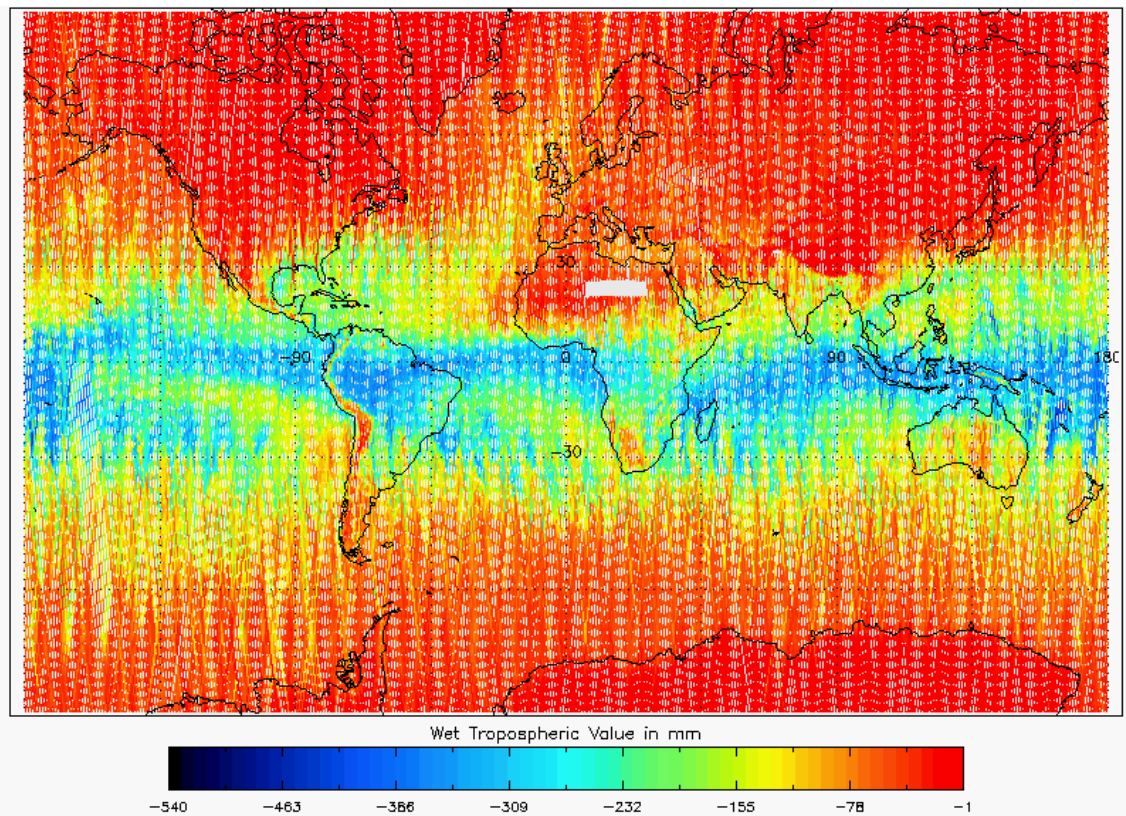
Figure 18 - Global plot of Wet Tropospheric Correction for cycle #102
