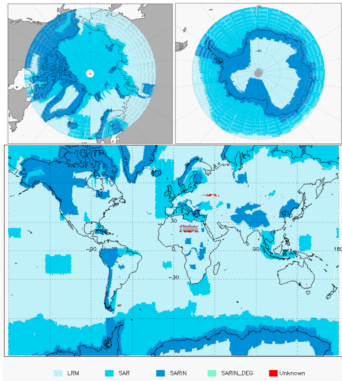
Figure 3 - Global and Polar plots of SIRAL Modes for cycle #102.
