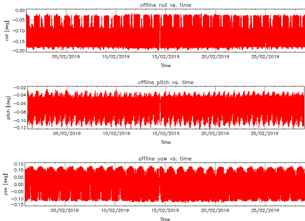
Figure 4 – Roll (top), Pitch (middle) and Yaw (bottom) values for L1B Products during cycle #102.
