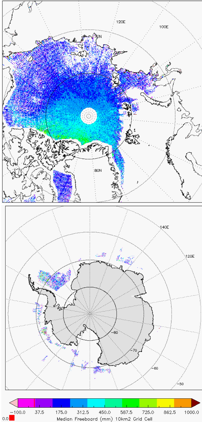
Figure 6 - Polar plots of 10km Gridded Freeboard values from L2 SAR products in cycle #100.
