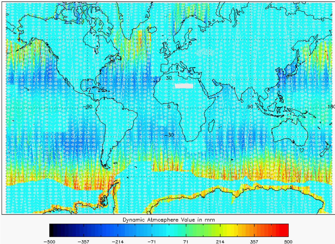
Figure 22 - Global plot of Dynamic Atmospheric Correction for cycle #100
