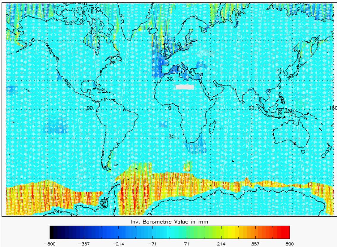
Figure 20 - Global plot of Inverse Barometric Correction for cycle #100
