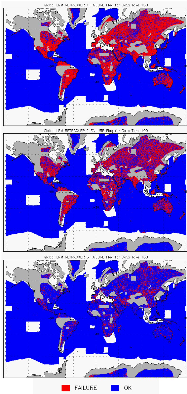
Figure 9 – Global plots showing Retracker Failure Flags for LRM mode for cycle #100: LRM CFI (top), LRM LIRT (middle), LRM OCOG (bottom)
