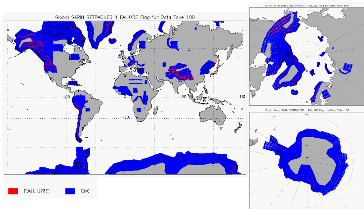
Figure 11 – Global plots showing Retracker Failure Flags for SARIn mode for cycle #100
