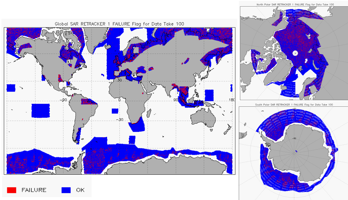
Figure 10 – Global plots showing Retracker Failure Flags for SAR mode for cycle #100
