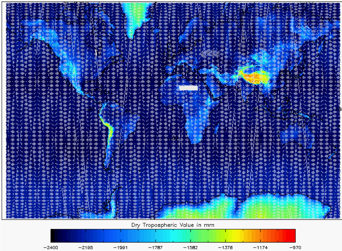
Figure 16 - Global plot of Dry Tropospheric Correction for cycle #100
