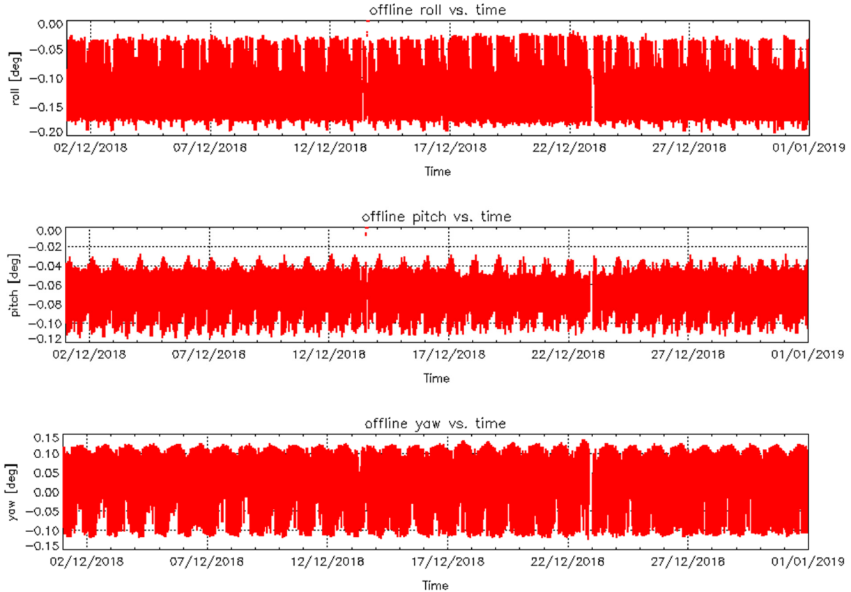
Figure 4 – Roll (top), Pitch (middle) and Yaw (bottom) values for L1B Products during cycle #100.
