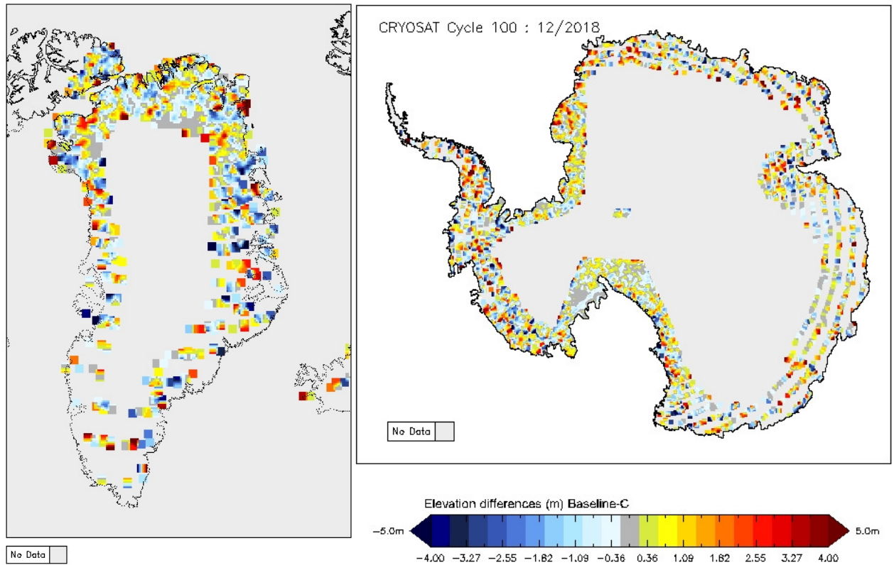
Figure 15 - Greenland and Antarctica maps of SARIn elevation differences for cycle #100
