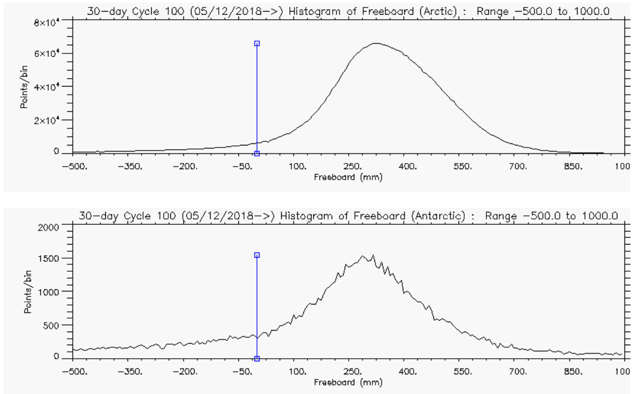
Figure 5 – Histogram of Freeboard for Arctic (above) and Antarctic (below) for cycle #100
