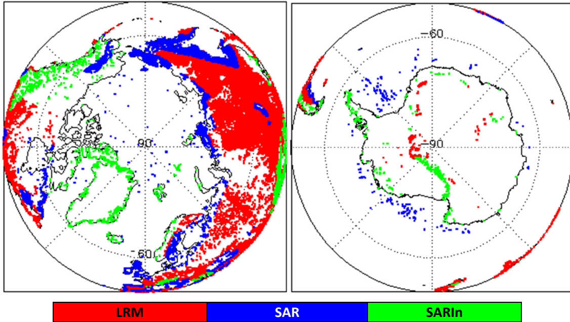
Figure 2 - Polar plots showing areas of loss of track in all SIRAL modes L0 data during December 2018.
