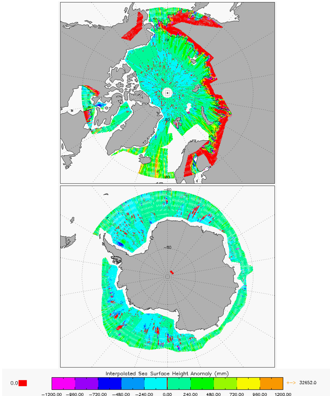
Figure 7 –Polar plots of SSHA for cycle #100.
