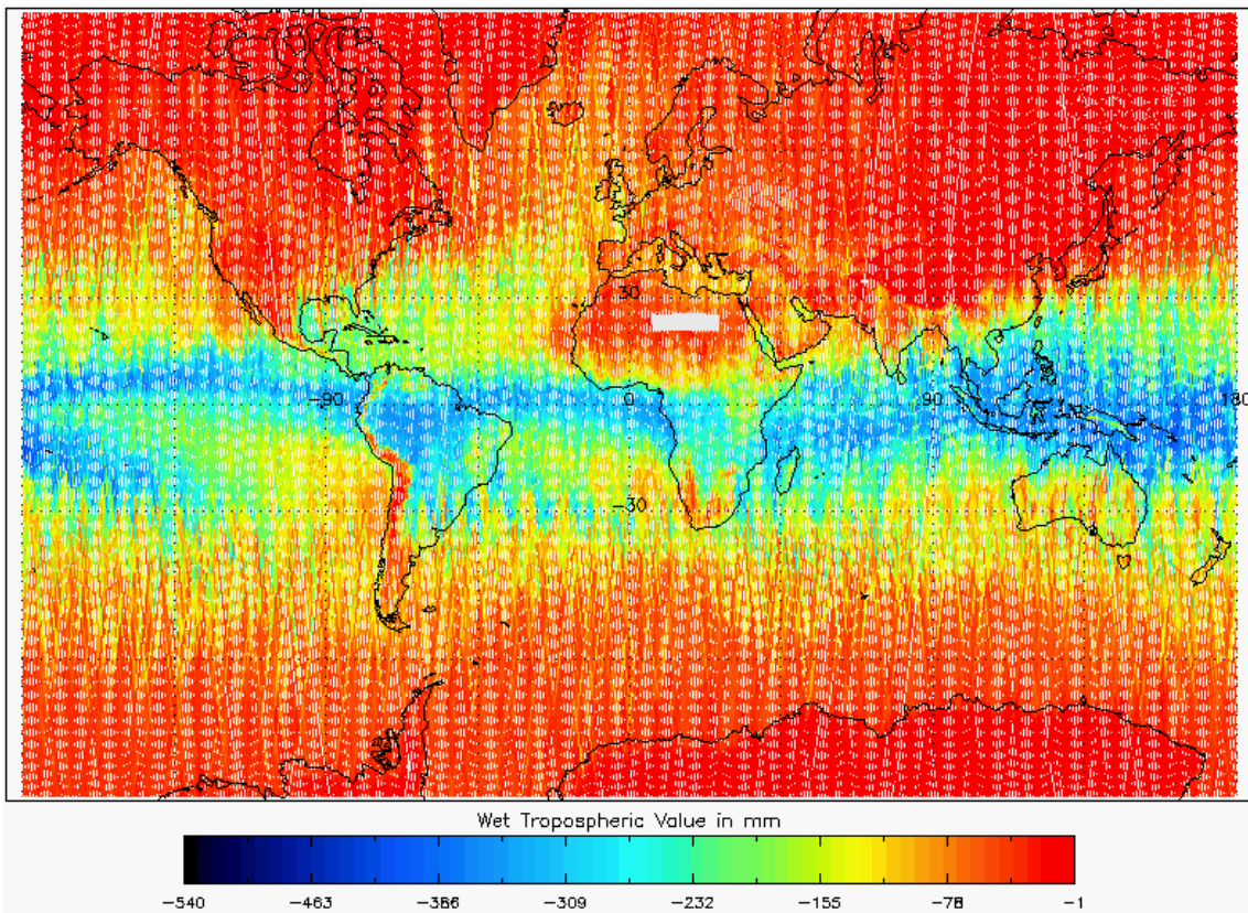
Figure 18 - Global plot of Wet Tropospheric Correction for cycle #100
