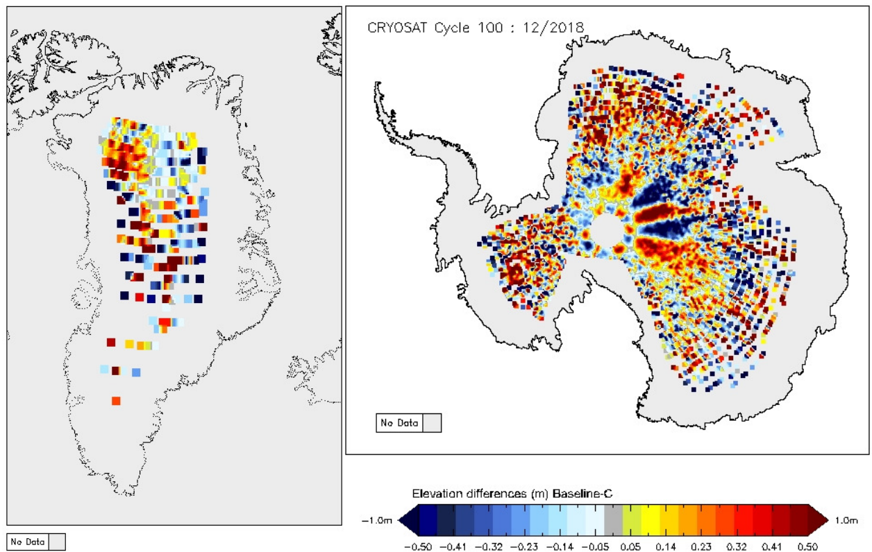
Figure 14 - Greenland and Antarctica maps of LRM elevation differences for cycle #100.
