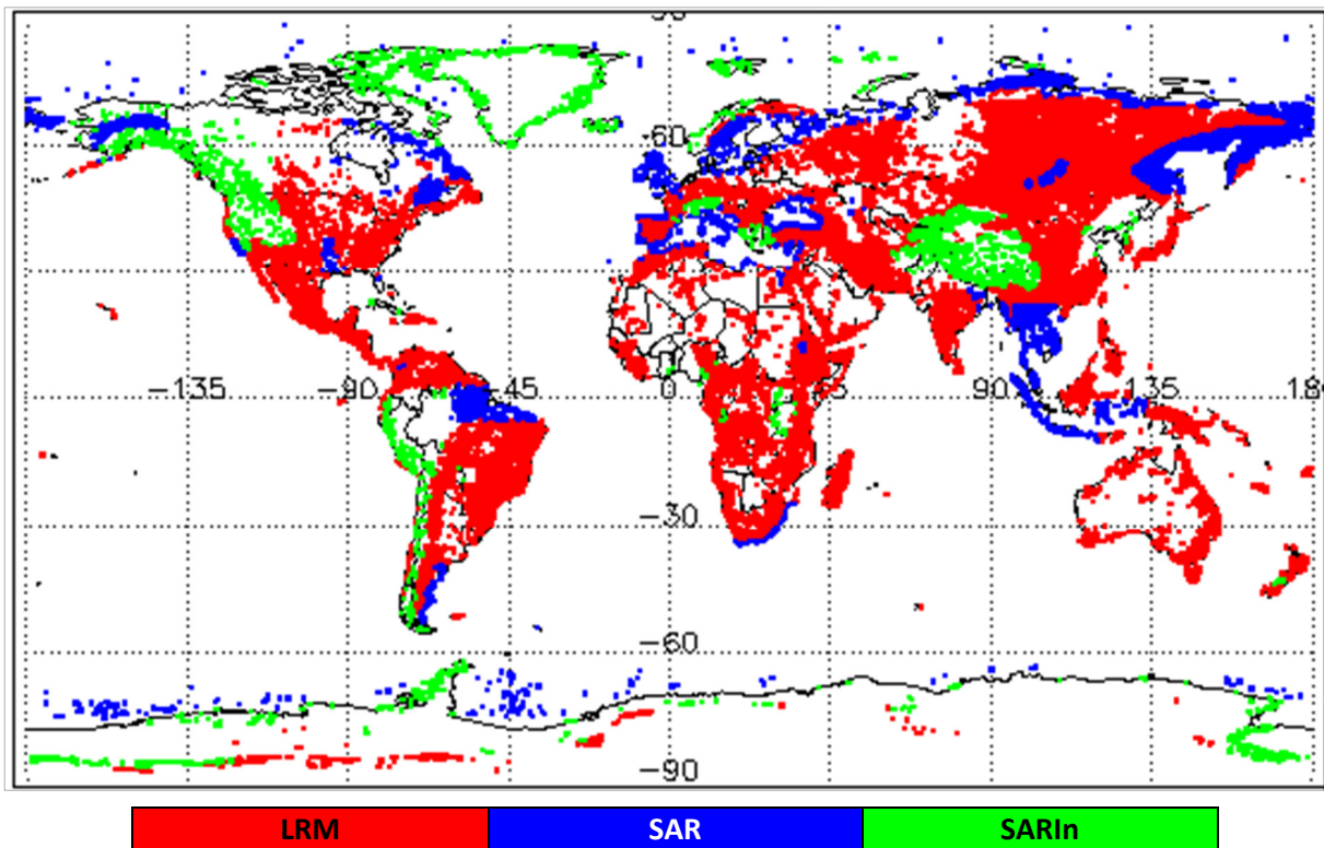
Figure 1 - Global plot showing areas of loss of track in all SIRAL modes L0 data during December 2018.
