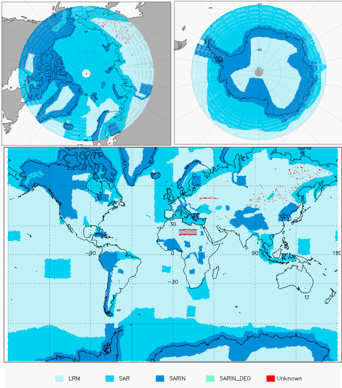
Figure 3 - Global and Polar plots of SIRAL Modes for cycle #100.
