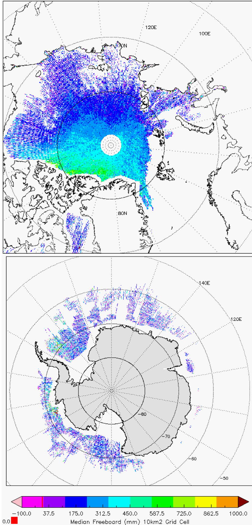
Figure 6 - Polar plots of 10km Gridded Freeboard values from L2 SAR products in cycle #99.
