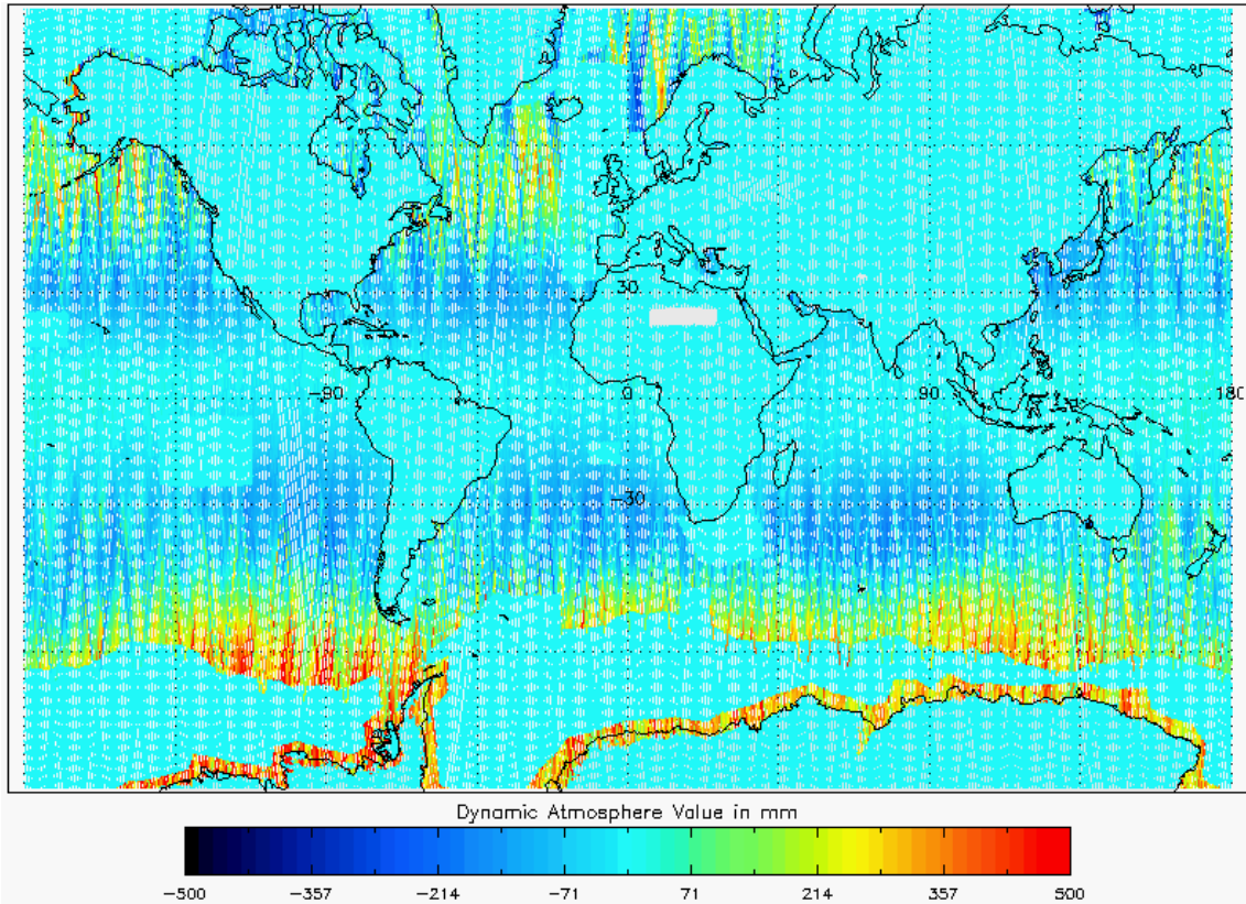
Figure 22 - Global plot of Dynamic Atmospheric Correction for cycle #99
