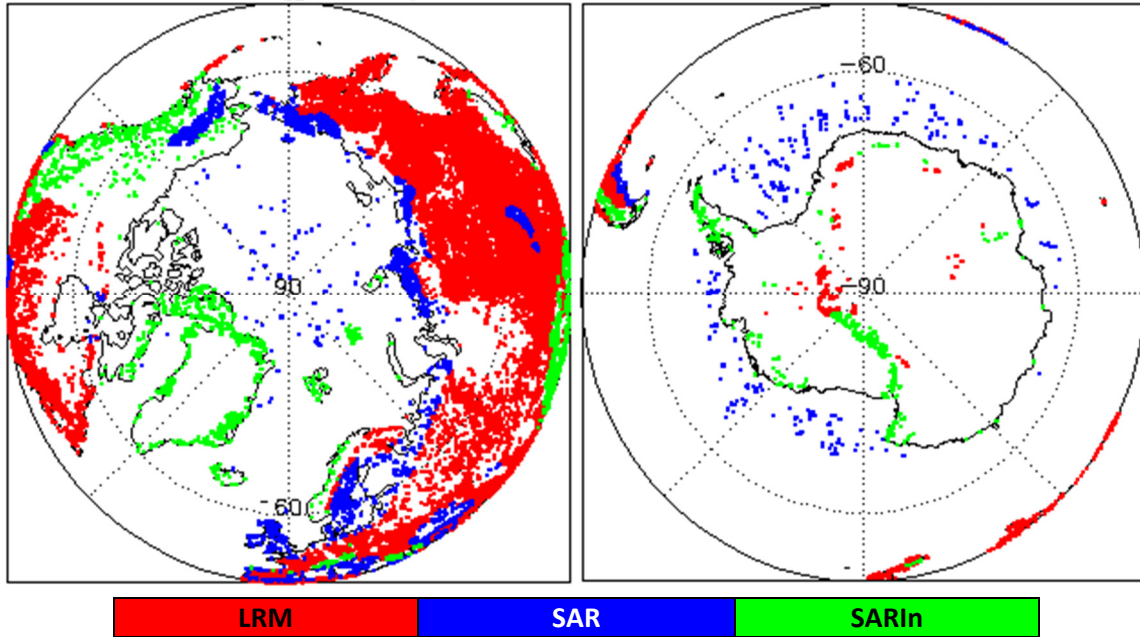
Figure 2 - Polar plots showing areas of loss of track in all SIRAL modes L0 data during November 2018.
