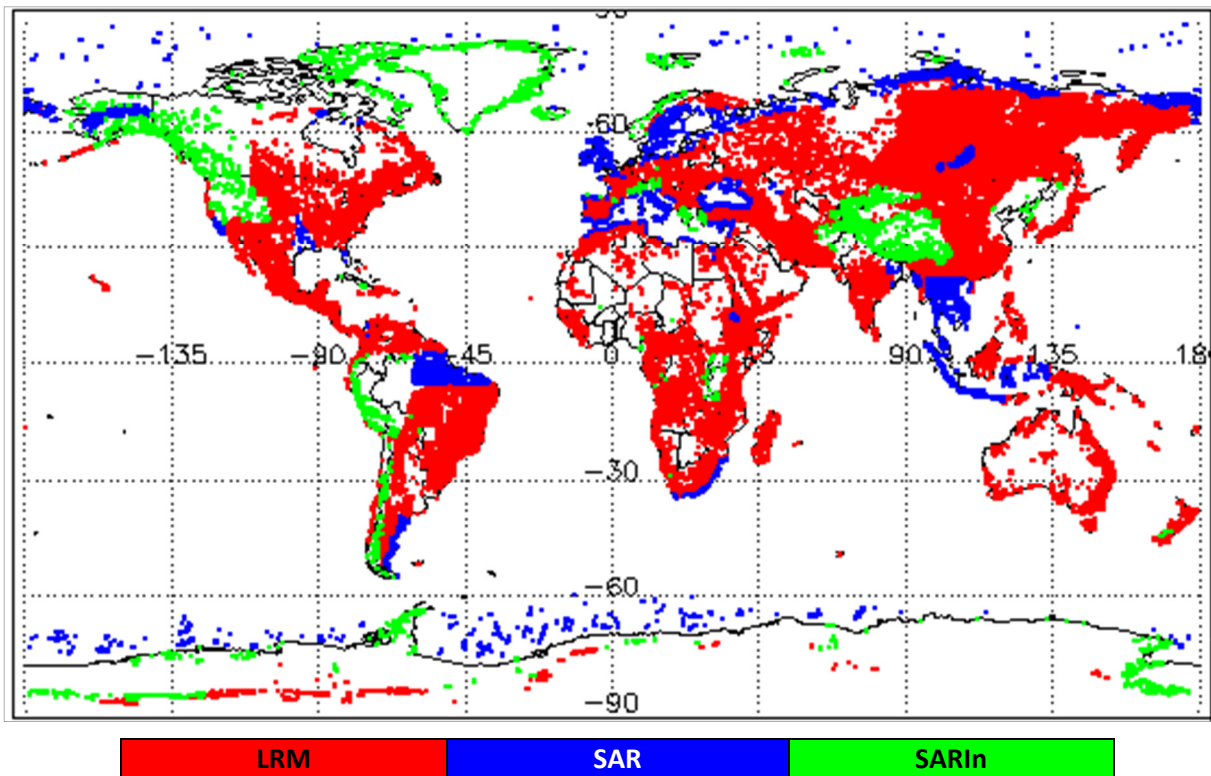
Figure 1 - Global plot showing areas of loss of track in all SIRAL modes L0 data during November 2018.
