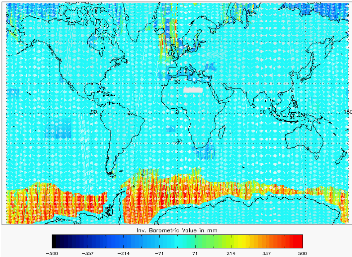
Figure 20 - Global plot of Inverse Barometric Correction for cycle #99
