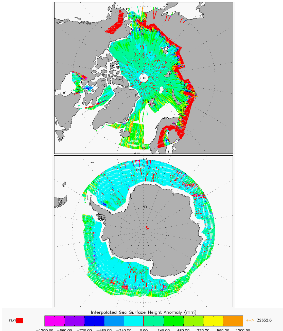
Figure 7 –Polar plots of SSHA for cycle #99.
