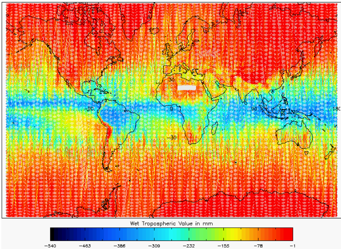
Figure 18 - Global plot of Wet Tropospheric Correction for cycle #99
