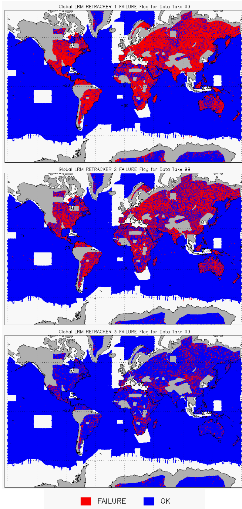
Figure 9 – Global plots showing Retracker Failure Flags for LRM mode for cycle #99:
