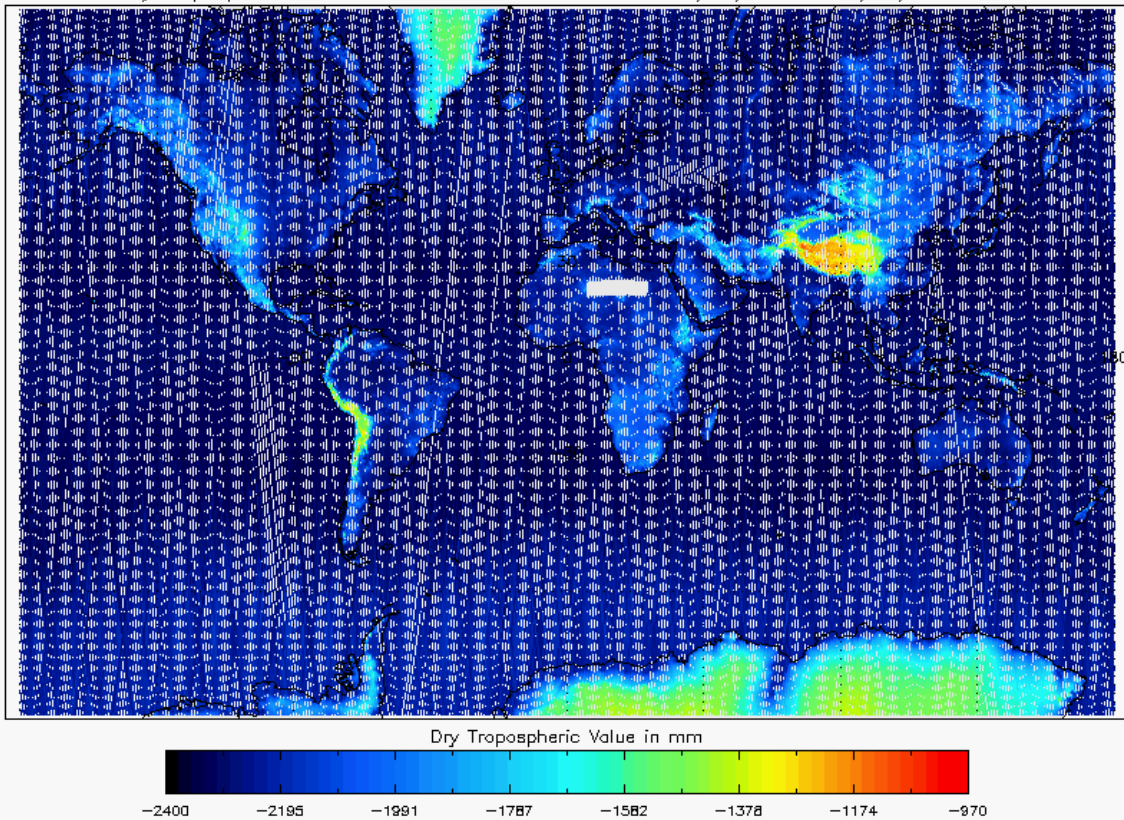
Figure 16 - Global plot of Dry Tropospheric Correction for cycle #99
