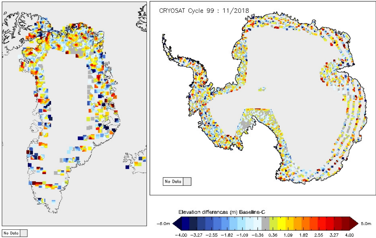
Figure 15 - Greenland and Antarctica maps of SARIn elevation differences for cycle #99
