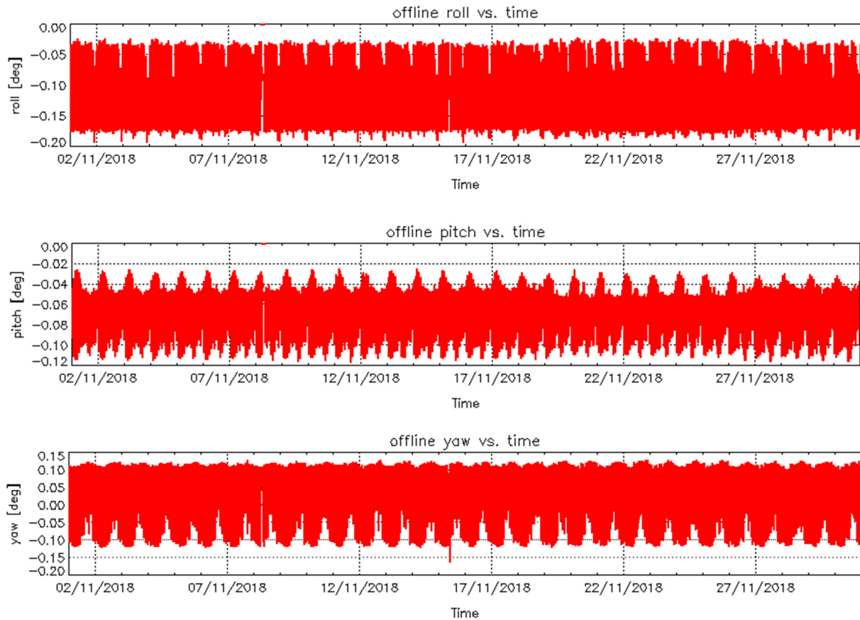
Figure 4 – Roll (top), Pitch (middle) and Yaw (bottom) values for L1B Products during cycle #99.
