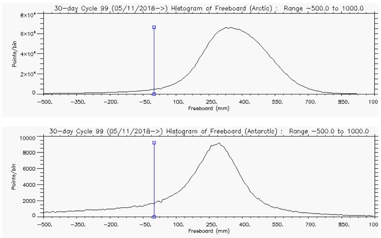
Figure 5 - Histogram of Freeboard for Arctic (above) and Antarctic (below) for cycle #99
