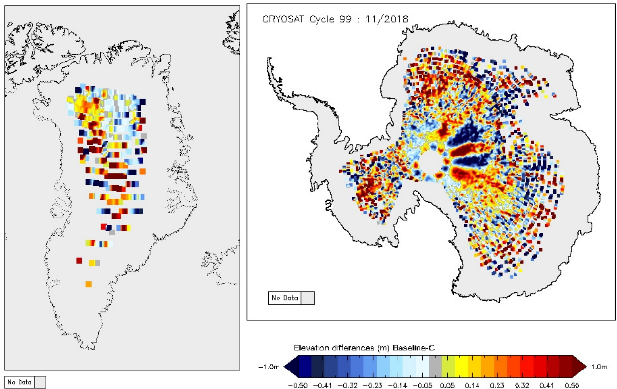
Figure 14 - Greenland and Antarctica maps of LRM elevation differences for cycle #99.
