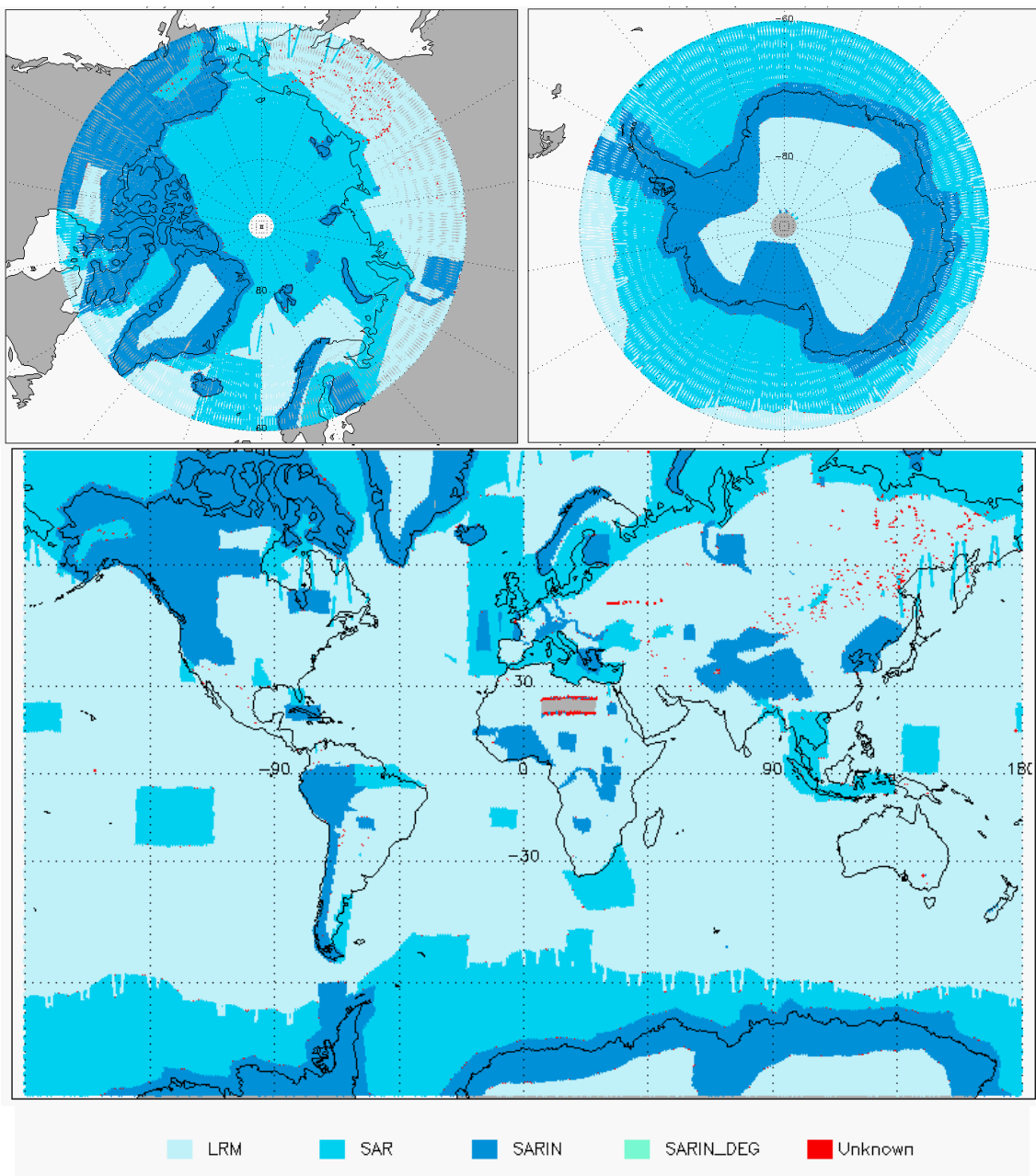
Figure 3 - Global and Polar plots of SIRAL Modes for cycle #99.
