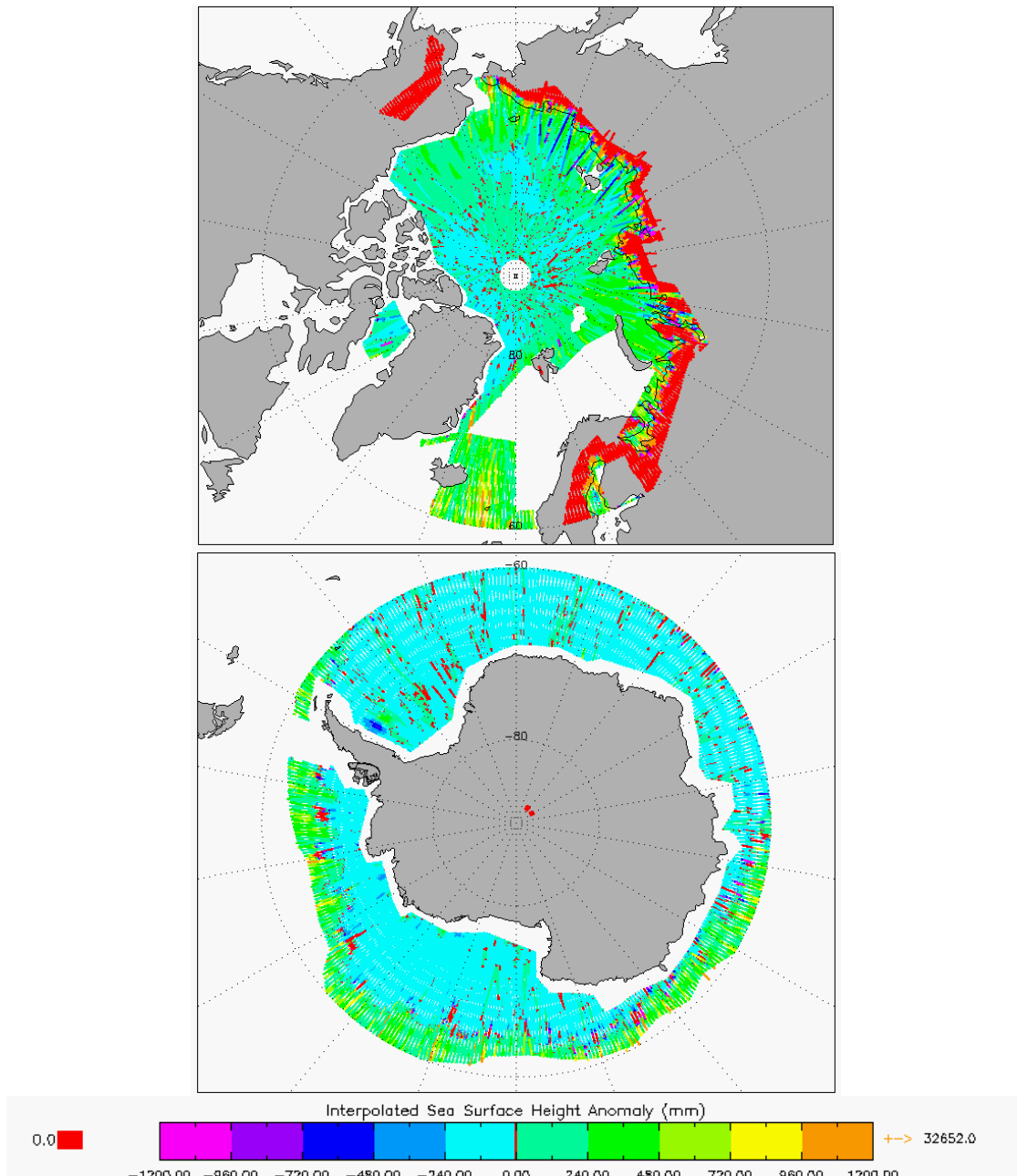
Figure 7 –Polar plots of SSHA for cycle #98.
