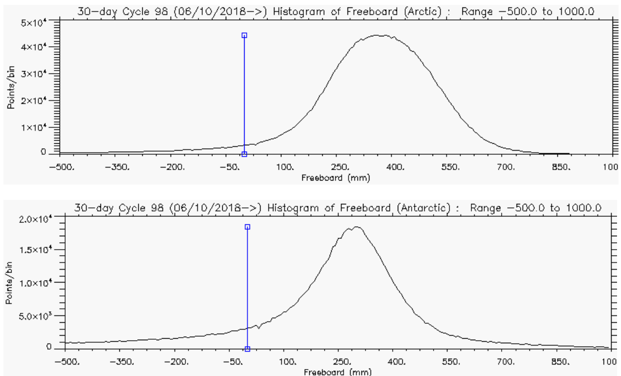
Figure 5 – Histogram of Freeboard for Arctic (above) and Antarctic (below) for cycle #98
