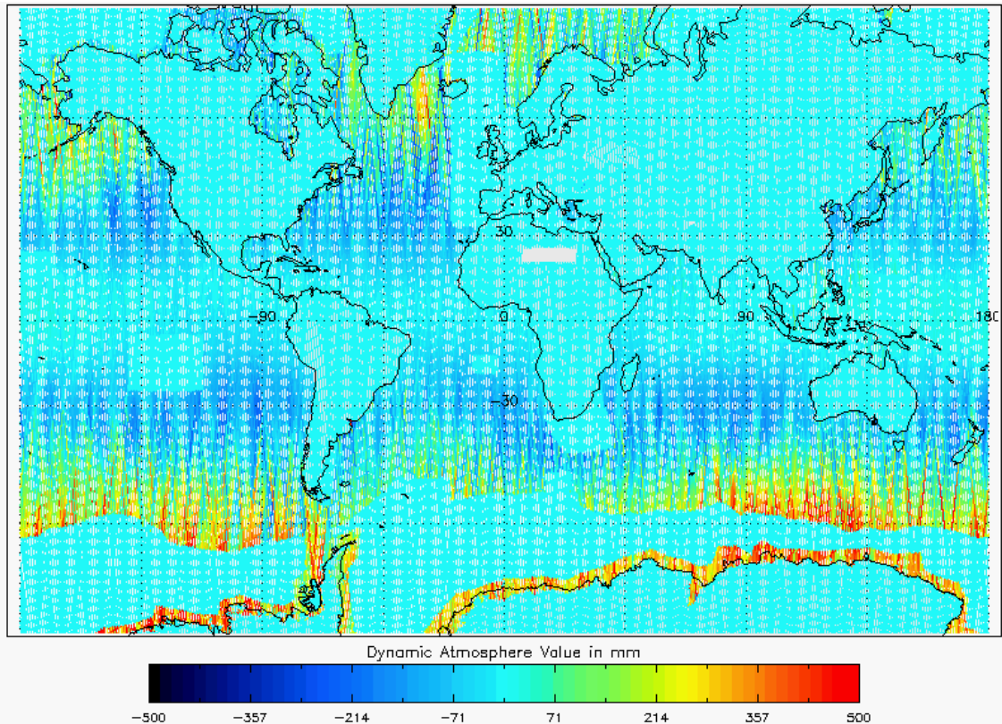
Figure 22 - Global plot of Dynamic Atmospheric Correction for cycle #98
