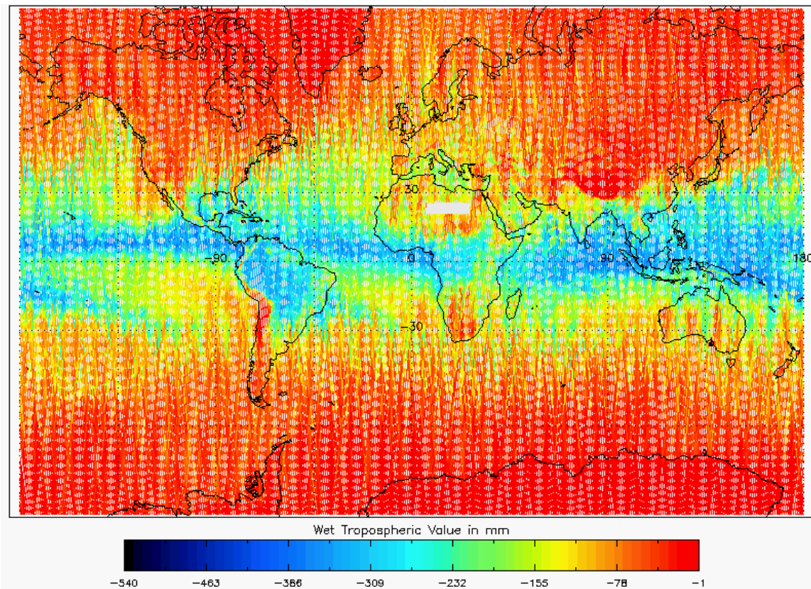
Figure 18 - Global plot of Wet Tropospheric Correction for cycle #98
