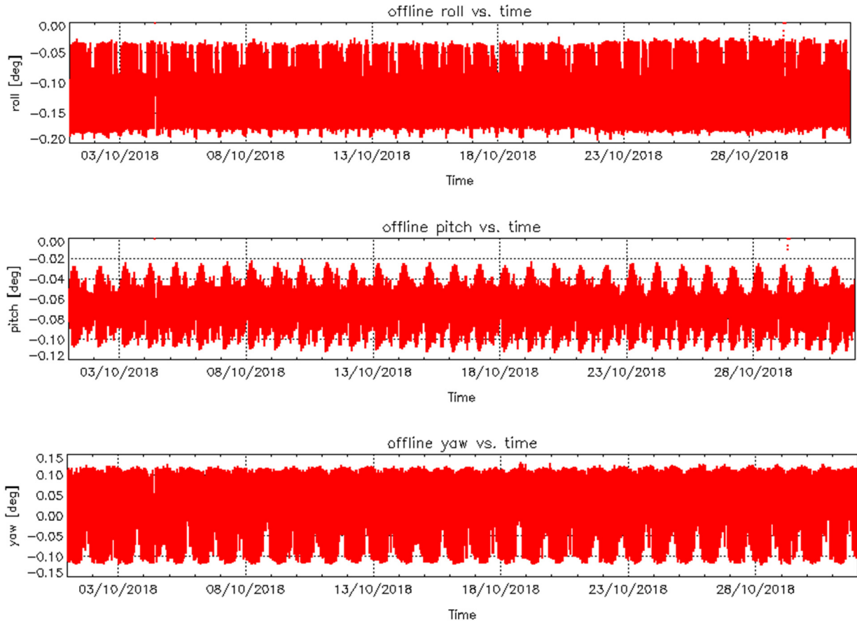
Figure 4 – Roll (top), Pitch (middle) and Yaw (bottom) values for L1B Products during cycle #98.
