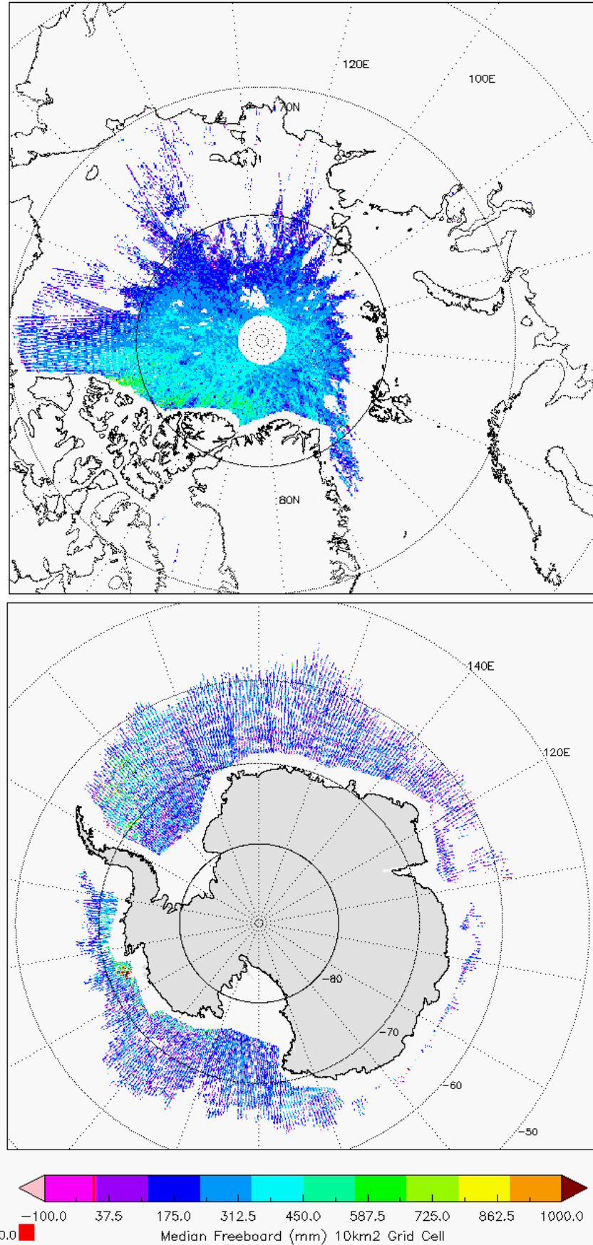
Figure 6 - Polar plots of 10km Gridded Freeboard values from L2 SAR products in cycle #98.
