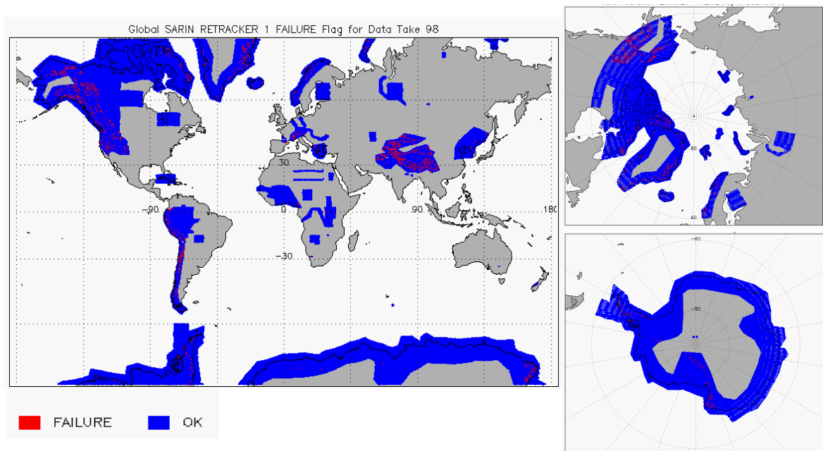
Figure 11 – Global plots showing Retracker Failure Flags for SARIn mode for cycle #98
