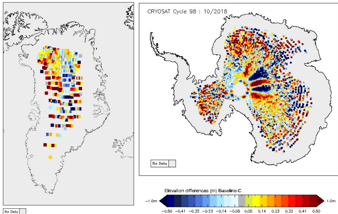
Figure 14 - Greenland and Antarctica maps of LRM elevation differences for cycle #98.
