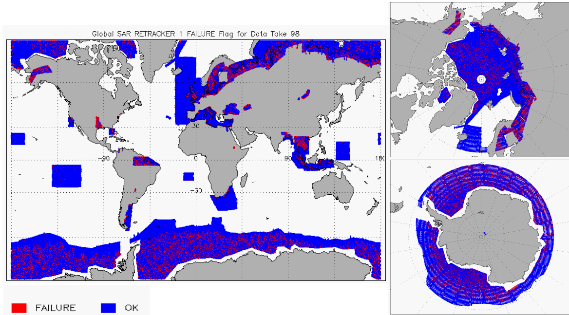
Figure 10 – Global plots showing Retracker Failure Flags for SAR mode for cycle #98
