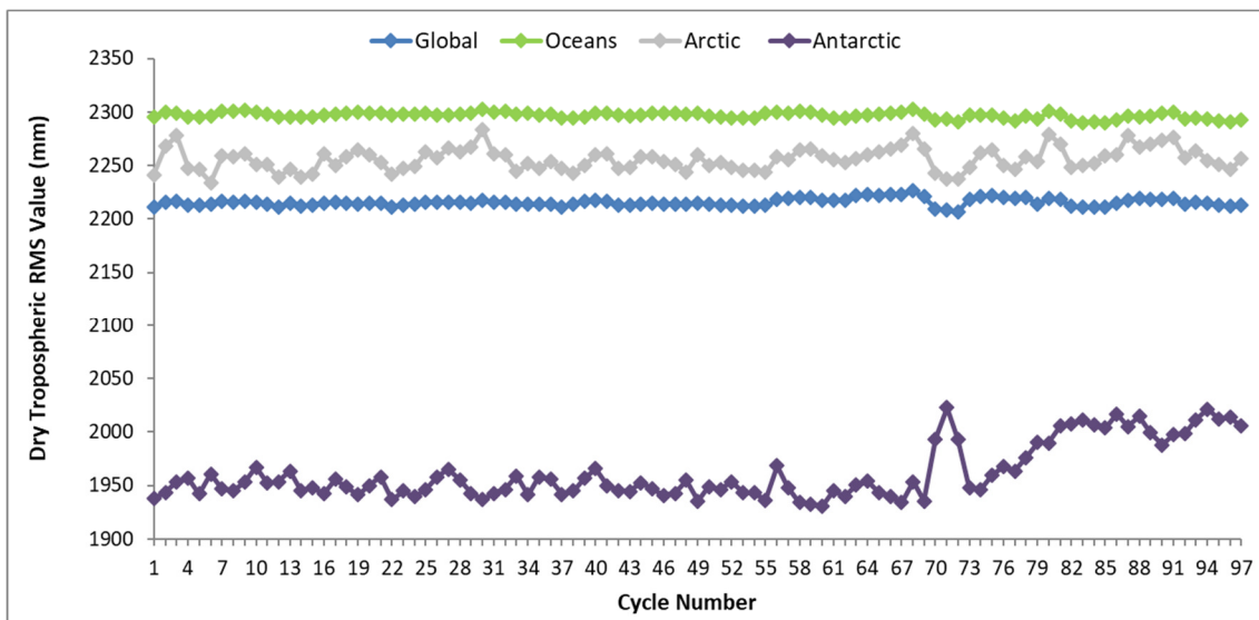
Figure 10 - Dry Tropospheric Correction RMS value trend from beginning of mission
