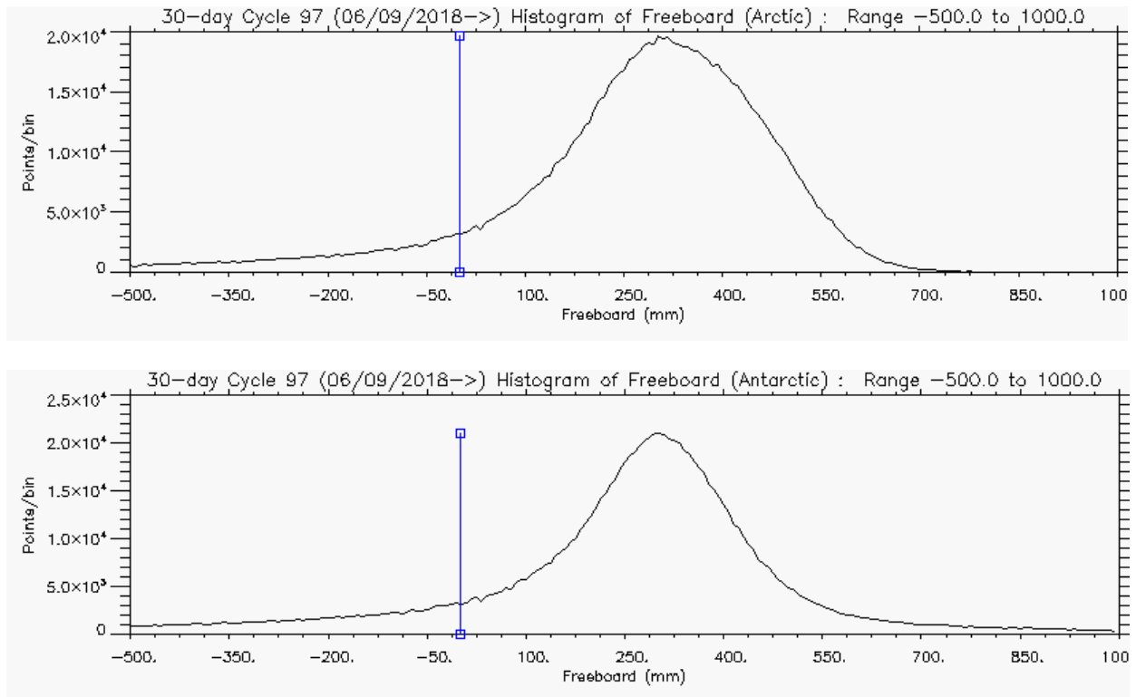
Figure 5 – Histogram of Freeboard for Arctic (above) and Antarctic (below) for cycle #97
