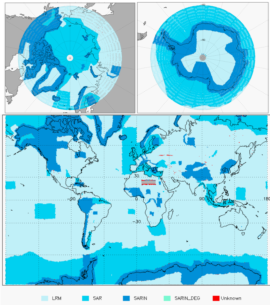
Figure 3 - Global and Polar plots of SIRAL Modes for cycle #97.
