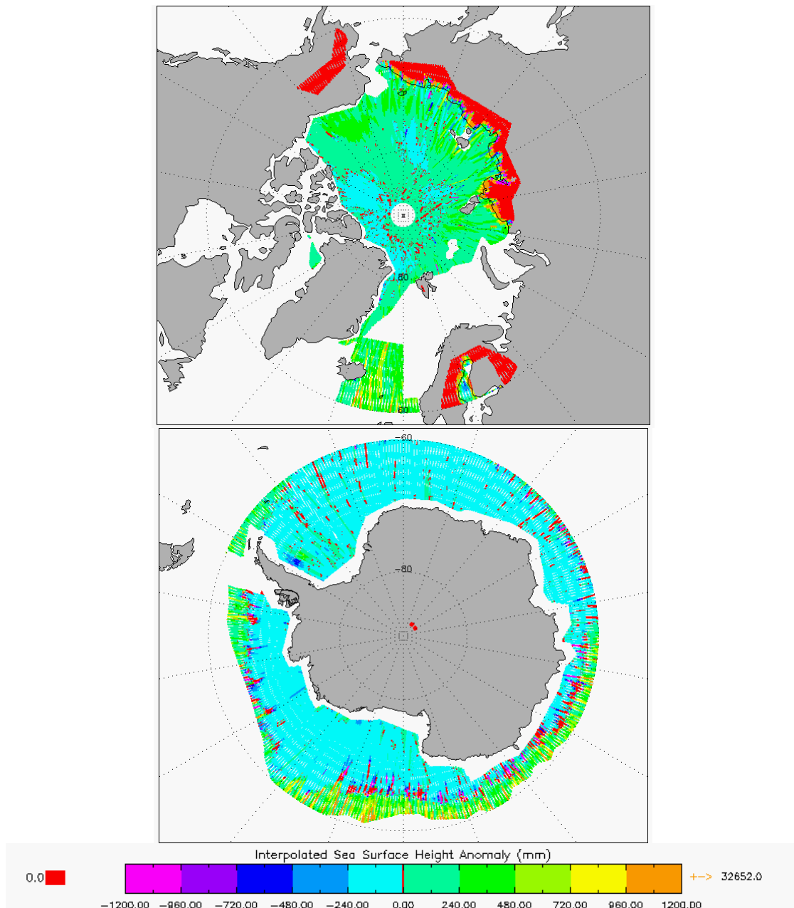
Figure 7 –Polar plots of SSHA for cycle #97.
