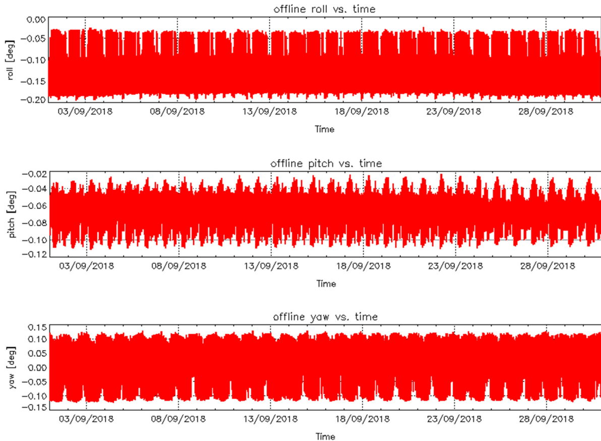
Figure 4 – Roll (top), Pitch (middle) and Yaw (bottom) values for L1B Products during cycle #97.
