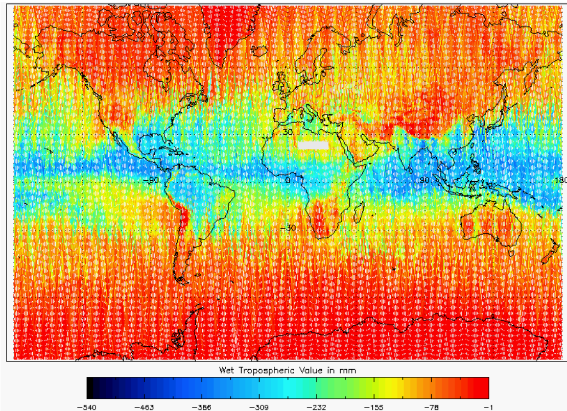
Figure 118 - Global plot of Wet Tropospheric Correction for cycle #97
