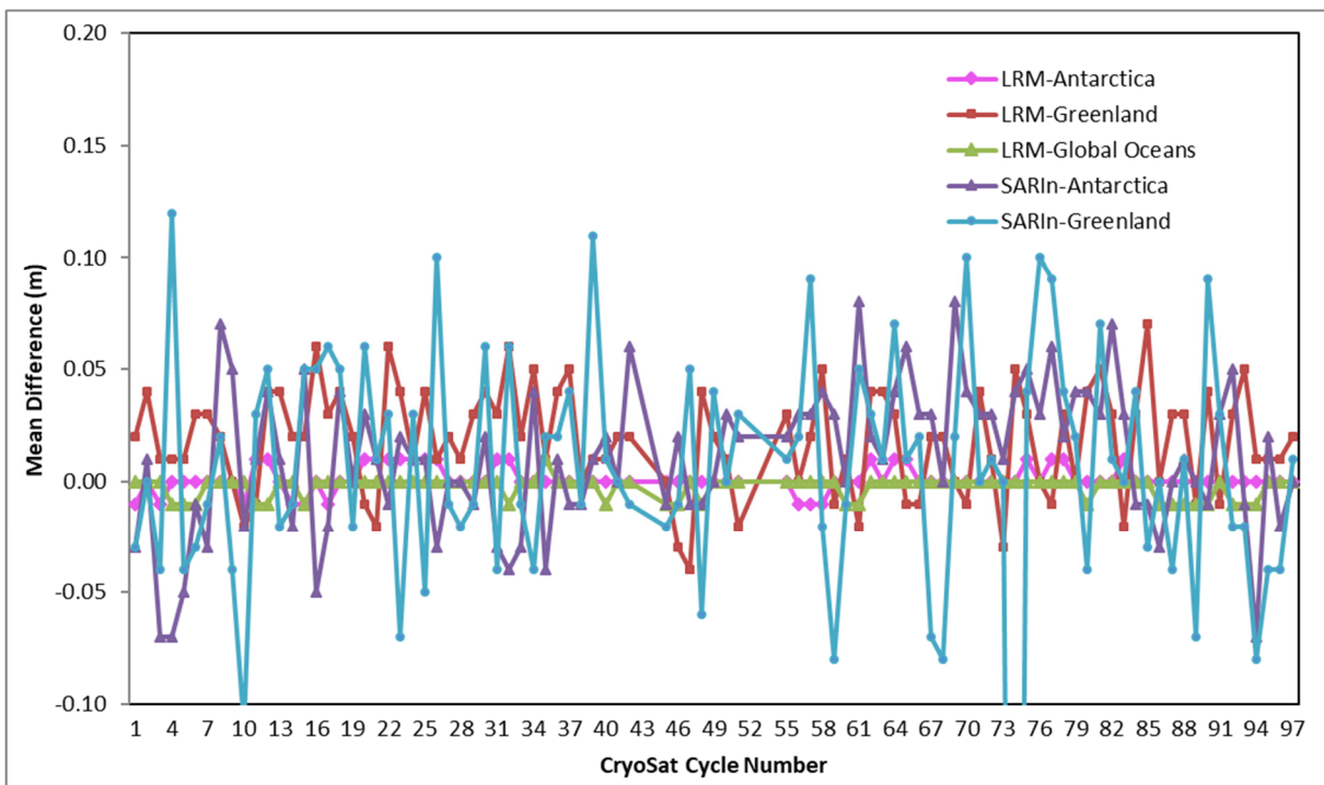
Figure 63 - Time series for Mean Difference in elevation at crossovers from beginning of the mission
