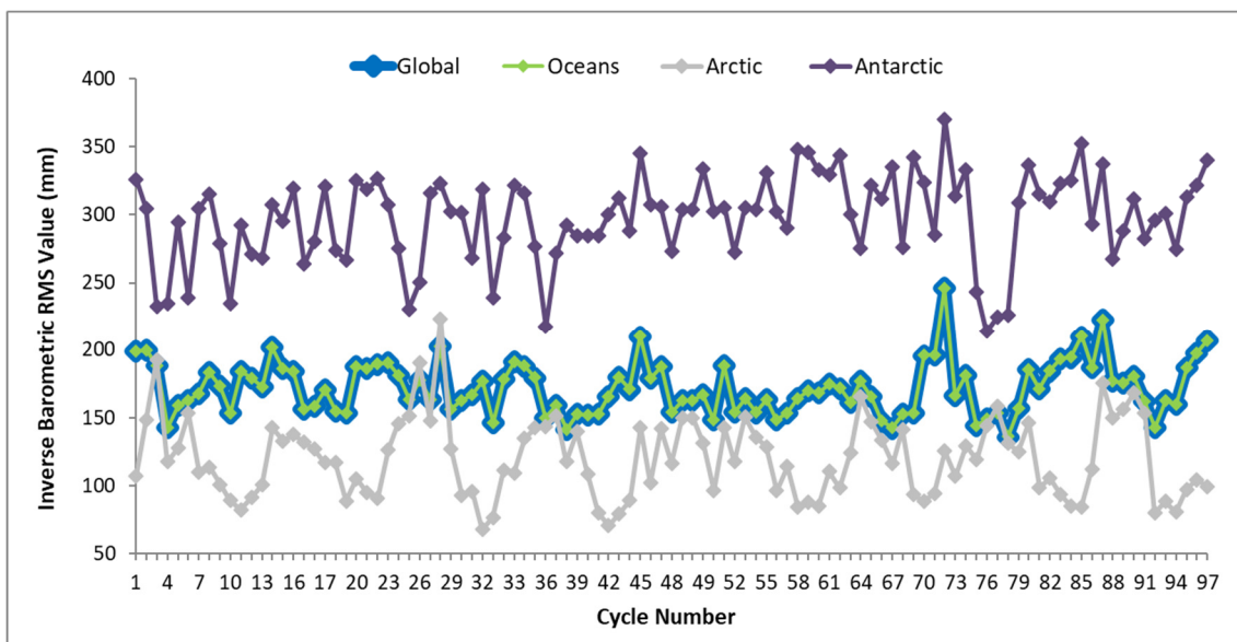
Figure 131 – Inverse Barometric Correction RMS value trend from beginning of mission
