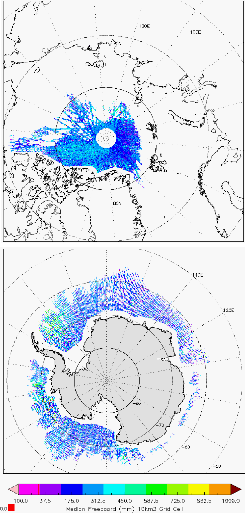
Figure 6 - Polar plots of 10km Gridded Freeboard values from L2 SAR products in cycle #97.
