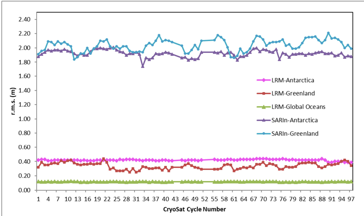
Figure 52 - Time series for crossover elevation r.m.s values from beginning of the mission
