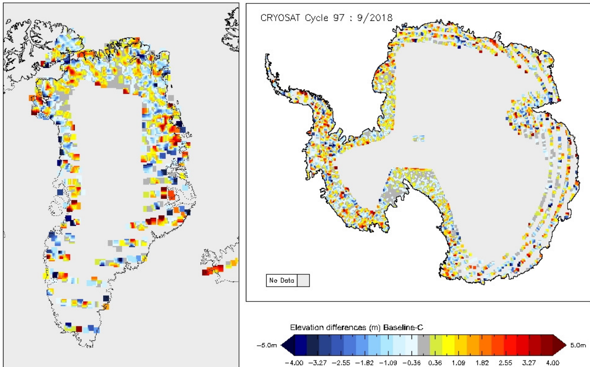
Figure 85 - Greenland and Antarctica maps of SARIn elevation differences for cycle #97
