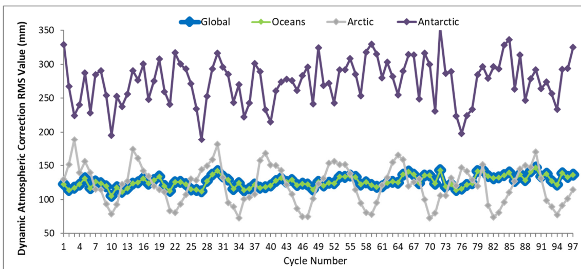
Figure 153 – Dynamic Atmospheric Correction RMS value trend from beginning of mission
