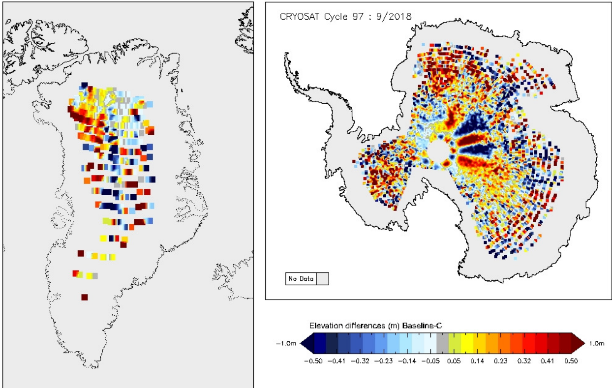
Figure 74 - Greenland and Antarctica maps of LRM elevation differences for cycle #97.
