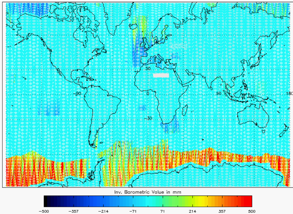
Figure 120 - Global plot of Inverse Barometric Correction for cycle #97
