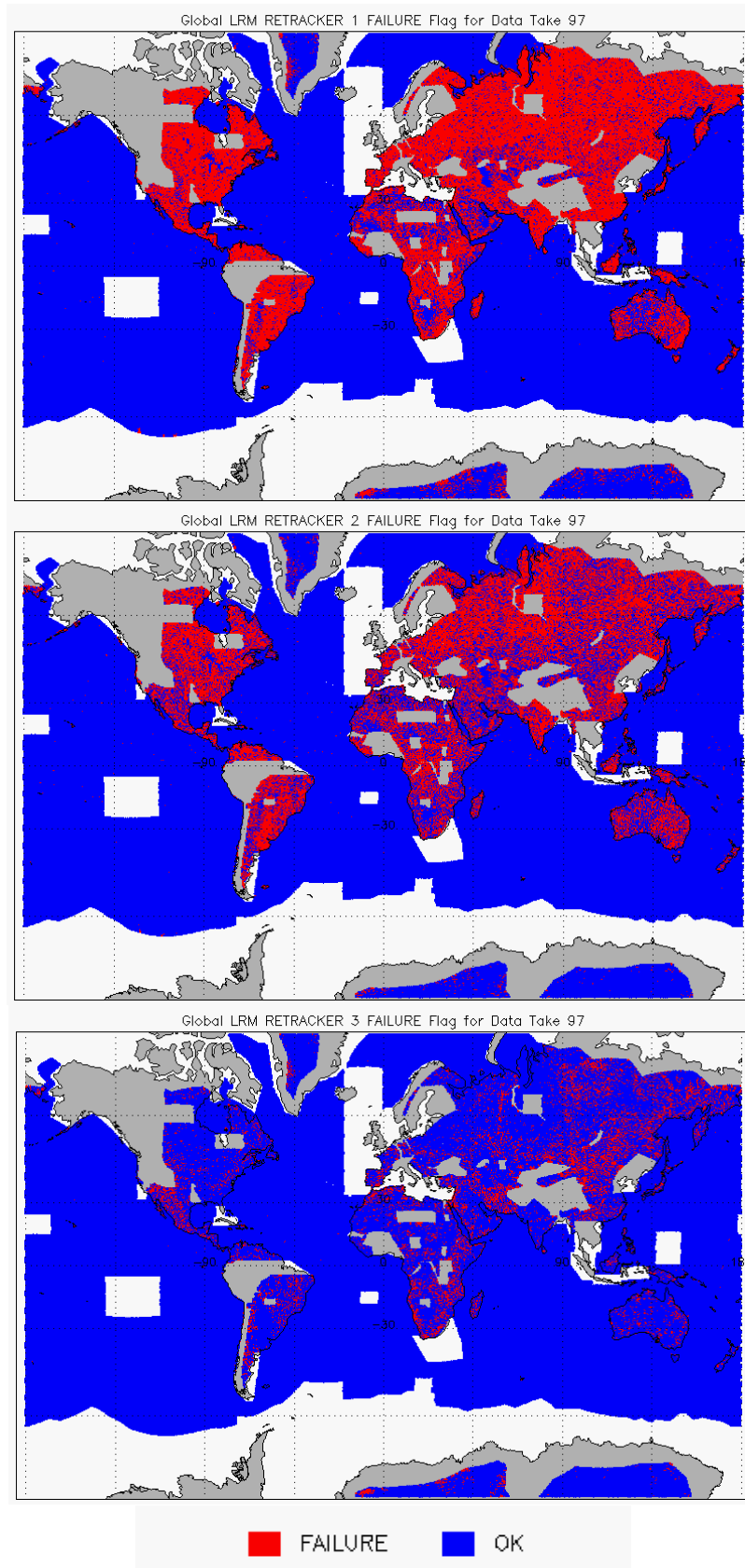
Figure 9 – Global plots showing Retracker Failure Flags for LRM mode for cycle #97:
