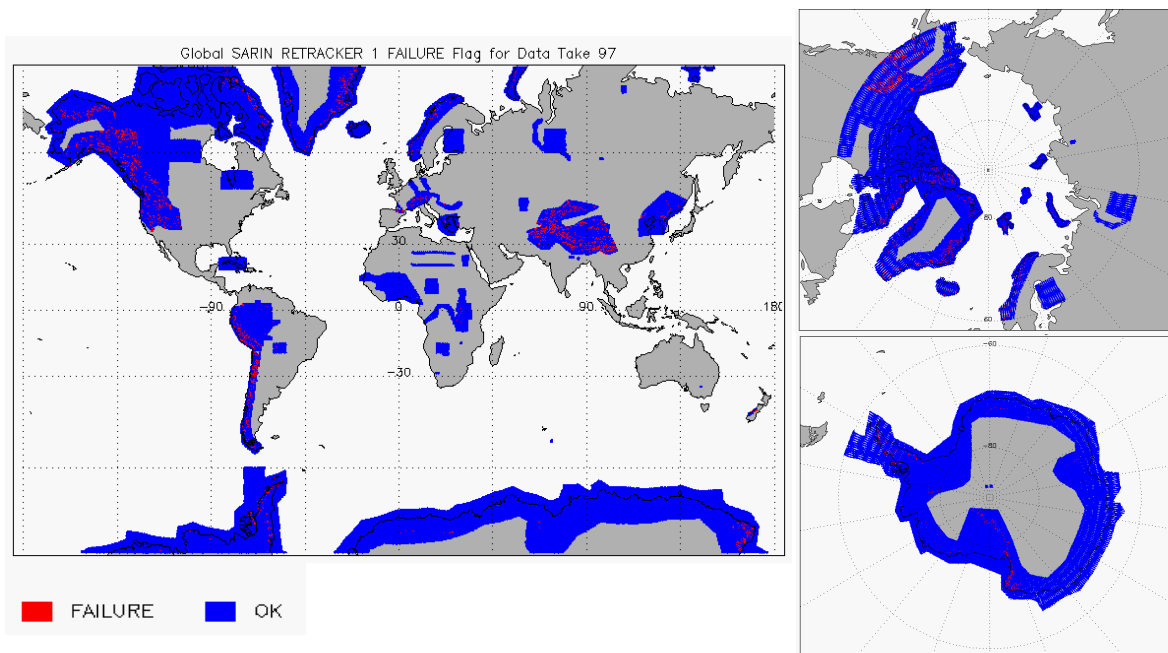
Figure 11 – Global plots showing Retracker Failure Flags for SARIn mode for cycle #97
