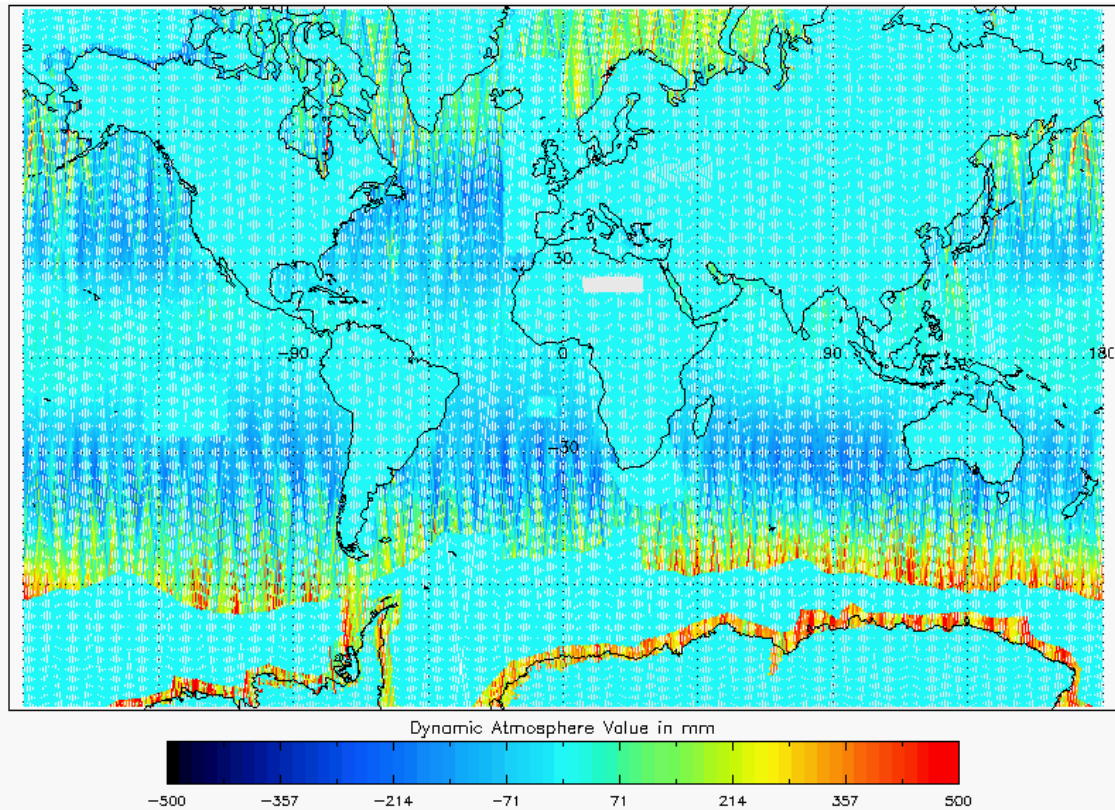
Figure 142 - Global plot of Dynamic Atmospheric Correction for cycle #97
