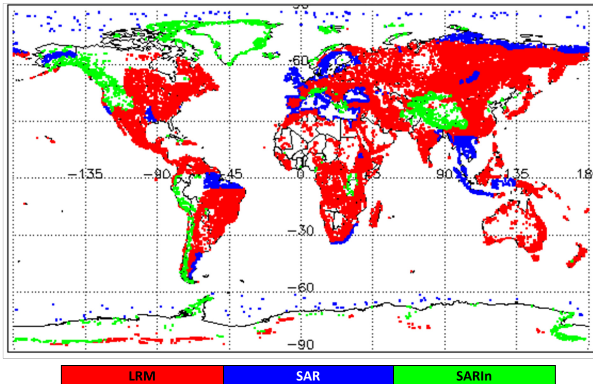
Figure 1 - Global plot showing areas of loss of track in all SIRAL modes L0 data during September 2018.
