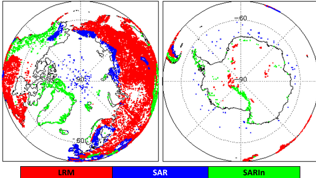
Figure 2 - Polar plots showing areas of loss of track in all SIRAL modes L0 data during September 2018.
