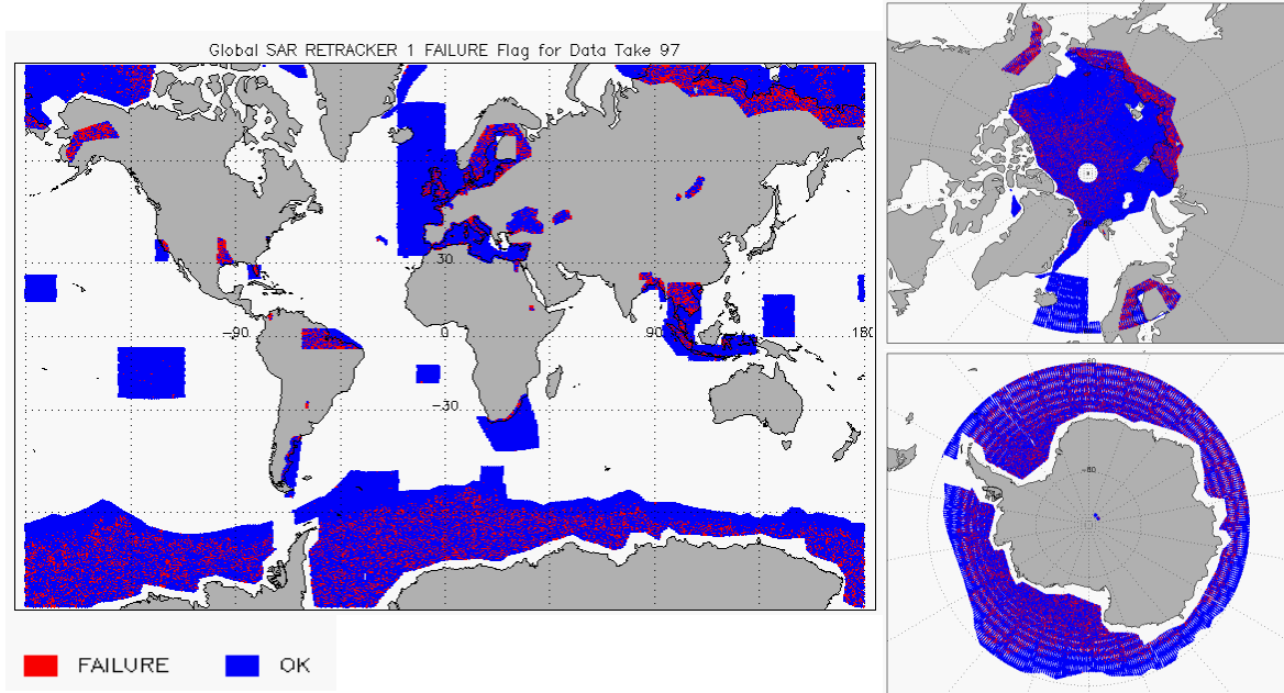
Figure 10 – Global plots showing Retracker Failure Flags for SAR mode for cycle #97
