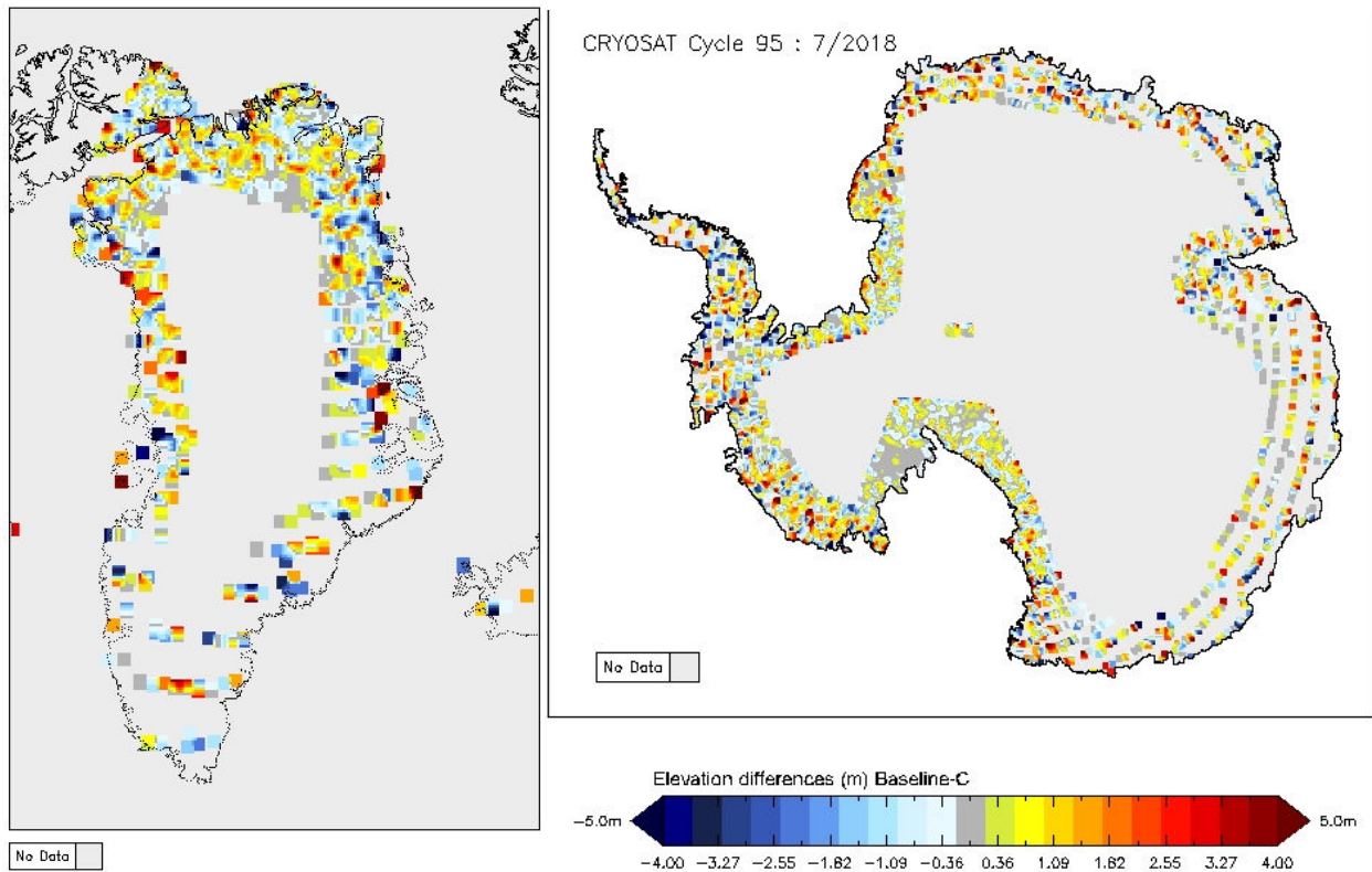
Figure 15 - Greenland and Antarctica maps of SARIn elevation differences for cycle #95
