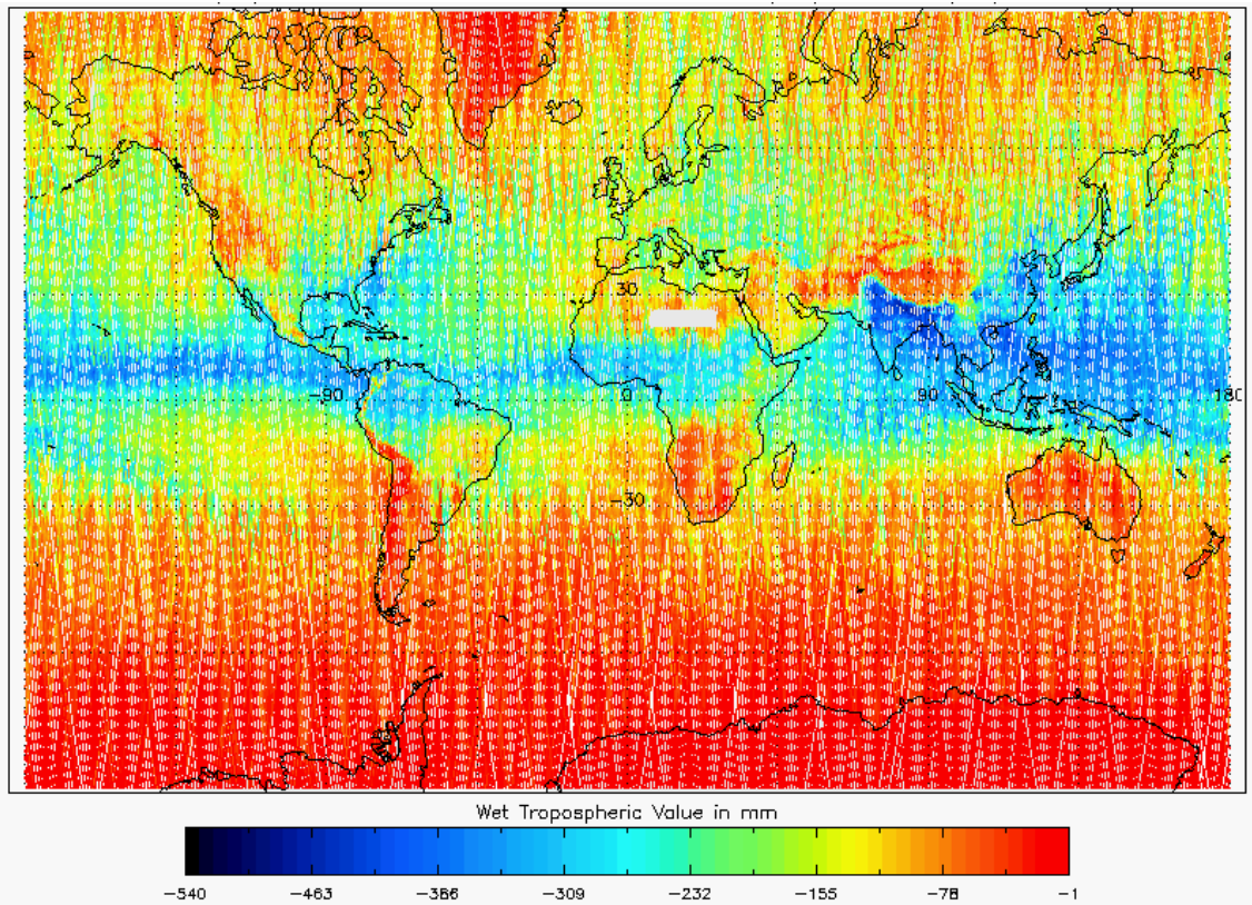
Figure 18 - Global plot of Wet Tropospheric Correction for cycle #95
