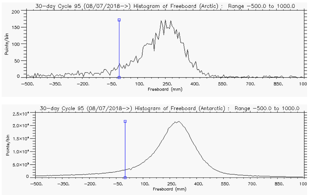
Figure 5 – Histogram of Freeboard for Arctic (above) and Antarctic (below) for cycle #95
