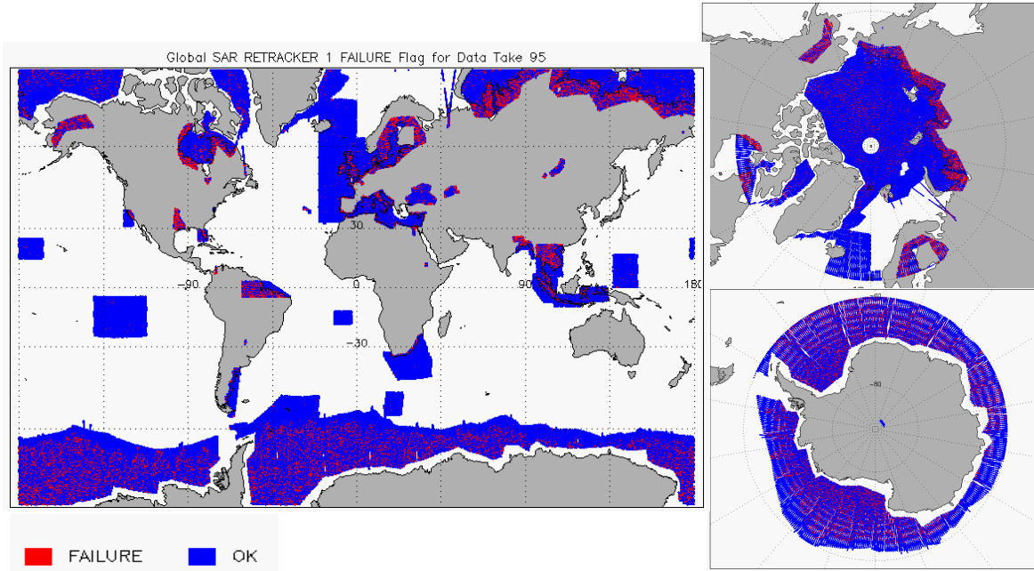
Figure 10 – Global plots showing Retracker Failure Flags for SAR mode for cycle #95
