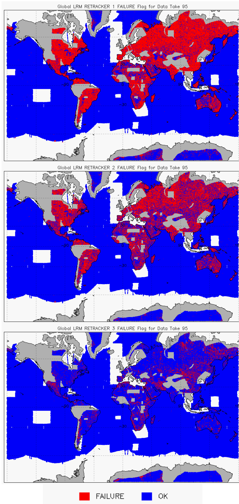
Figure 9 – Global plots showing Retracker Failure Flags for LRM mode for cycle #95:
