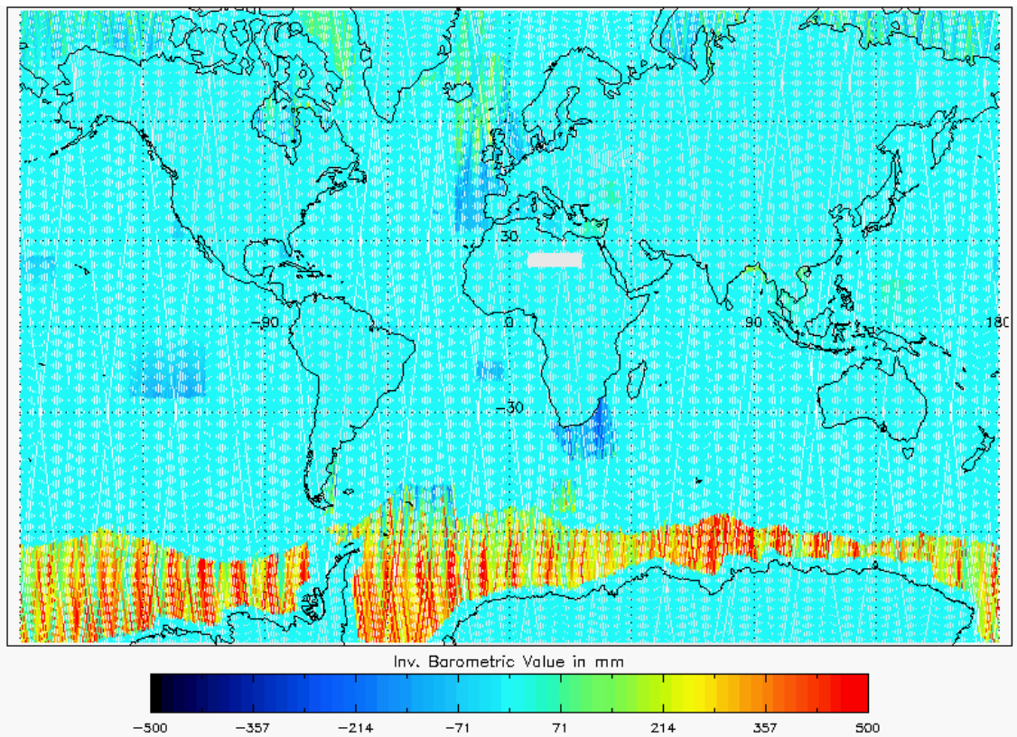
Figure 20 - Global plot of Inverse Barometric Correction for cycle #95
