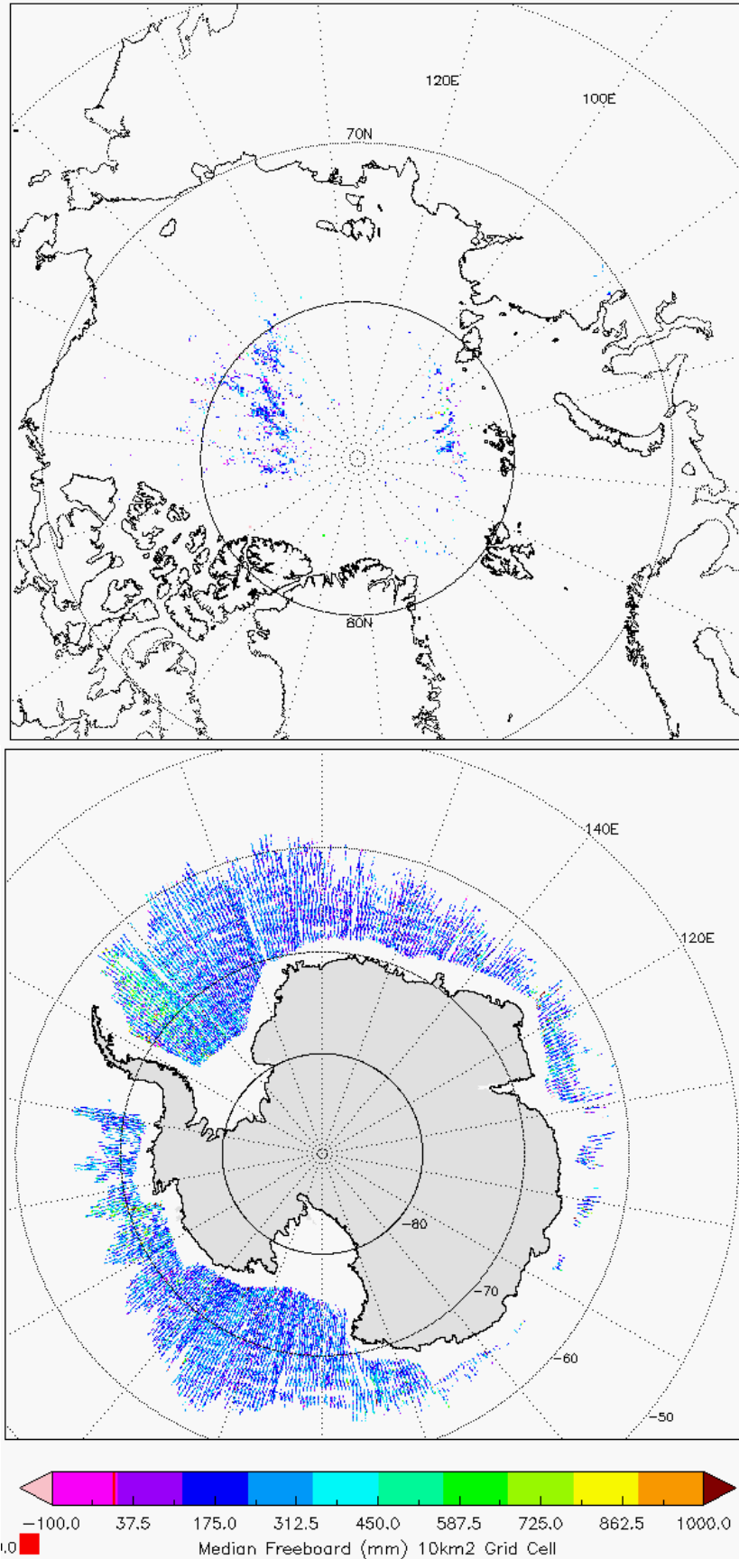
Figure 6 - Polar plots of 10km Gridded Freeboard values from L2 SAR products in cycle #95.
