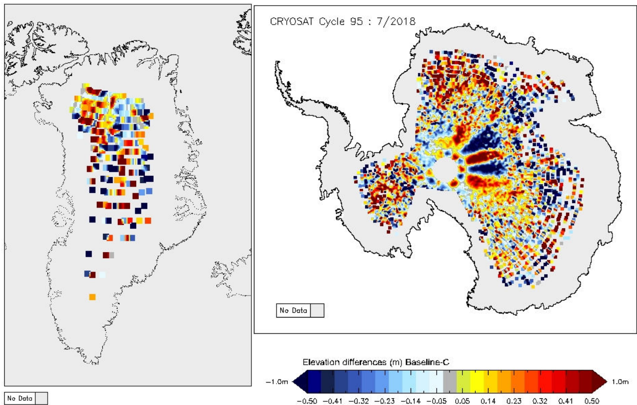
Figure 14 - Greenland and Antarctica maps of LRM elevation differences for cycle #95.
