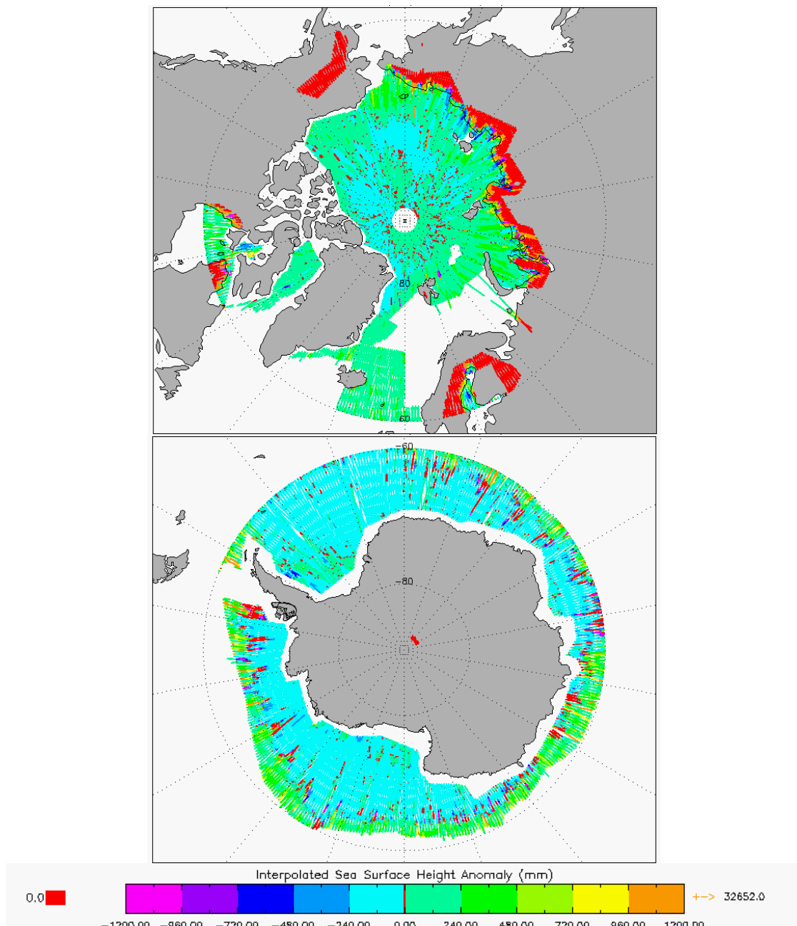
Figure 7 –Polar plots of SSHA for cycle #95.
