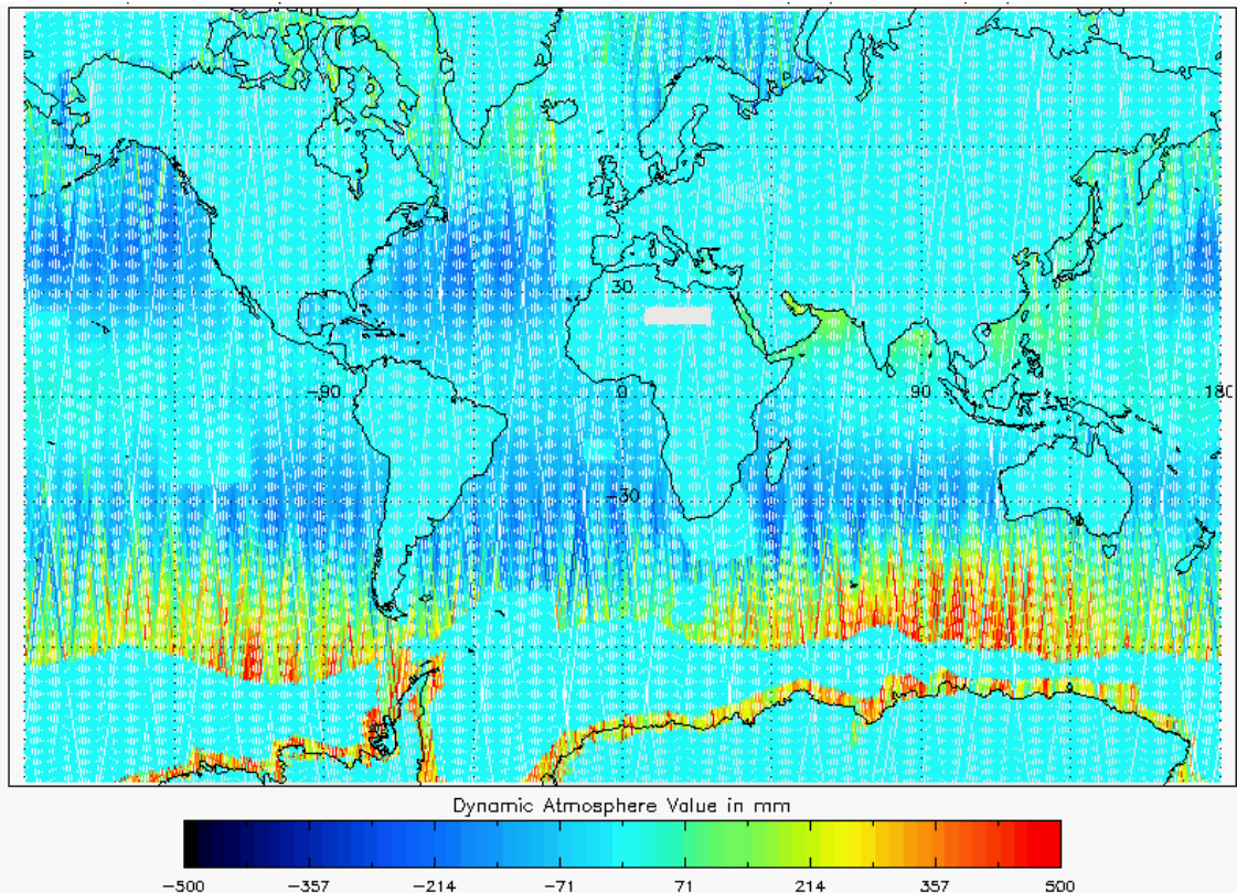
Figure 22 - Global plot of Dynamic Atmospheric Correction for cycle #95
