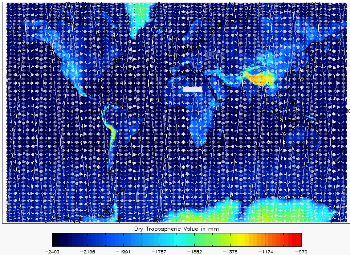
Figure 16 - Global plot of Dry Tropospheric Correction for cycle #95
