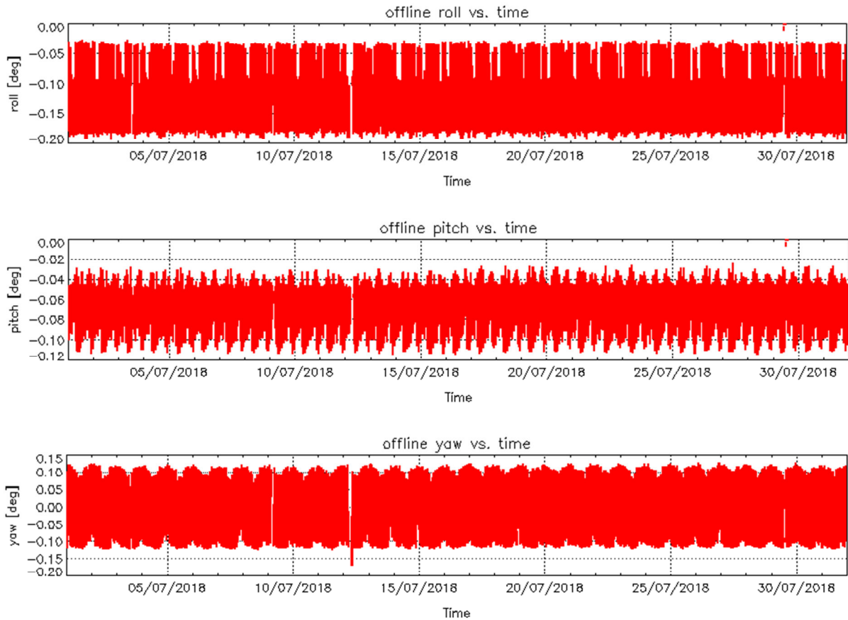
Figure 4 – Roll (top), Pitch (middle) and Yaw (bottom) values for L1B Products during cycle #95.
