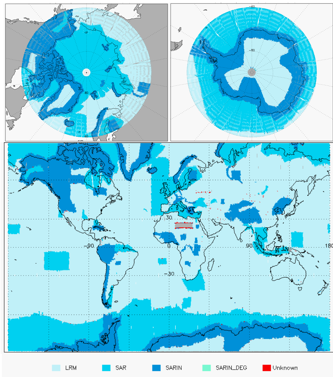
Figure 3 - Global and Polar plots of SIRAL Modes for cycle #95.
