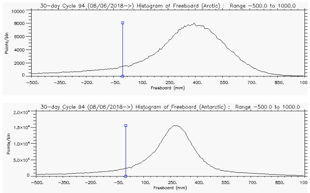
Figure 5 – Histogram of Freeboard for Arctic (above) and Antarctic (below) for cycle #94
