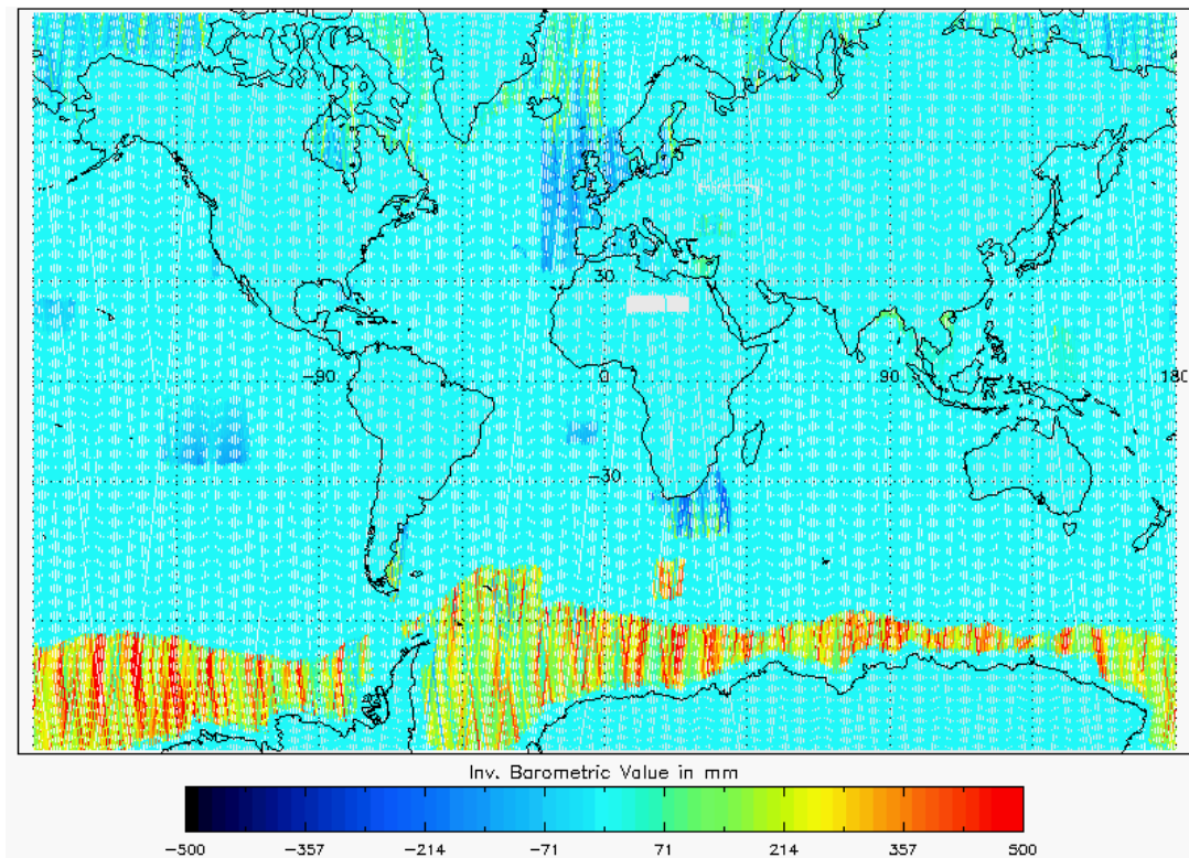
Figure 20 - Global plot of Inverse Barometric Correction for cycle #94
