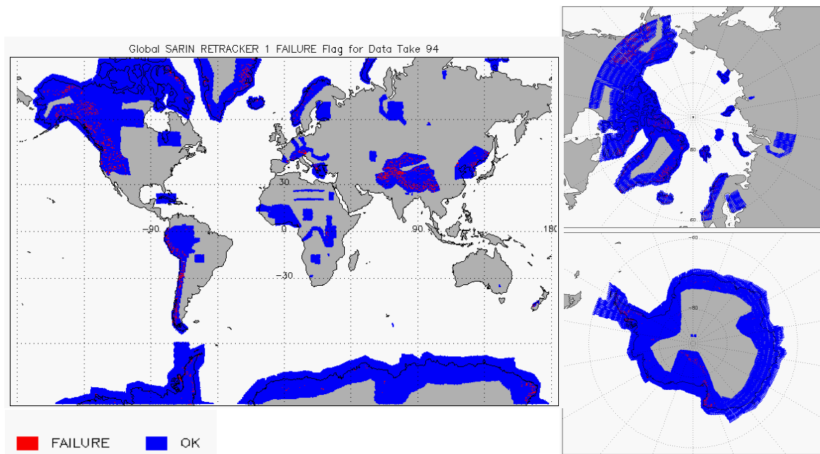
Figure 11 – Global plots showing Retracker Failure Flags for SARIn mode for cycle #94
