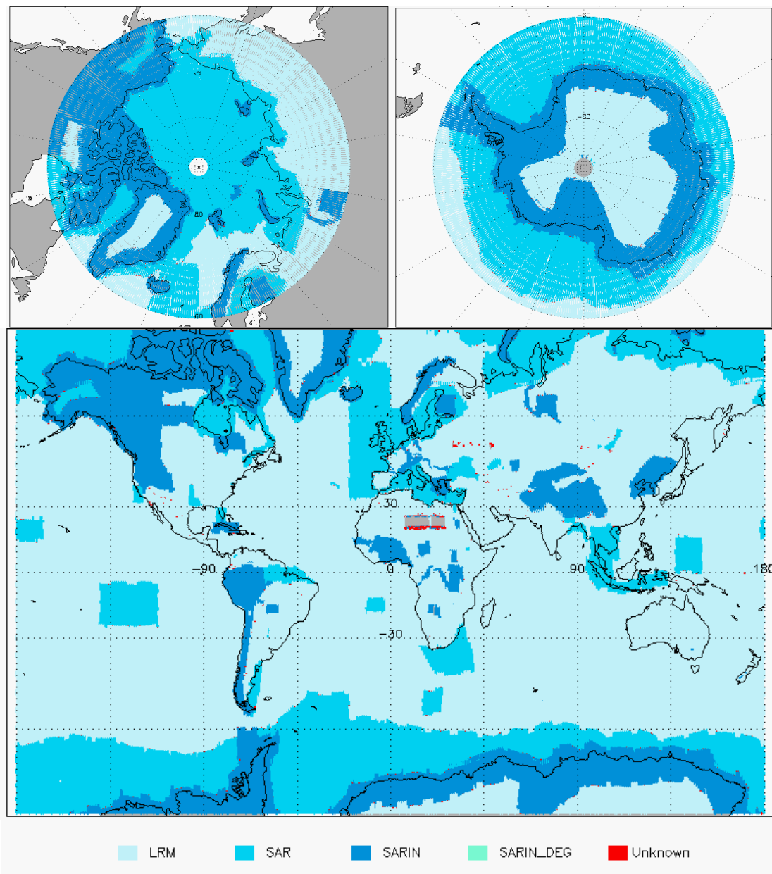
Figure 3 - Global and Polar plots of SIRAL Modes for cycle #94.
