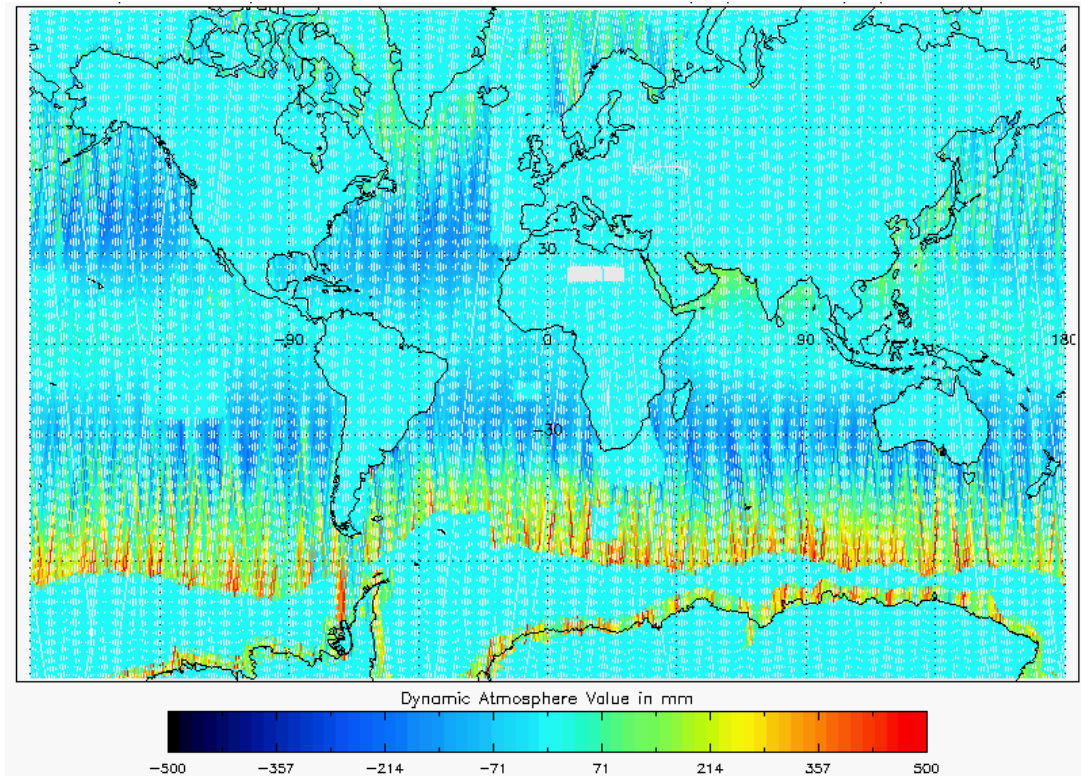
Figure 22 - Global plot of Dynamic Atmospheric Correction for cycle #94
