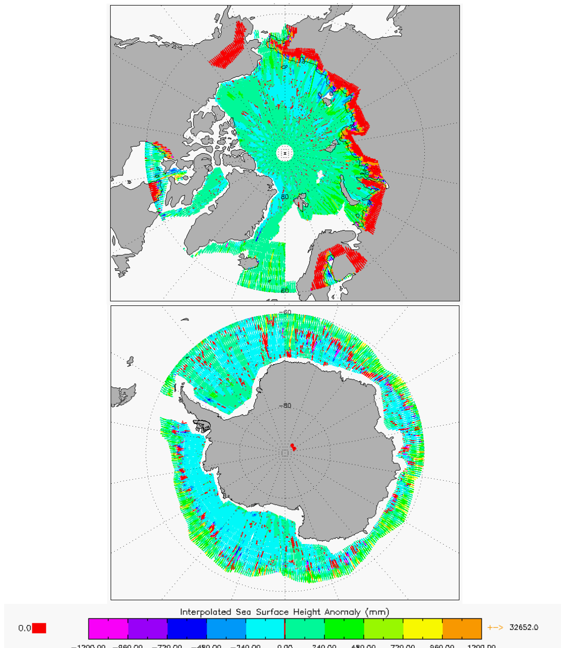
Figure 7 –Polar plots of SSHA for cycle #94.
