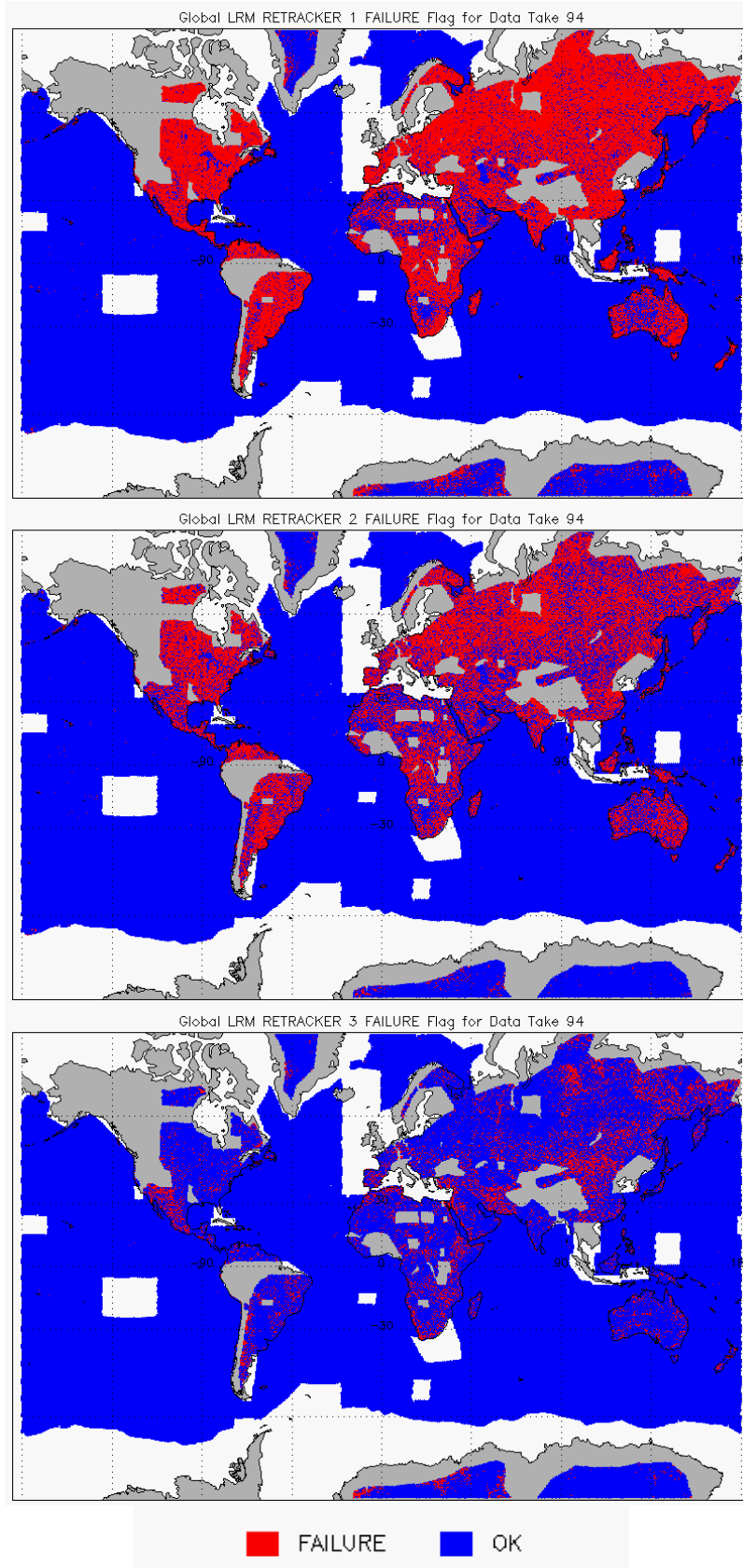
Figure 9 – Global plots showing Retracker Failure Flags for LRM mode for cycle #94: LRM CFI (top), LRM LIRT (middle), LRM OCOG (bottom)
