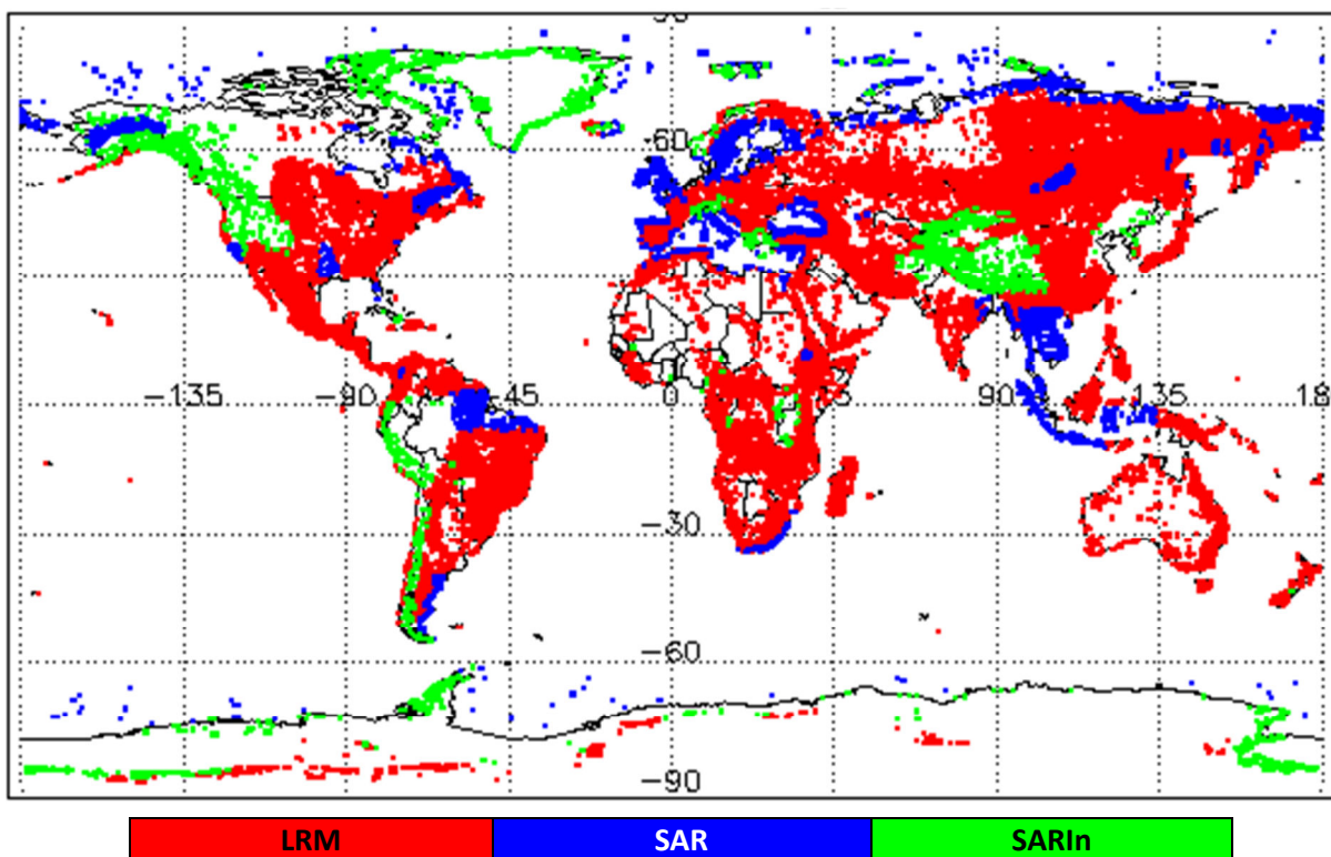
Figure 1 - Global plot showing areas of loss of track in all SIRAL modes L0 data during June 2018.
