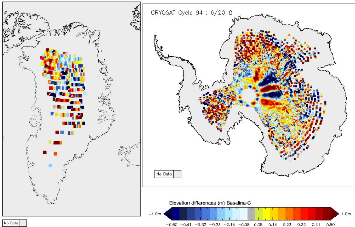
Figure 14 - Greenland and Antarctica maps of LRM elevation differences for cycle #94.
