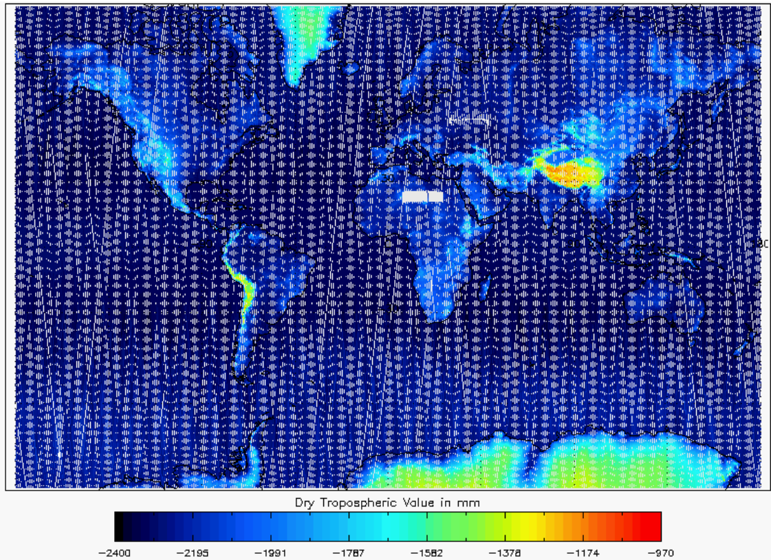
Figure 16 - Global plot of Dry Tropospheric Correction for cycle #94
