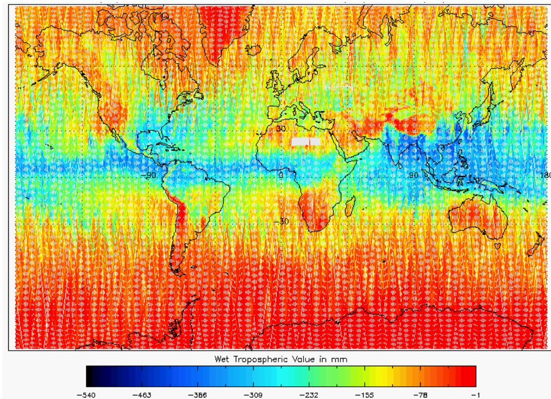
Figure 18 - Global plot of Wet Tropospheric Correction for cycle #94
