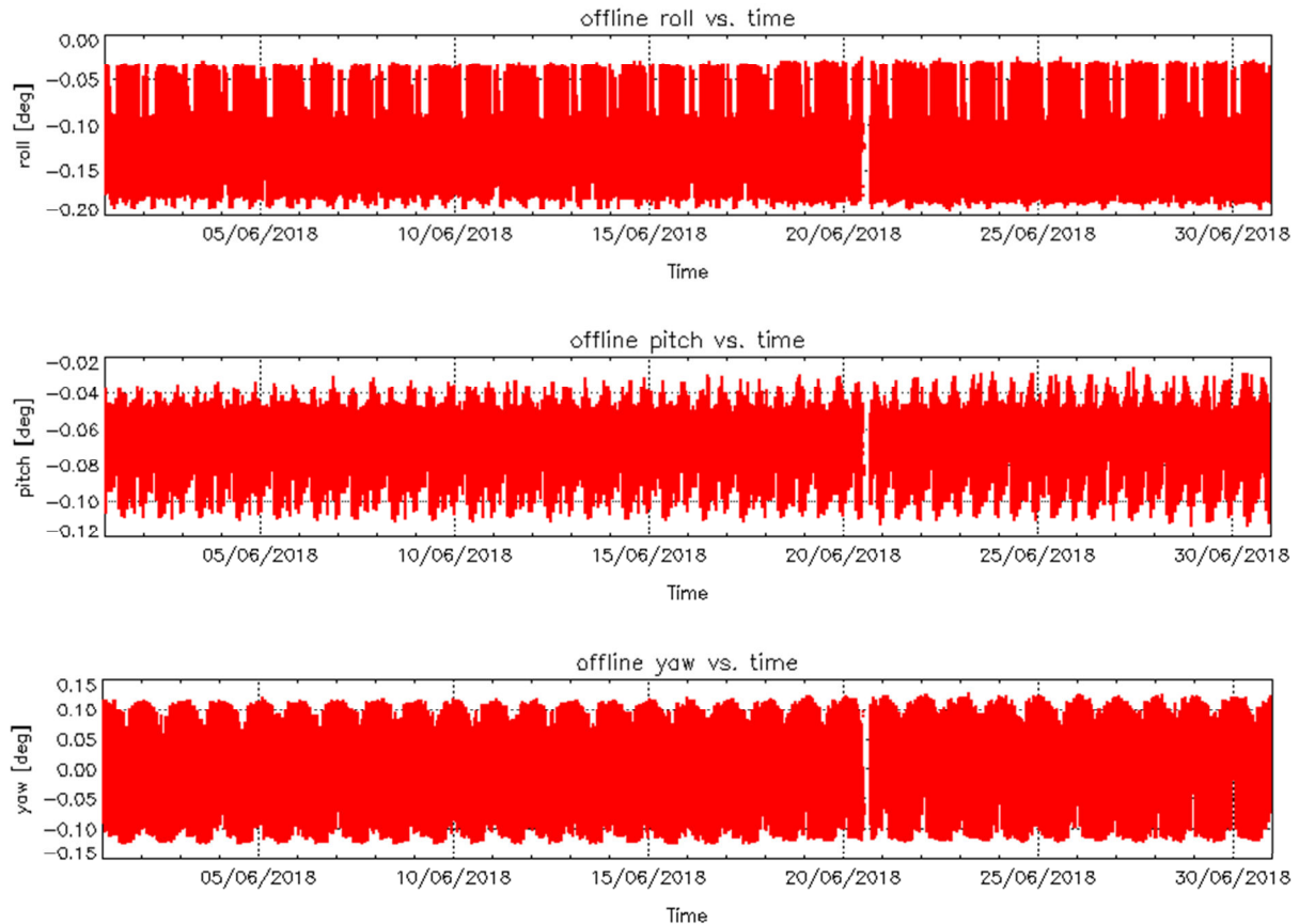
Figure 4 – Roll (top), Pitch (middle) and Yaw (bottom) values for L1B Products during cycle #94.
