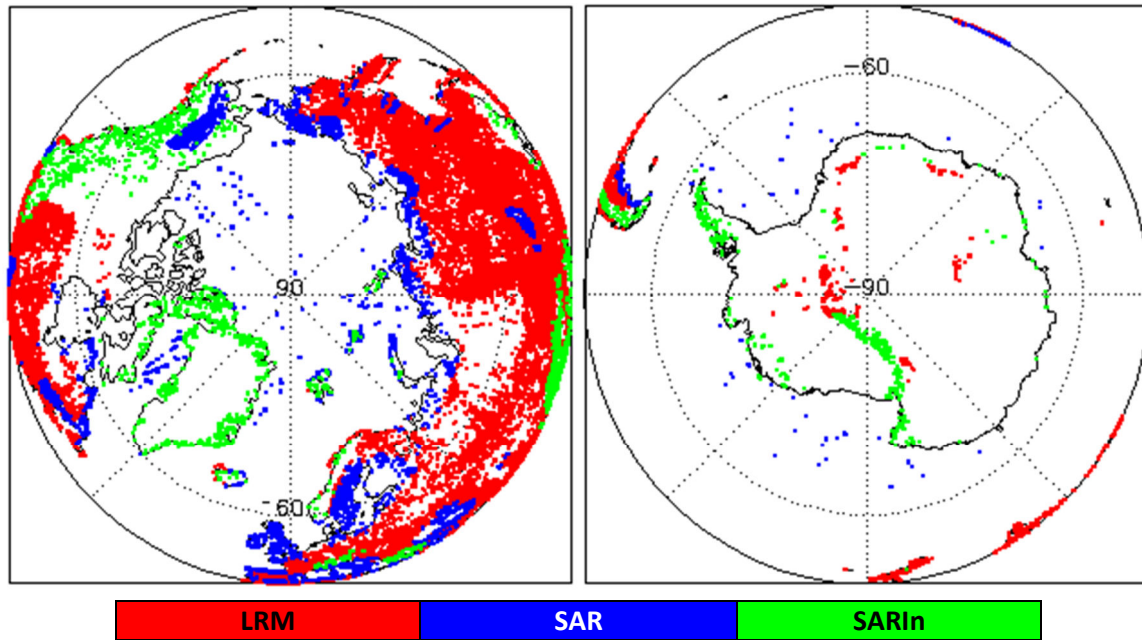
Figure 2 - Polar plots showing areas of loss of track in all SIRAL modes L0 data during June 2018.
