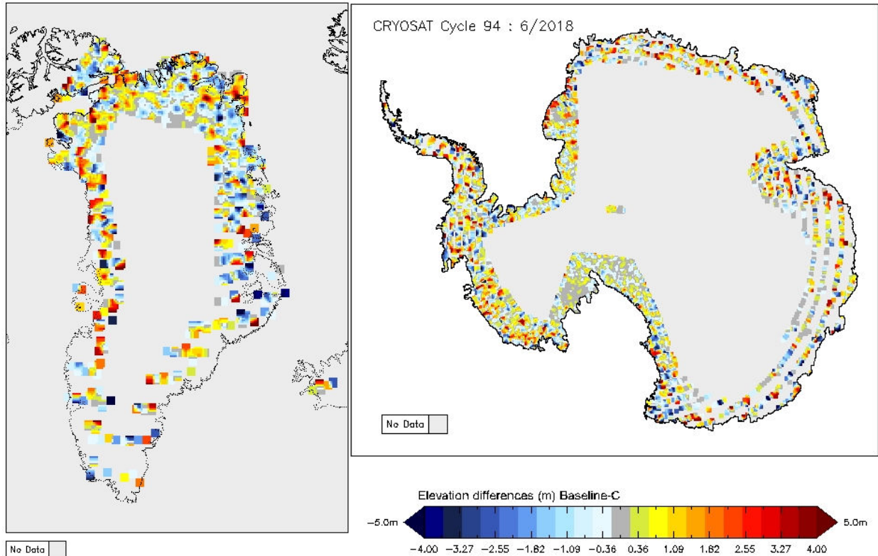
Figure 15 - Greenland and Antarctica maps of SARIn elevation differences for cycle #94
