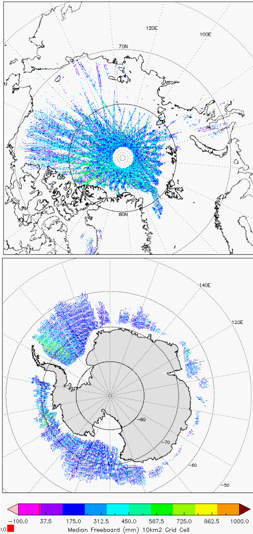
Figure 6 - Polar plots of 10km Gridded Freeboard values from L2 SAR products in cycle #94.
