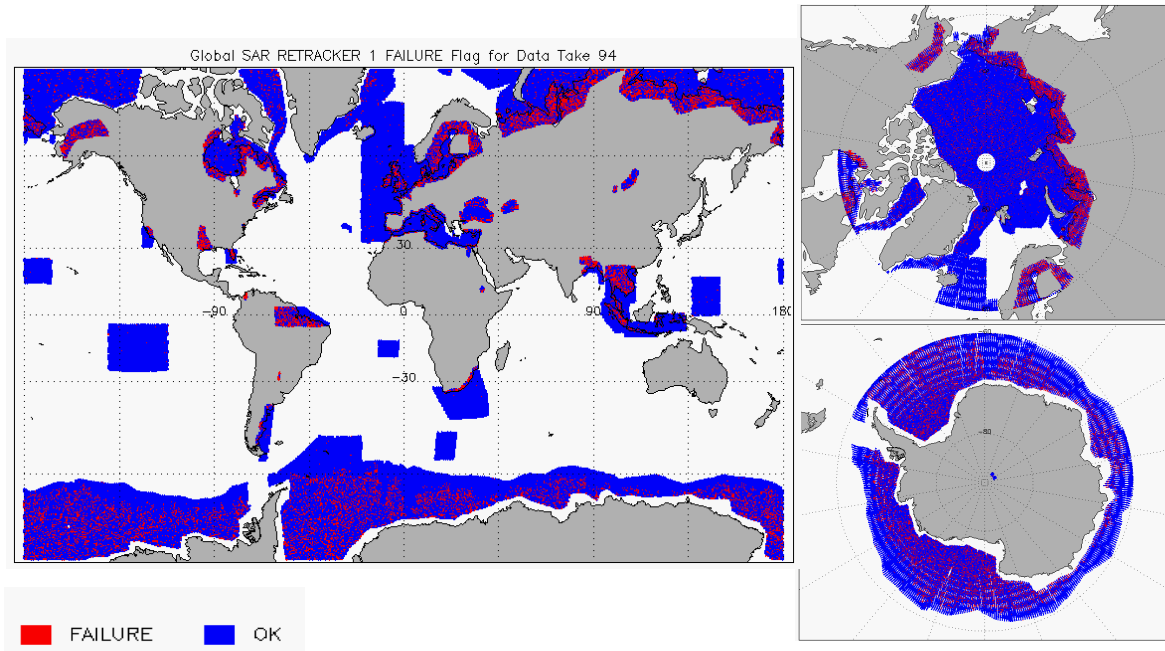
Figure 10 – Global plots showing Retracker Failure Flags for SAR mode for cycle #94
