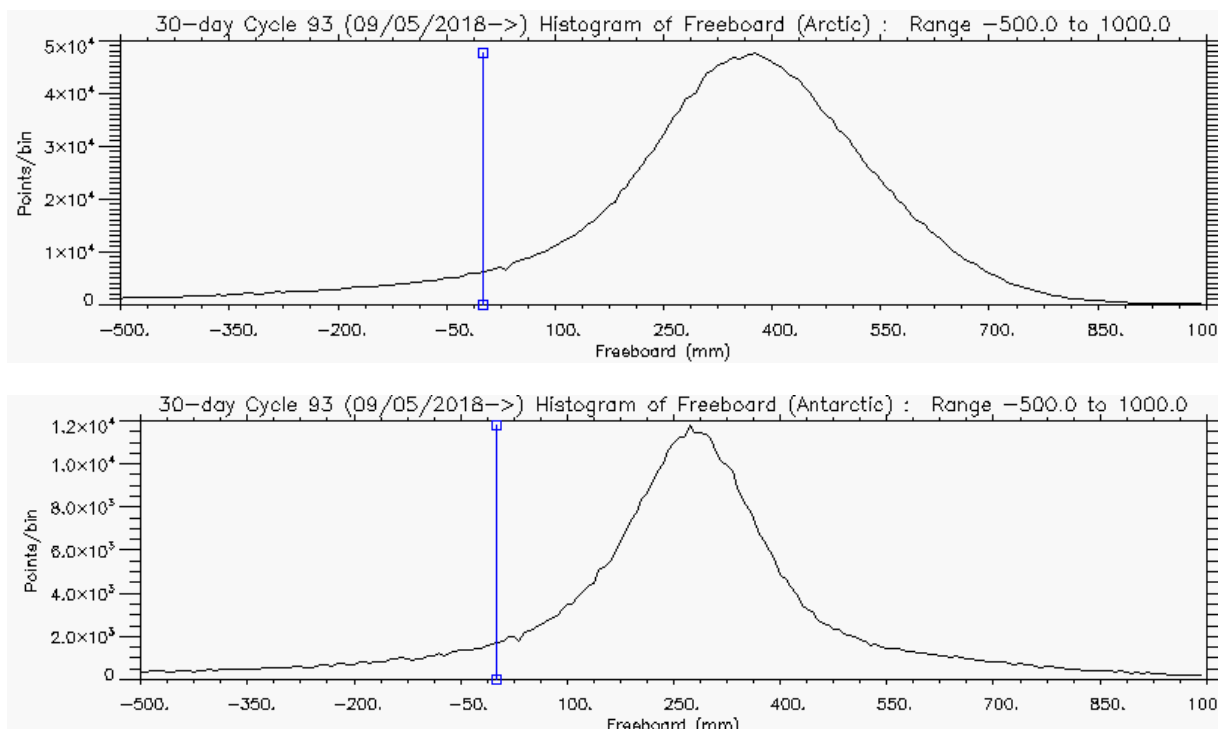
Figure 5 – Histogram of Freeboard for Arctic (above) and Antarctic (below) for cycle #93
