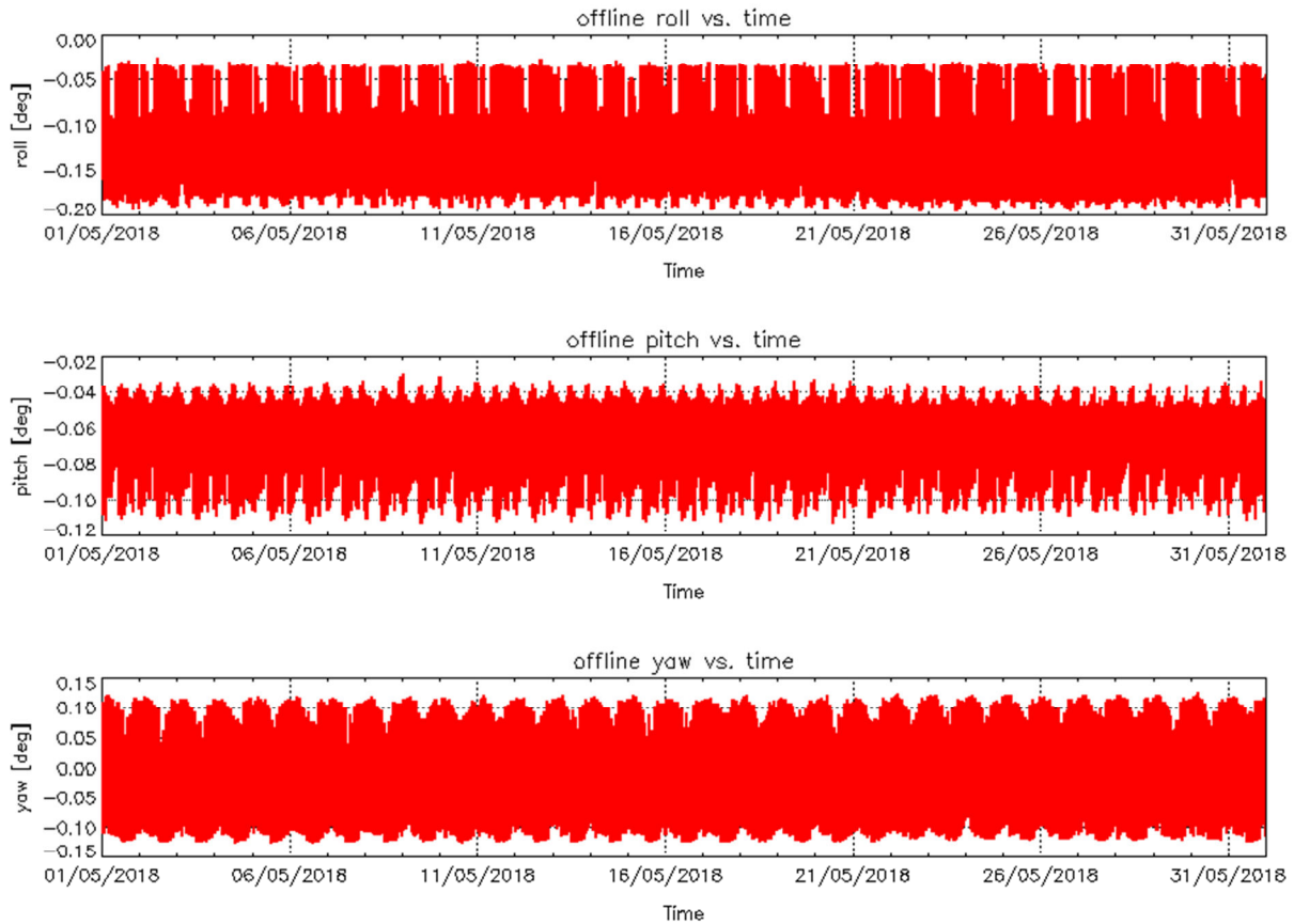
Figure 4 – Roll (top), Pitch (middle) and Yaw (bottom) values for L1B Products during cycle #93.
