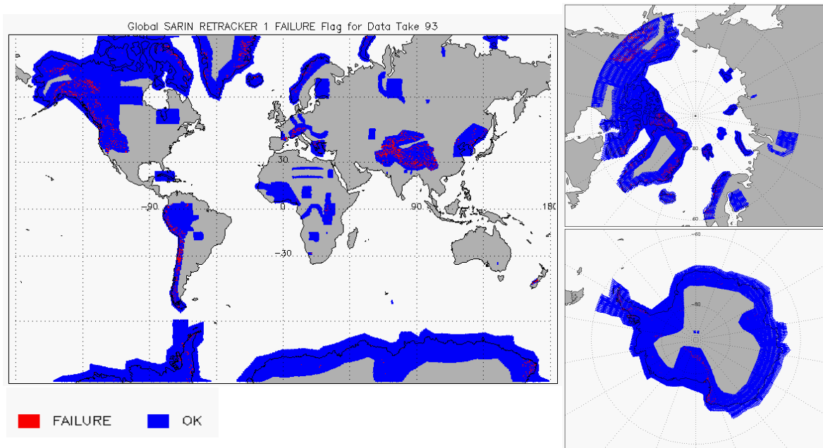
Figure 11 – Global plots showing Retracker Failure Flags for SARIn mode for cycle #93
