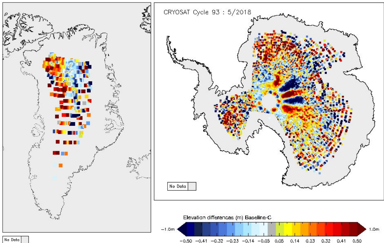
Figure 14 - Greenland and Antarctica maps of LRM elevation differences for cycle #93.
