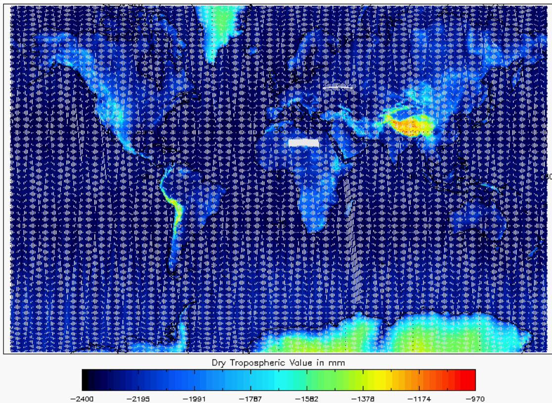
Figure 16 - Global plot of Dry Tropospheric Correction for cycle #93
