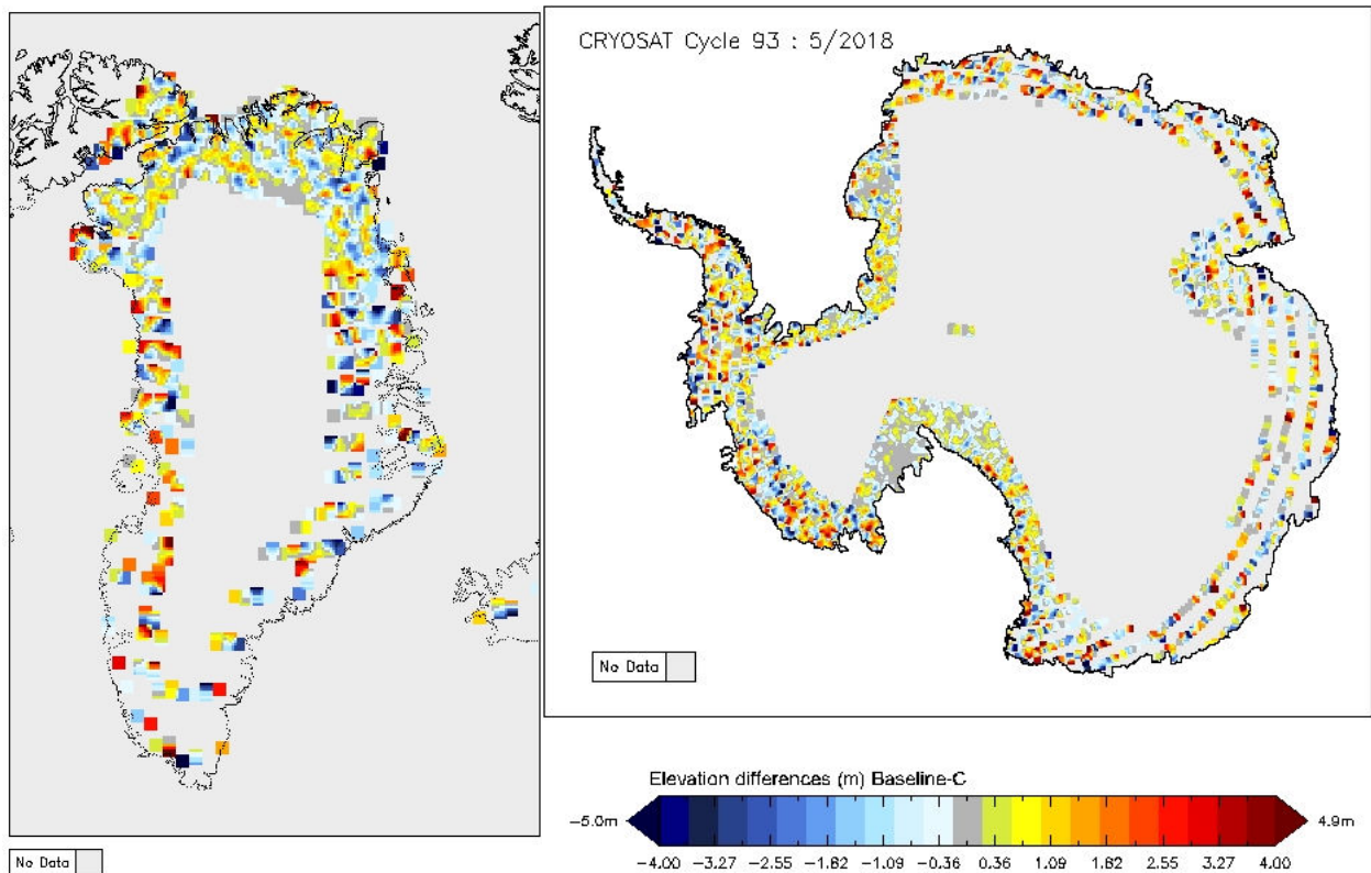
Figure 15 - Greenland and Antarctica maps of SARIn elevation differences for cycle #93
