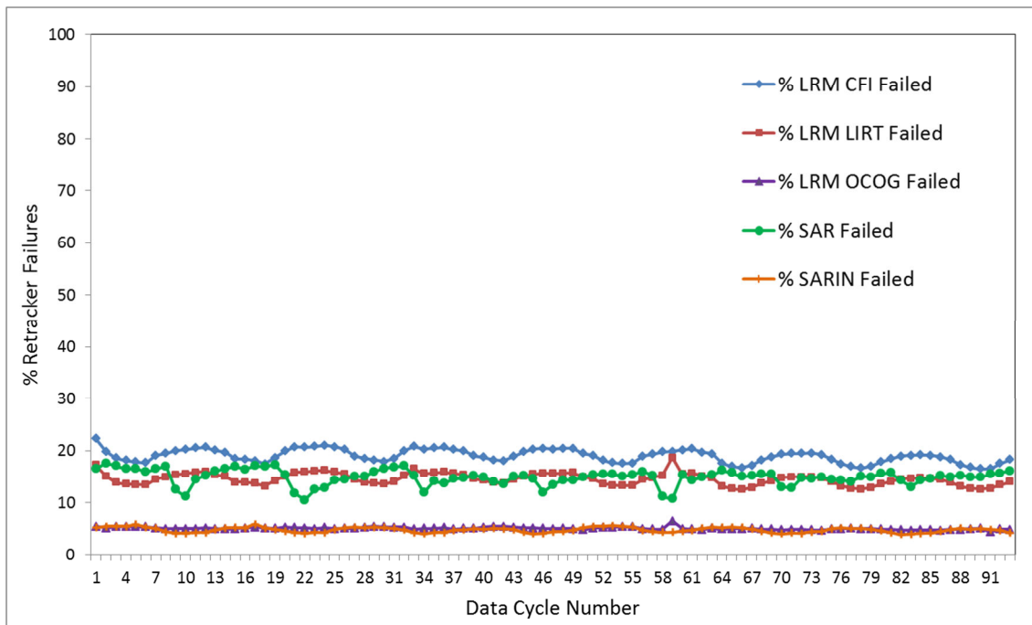
Figure 8 – Time Series for Retracker Failure Flags
