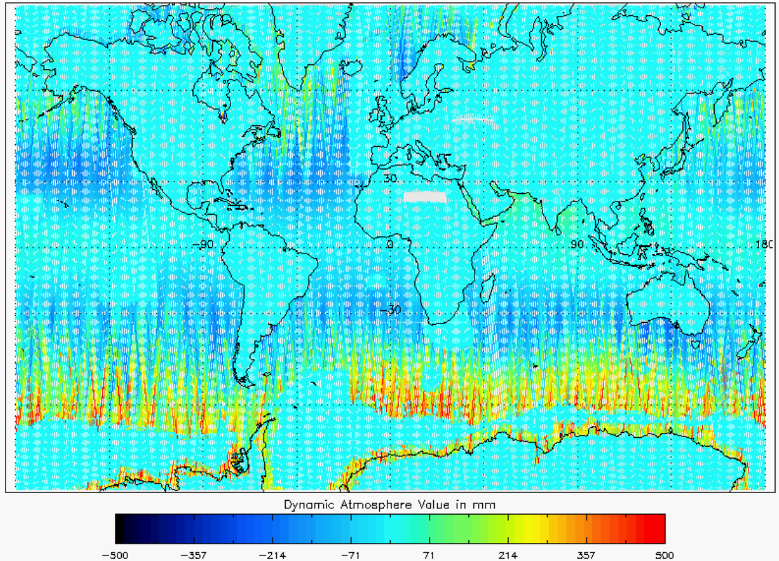
Figure 22 - Global plot of Dynamic Atmospheric Correction for cycle #93
