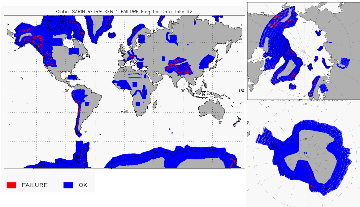
Figure 11 – Global plots showing Retracker Failure Flags for SARIn mode for cycle #92
