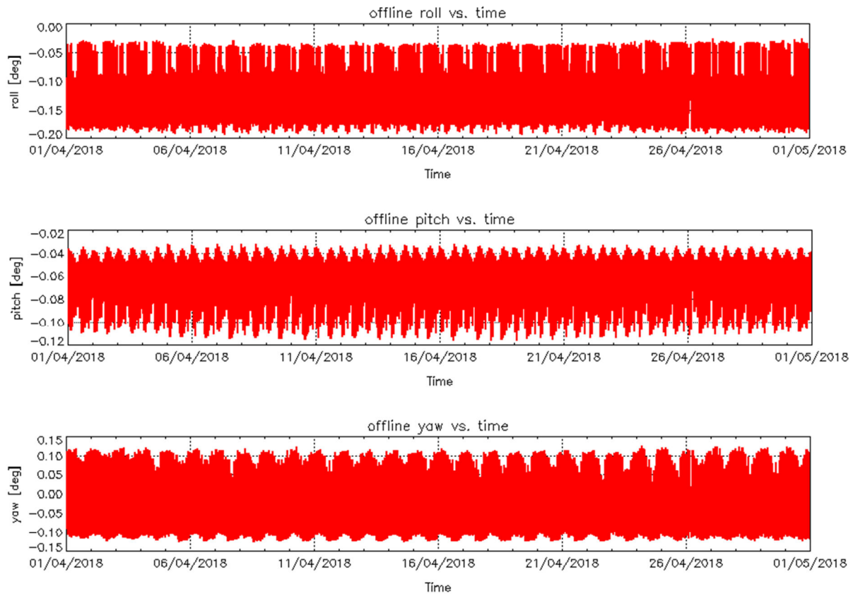
Figure 4 – Roll (top), Pitch (middle) and Yaw (bottom) values for L1B Products during cycle #92.
