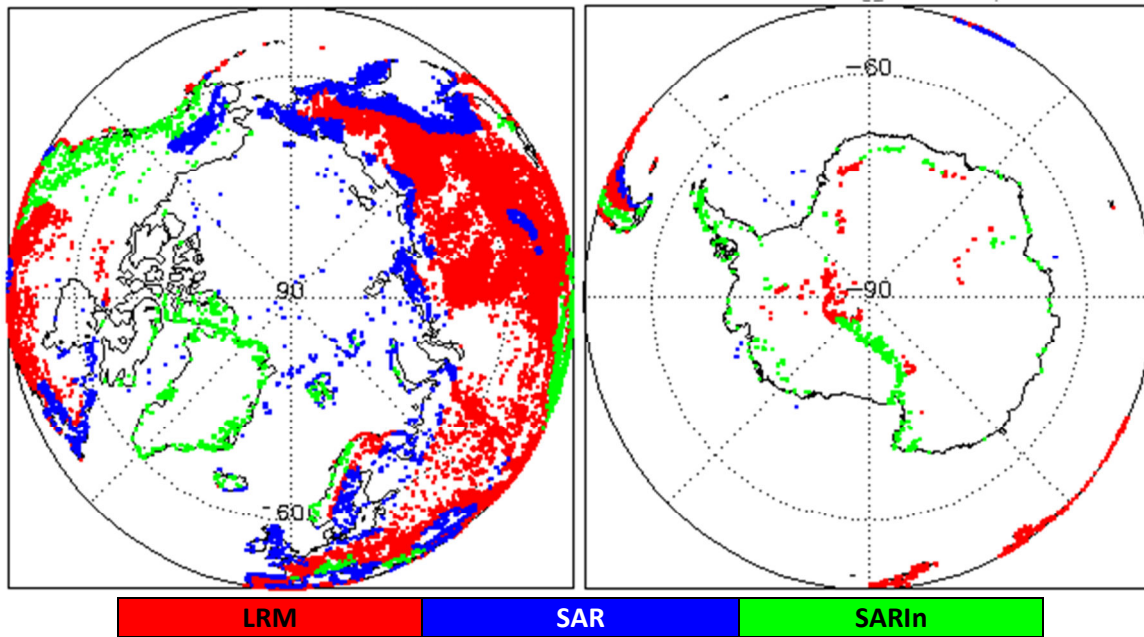
Figure 2 - Polar plots showing areas of loss of track in all SIRAL modes L0 data during April 2018.
