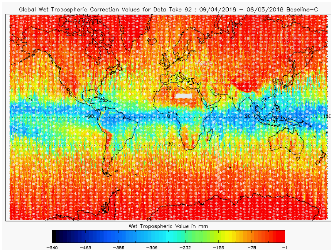
Figure 18 - Global plot of Wet Tropospheric Correction for cycle #92
