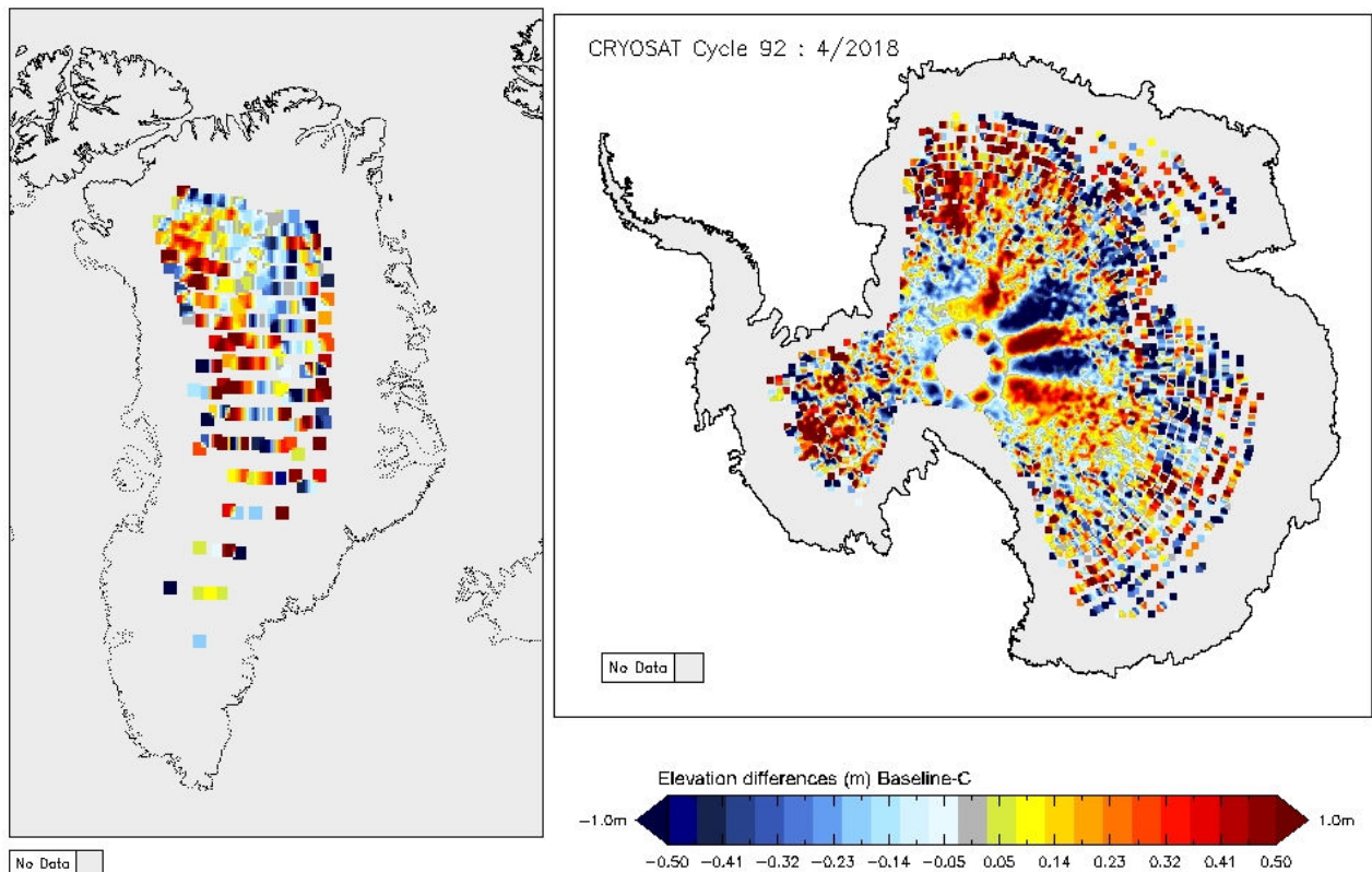
Figure 14 - Greenland and Antarctica maps of LRM elevation differences for cycle #92.
