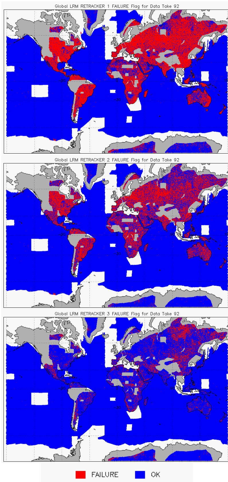
Figure 9 – Global plots showing Retracker Failure Flags for LRM mode for cycle #92: LRM CFI (top), LRM LIRT (middle), LRM OCOG (bottom)
