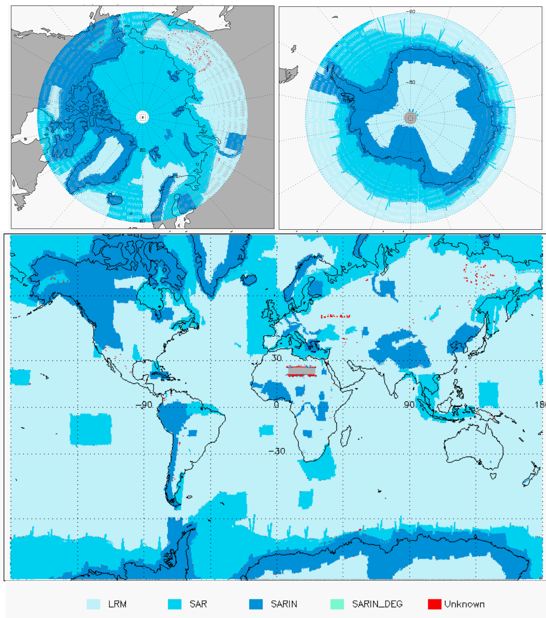
Figure 3 - Global and Polar plots of SIRAL Modes for cycle #92.
