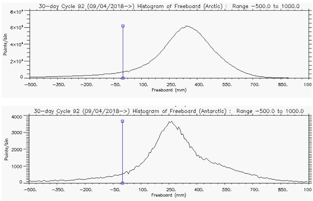
Figure 5 – Histogram of Freeboard for Arctic (above) and Antarctic (below) for cycle #92
