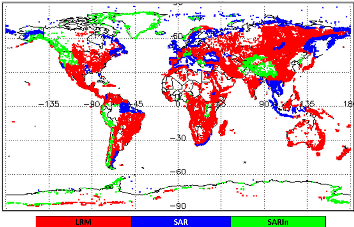
Figure 1 - Global plot showing areas of loss of track in all SIRAL modes L0 data during April 2018.
