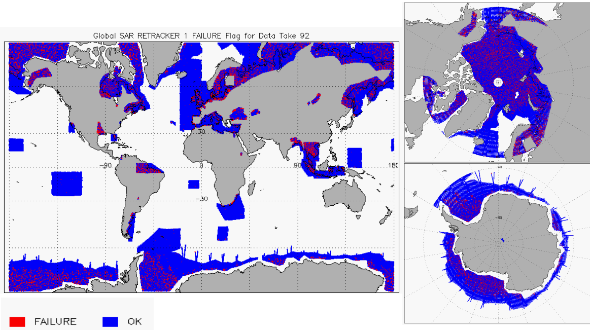
Figure 10 – Global plots showing Retracker Failure Flags for SAR mode for cycle #92
