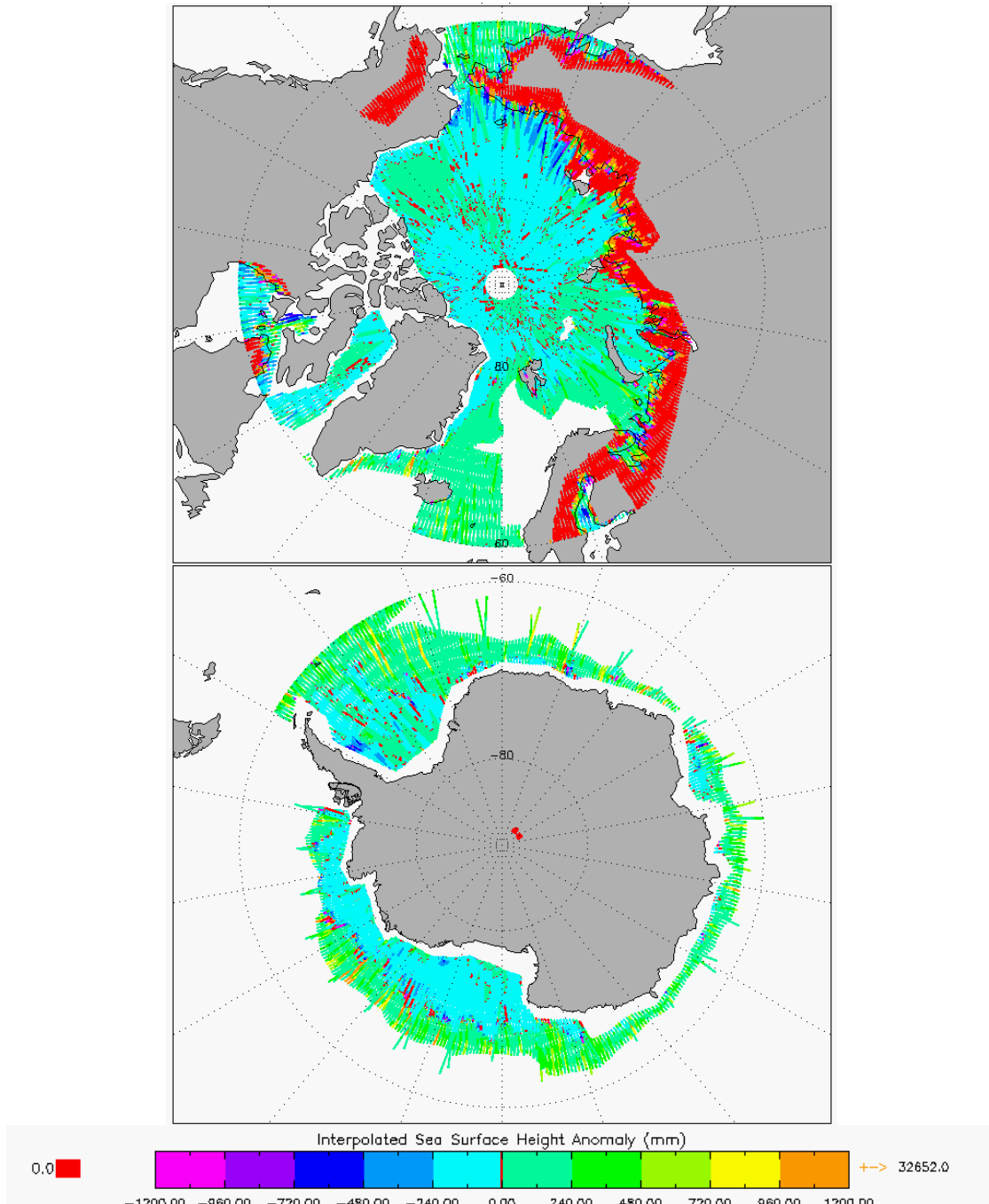
Figure 7 –Polar plots of SSHA for cycle #92.
