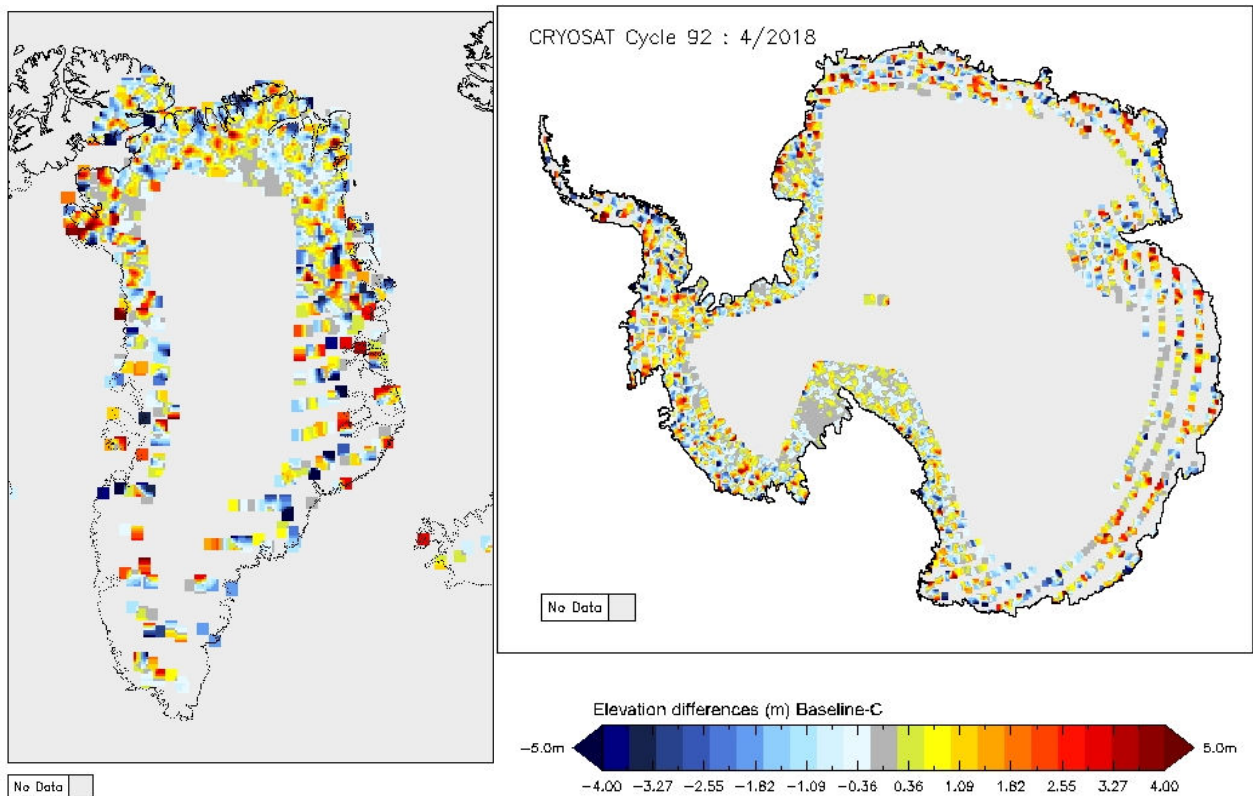
Figure 15 - Greenland and Antarctica maps of SARIn elevation differences for cycle #92
