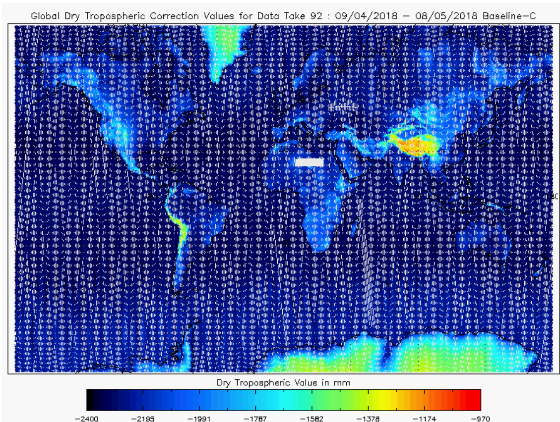
Figure 16 - Global plot of Dry Tropospheric Correction for cycle #92
