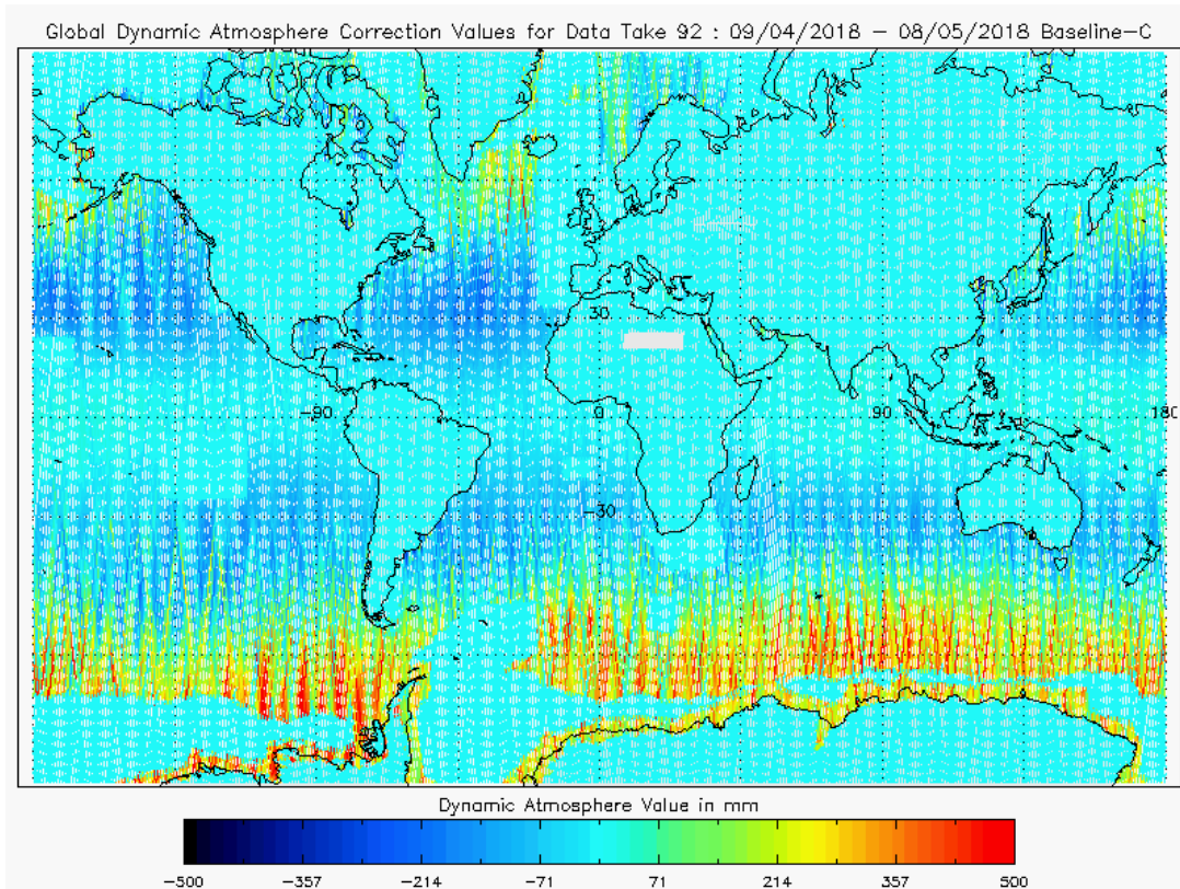
Figure 22 - Global plot of Dynamic Atmospheric Correction for cycle #92
