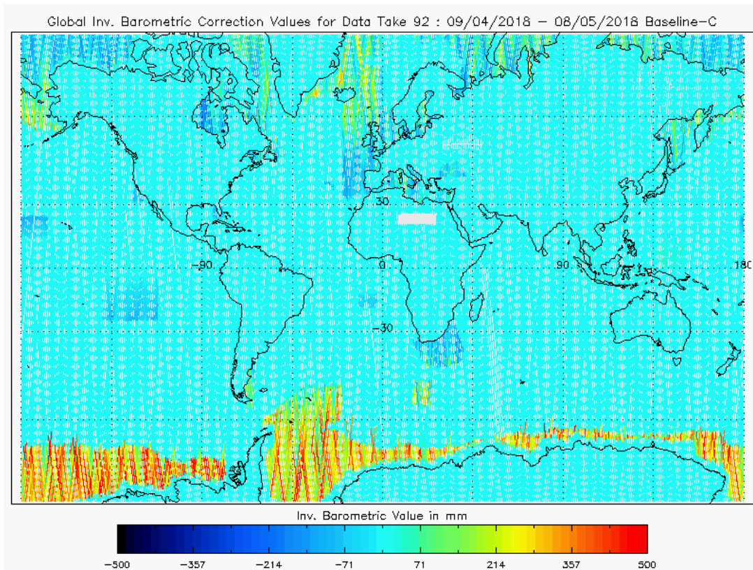
Figure 20 - Global plot of Inverse Barometric Correction for cycle #92
