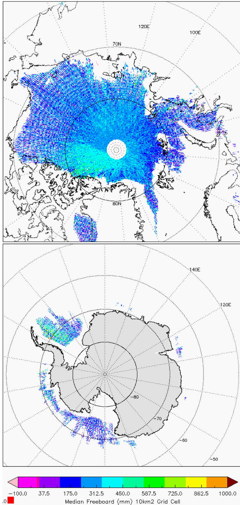
Figure 6 - Polar plots of 10km Gridded Freeboard values from L2 SAR products in cycle #92.
