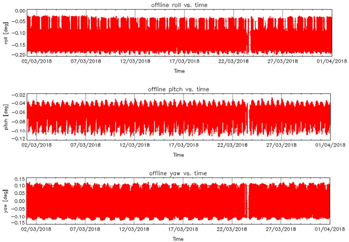
Figure 4 – Roll (top), Pitch (middle) and Yaw (bottom) values for L1B Products during cycle #91.
