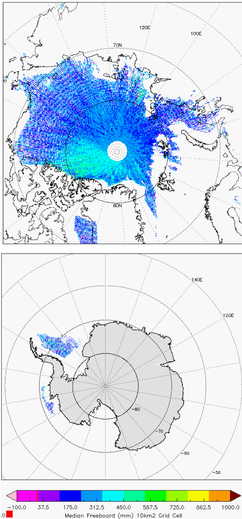
Figure 7 - Polar plots of 10km Gridded Freeboard values from L2 SAR products in cycle #90.
