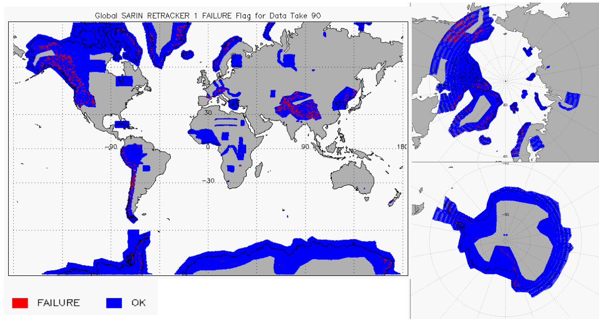
Figure 12 – Global plots showing Retracker Failure Flags for SARIn mode for cycle #90
