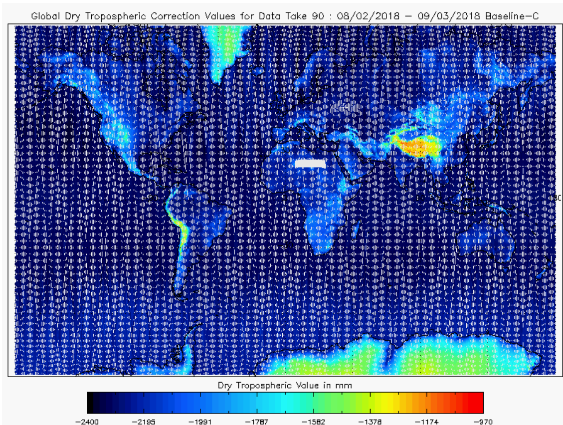
Figure 17 - Global plot of Dry Tropospheric Correction for cycle #90
