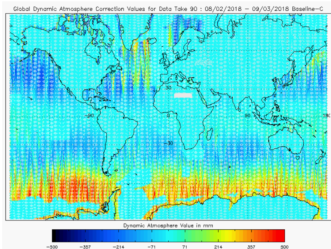
Figure 23 - Global plot of Dynamic Atmospheric Correction for cycle #90
