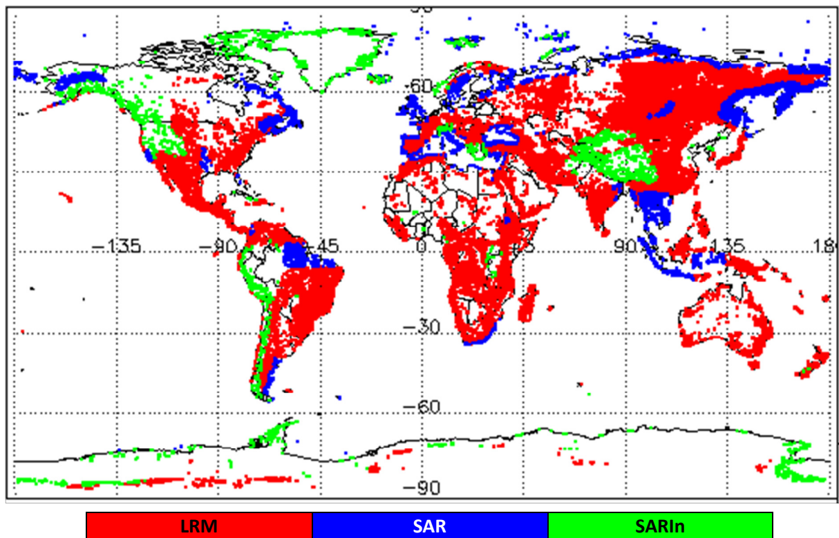
Figure 1 - Global plot showing areas of loss of track in all SIRAL modes L0 data during February 2018.
