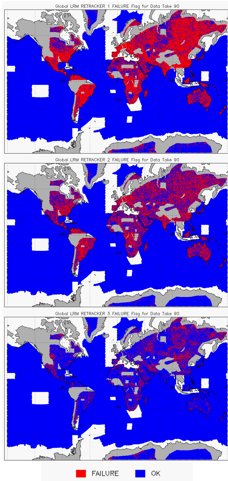
Figure 10 – Global plots showing Retracker Failure Flags for LRM mode for cycle #90: LRM CFI (top), LRM LIRT (middle), LRM OCOG (bottom)
