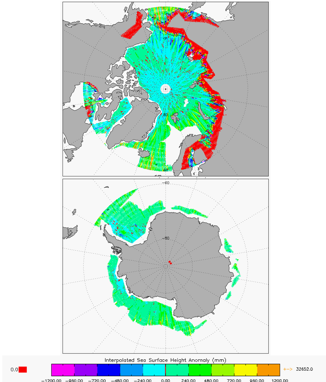
Figure 8 –Polar plots of SSHA for cycle #90.
