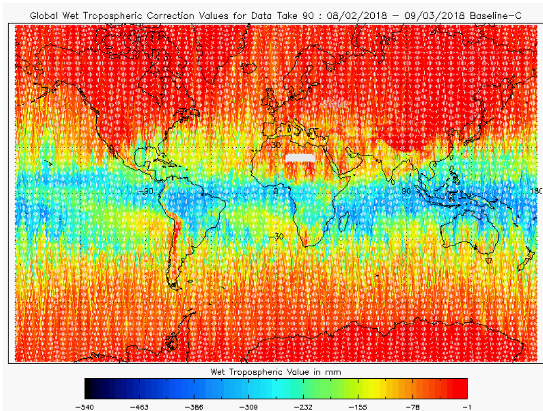
Figure 19 - Global plot of Wet Tropospheric Correction for cycle #90
