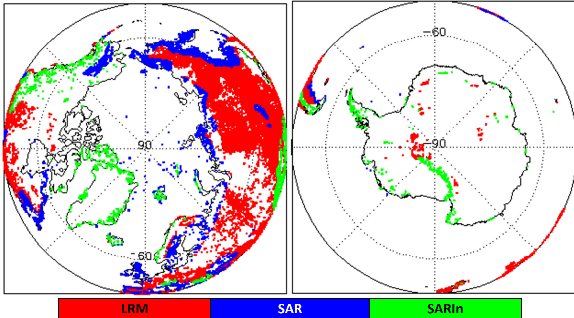
Figure 2 - Polar plots showing areas of loss of track in all SIRAL modes L0 data during February 2018.
