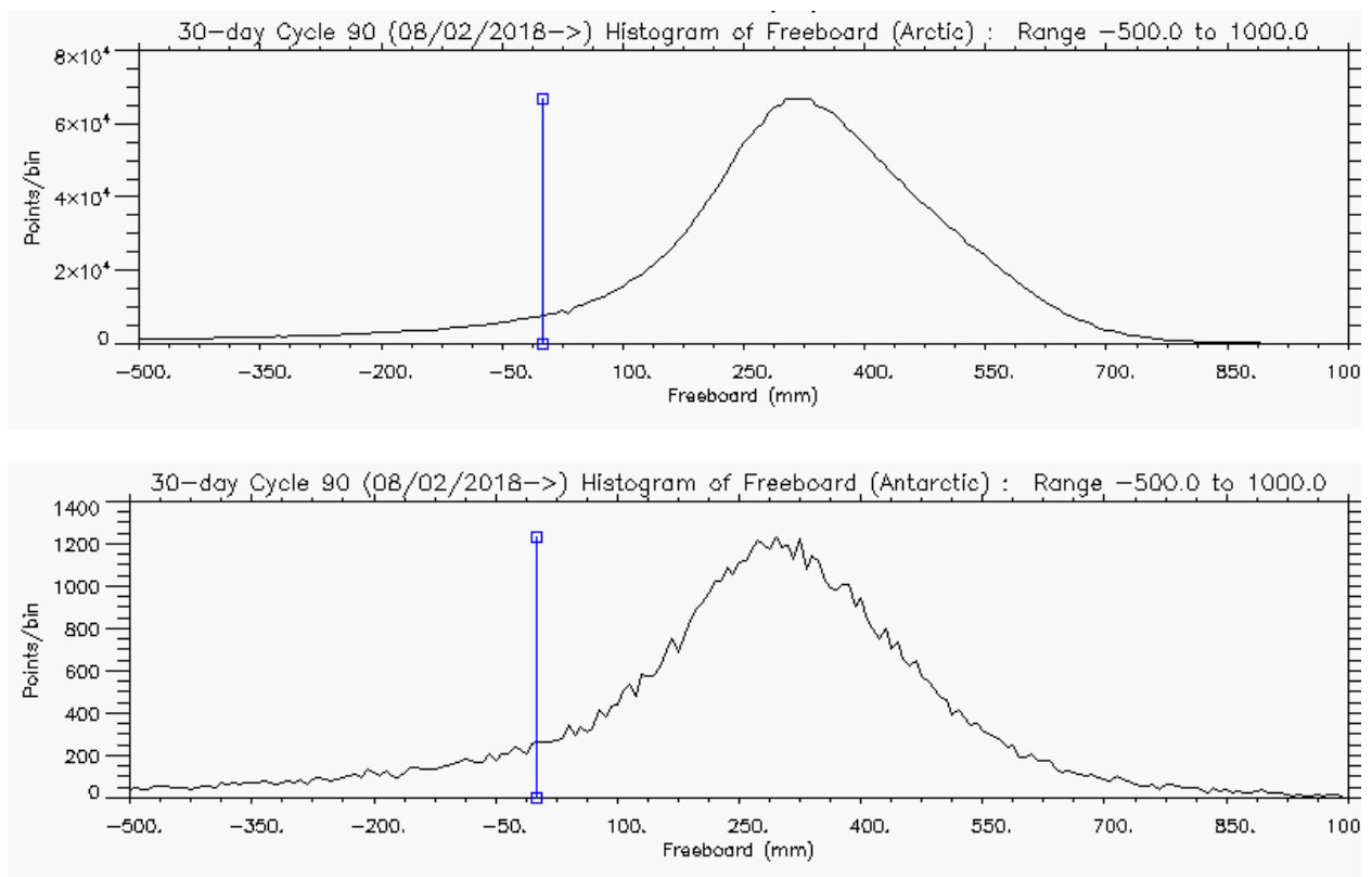
Figure 6 – Histogram of Freeboard for Arctic (above) and Antarctic (below) for cycle #90
