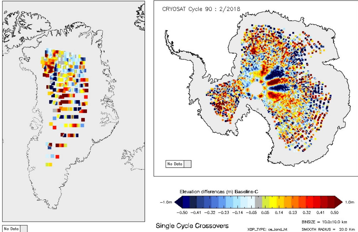
Figure 15 - Greenland and Antarctica maps of LRM elevation differences for cycle #90.
