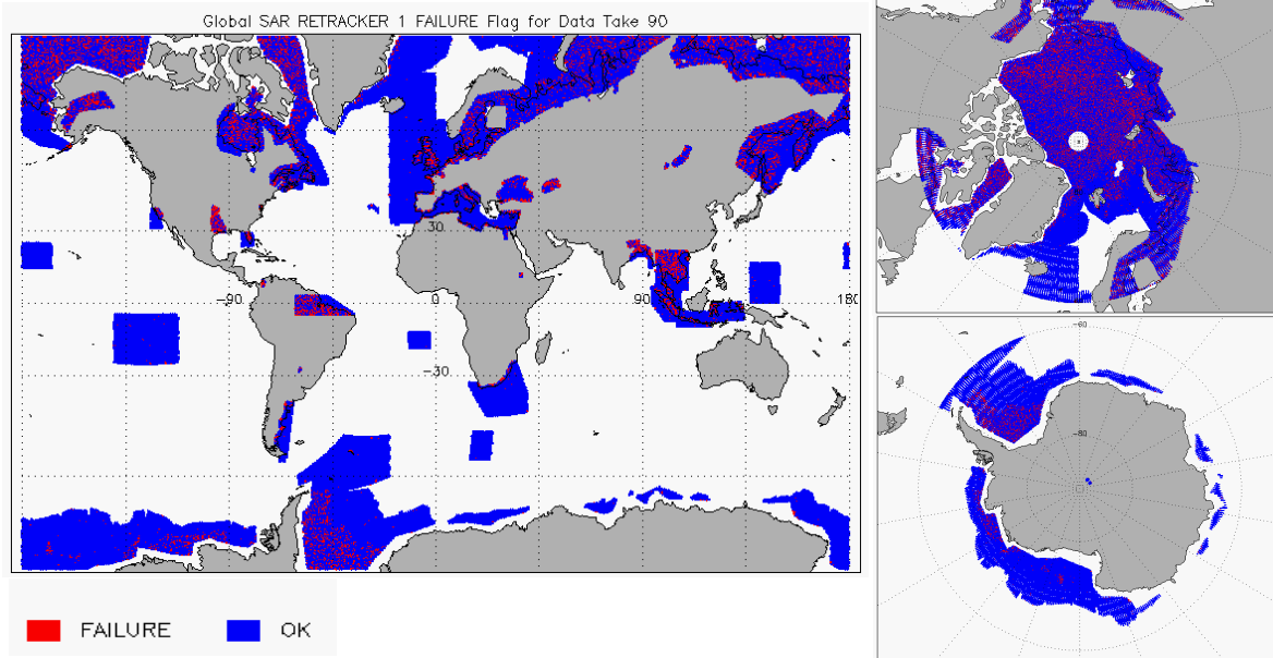
Figure 11 – Global plots showing Retracker Failure Flags for SAR mode for cycle #90
