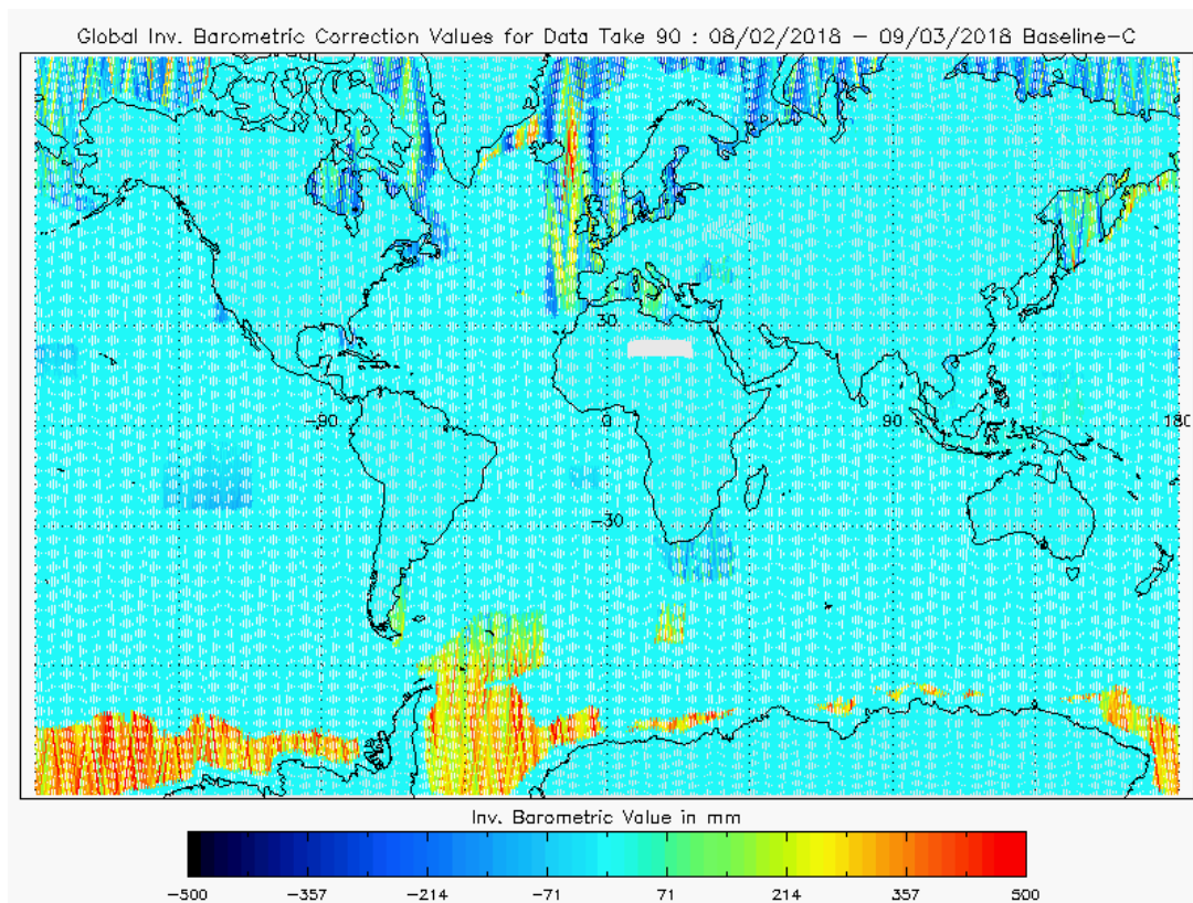
Figure 21 - Global plot of Inverse Barometric Correction for cycle #90
