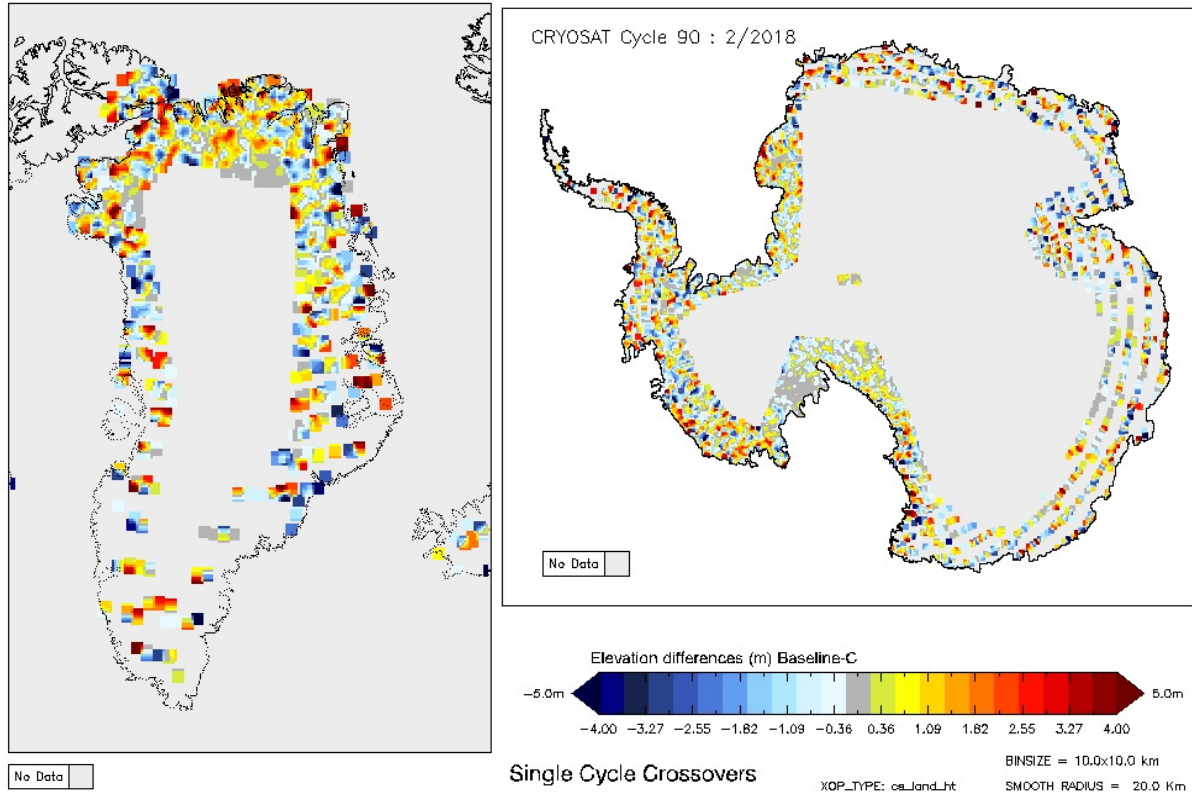
Figure 16 - Greenland and Antarctica maps of SARIn elevation differences for cycle #90
