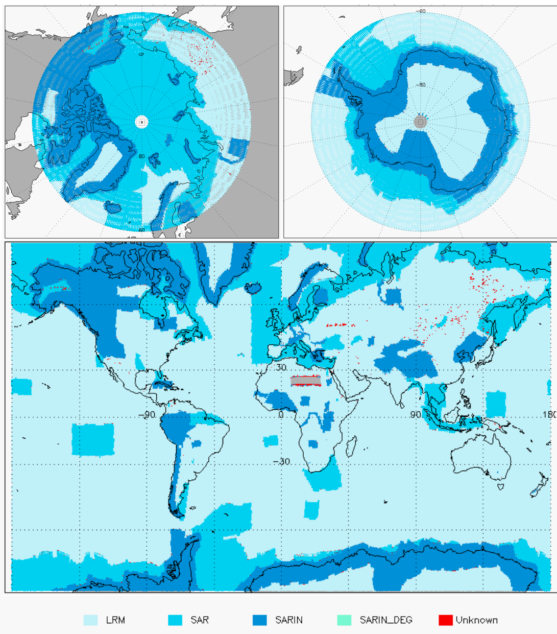
Figure 3 - Global and Polar plots of SIRAL Modes for cycle #90.
