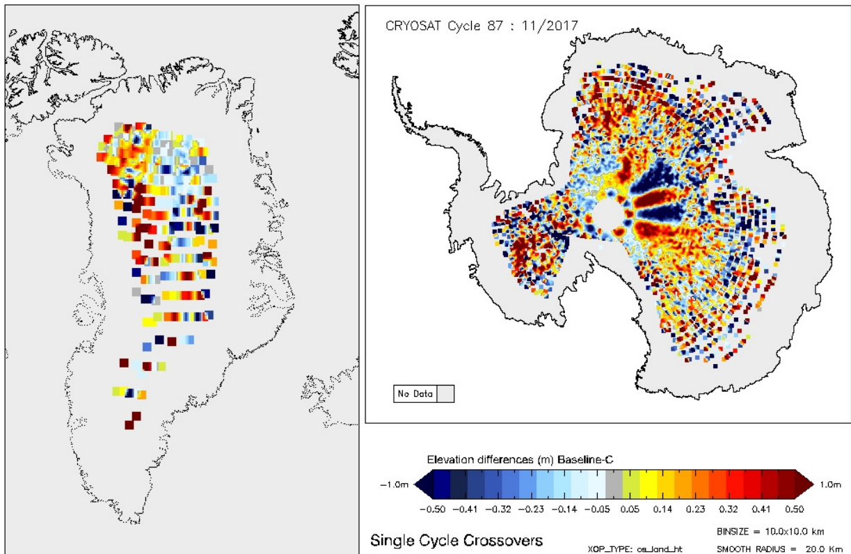
Figure 14 - Greenland and Antarctica maps of LRM elevation differences for cycle #87.
