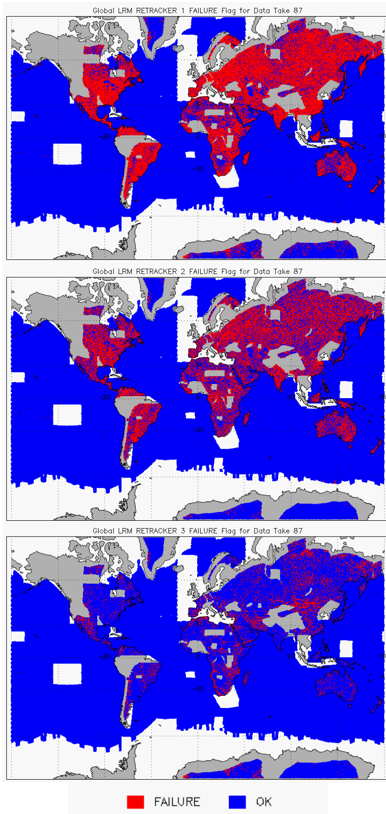
Figure 9 – Global plots showing Retracker Failure Flags for LRM mode for cycle #87: LRM CFI (top), LRM LIRT (middle), LRM OCOG (bottom)
