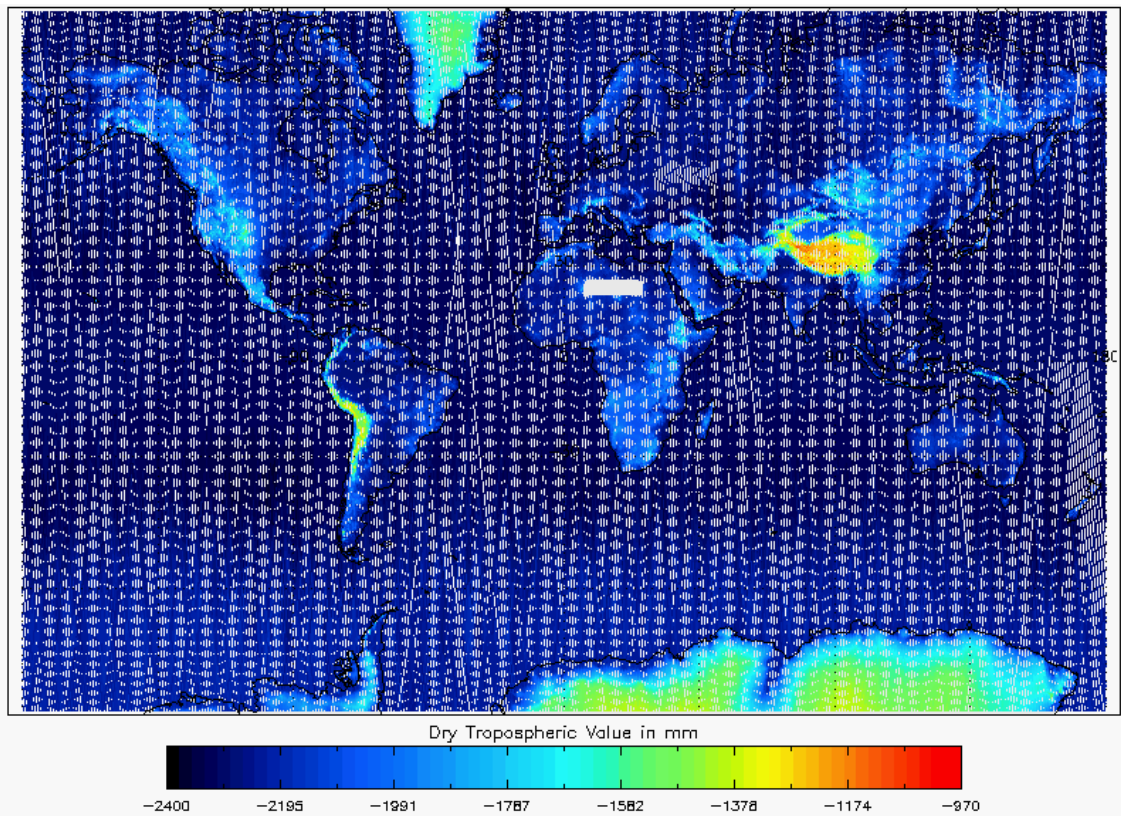
Figure 16 - Global plot of Dry Tropospheric Correction for cycle #87
