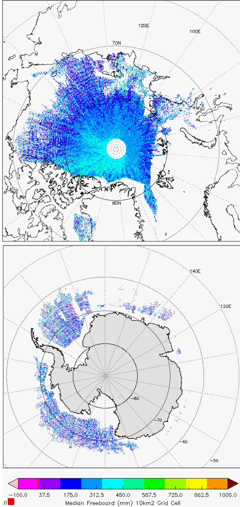
Figure 6 - Polar plots of 10km Gridded Freeboard values from L2 SAR products in cycle #87.
