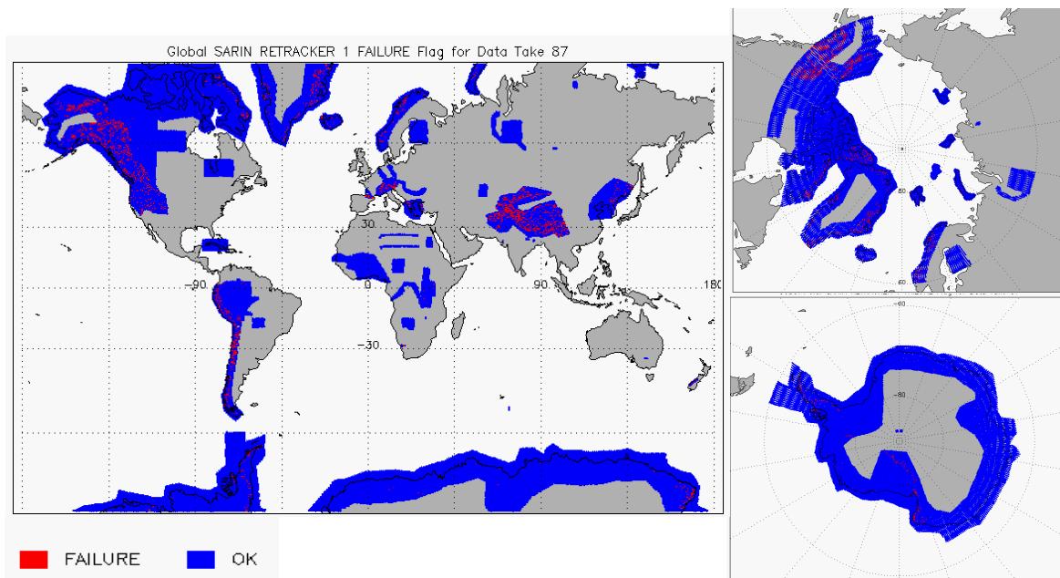
Figure 11 – Global plots showing Retracker Failure Flags for SARIn mode for cycle #87
