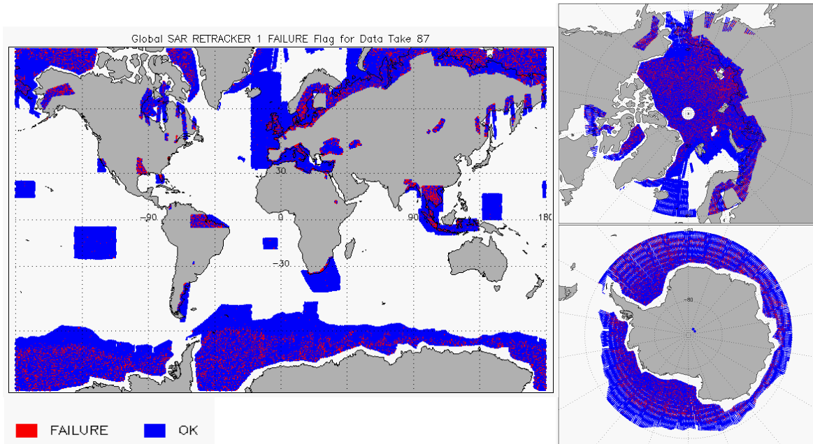
Figure 10 – Global plots showing Retracker Failure Flags for SAR mode for cycle #87
