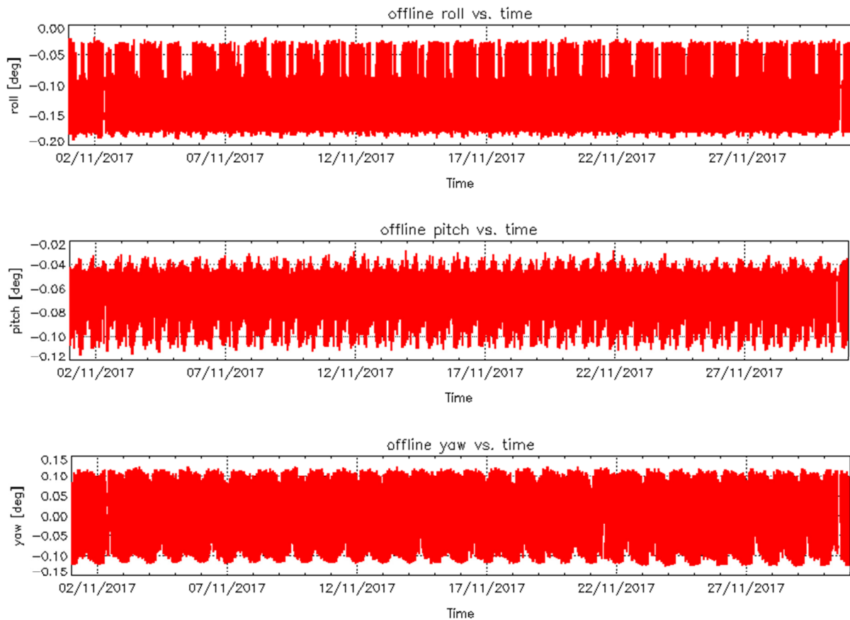
Figure 4 – Roll (top), Pitch (middle) and Yaw (bottom) values for L1B Products during cycle #87.
