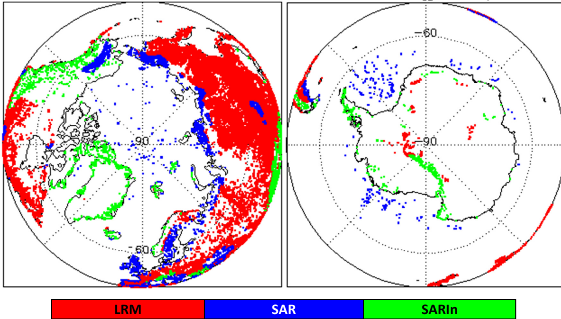
Figure 2 - Polar plots showing areas of loss of track in all SIRAL modes L0 data during November 2017.
