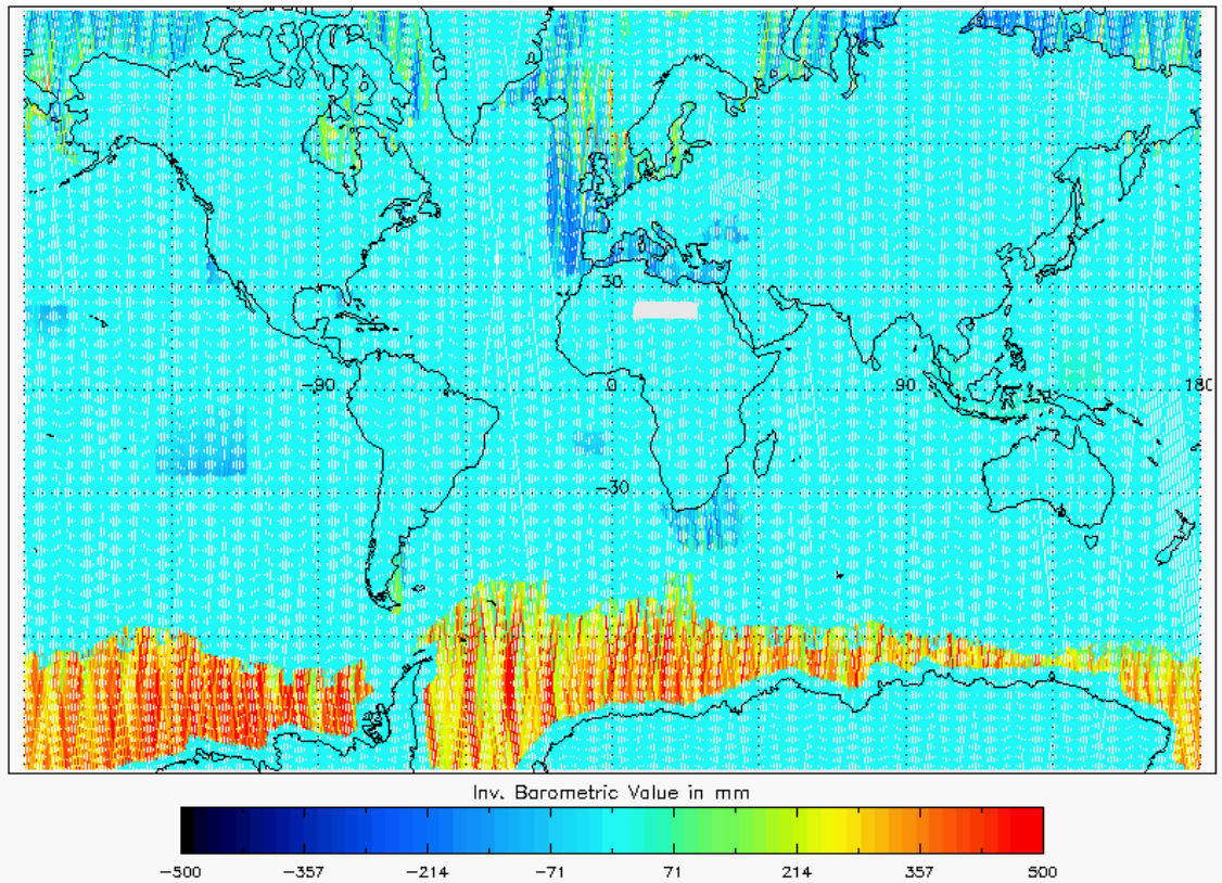
Figure 20 - Global plot of Inverse Barometric Correction for cycle #87
