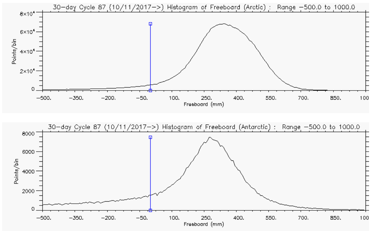
Figure 5 – Histogram of Freeboard for Arctic (above) and Antarctic (below) for cycle #87
