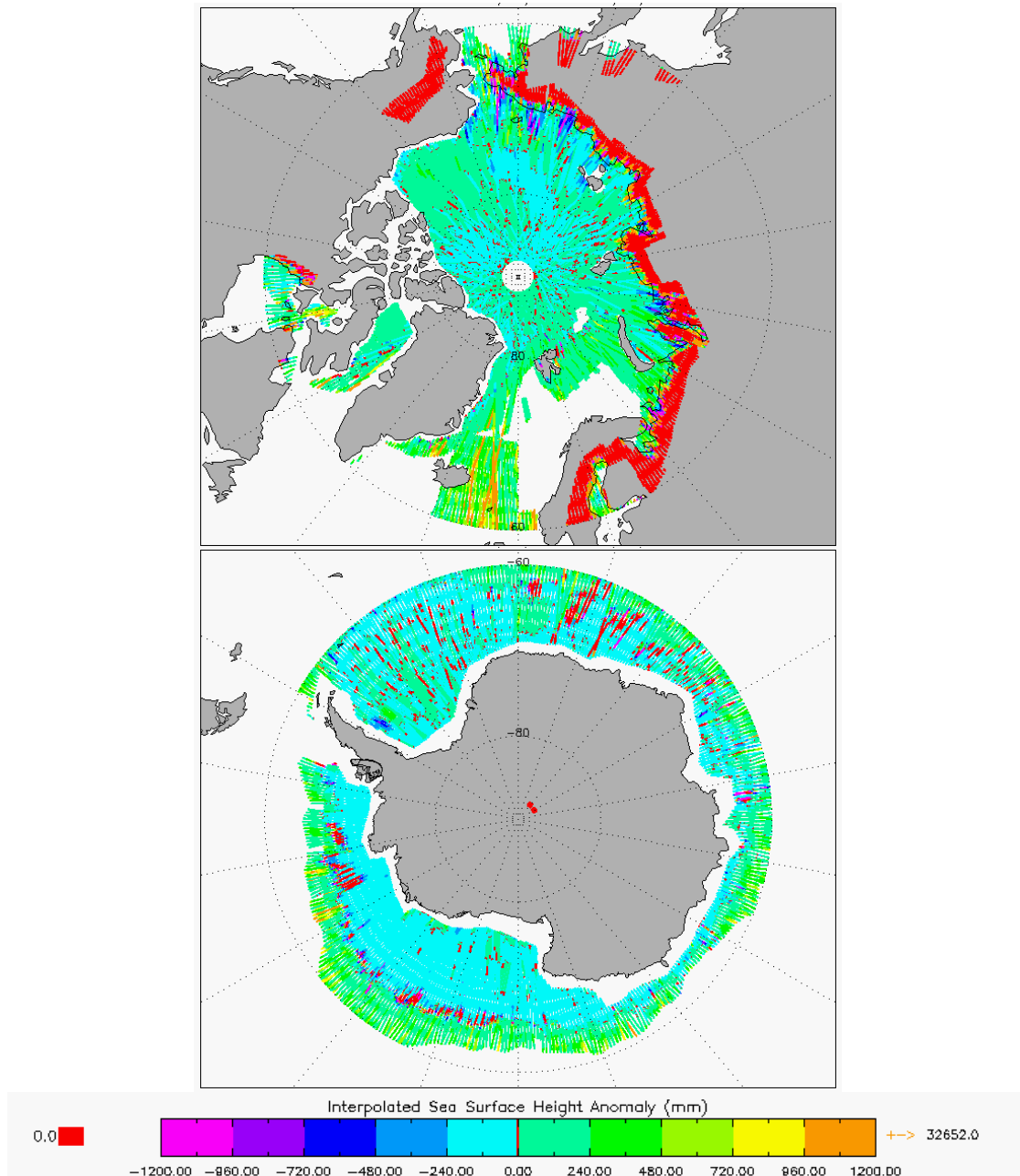
Figure 7 –Polar plots of SSHA for cycle #87.
