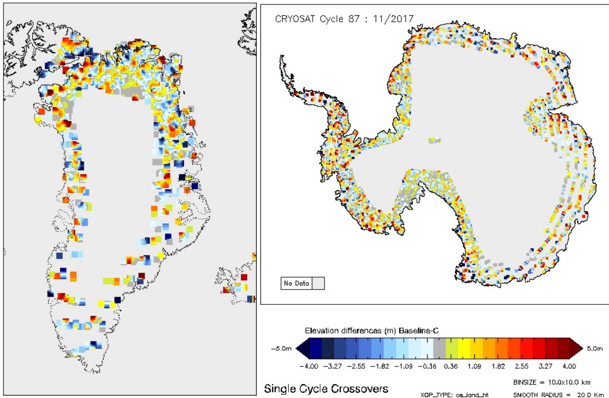
Figure 15 - Greenland and Antarctica maps of SARIn elevation differences for cycle #87
