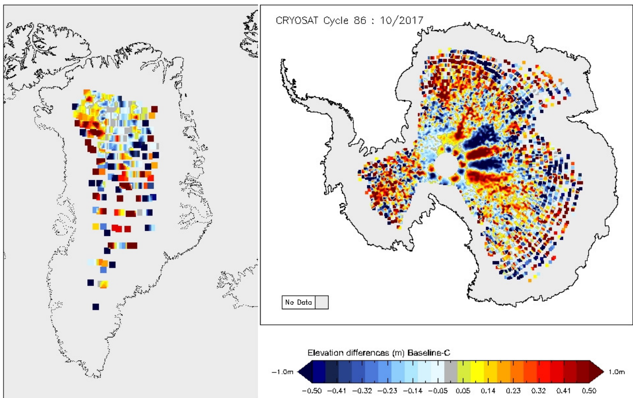
Figure 14 - Greenland and Antarctica maps of LRM elevation differences for cycle #86.
