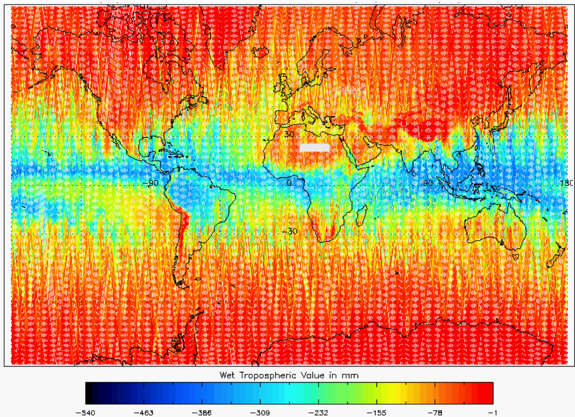
Figure 18 - Global plot of Wet Tropospheric Correction for cycle #86
