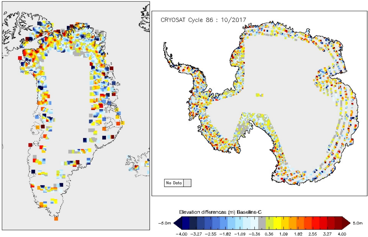
Figure 15 - Greenland and Antarctica maps of SARIn elevation differences for cycle #86
