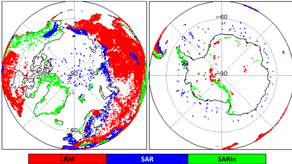
Figure 2 - Polar plots showing areas of loss of track in all SIRAL modes L0 data during October 2017.
