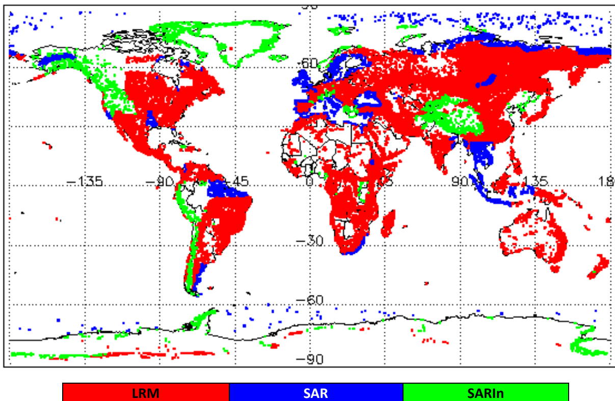
Figure 1 - Global plot showing areas of loss of track in all SIRAL modes L0 data during August 2017.
