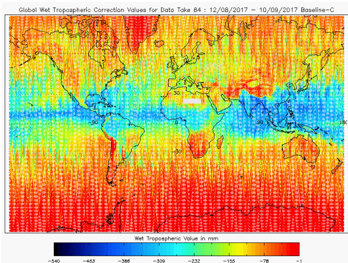
Figure 18 - Global plot of Wet Tropospheric Correction for cycle #84
