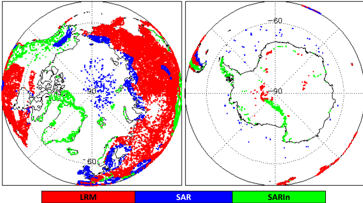
Figure 2 - Polar plots showing areas of loss of track in all SIRAL modes L0 data during August 2017.
