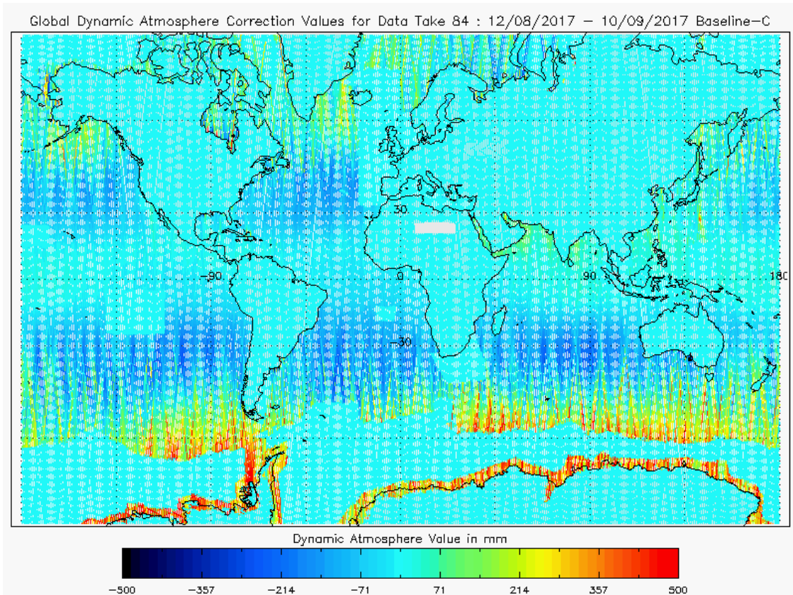
Figure 22 - Global plot of Dynamic Atmospheric Correction for cycle #84
