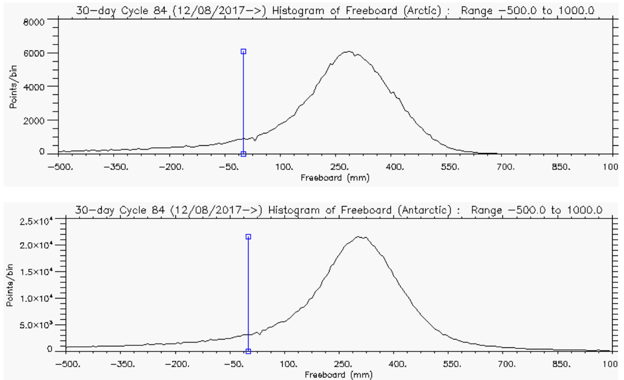
Figure 5 – Histogram of Freeboard for Arctic (above) and Antarctic (below) for cycle #84
