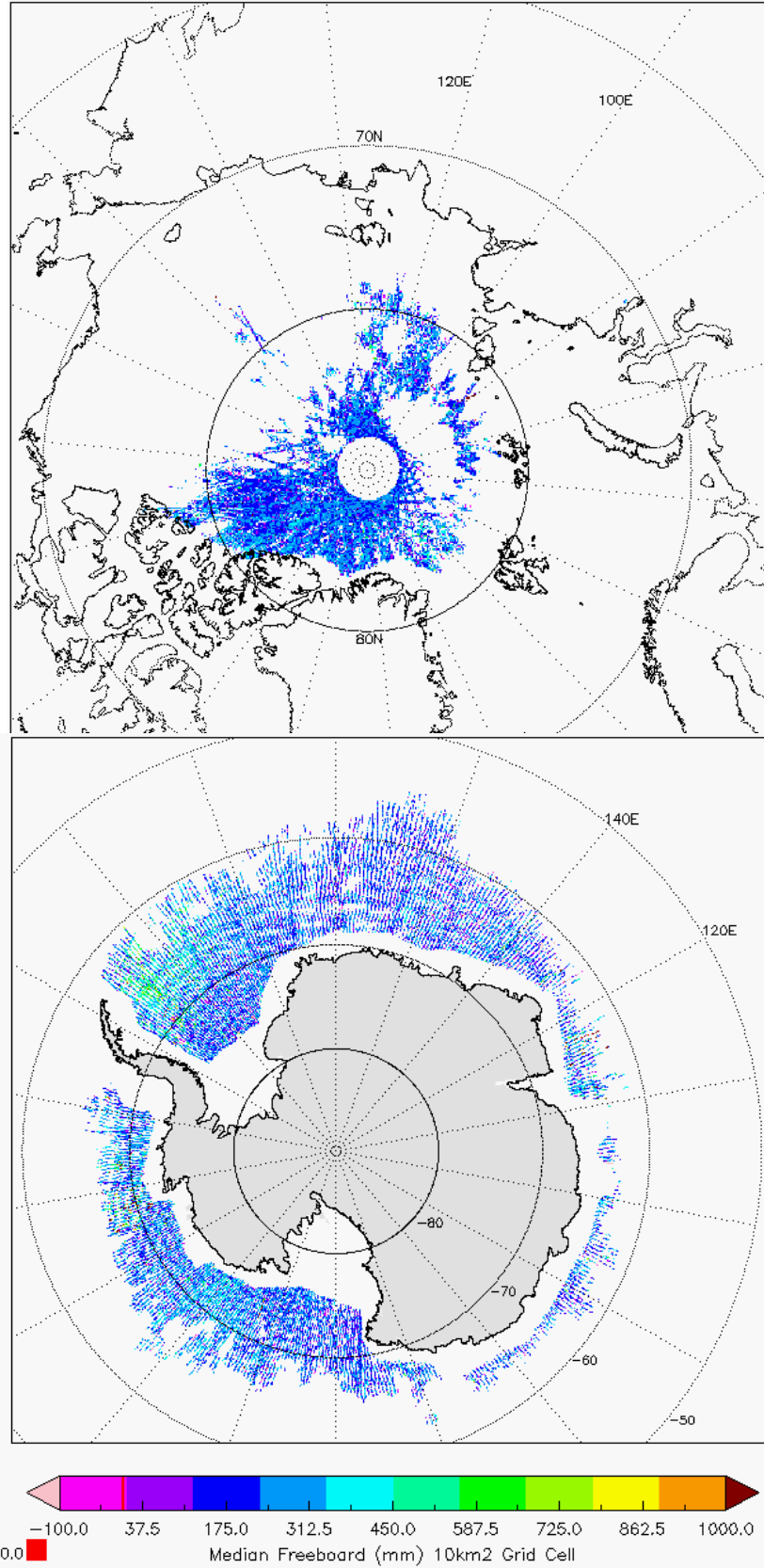
Figure 6 - Polar plots of 10 km gridded Freeboard values from L2 SAR products in cycle #84.
