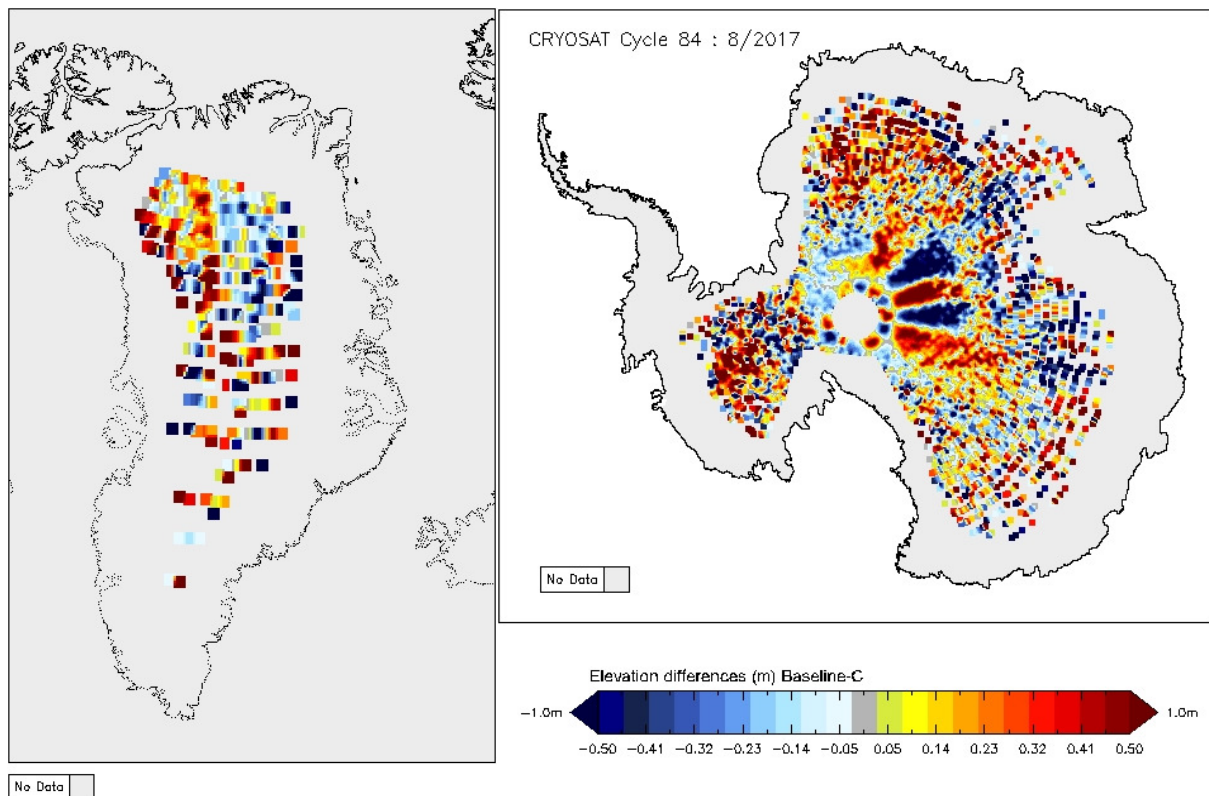
Figure 14 - Greenland and Antarctica maps of LRM elevation differences for cycle #84.
