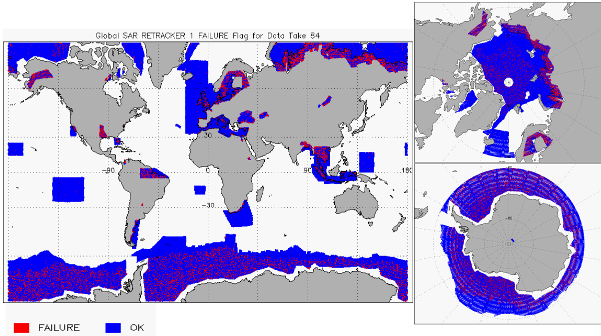
Figure 10 – Global plots showing Retracker Failure Flags for SAR mode for cycle #84
