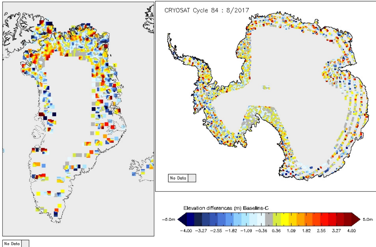
Figure 15 - Greenland and Antarctica maps of SARIn elevation differences for cycle #84
