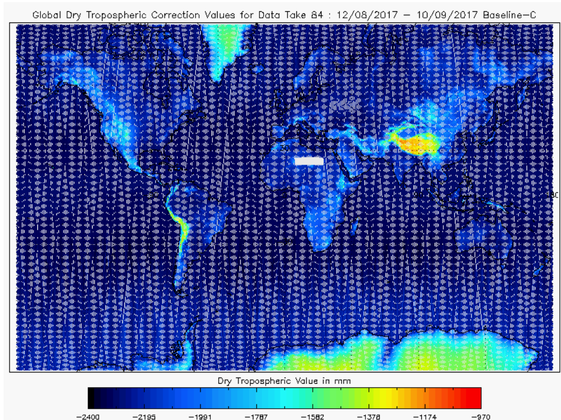
Figure 16 - Global plot of Dry Tropospheric Correction for cycle #84
