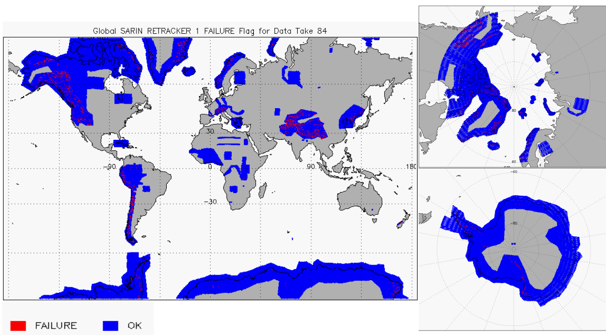
Figure 11 – Global plots showing Retracker Failure Flags for SARIn mode for cycle #84
