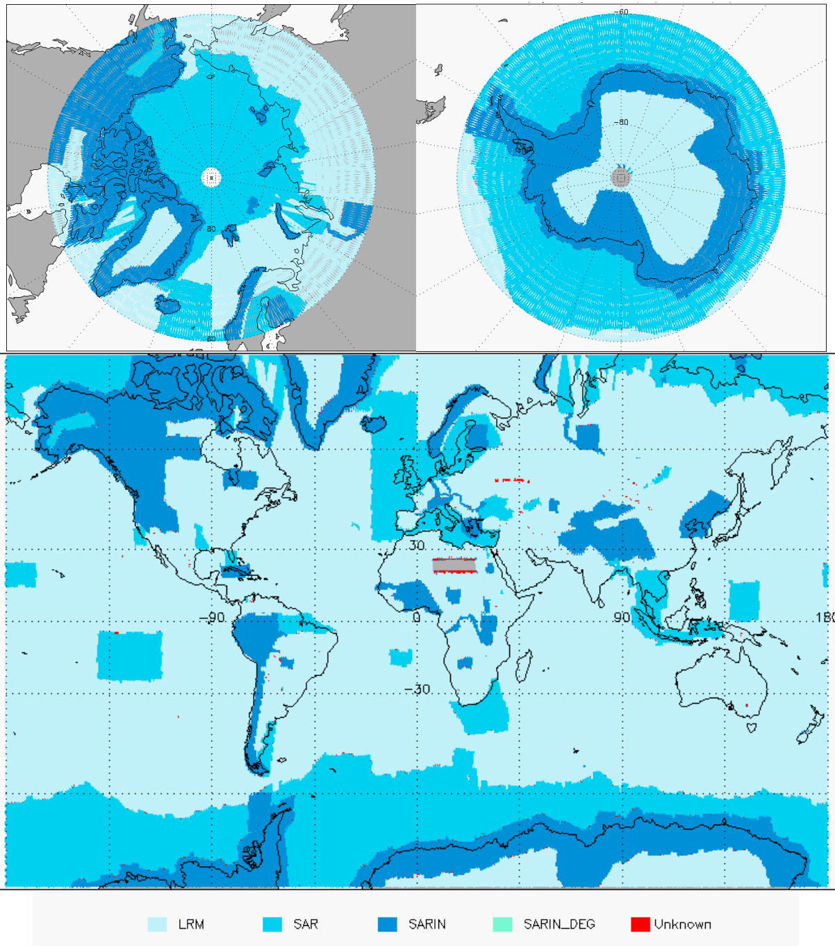
Figure 3 - Global and Polar plots of SIRAL Modes for cycle #84.
