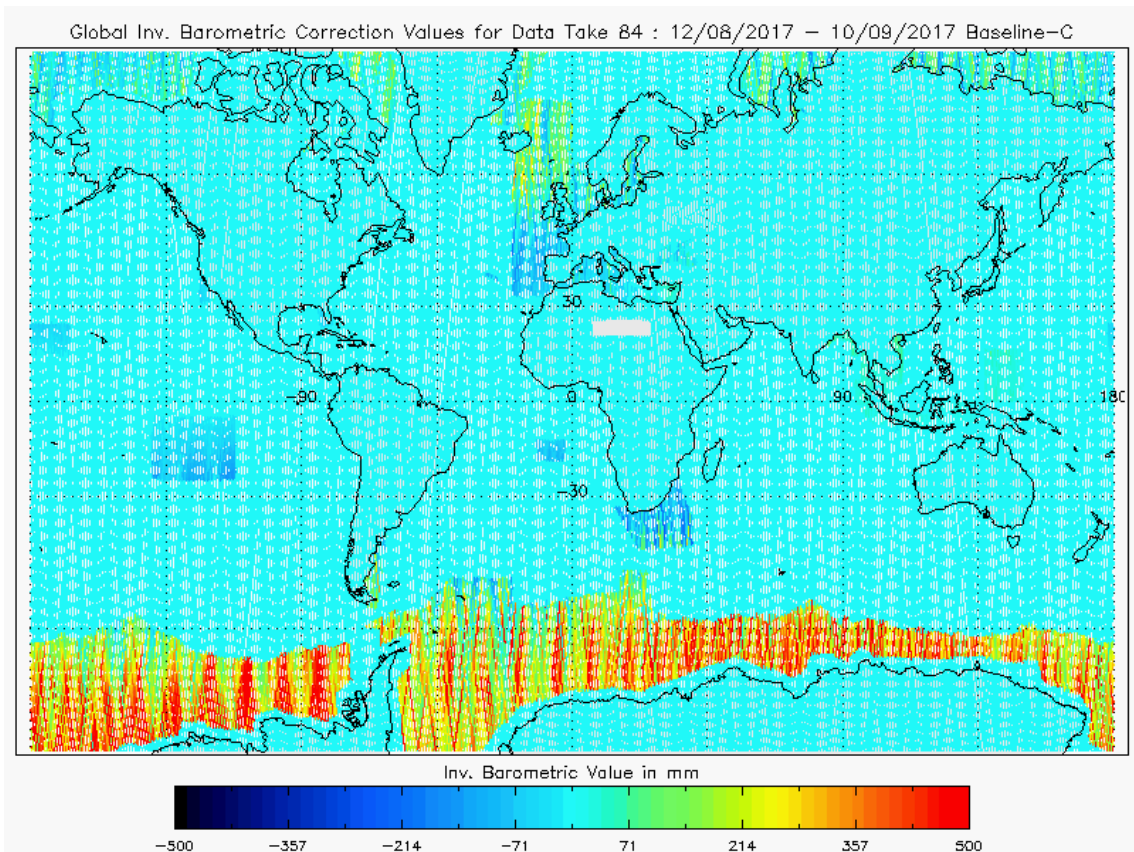
Figure 20 - Global plot of Inverse Barometric Correction for cycle #84
