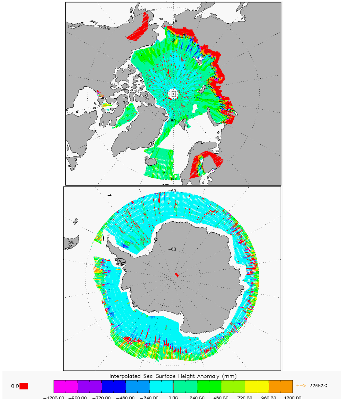
Figure 7 –Polar plots of SSHA for cycle #84.
