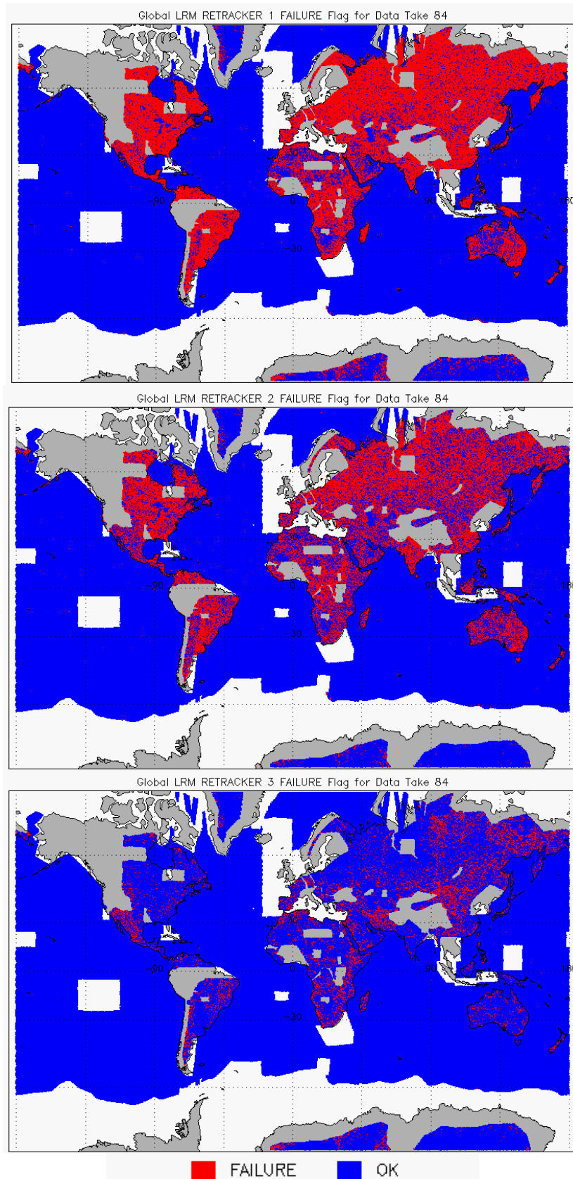
Figure 9 – Global plots showing Retracker Failure Flags for LRM mode for cycle #84: LRM CFI (top), LRM LIRT (middle), LRM OCOG (bottom)
