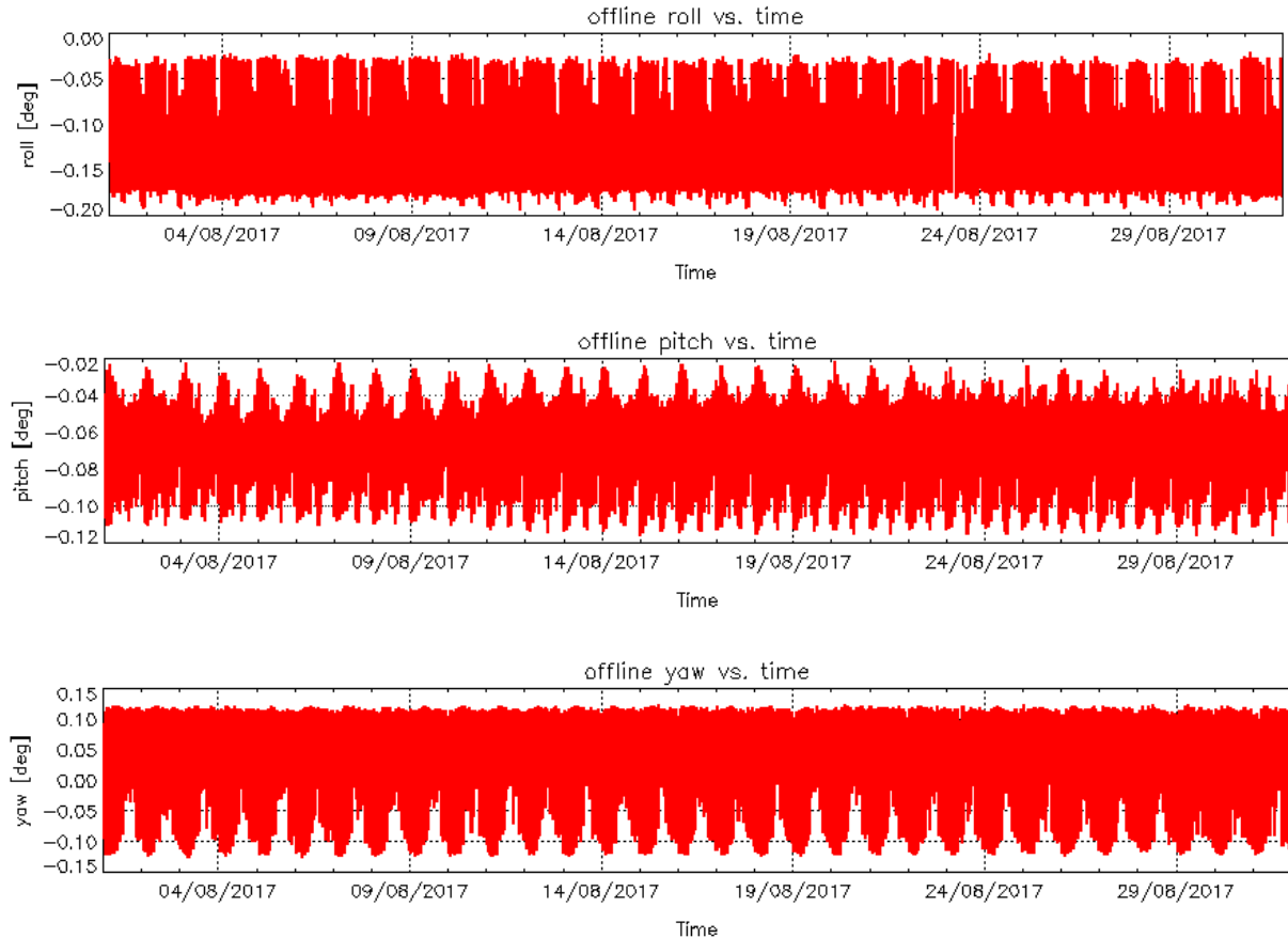
Figure 4 – Roll (top), Pitch (middle) and Yaw (bottom) values for L1B Products during cycle #84.
