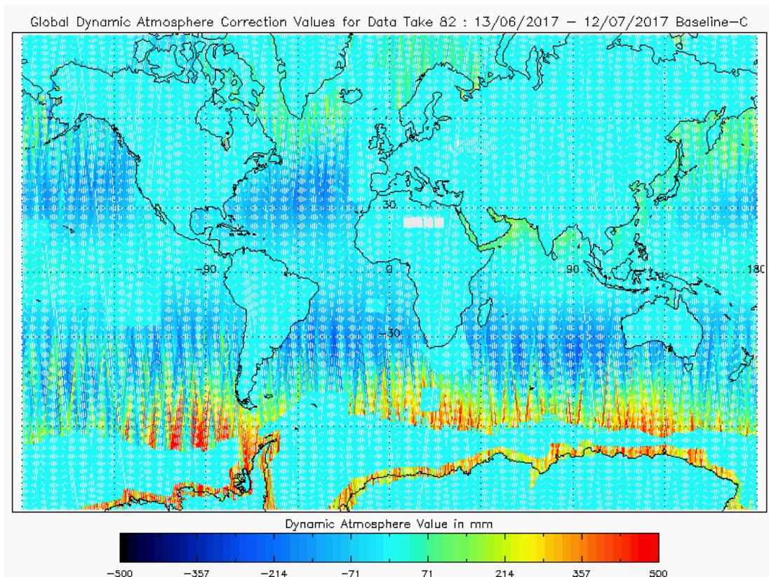
Figure 22 - Global plot of Dynamic Atmospheric Correction for cycle #82
