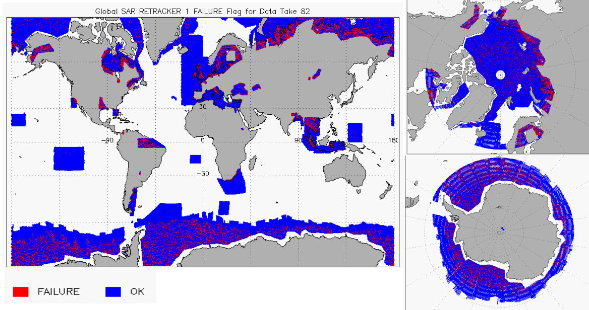
Figure 10 – Global plots showing Retracker Failure Flags for SAR mode for cycle #82
