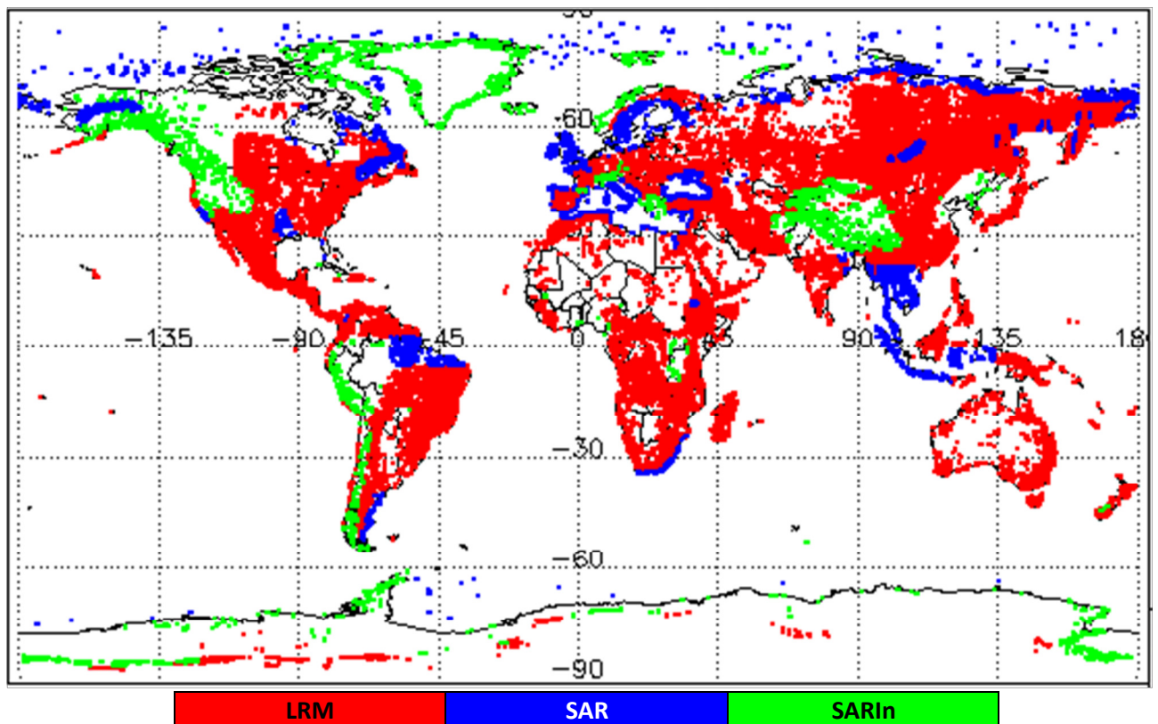
Figure 1 - Global plot showing areas of loss of track in all SIRAL modes L0 data during June 2016.
