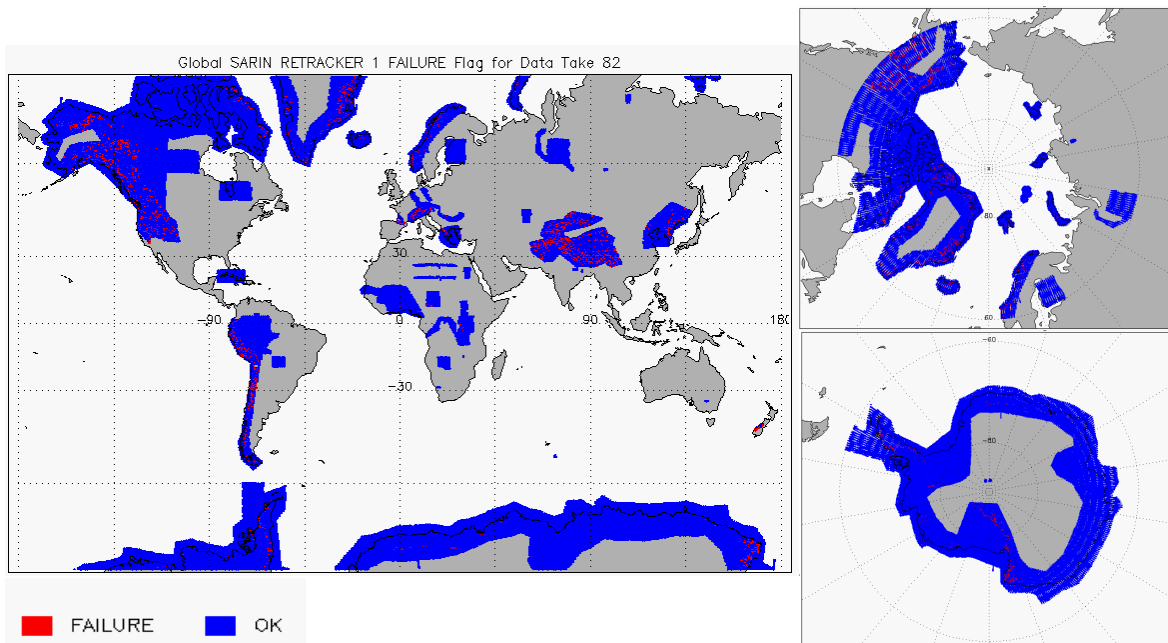
Figure 11 – Global plots showing Retracker Failure Flags for SARIn mode for cycle #82
