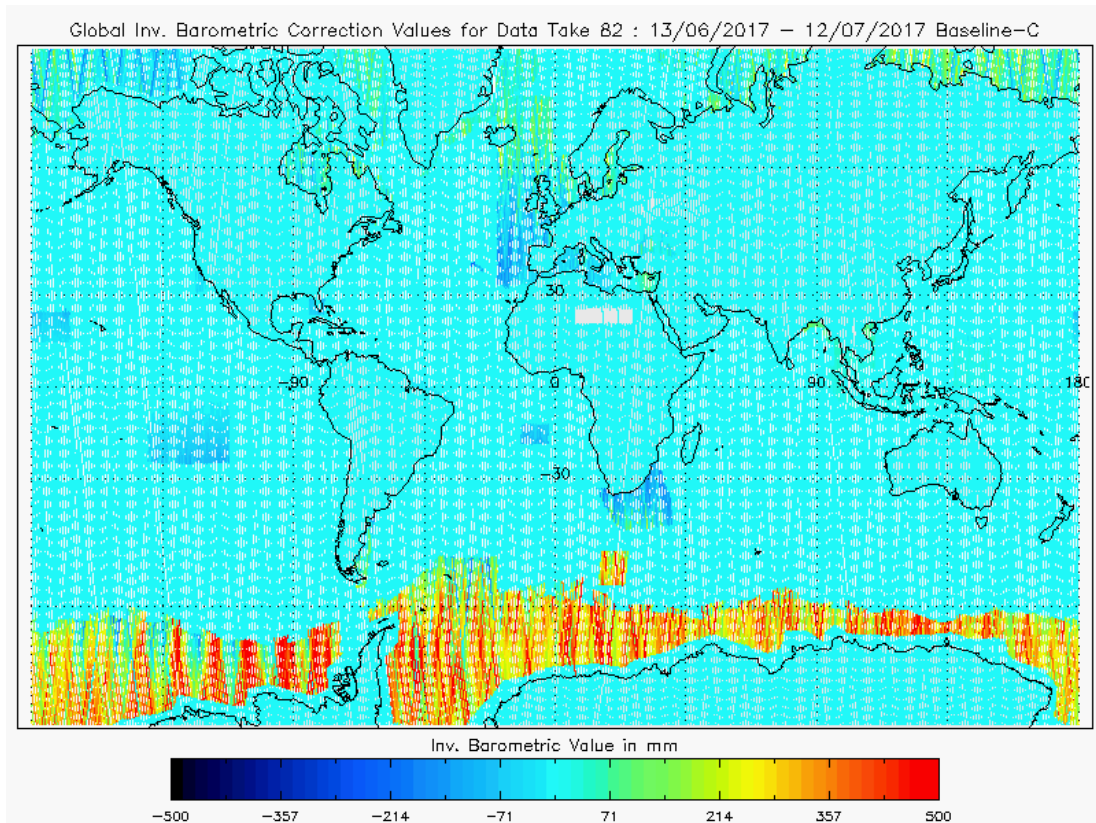
Figure 20 - Global plot of Inverse Barometric Correction for cycle #82
