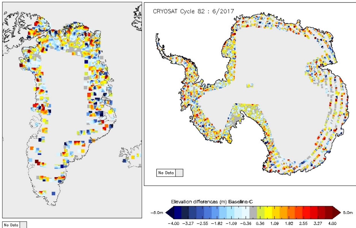
Figure 15 - Greenland and Antarctica maps of SARIn elevation differences for cycle #82
