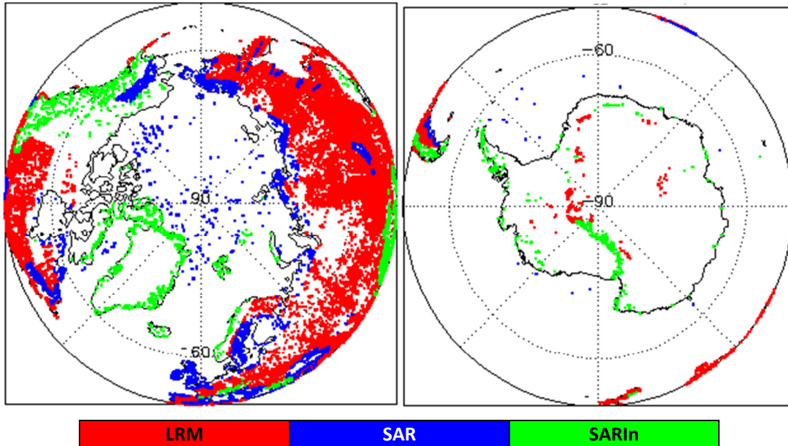
Figure 2 - Polar plots showing areas of loss of track in all SIRAL modes L0 data during June 2016.
