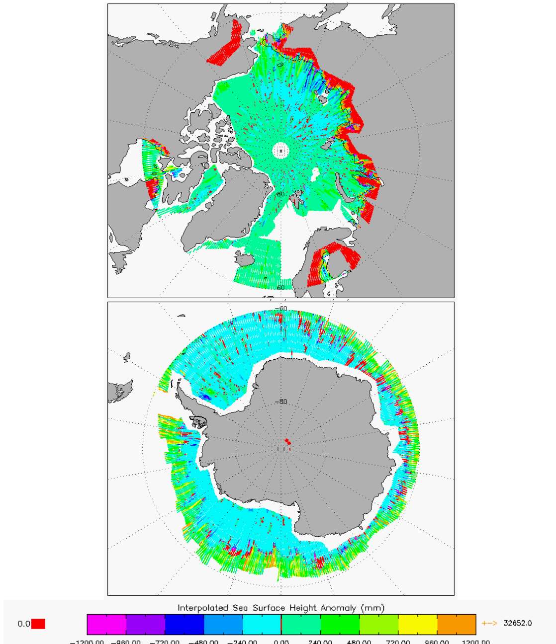
Figure 7 –Polar plots of SSHA for cycle #82
