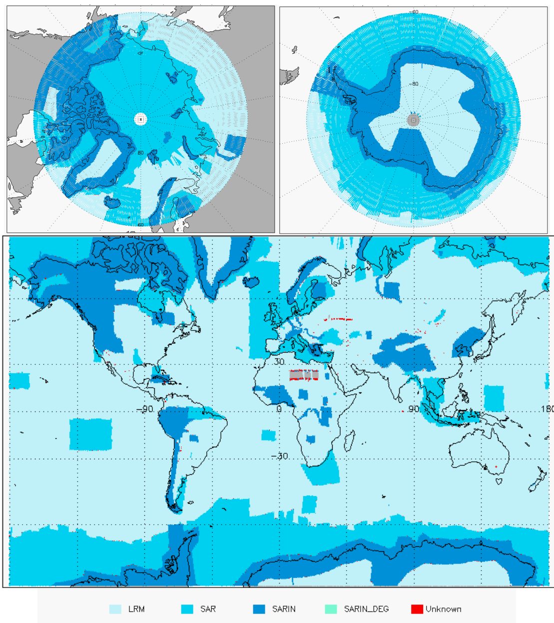
Figure 3 - Global and Polar plots of SIRAL Modes for cycle #82.
