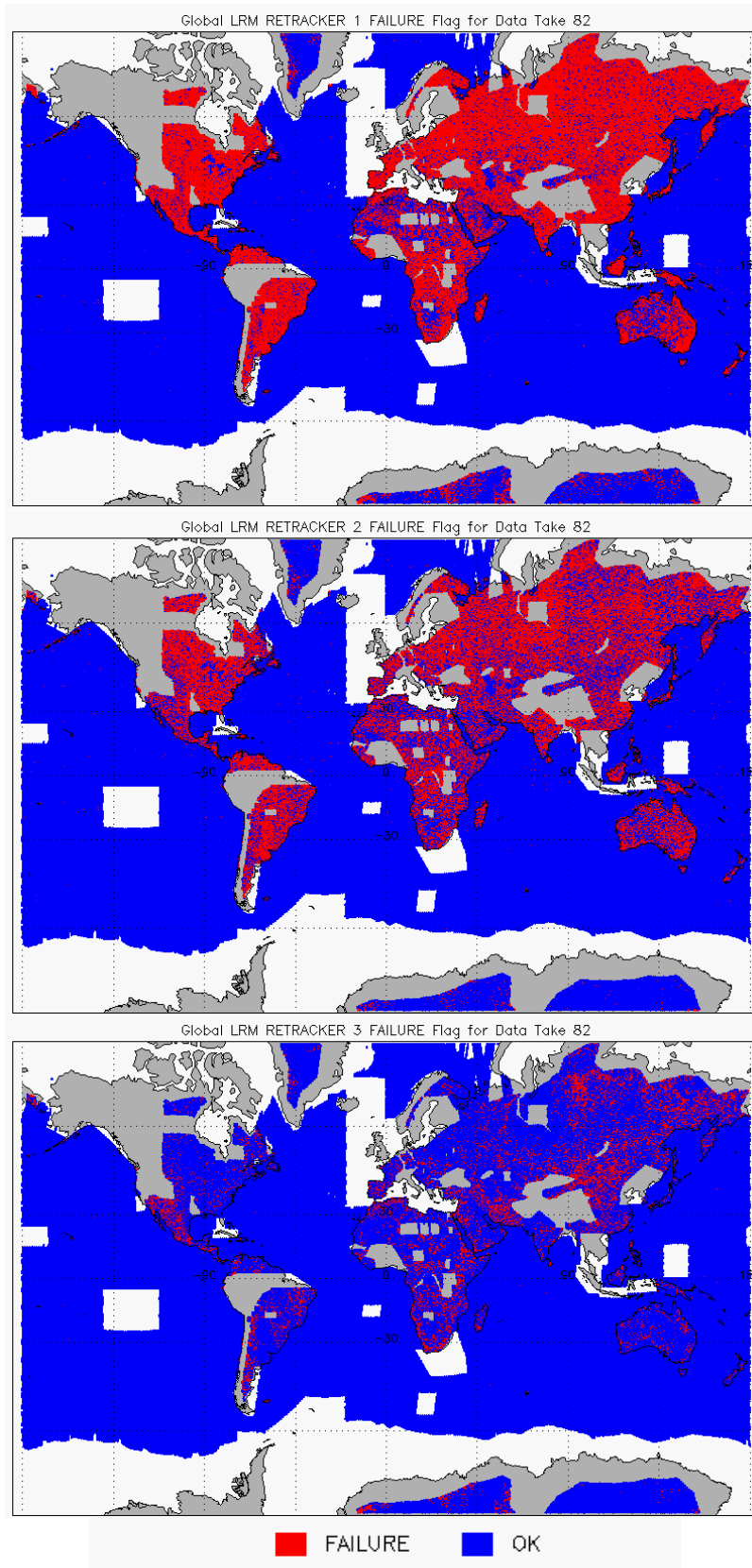
Figure 9 – Global plots showing Retracker Failure Flags for LRM mode for cycle #82: LRM CFI (top), LRM LIRT (middle), LRM OCOG (bottom)
