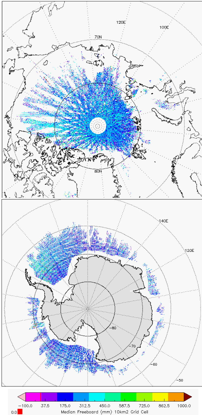
Figure 6 - Polar plots of 10km Gridded Freeboard values from L2 SAR products in cycle #82.
