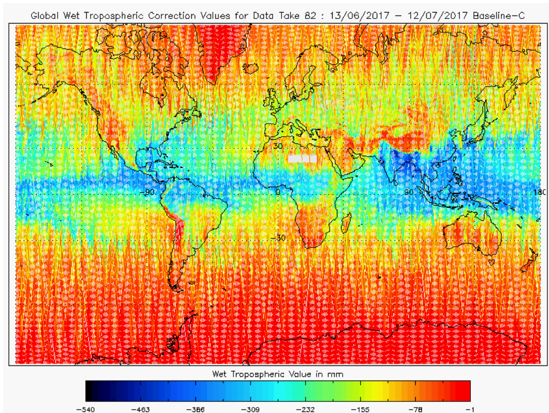
Figure 18 - Global plot of Wet Tropospheric Correction for cycle #82
