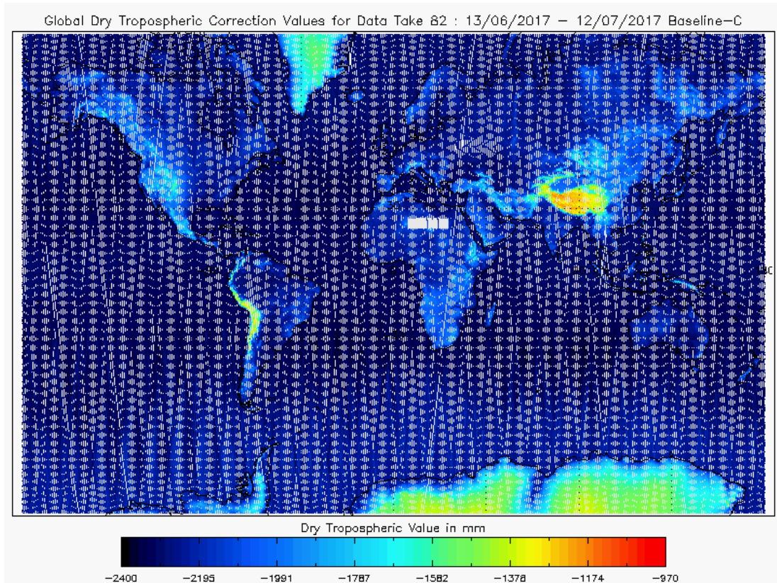
Figure 16 - Global plot of Dry Tropospheric Correction for cycle #82
