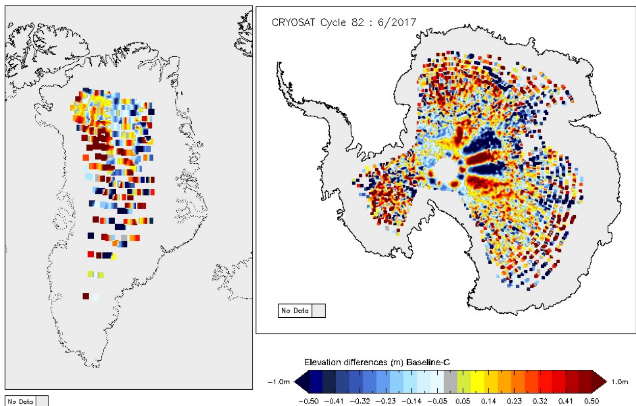
Figure 14 - Greenland and Antarctica maps of LRM elevation differences for cycle #82
