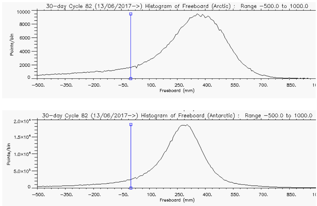
Figure 5 – Histogram of Freeboard for Arctic (above) and Antarctic (below) for cycle #82
