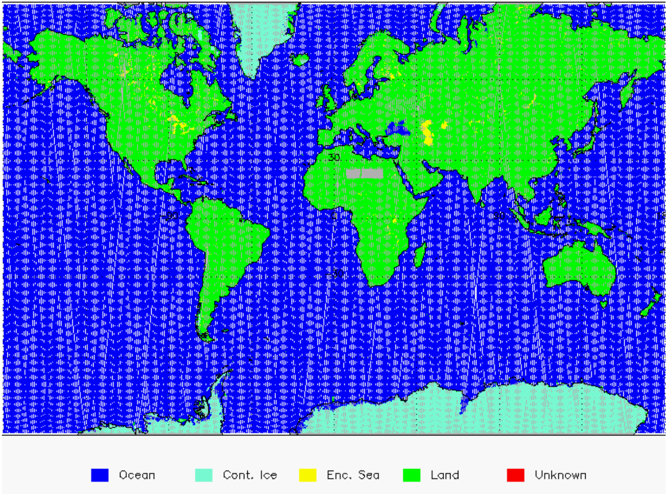
Figure 5-3 Global plot of Surface Type for cycle 11.
