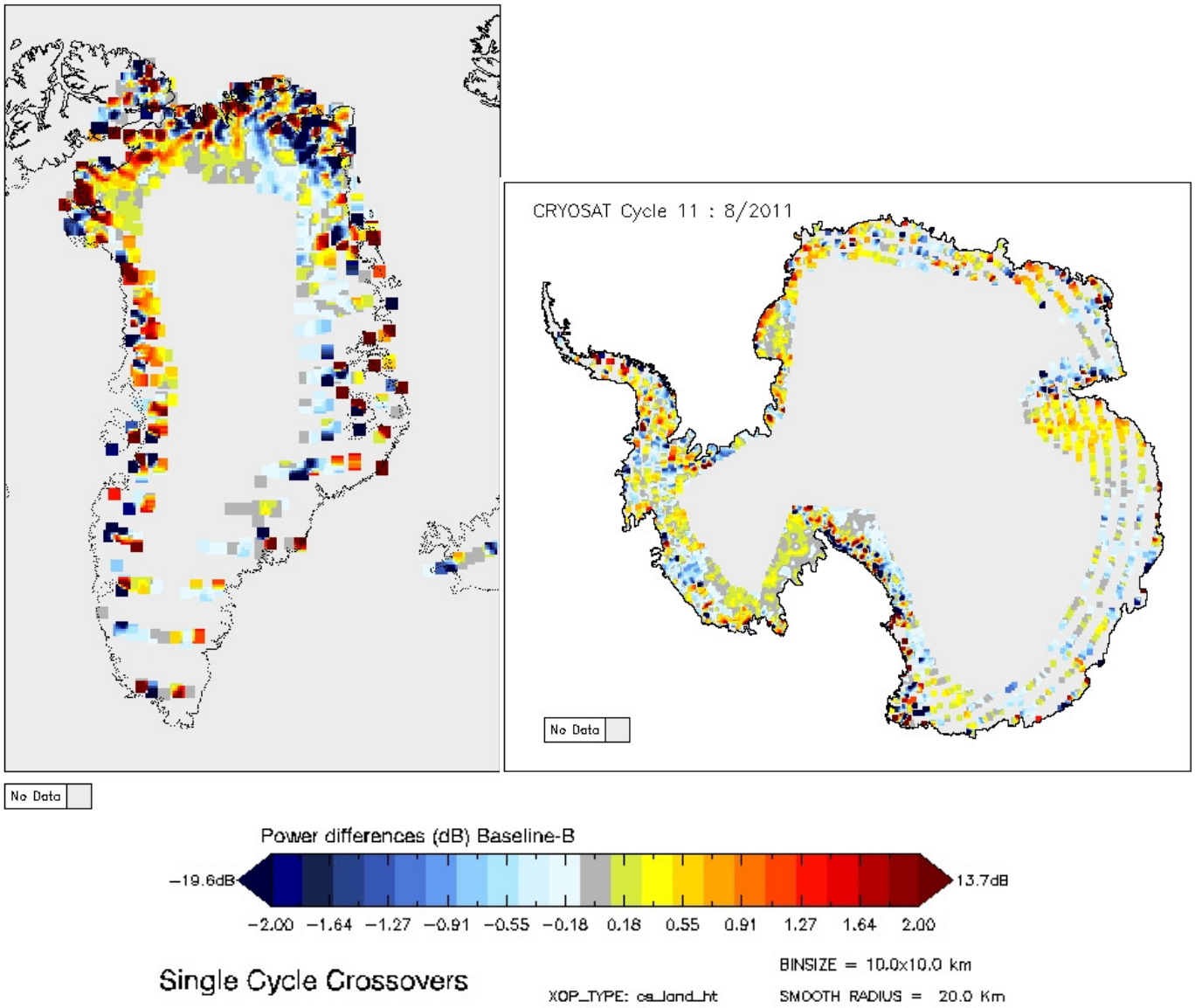
Figure 5-19 Greenland and Antarctica maps of SARIn power differences for cycle 11.
