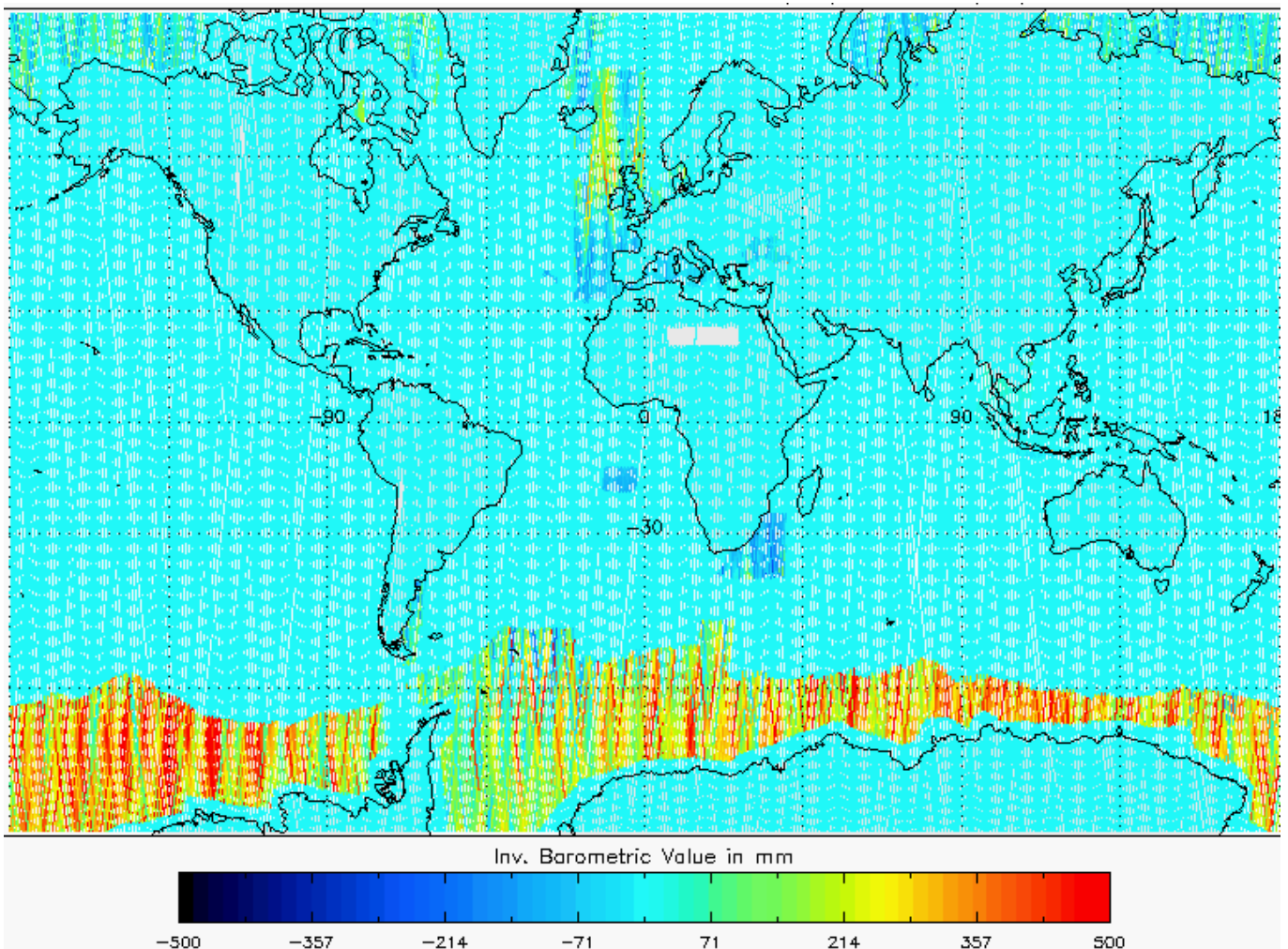
Figure 5-22 Global plot of Inverse Barometric Correction for cycle 11.
