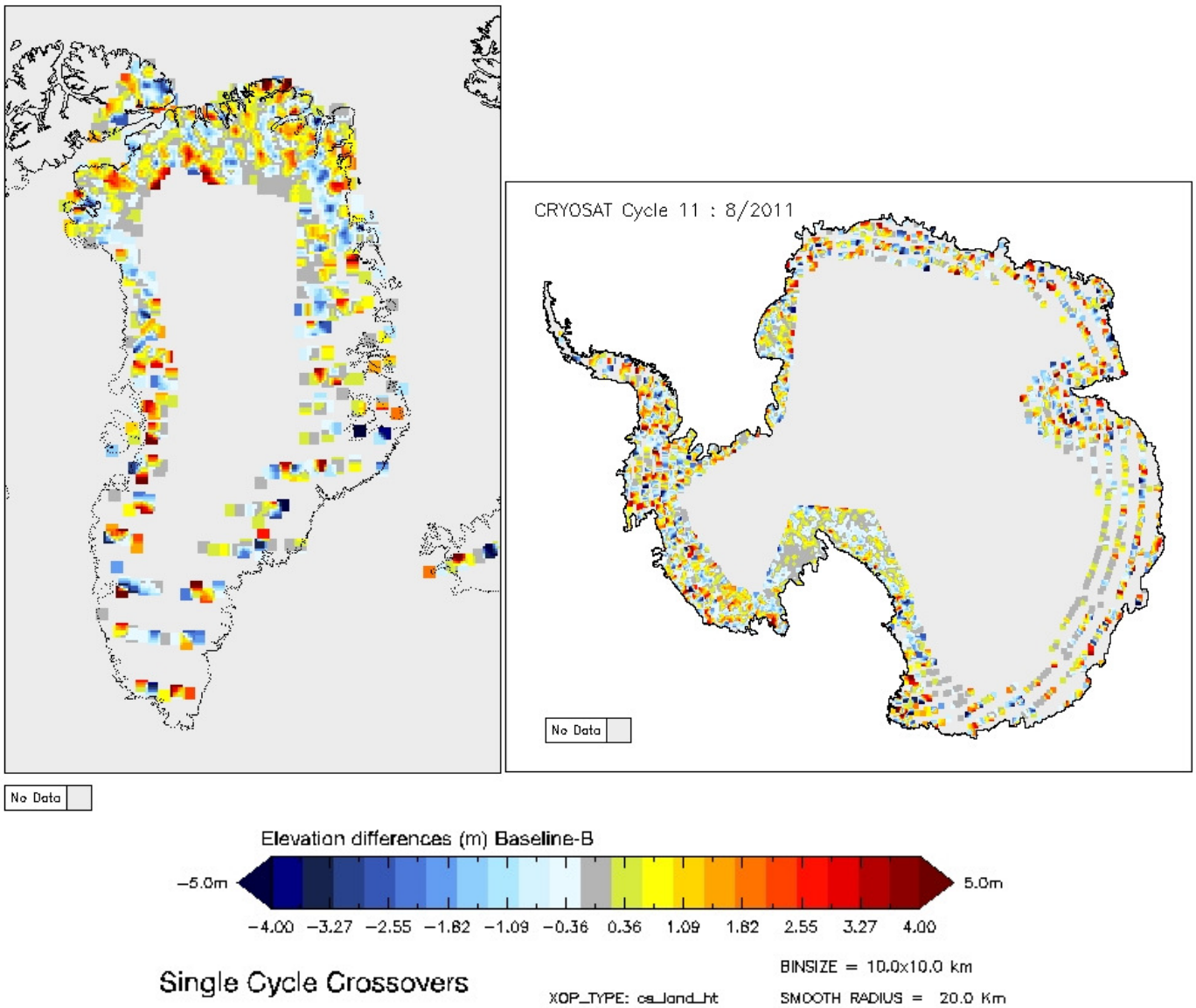
Figure 5-17 Greenland and Antarctica maps of SARIn elevation differences for cycle 11.
