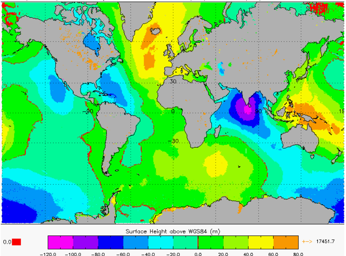
Figure 5-15 Global plots of Sea Surface Height over ocean areas only, for cycle 11.
