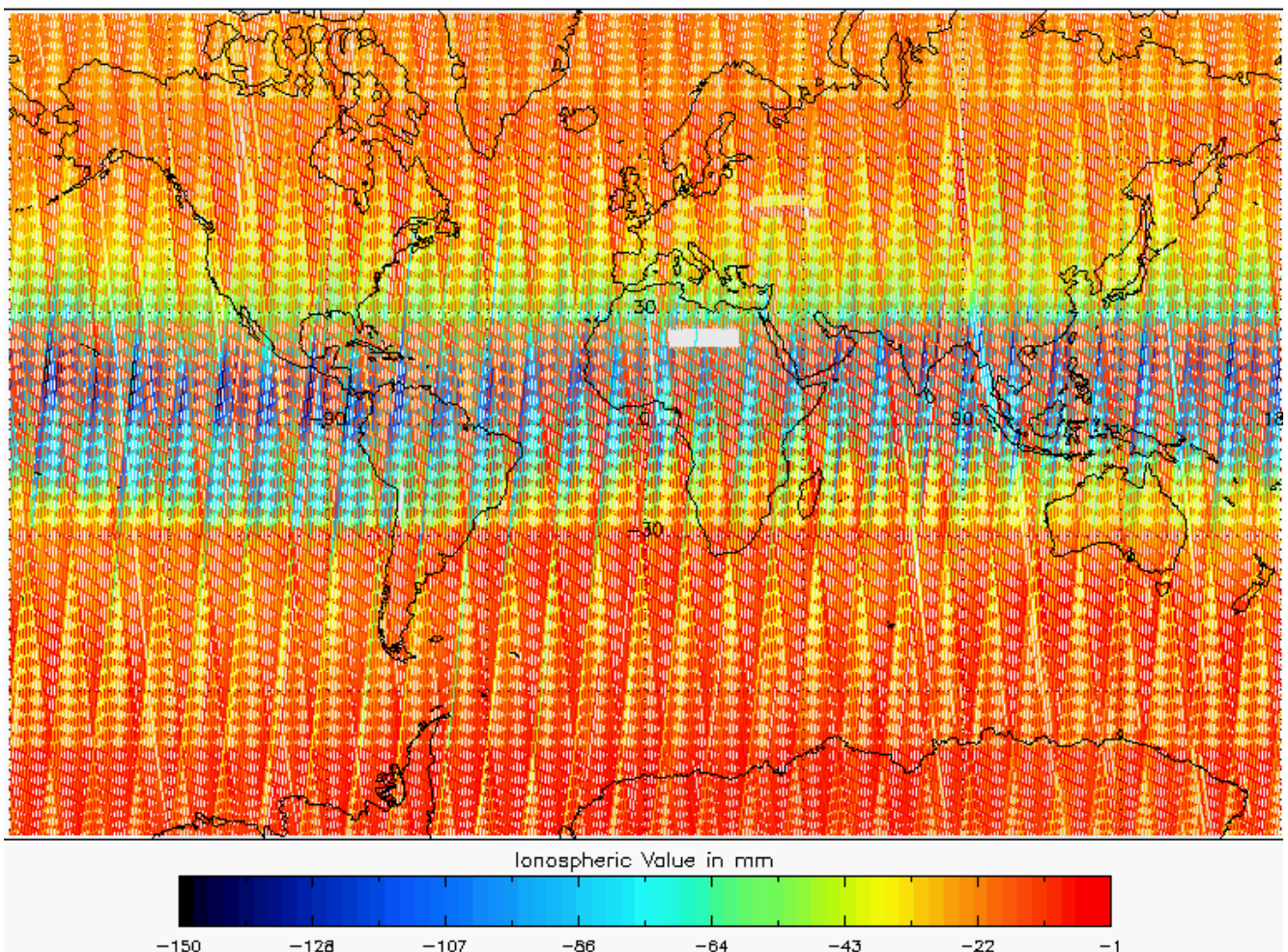
Figure 5-24 Global plot of Ionospheric Correction for cycle 11.
