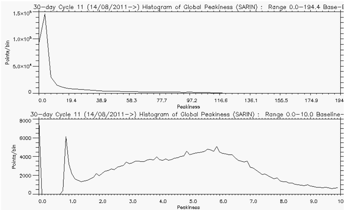
Figure 5-10 Histogram of global Peakiness for SARIn, for cycle 11.
