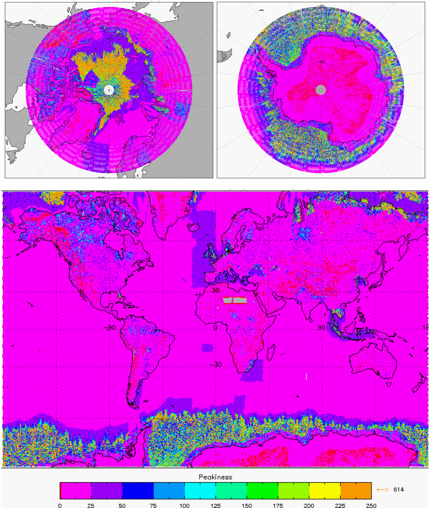
Figure 5-11 Global and Polar plots of Waveform Peakiness for cycle 11.
