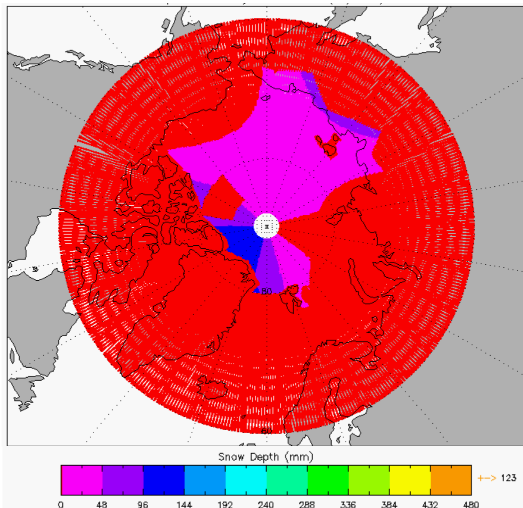
Figure 5-12 Arctic plot of Snow Depth for cycle 11.
