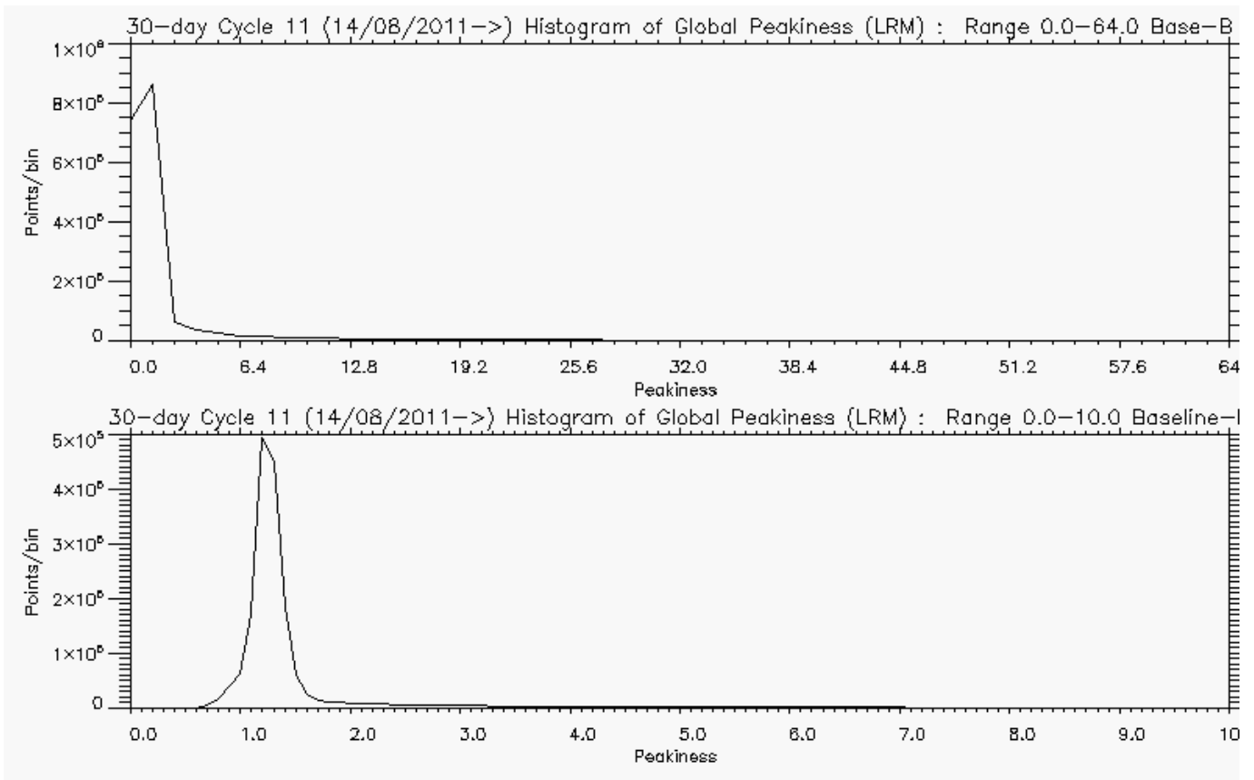
Figure 5-8 Histogram of global Peakiness for LRM, for cycle 11.
