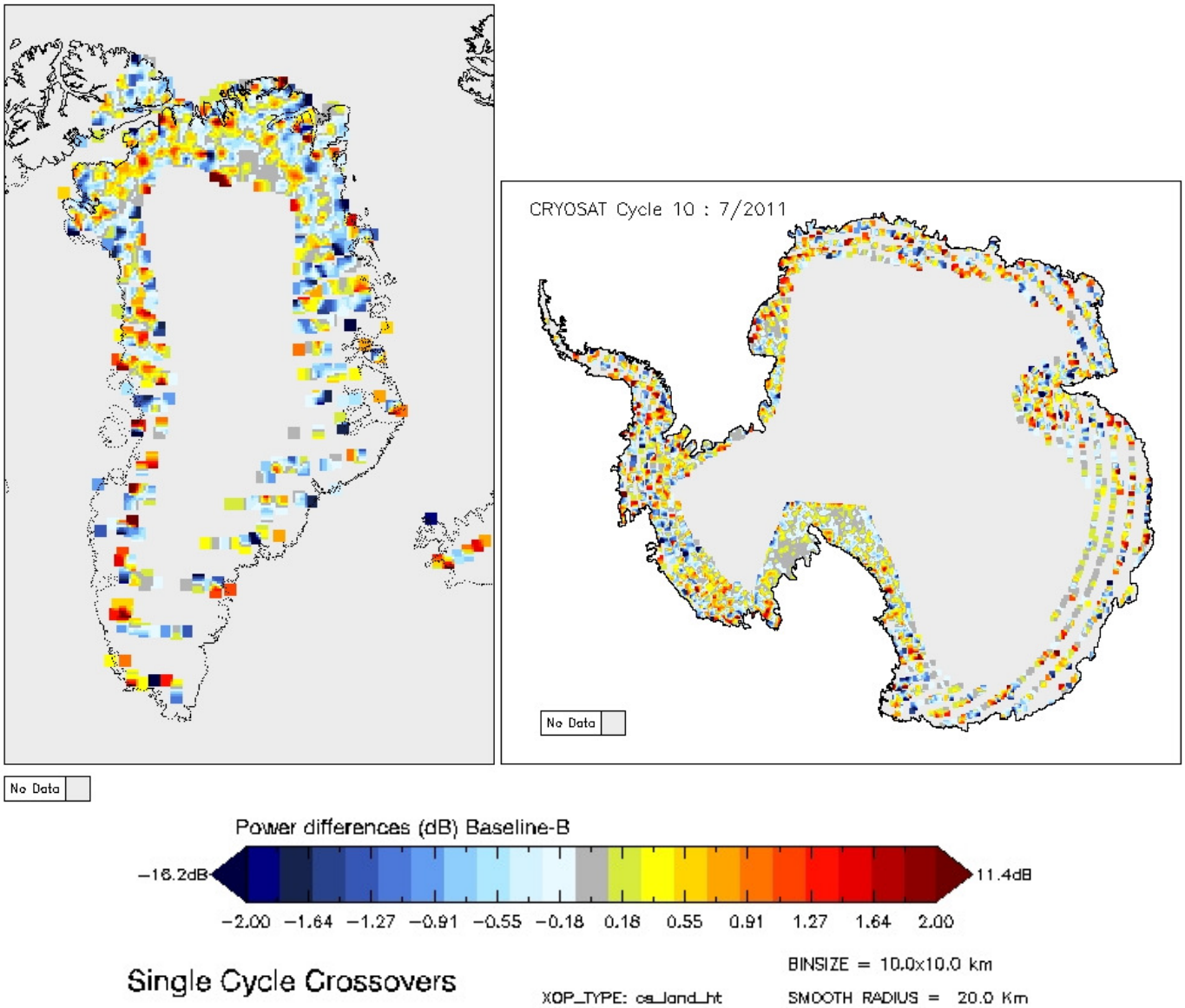
Figure 5-17 Greenland and Antarctica maps of SARIn elevation differences for cycle 10.
