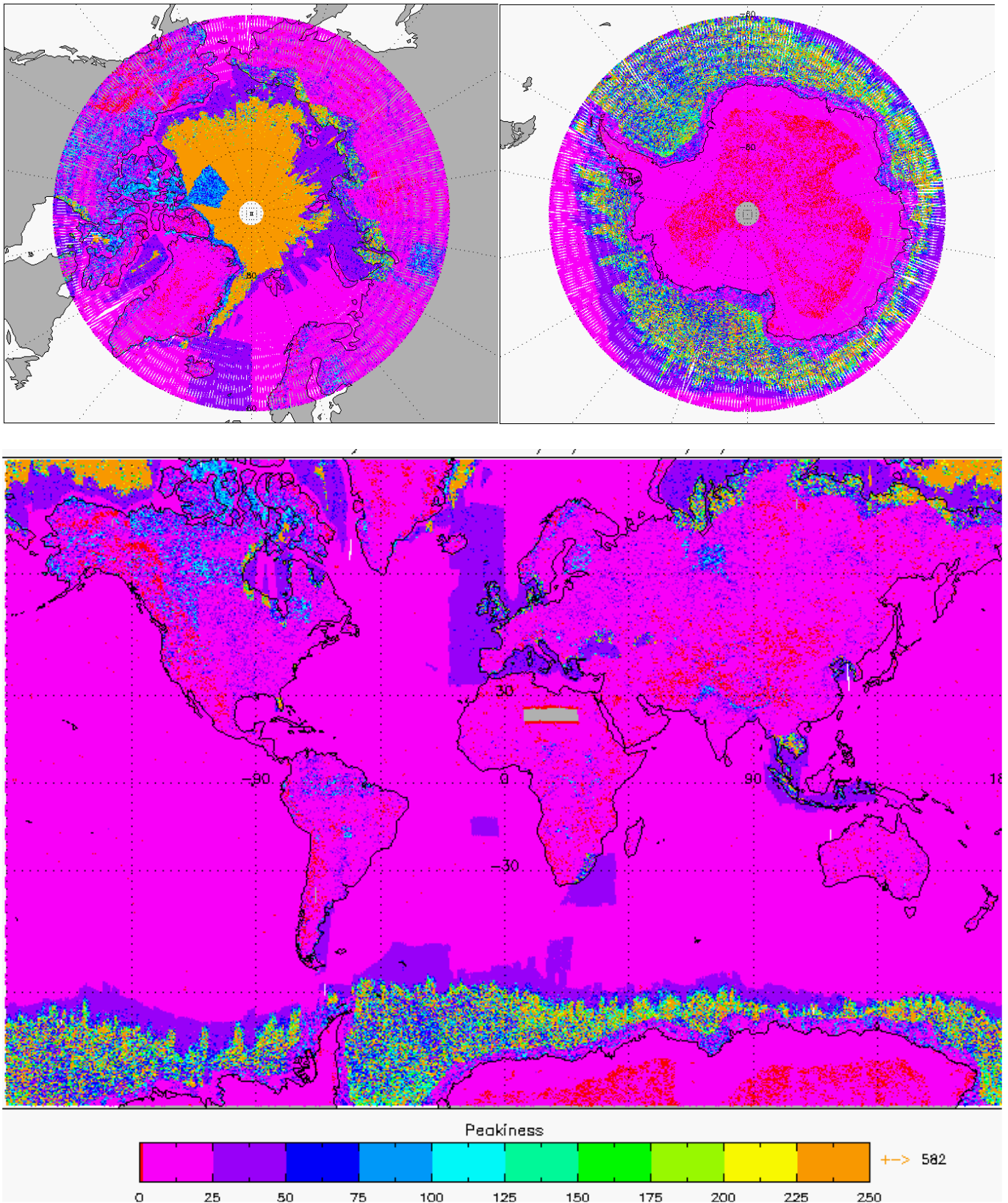
Figure 5-11 Global and Polar plots of Waveform Peakiness for cycle 10.
