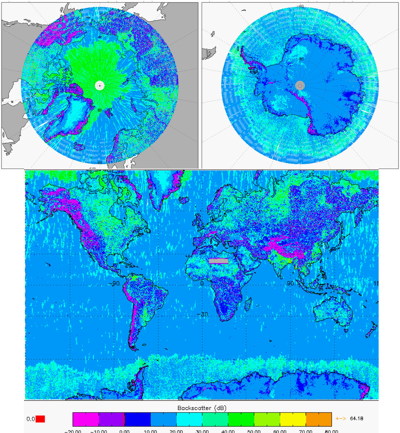
Figure 5-4 Global and Polar plots of Backscatter for cycle 10.
