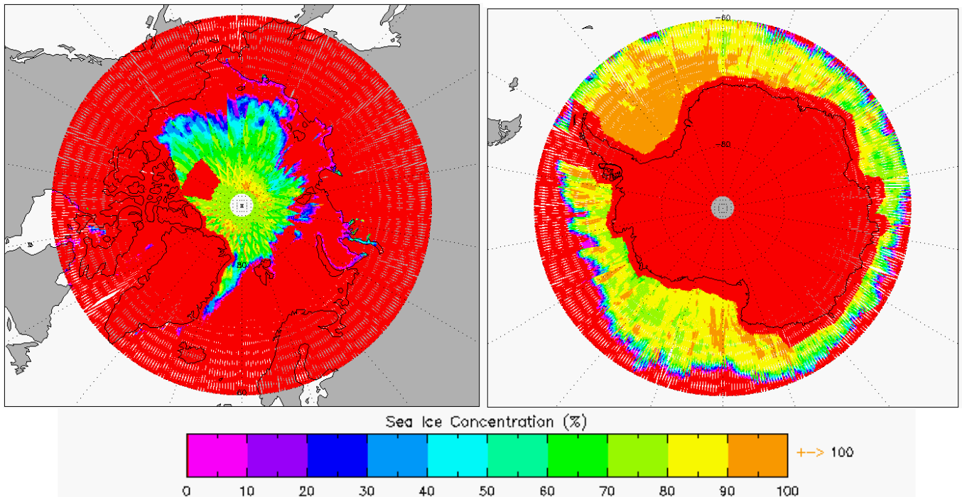
Figure 5-13 Polar plots of Sea Ice Concentration for cycle 10.
