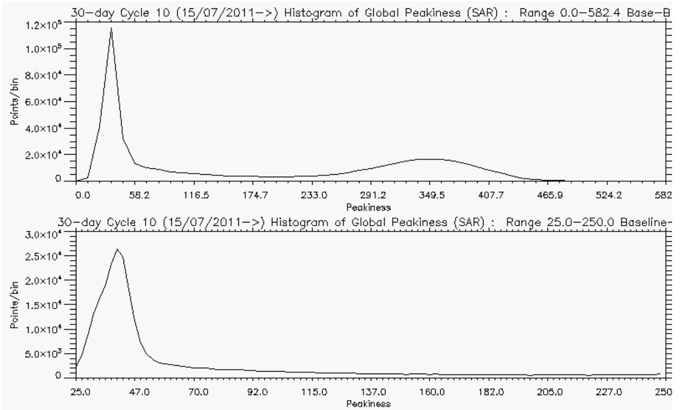
Figure 5-9 Histogram of global Peakiness for SAR, for cycle 10.
