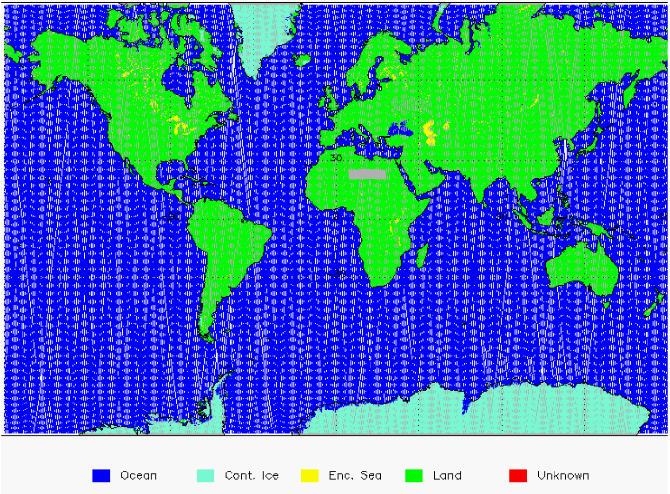
Figure 5-3 Global plot of Surface Type for cycle 10.
