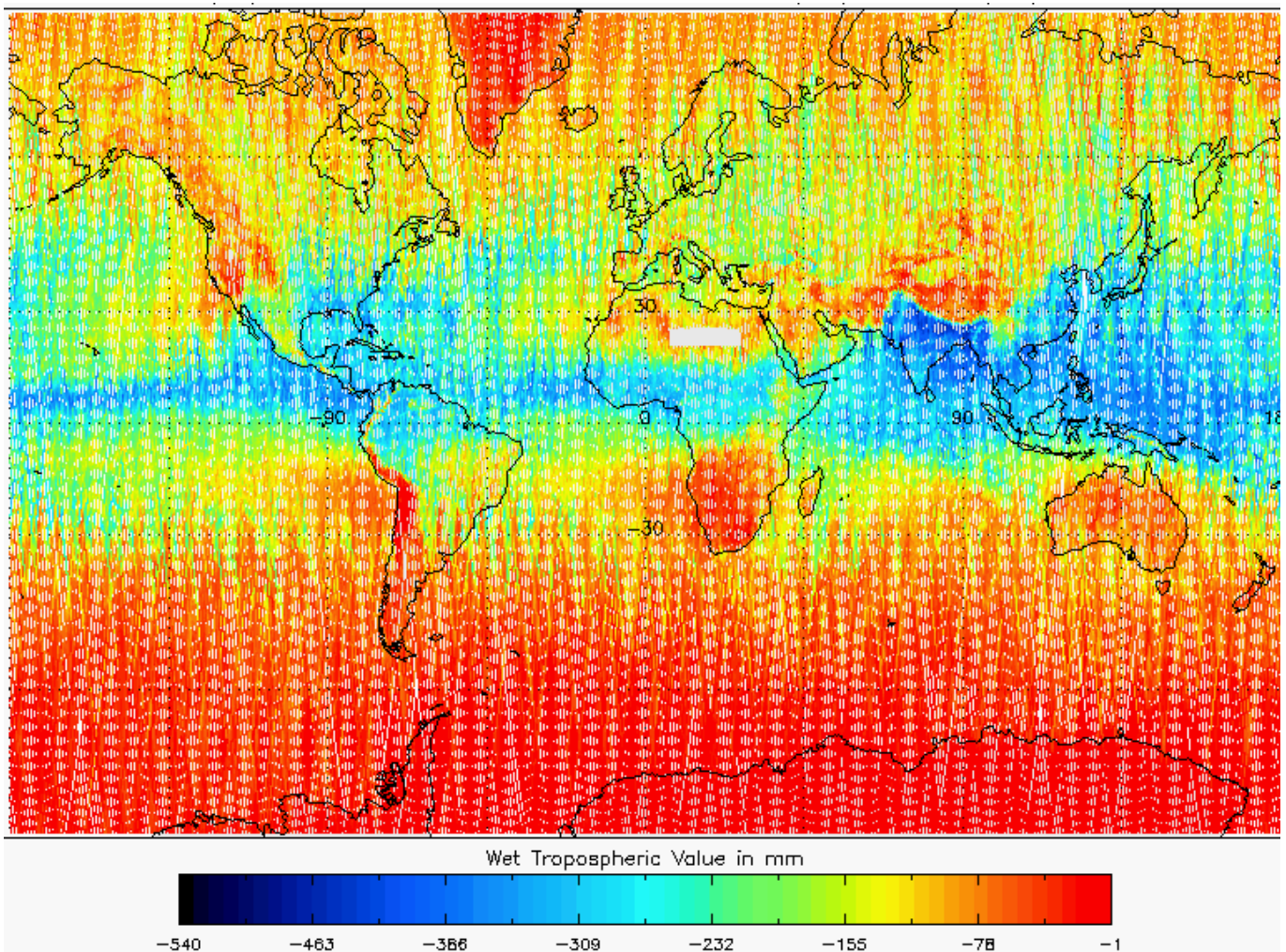
Figure 5-21 Global plot of Wet Tropospheric Correction for cycle 10.
