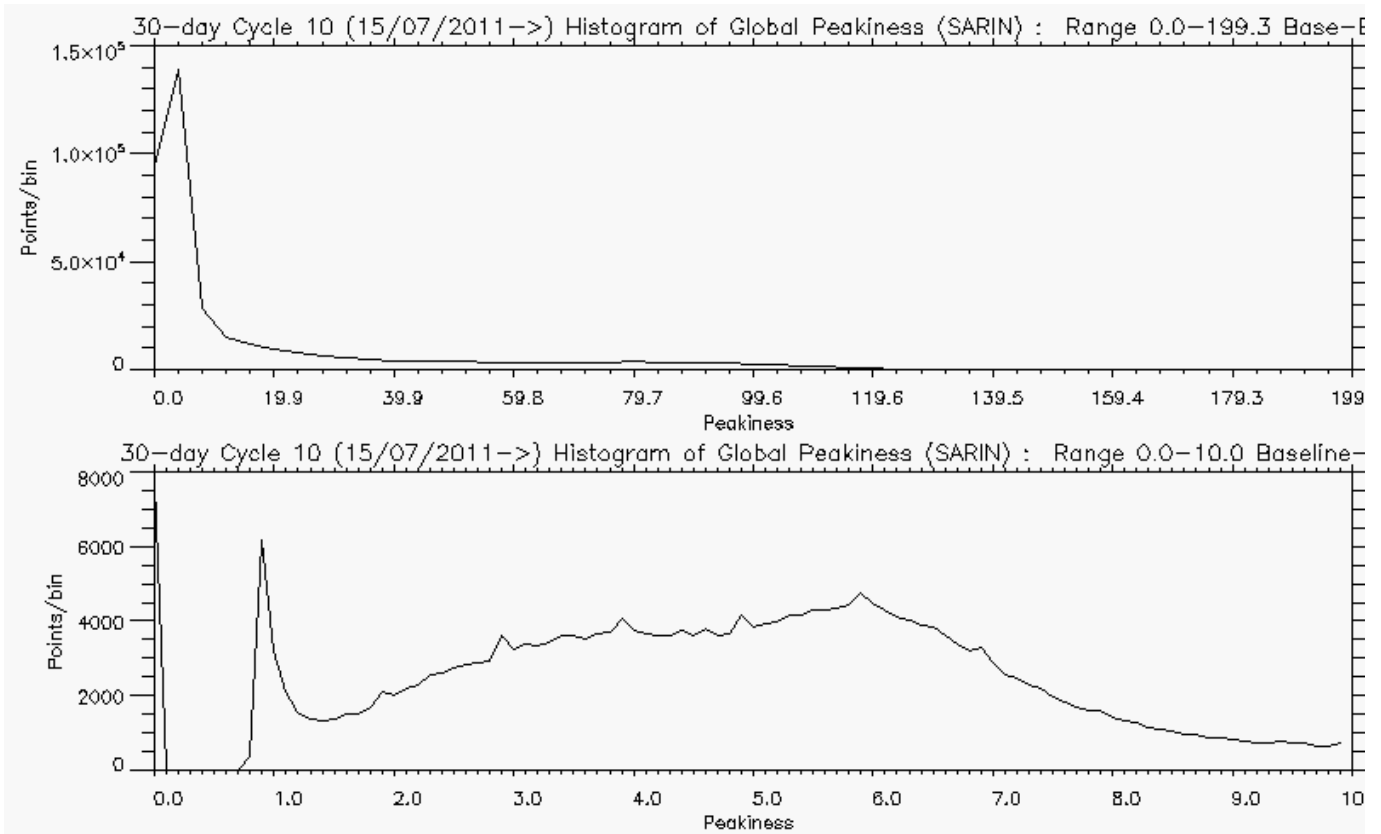
Figure 5-10 Histogram of global Peakiness for SARIn, for cycle 10.
