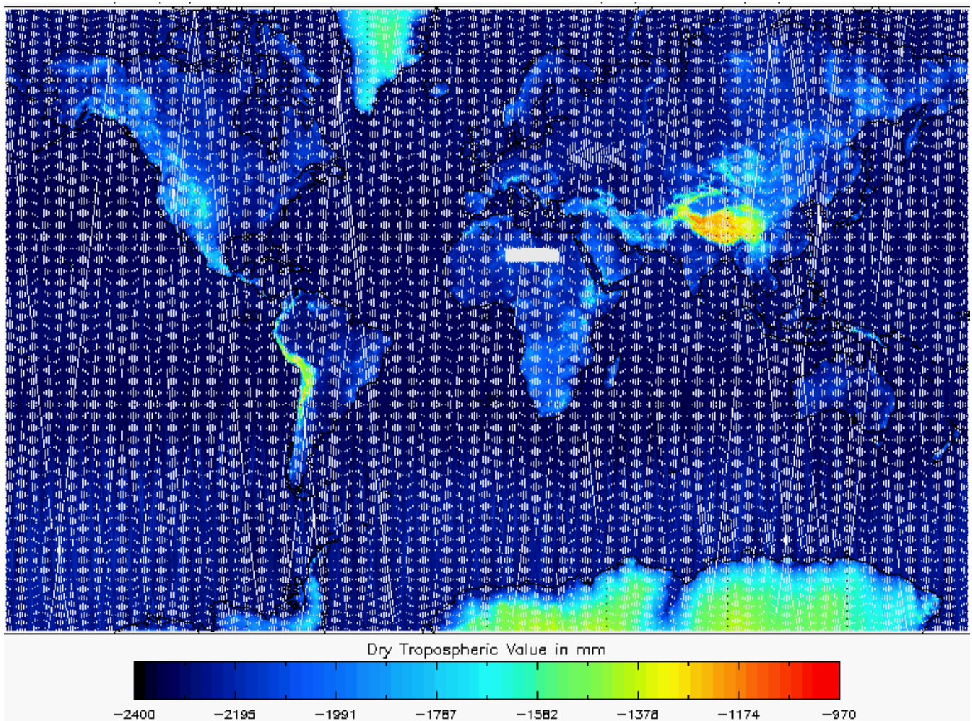
Figure 5-20 Global plot of Dry Tropospheric Correction for cycle 10.
