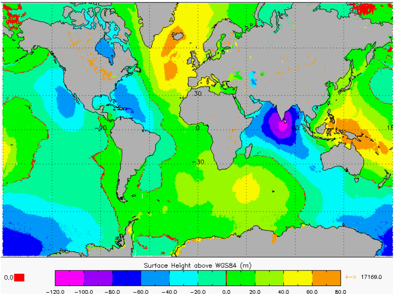
Figure 5-15 Global plots of Sea Surface Height over ocean areas only, for cycle 10.
