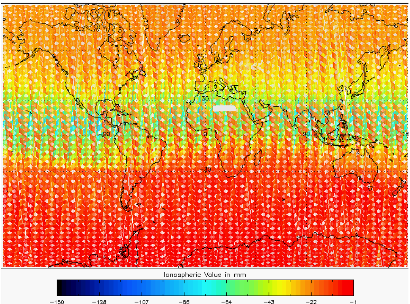
Figure 5-24 Global plot of Ionospheric Correction for cycle 10.
