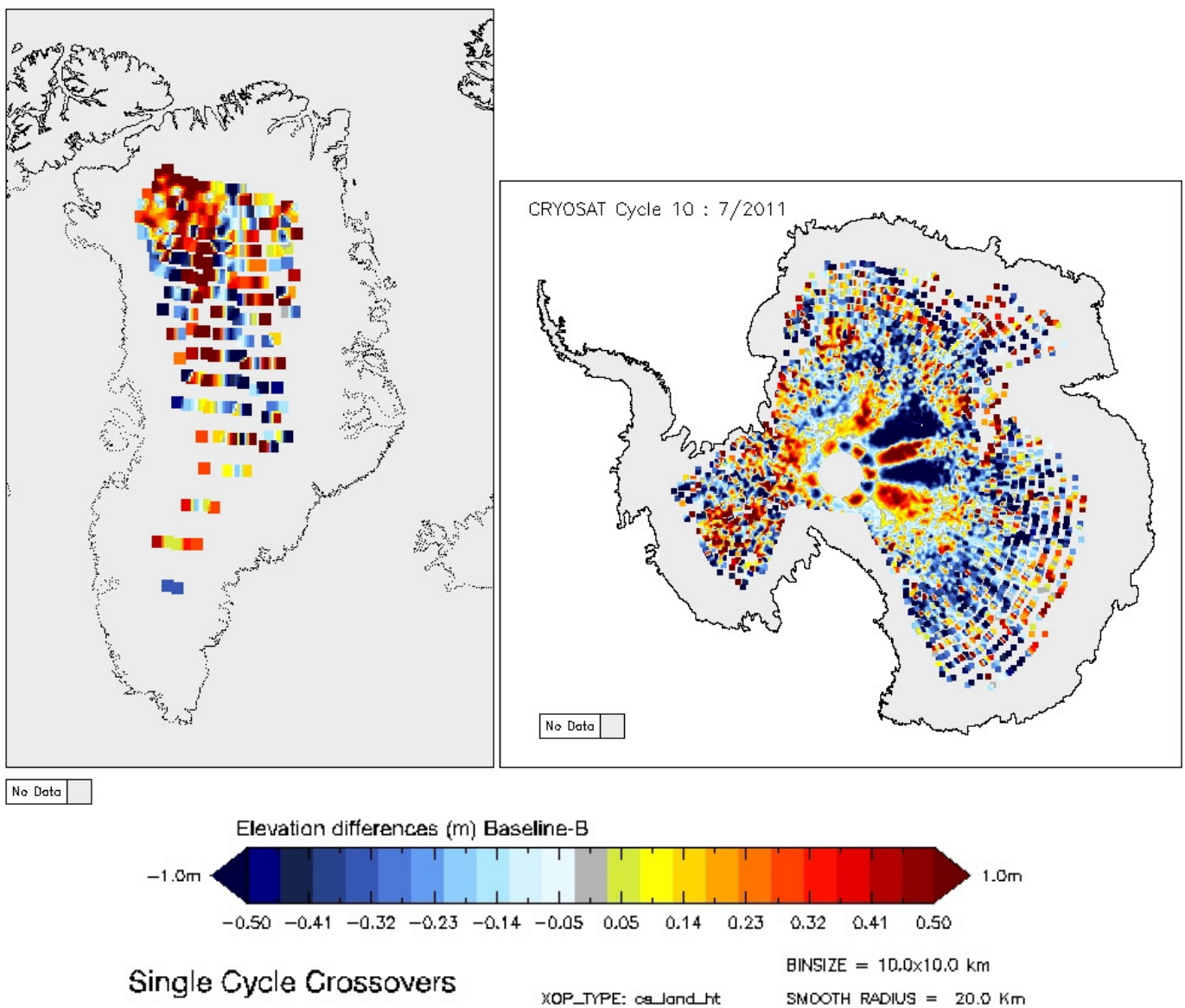
Figure 5-16 Greenland and Antarctica maps of LRM elevation differences for cycle 10.
