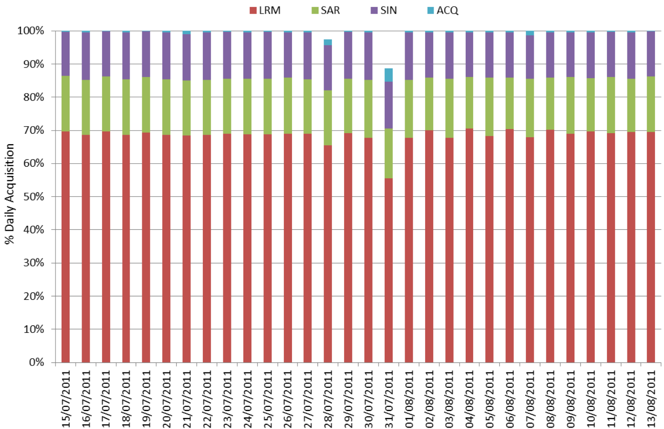
Figure 5-1 Daily percentages of SIRAL modes for cycle 10.
