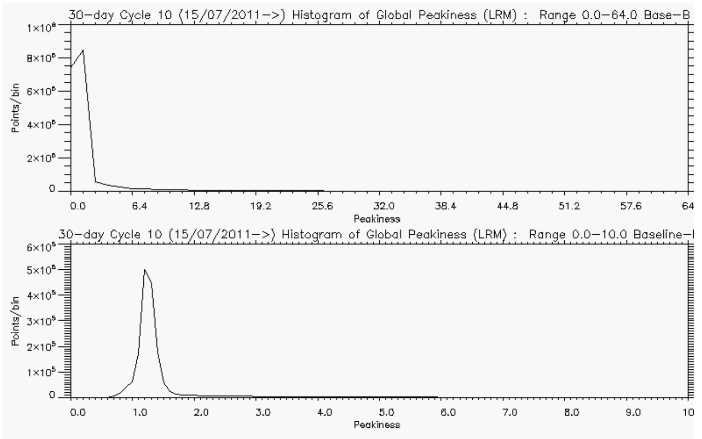
Figure 5-8 Histogram of global Peakiness for LRM, for cycle 10.
