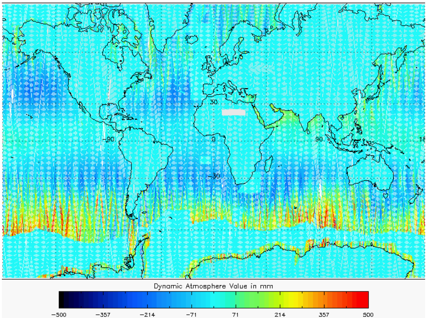
Figure 5-23 Global plot of Dynamic Atmosphere Correction for cycle 10.
