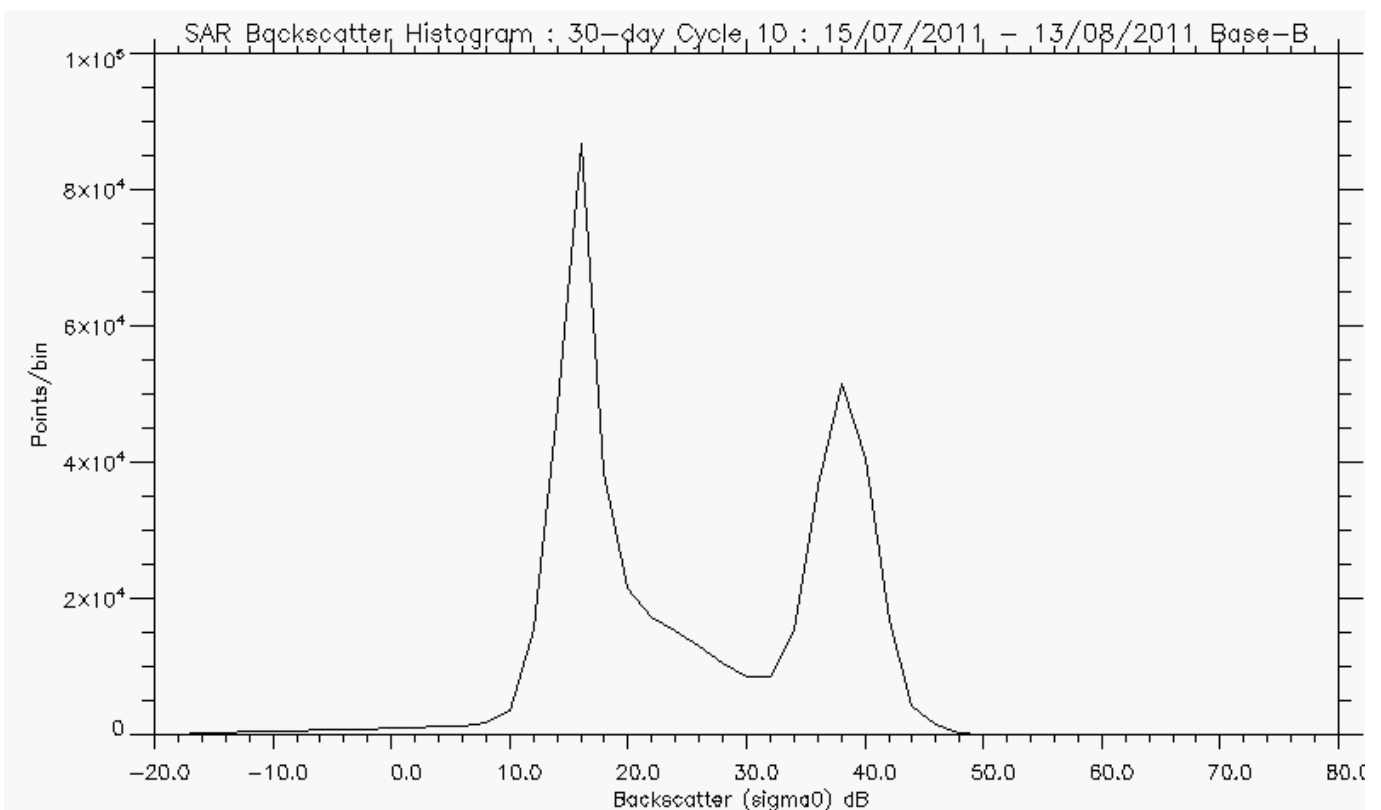
Figure 5-6 Backscatter Histogram for SAR, cycle 10.
