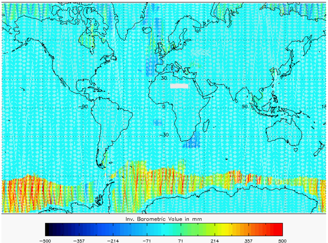
Figure 5-22 Global plot of Inverse Barometric Correction for cycle 10.
