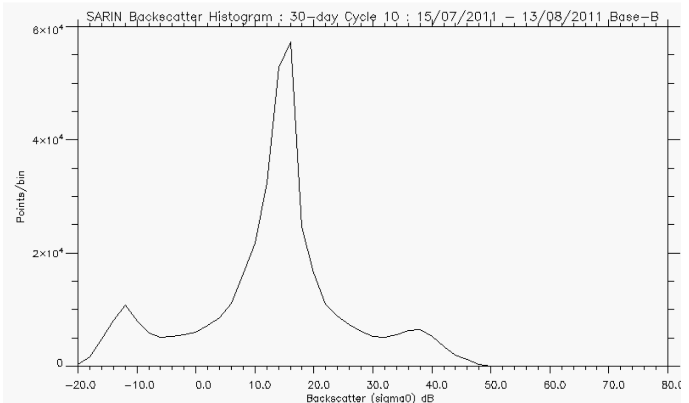
Figure 5-7 Backscatter Histogram for SARIn, cycle 10.
