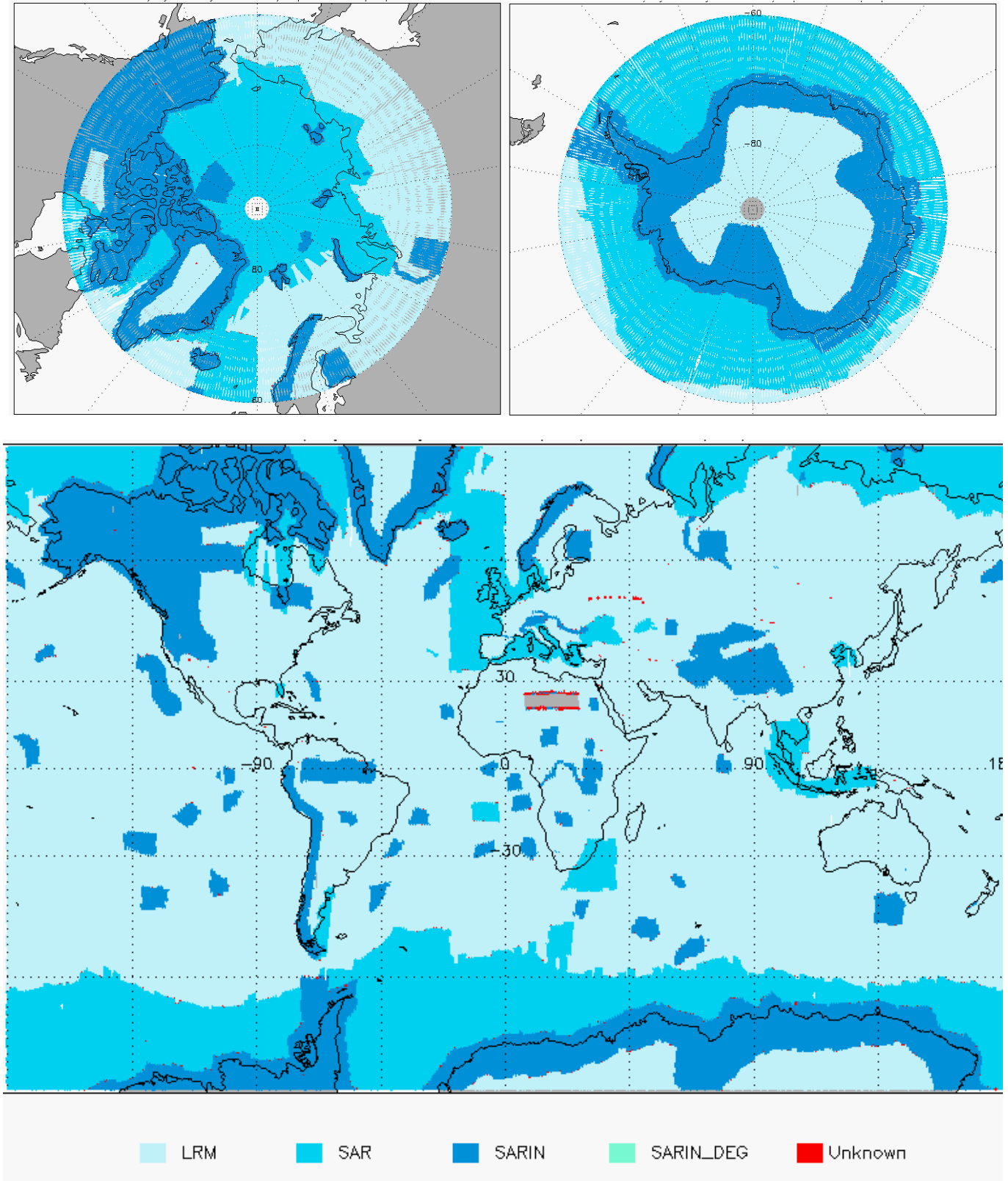
Figure 5-2 Global and Polar plots of SIRAL Modes for cycle 10.
