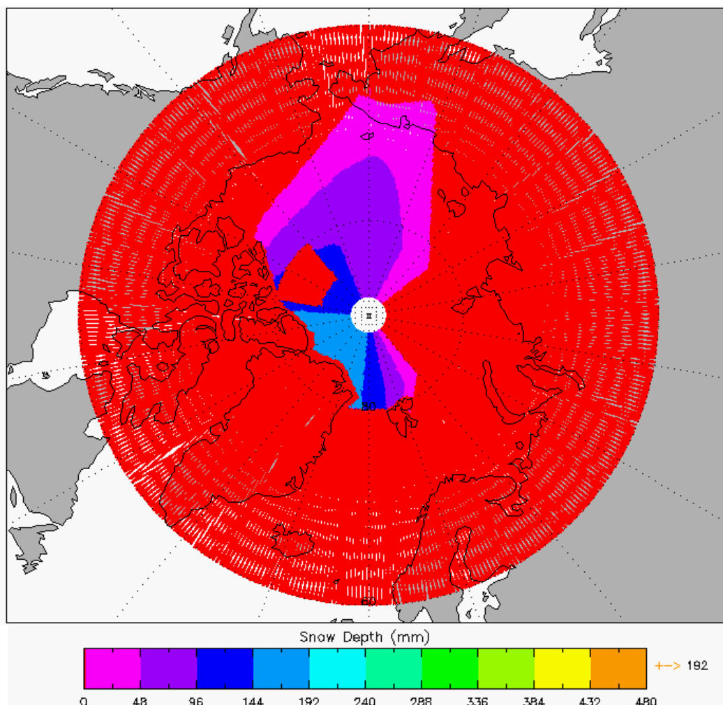
Figure 5-12 Arctic plot of Snow Depth for cycle 10.
