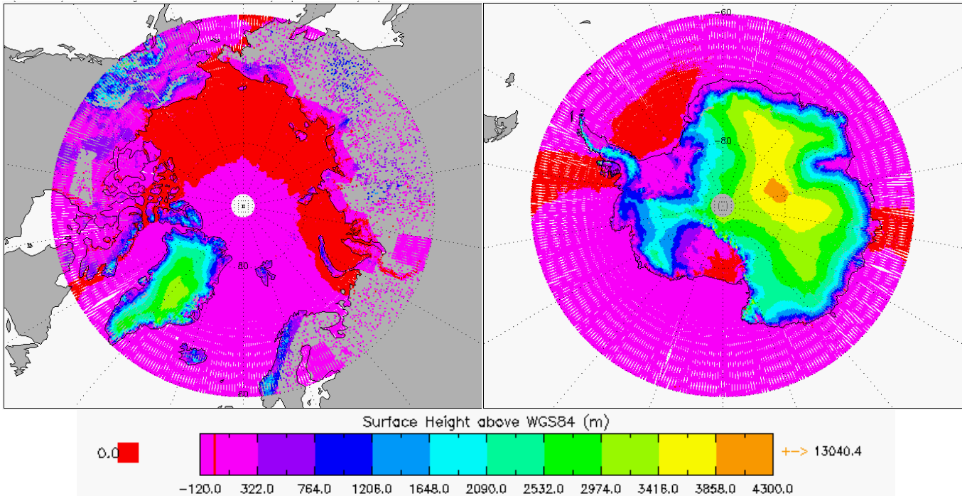
Figure 5-14 Polar plots of Surface Height over land and ocean areas for cycle 10.
