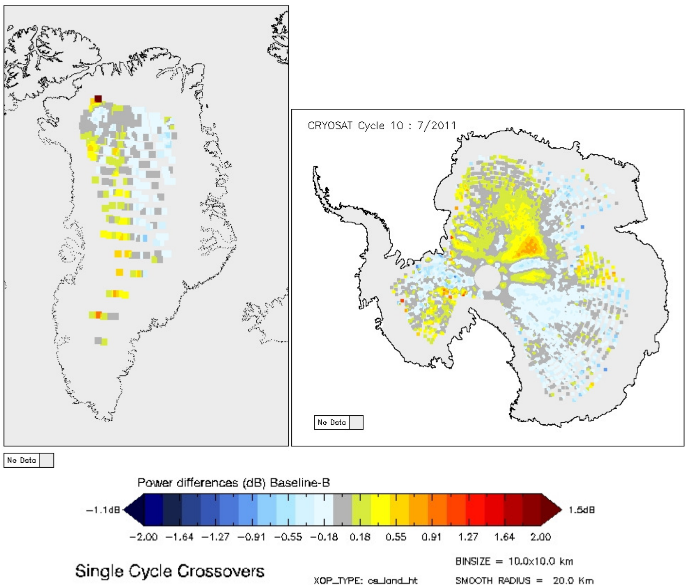
Figure 5-18 Greenland and Antarctica maps of LRM power differences for cycle 10.
