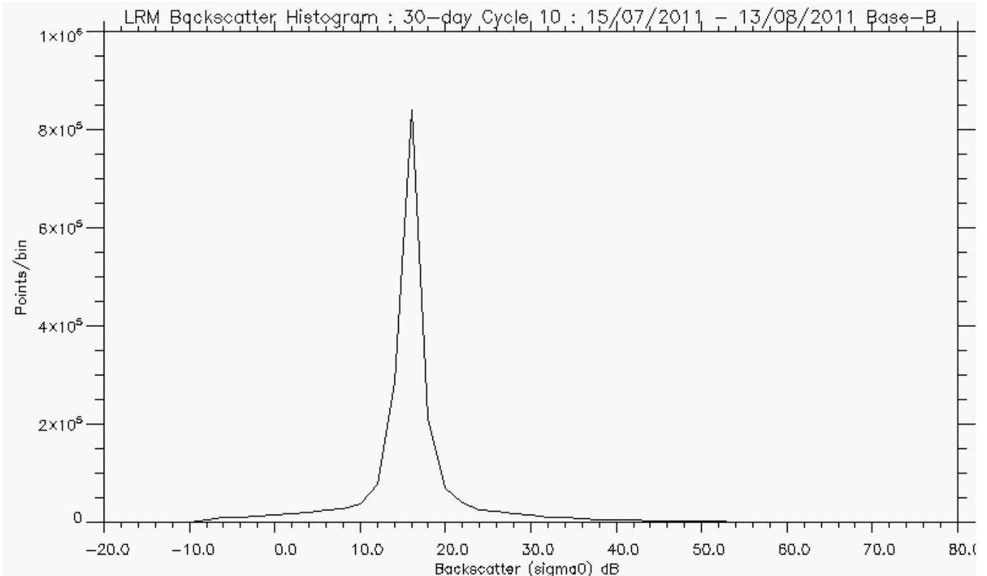
Figure 5-5 Backscatter Histogram for LRM, cycle 10.
