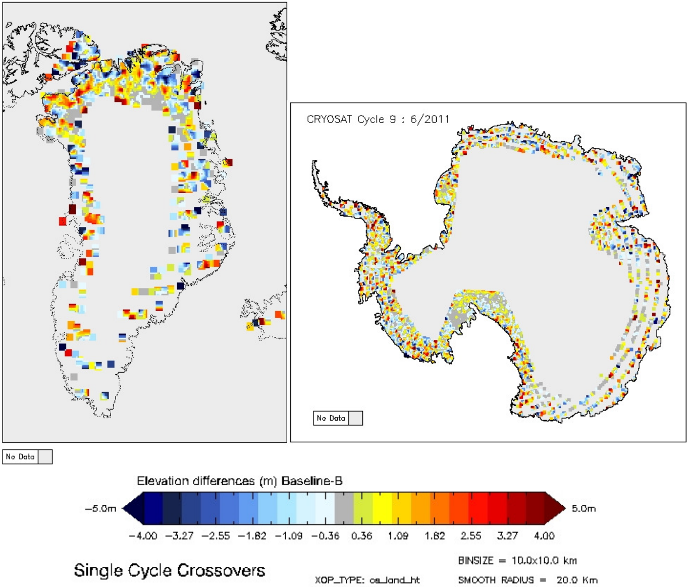
Figure 5-17 Greenland and Antarctica maps of SARIn elevation differences for cycle 9.
