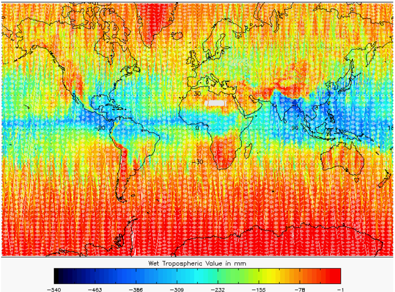
Figure 5-21 Global plot of Wet Tropospheric Correction for cycle 9.
