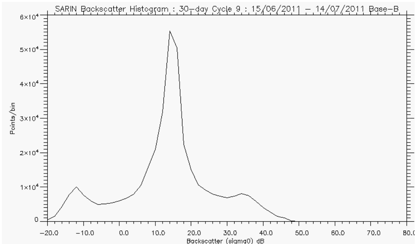
Figure 5-7 Backscatter Histogram for SARin, cycle 9.
