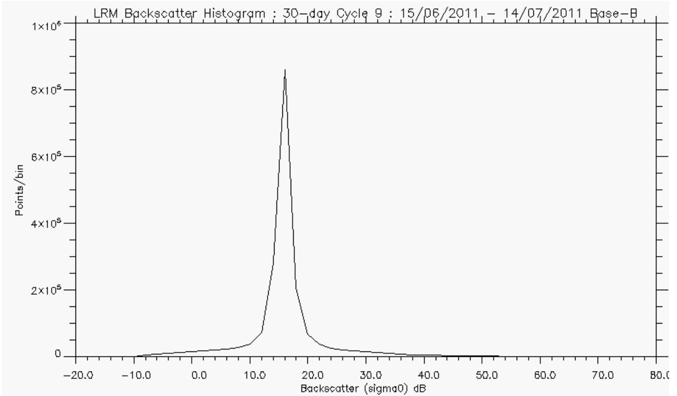
Figure 5-5 Backscatter Histogram for LRM, cycle 9.
