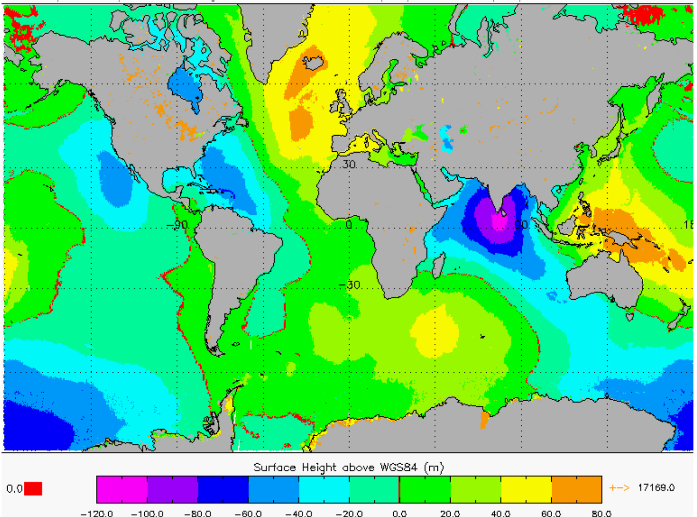
Figure 5-15 Global plots of Sea Surface Height over ocean areas only, for cycle 9.
