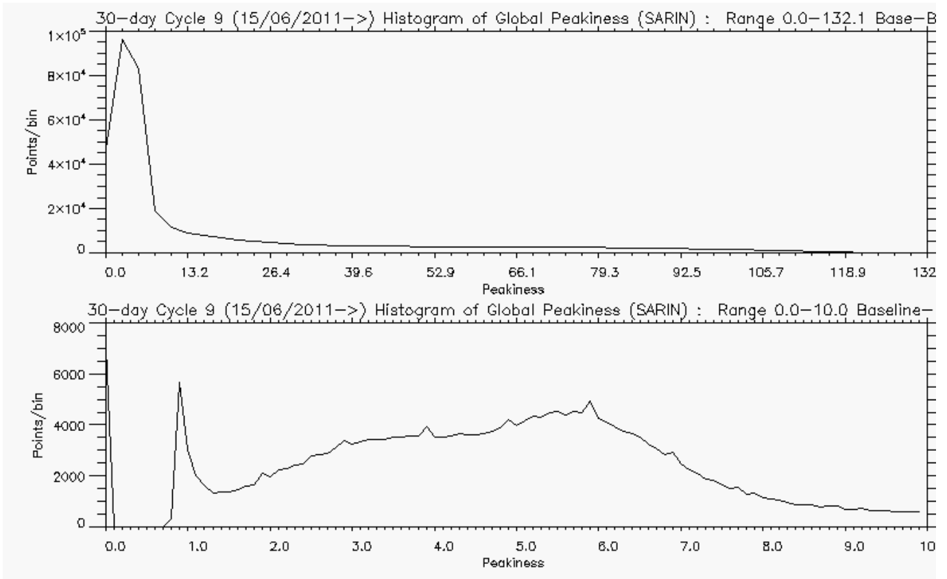
Figure 5-10 Histogram of global Peakiness for SARIn, for cycle 9.
