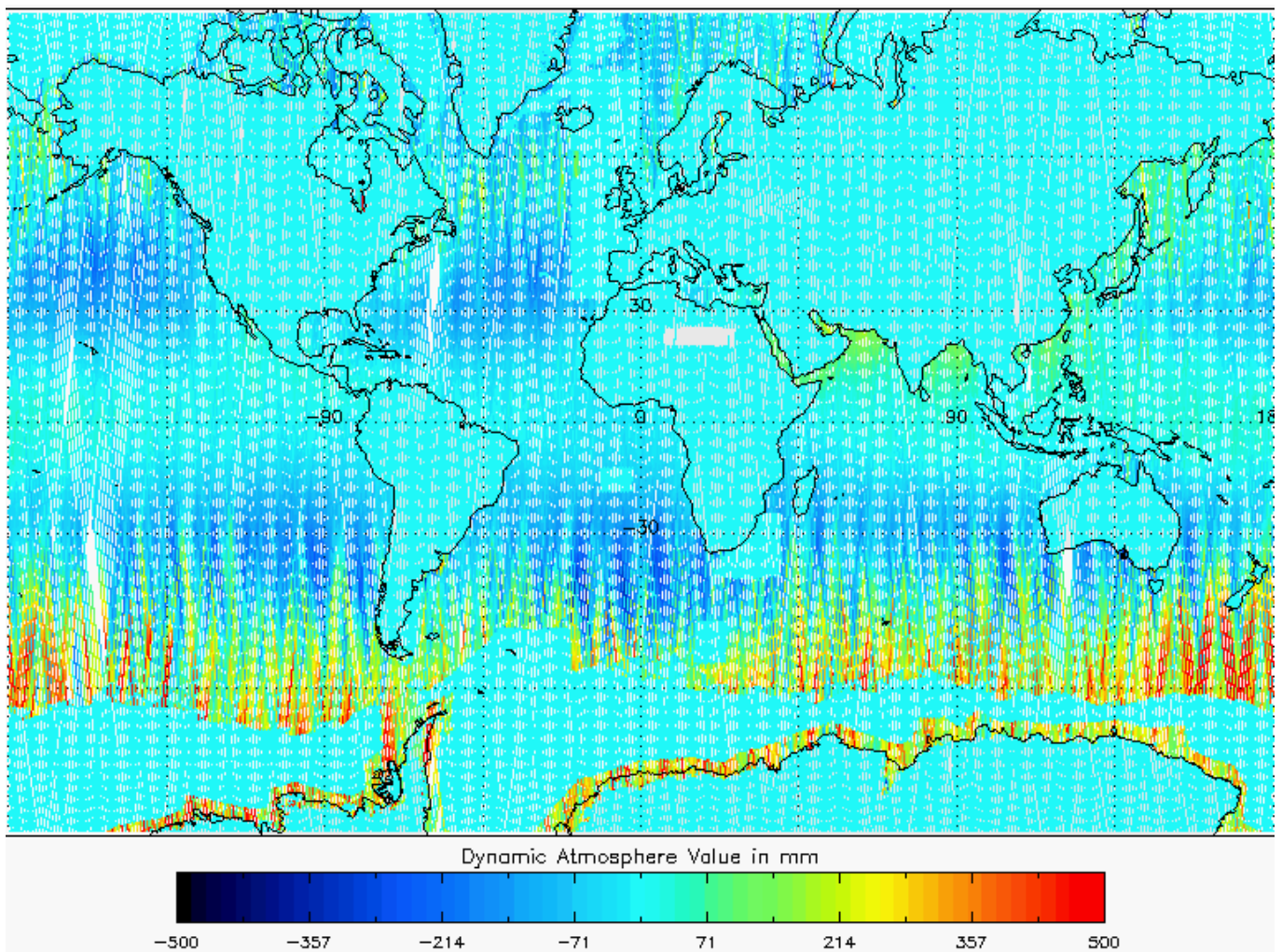
Figure 5-23 Global plot of Dynamic Atmosphere Correction for cycle 9.
