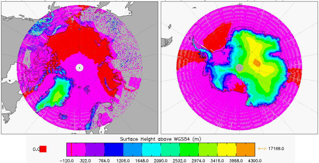
Figure 5-14 Polar plots of Surface Height over land and ocean areas for cycle 9.
