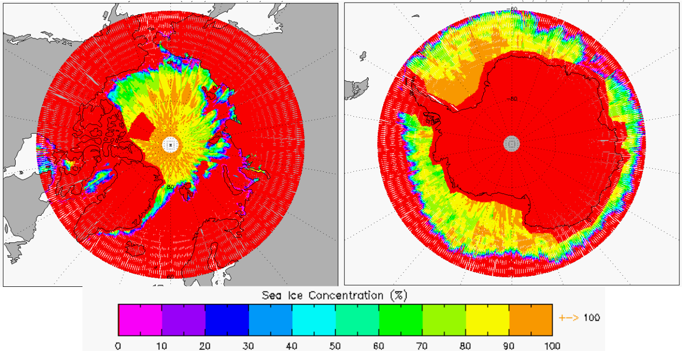
Figure 5-13 Polar plots of Sea Ice Concentration for cycle 9.
