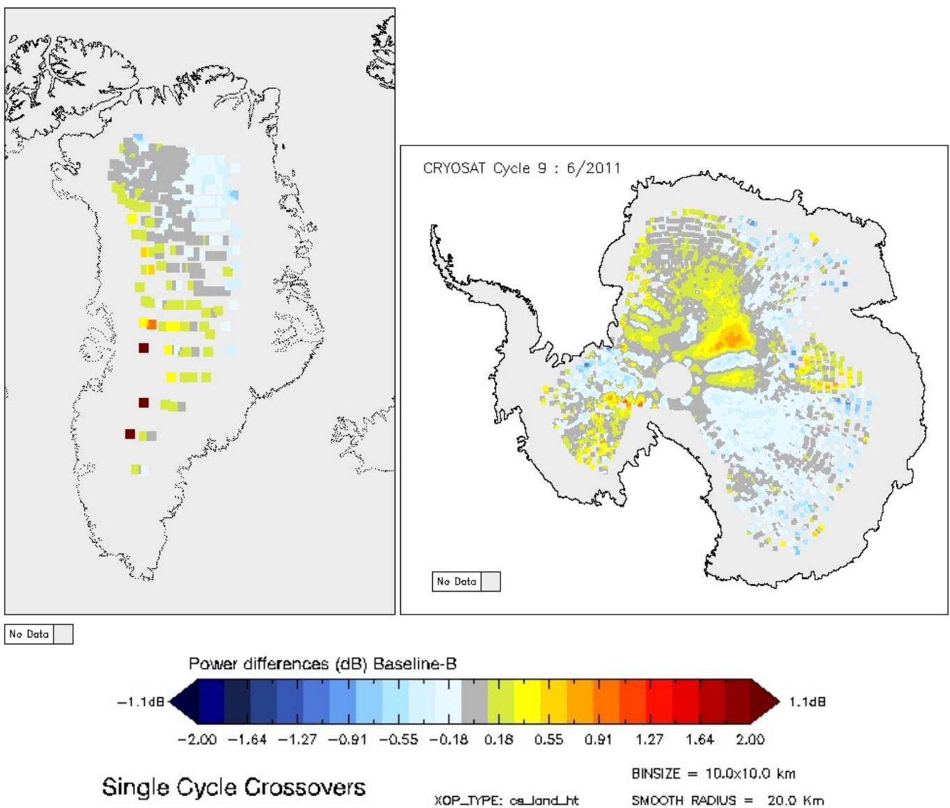
Figure 5-18 Greenland and Antarctica maps of LRM power differences for cycle 9.
