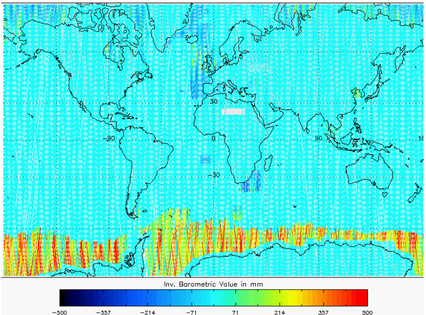
Figure 5-22 Global plot of Inverse Barometric Correction for cycle 9.
