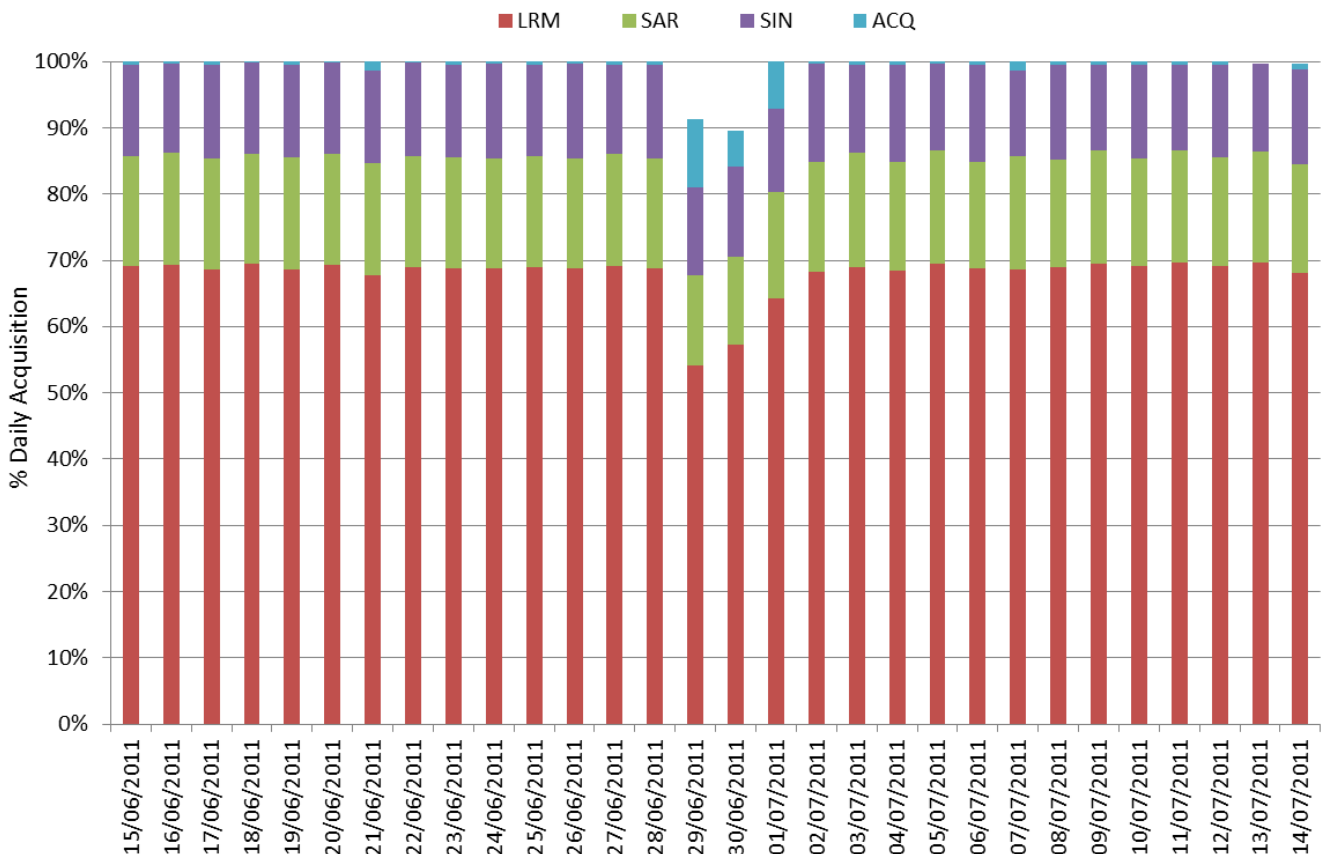
Figure 5-1 Daily percentages of SIRAL modes for cycle 9.
