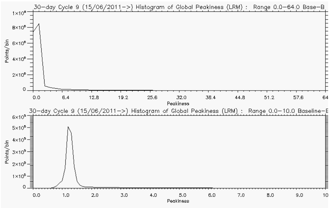
Figure 5-8 Histogram of global Peakiness for LRM, for cycle 9.
