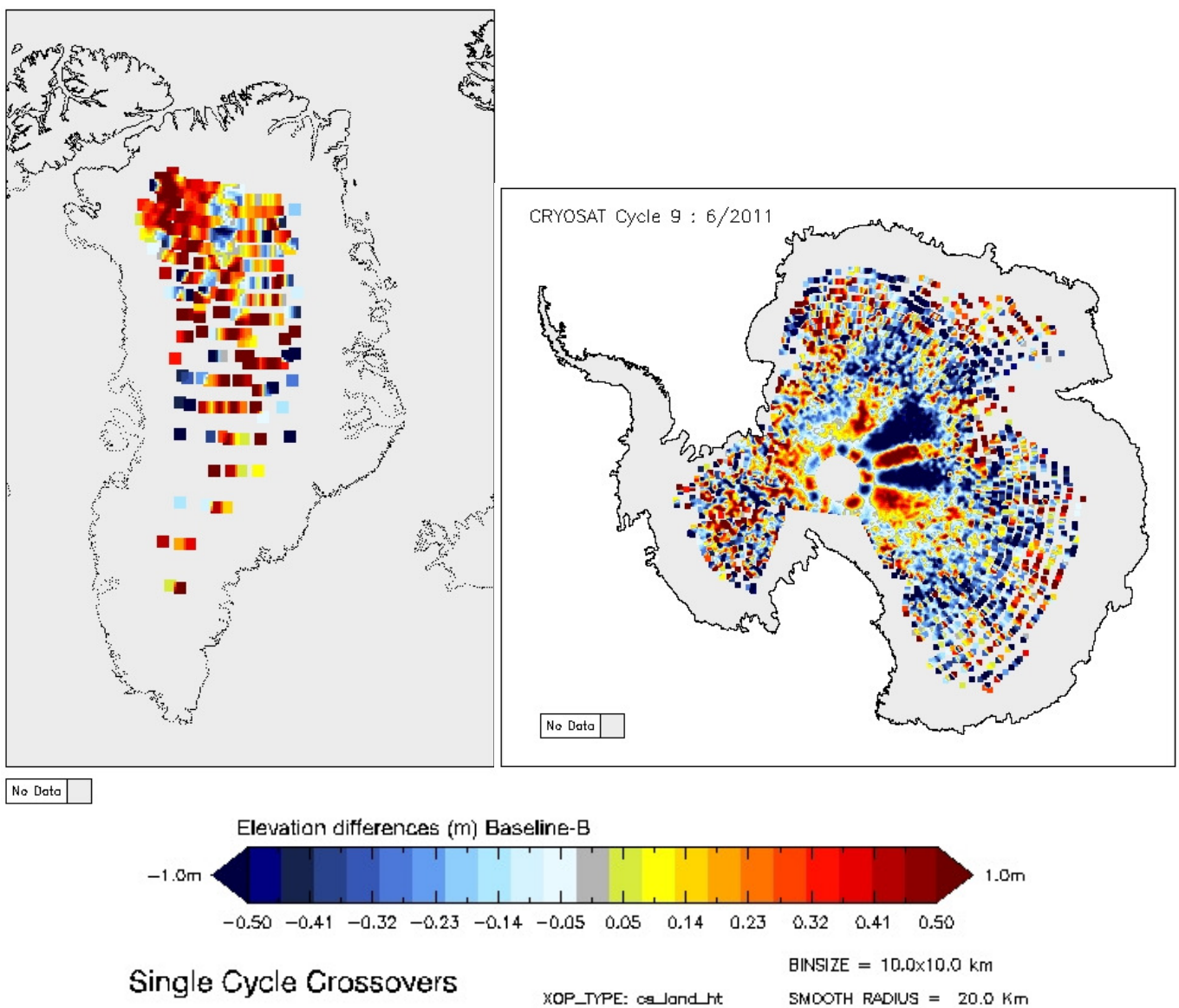
Figure 5-16 Greenland and Antarctica maps of LRM elevation differences for cycle 9.
