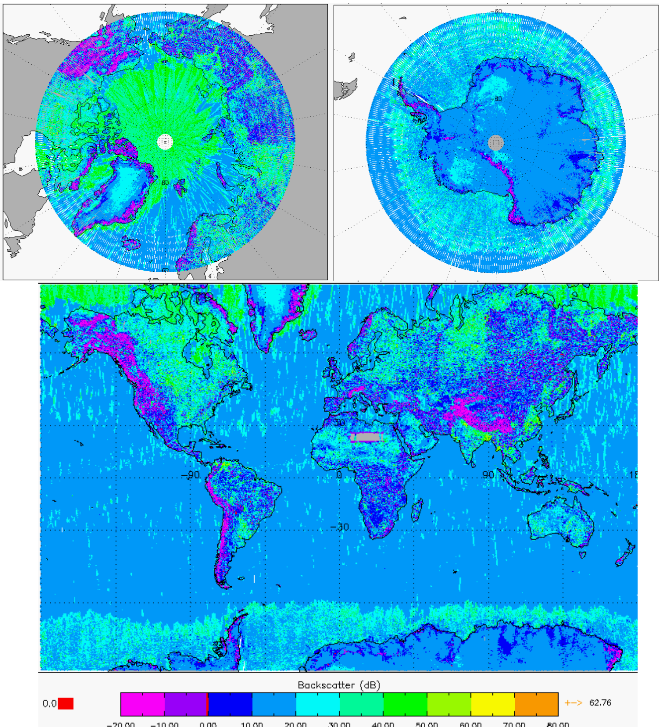
Figure 5-4 Global and Polar plots of Backscatter for cycle 9.
