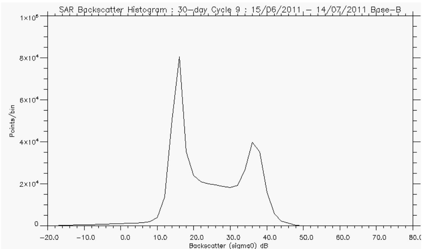
Figure 5-6 Backscatter Histogram for SAR, cycle 9.
