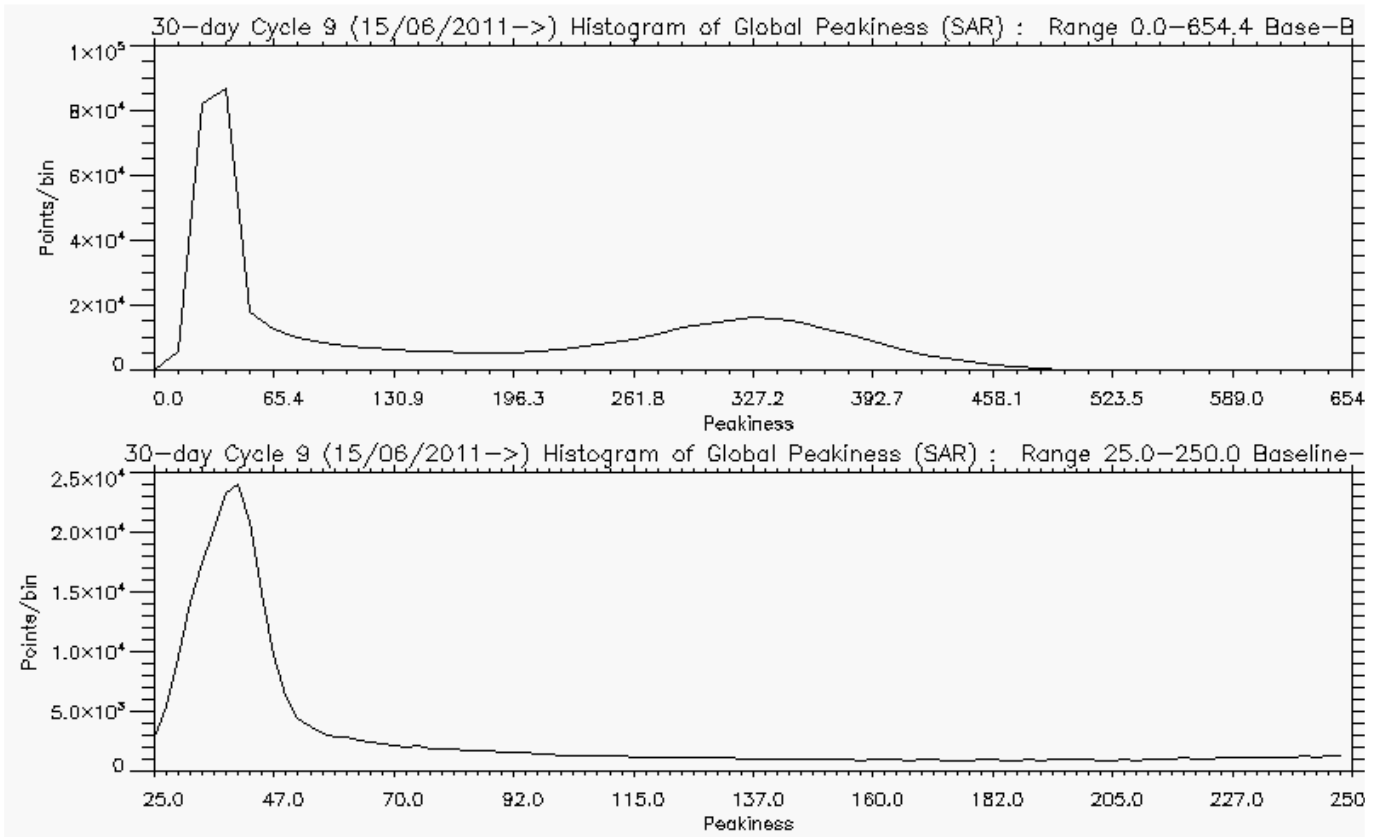
Figure 5-9 Histogram of global Peakiness for SAR, for cycle 9.
