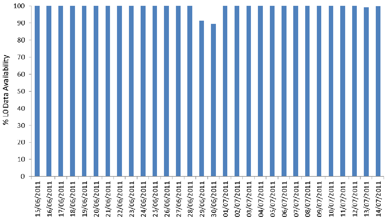
Figure 4-1 SIRAL L0 Data Availability for cycle 9.
