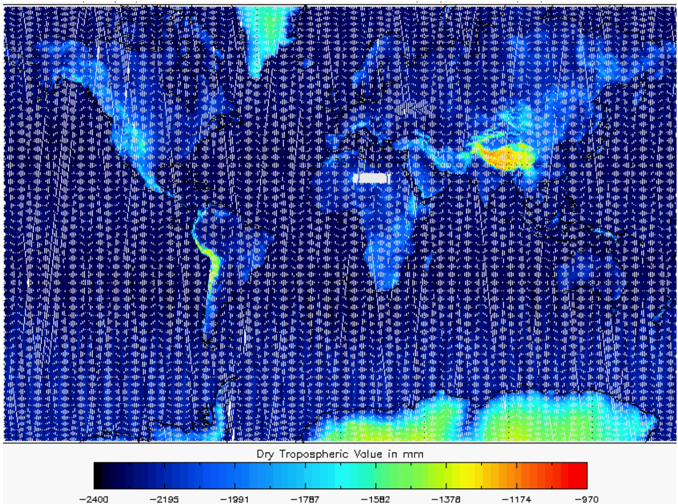
Figure 5-20 Global plot of Dry Tropospheric Correction for cycle 9.
