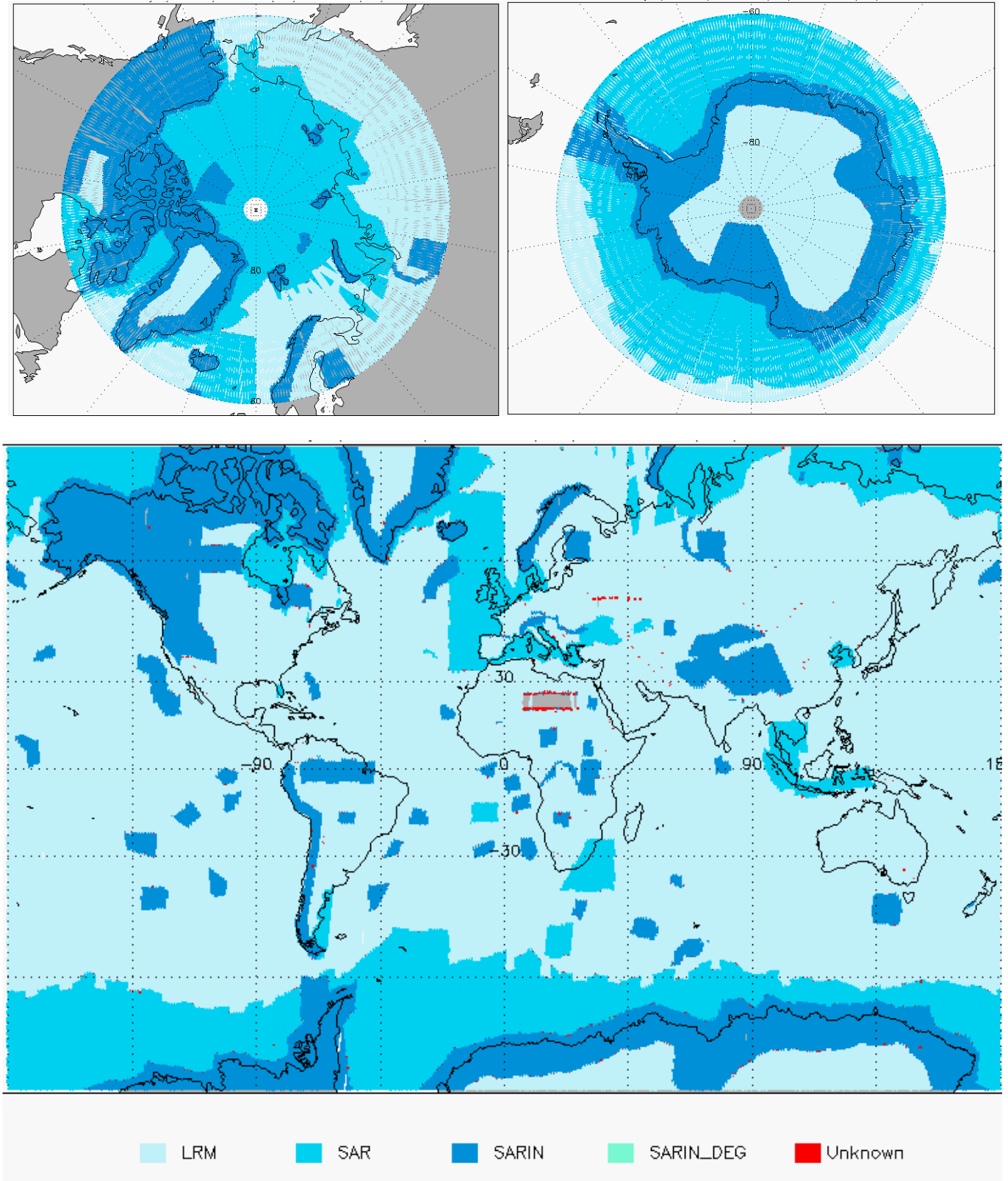
Figure 5-2 Global and Polar plots of SIRAL Modes for cycle 9.
