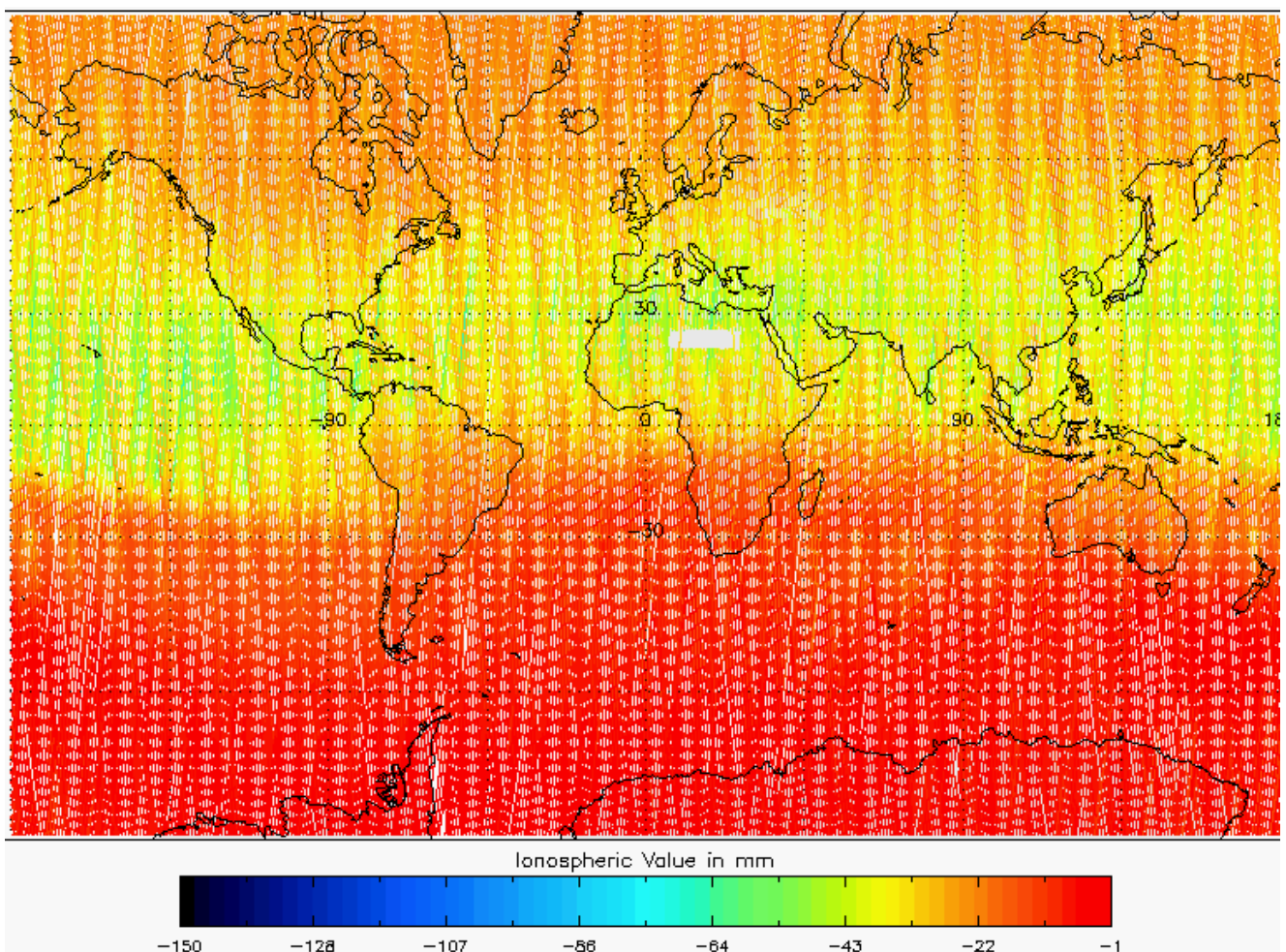
Figure 5-24 Global plot of Ionospheric Correction for cycle 9.
