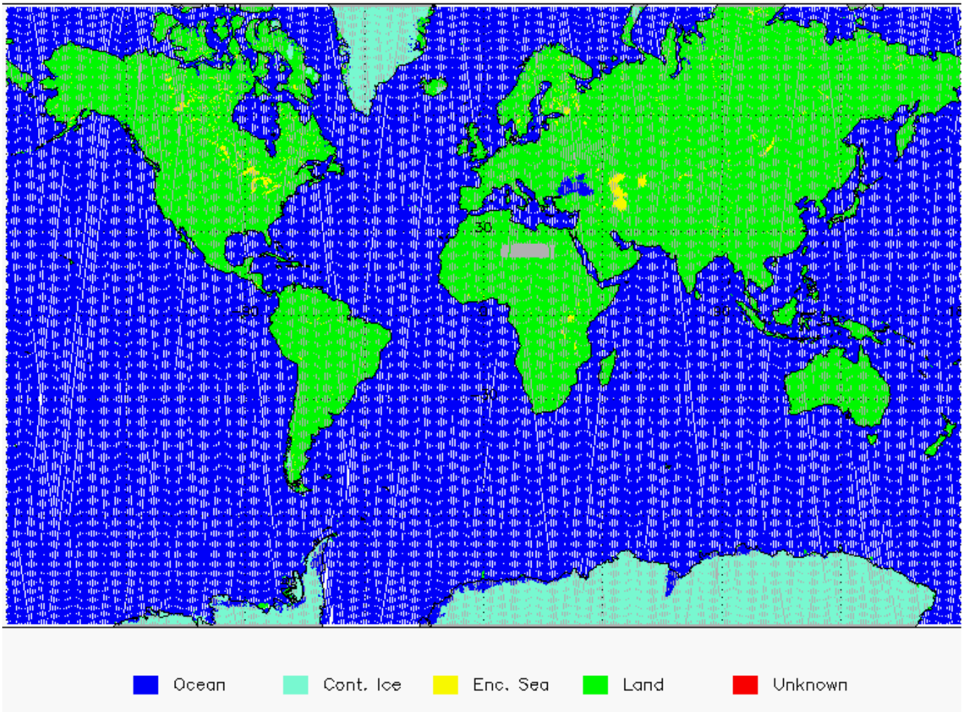
Figure 5-3 Global plot of Surface Type for cycle 9.
