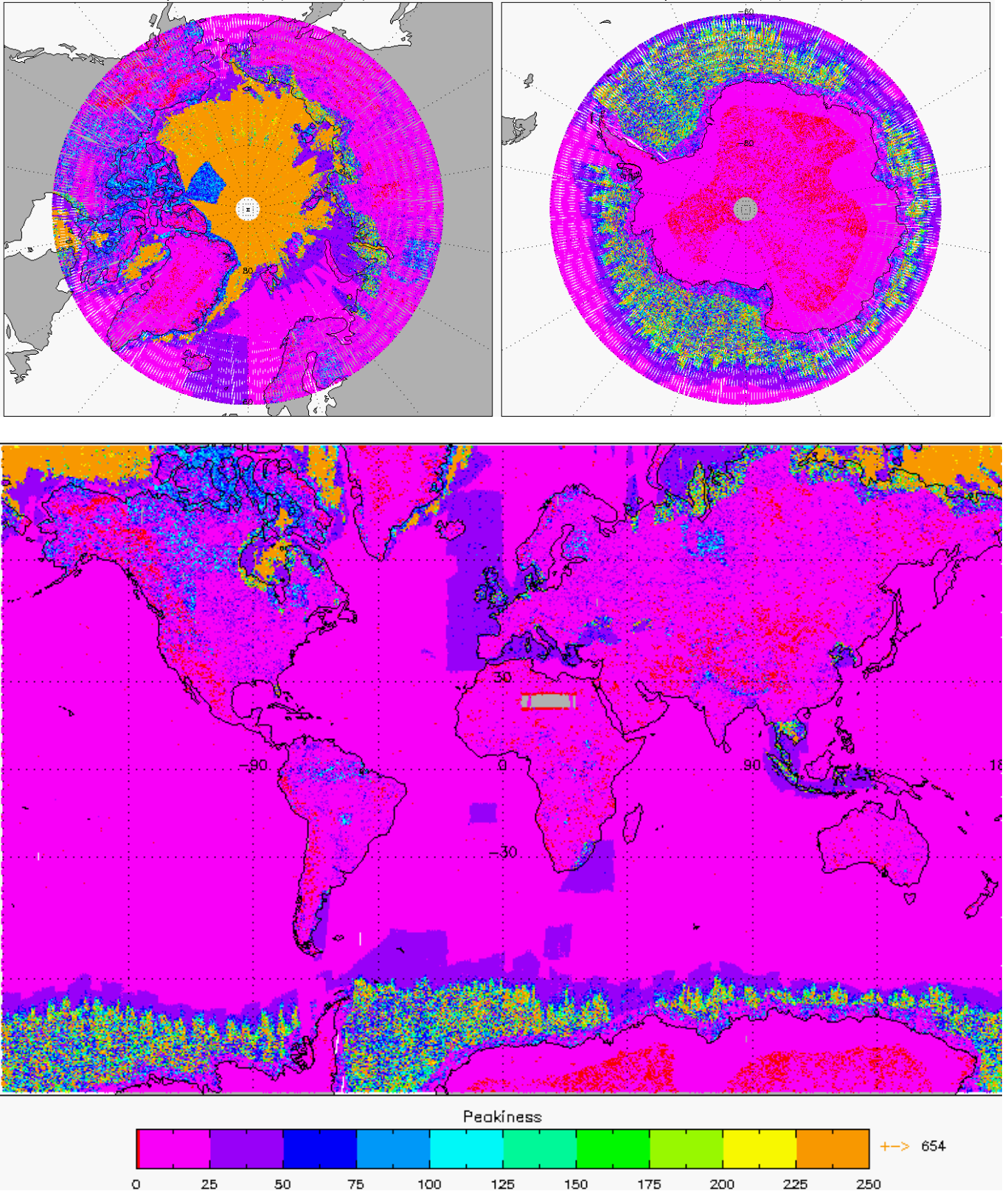
Figure 5-11 Global and Polar plots of Waveform Peakiness for cycle 9.
