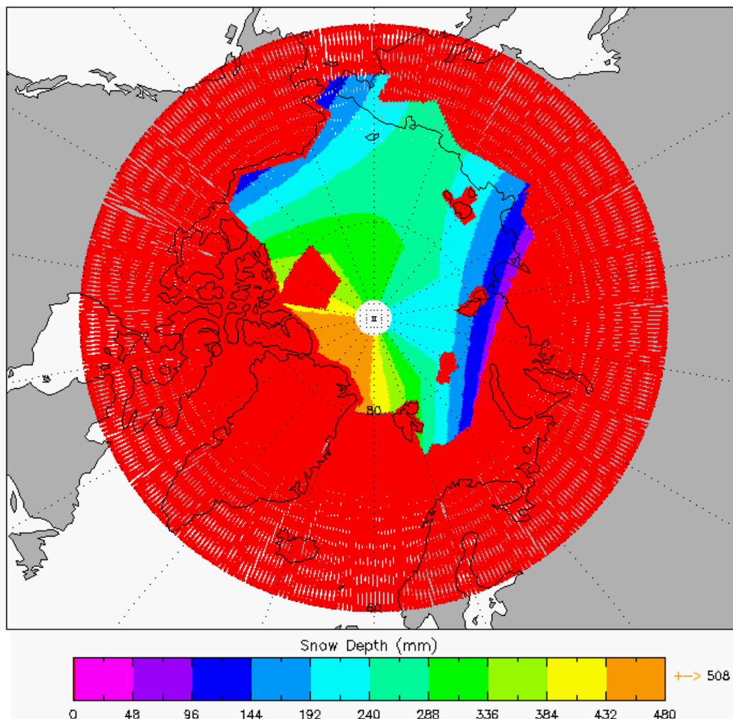
Figure 5-12 Arctic plot of Snow Depth for cycle 9.
