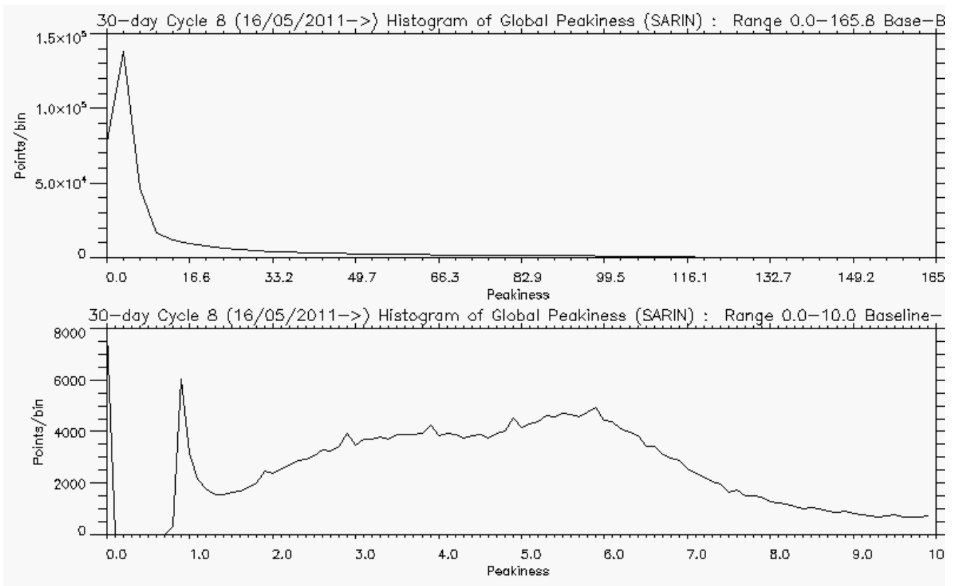
Figure 5-10 Histogram of global Peakiness for SARIn, for cycle 8.
