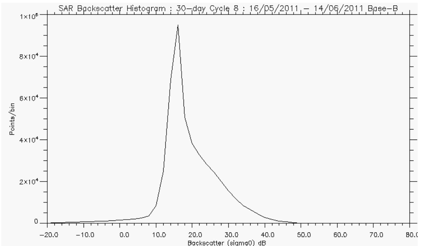
Figure 5-6 Backscatter Histogram for SAR, cycle 8.
