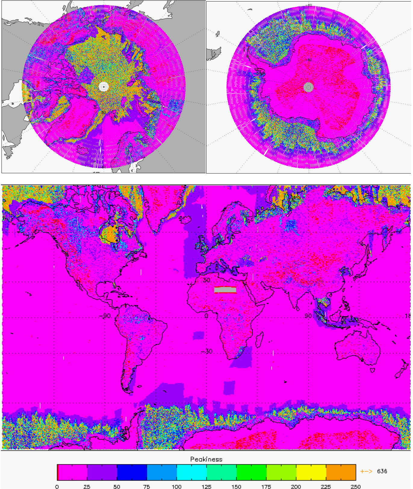
Figure 5-11 Global and Polar plots of Waveform Peakiness for cycle 8.
