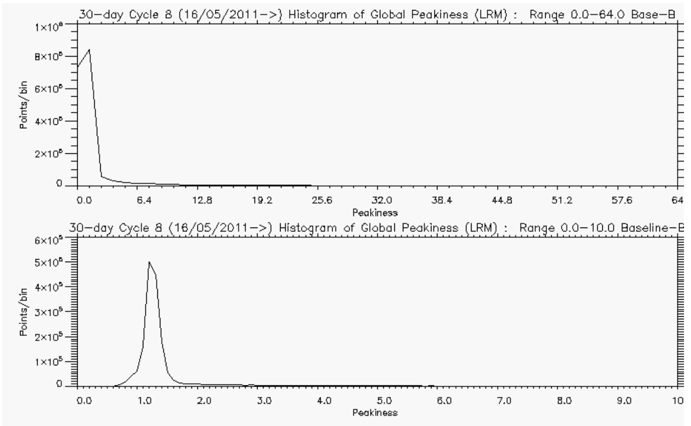
Figure 5-8 Histogram of global Peakiness for LRM, for cycle 8.
