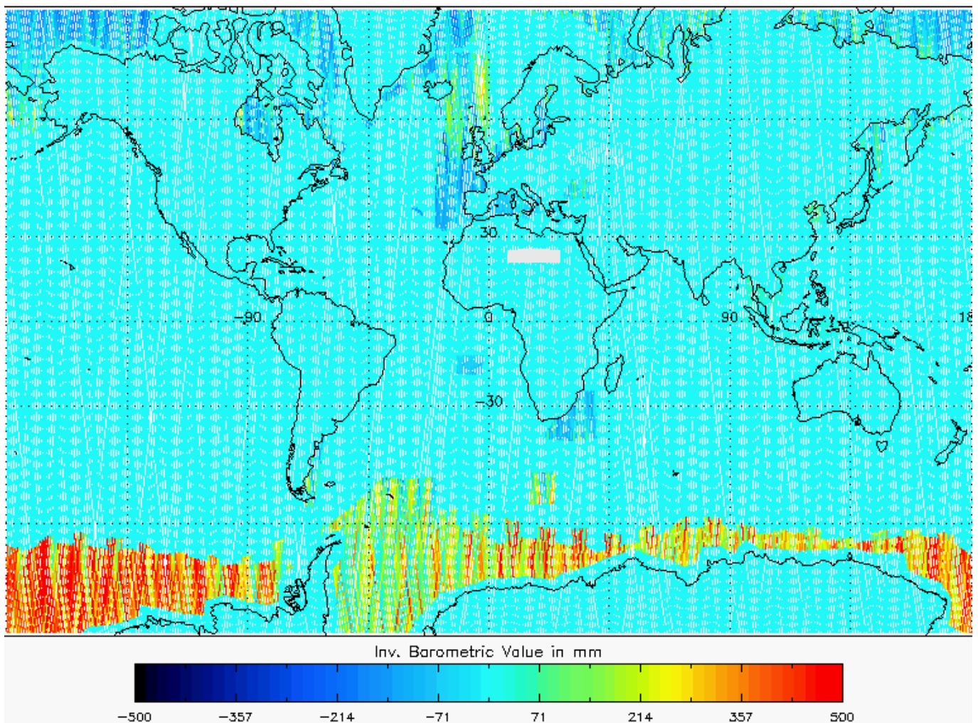
Figure 5-22 Global plot of Inverse Barometric Correction for cycle 8.
