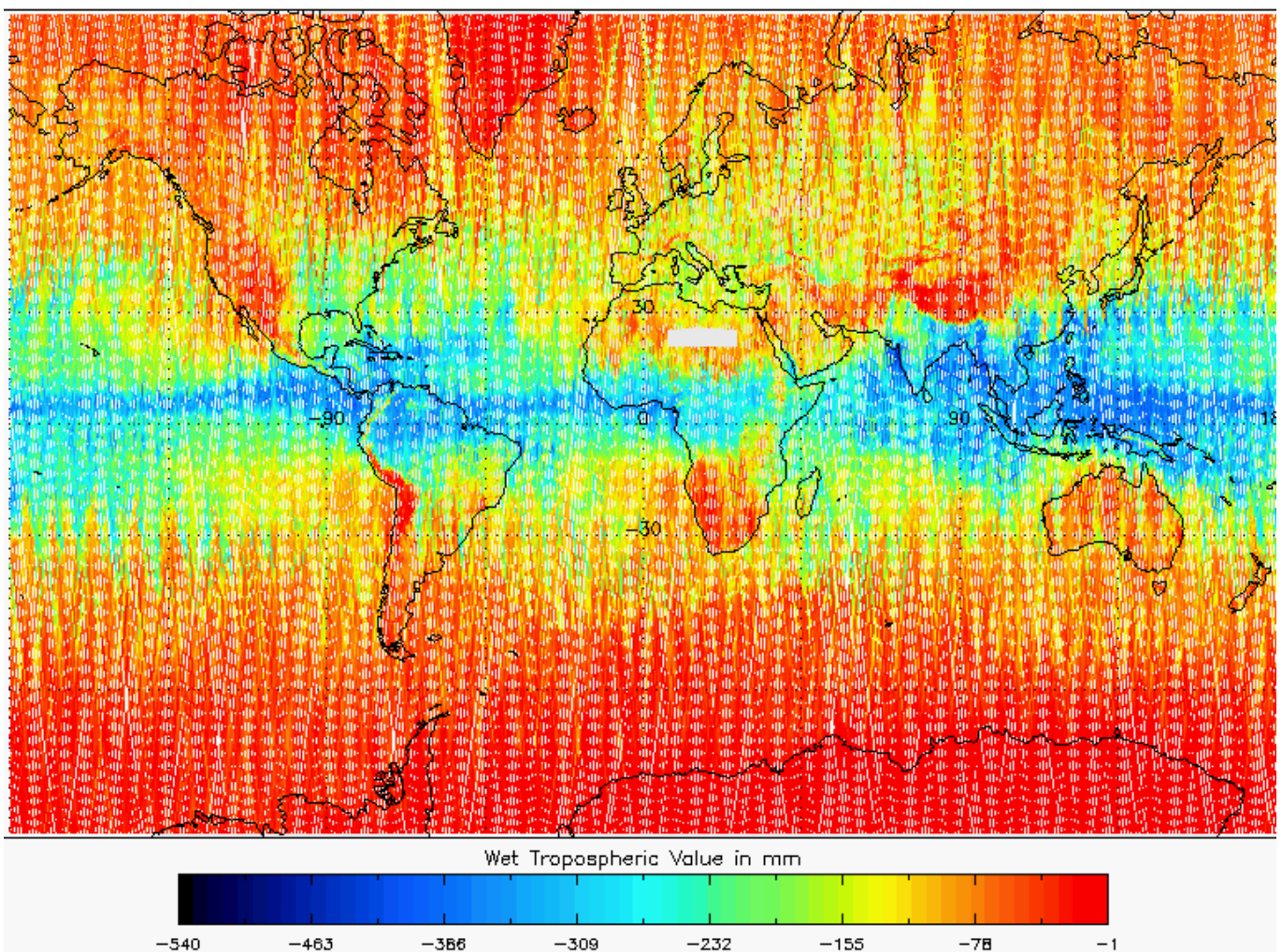
Figure 5-21 Global plot of Wet Tropospheric Correction for cycle 8.
