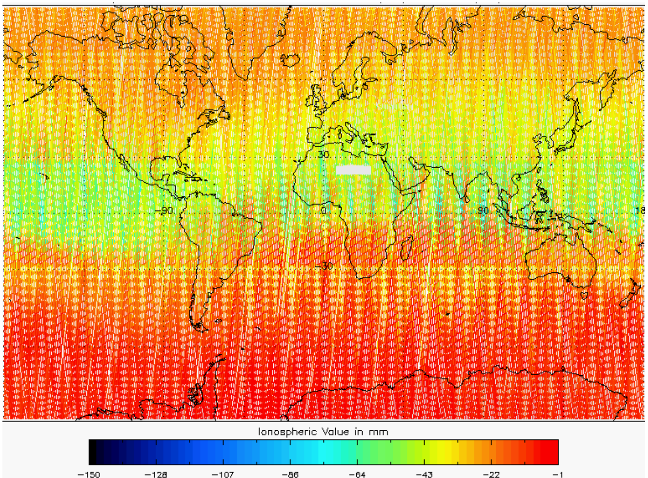
Figure 5-24 Global plot of Ionospheric Correction for cycle 8.
