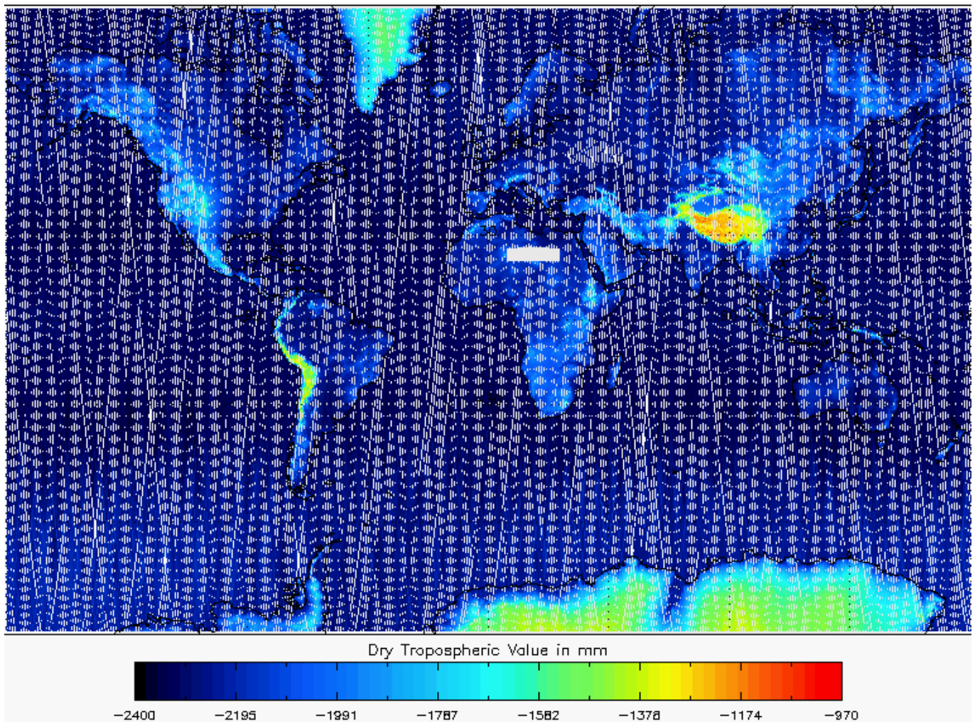
Figure 5-20 Global plot of Dry Tropospheric Correction for cycle 8.
