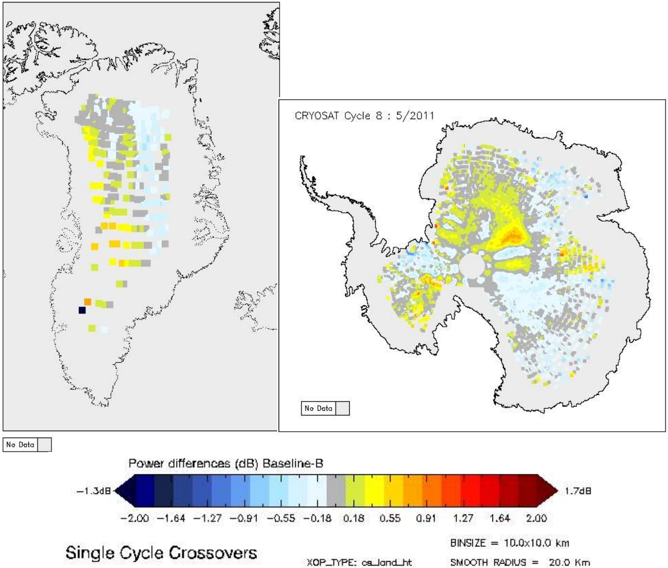
Figure 5-18 Greenland and Antarctica maps of LRM power differences for cycle 8.
