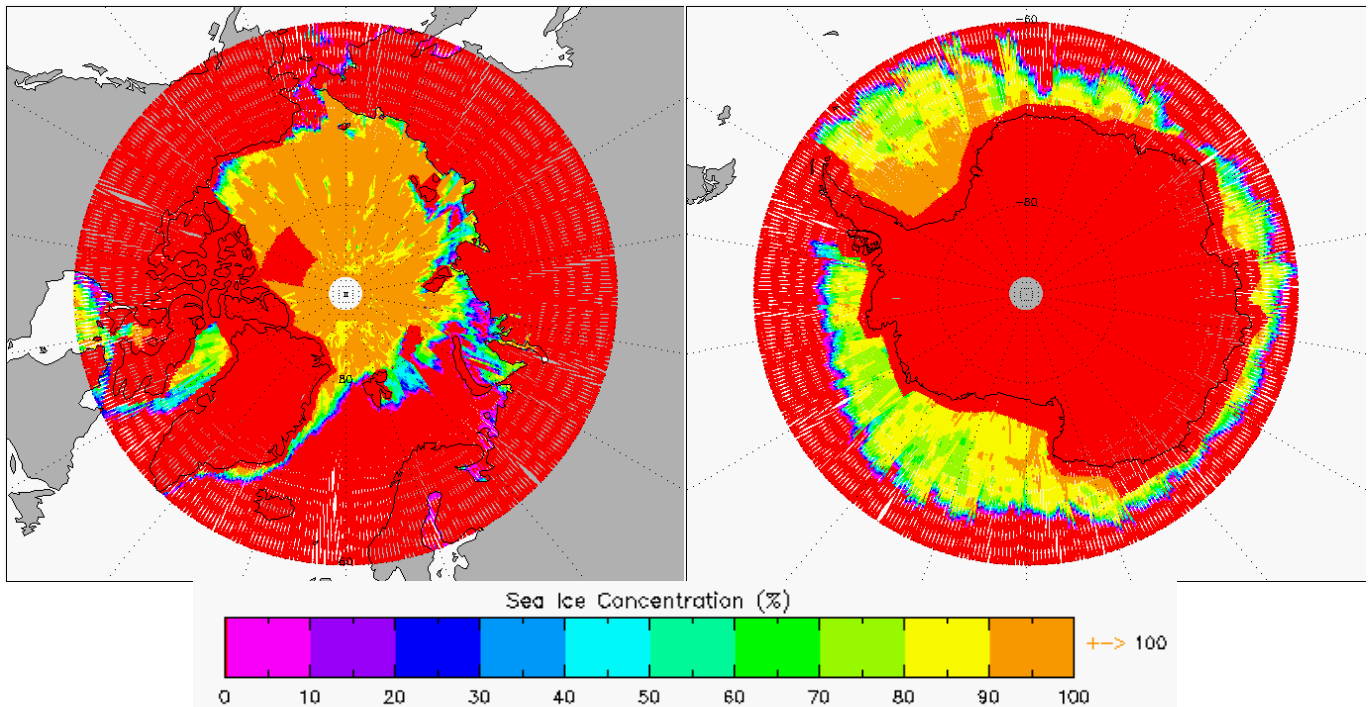
Figure 5-13 Polar plots of Sea Ice Concentration for cycle 8.
