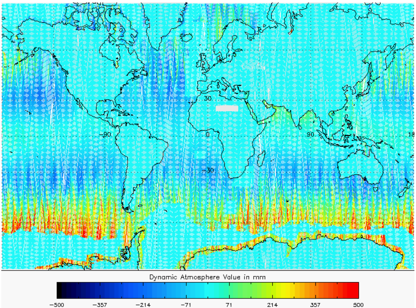
Figure 5-23 Global plot of Dynamic Atmosphere Correction for cycle 8.
