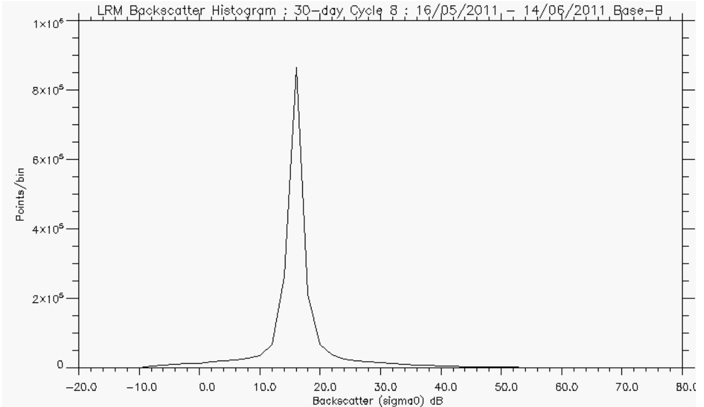
Figure 5-5 Backscatter Histogram for LRM, cycle 8.
