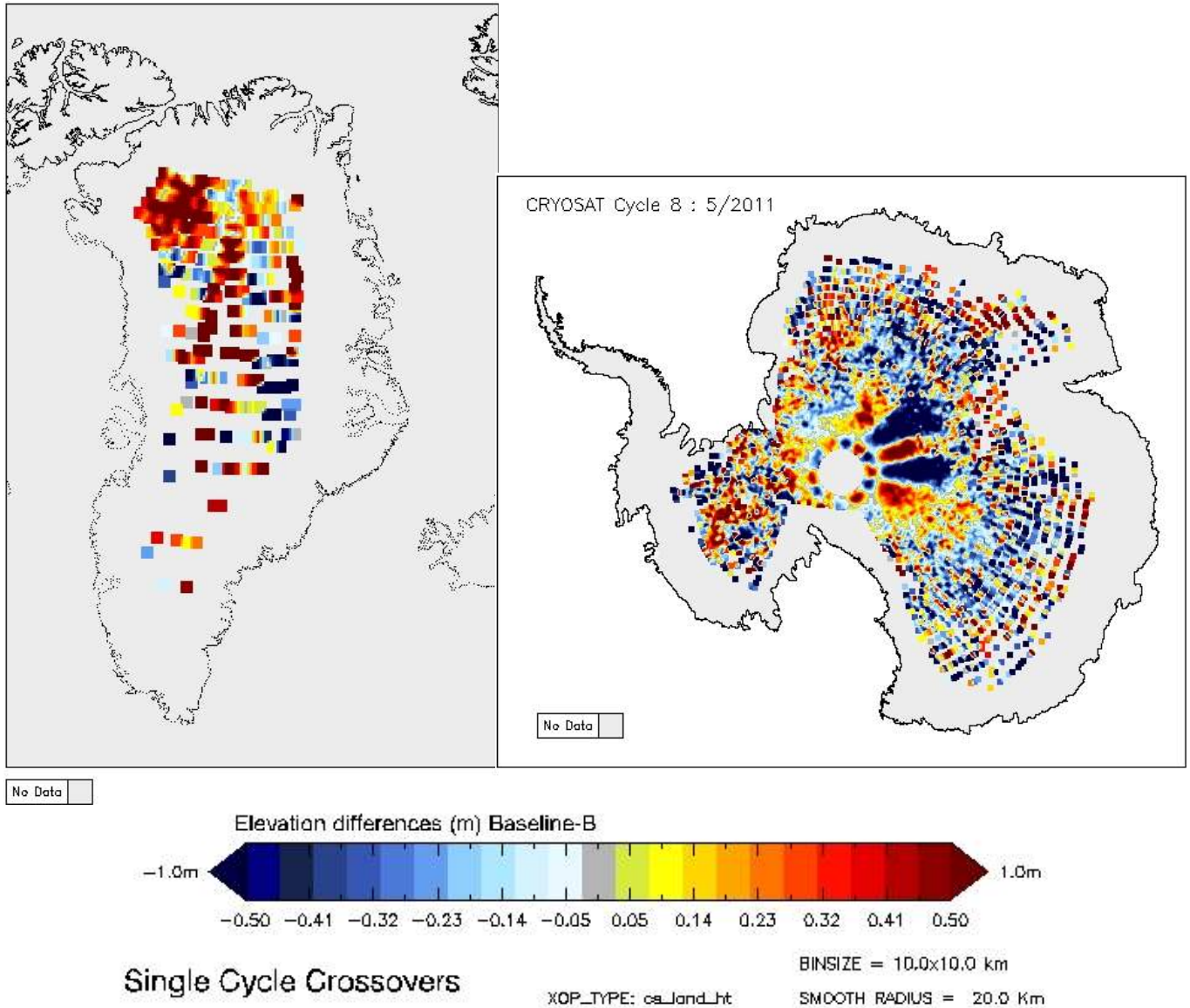
Figure 5-16 Greenland and Antarctica maps of LRM elevation differences for cycle 8.
