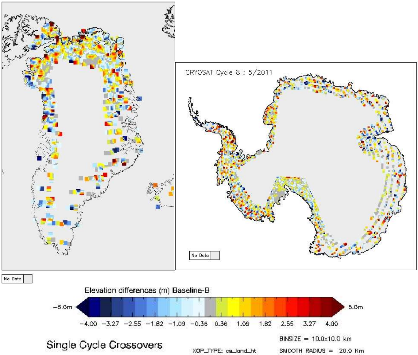
Figure 5-17 Greenland and Antarctica maps of SARIn elevation differences for cycle 8.
