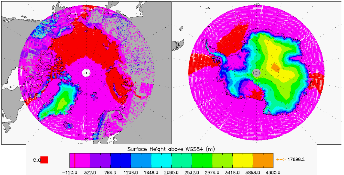
Figure 5-14 Polar plots of Surface Height over land and ocean areas for cycle 8.
