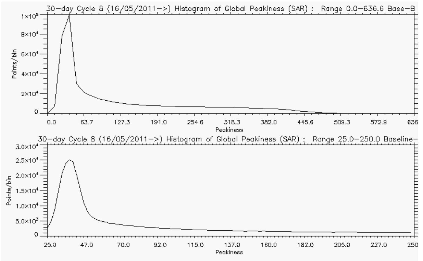
Figure 5-9 Histogram of global Peakiness for SAR, for cycle 8.
