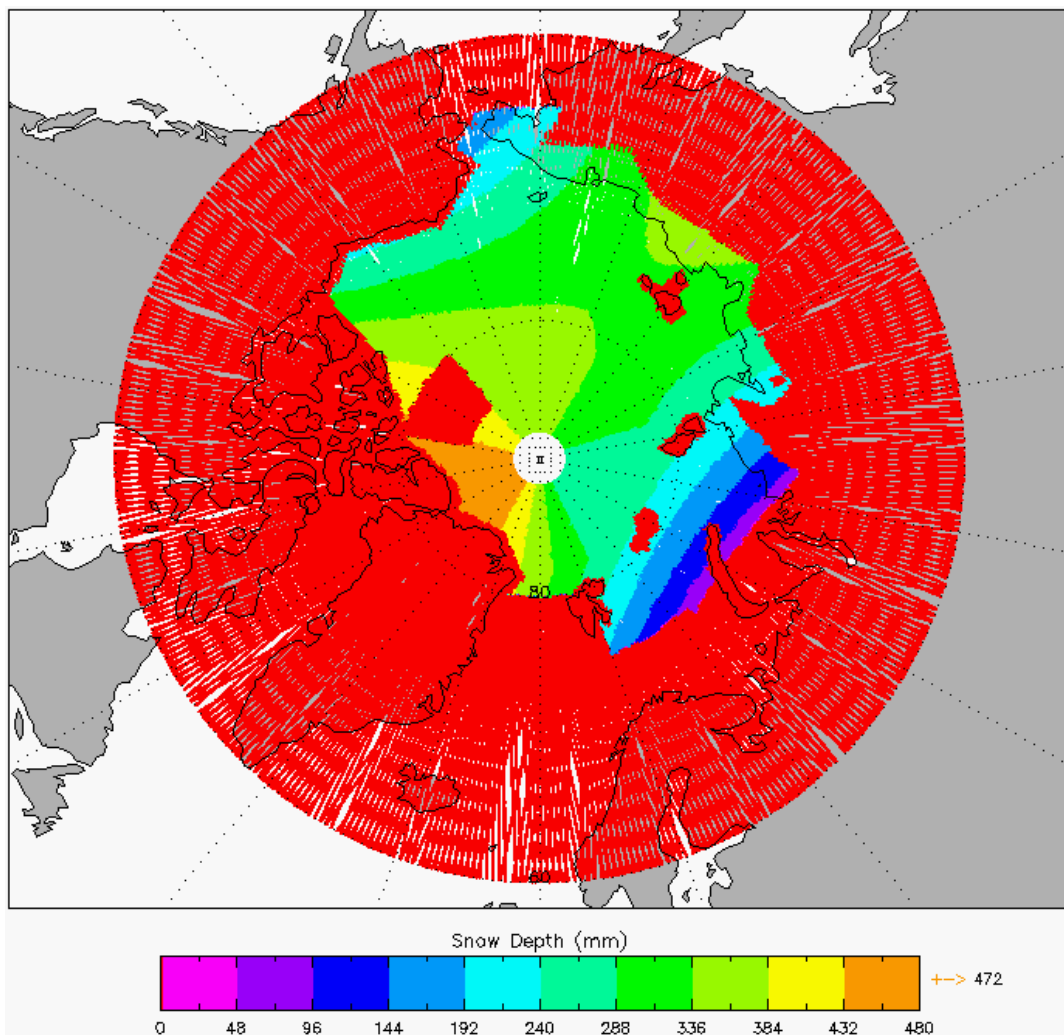
Figure 5-12 Arctic plot of Snow Depth for cycle 8.
