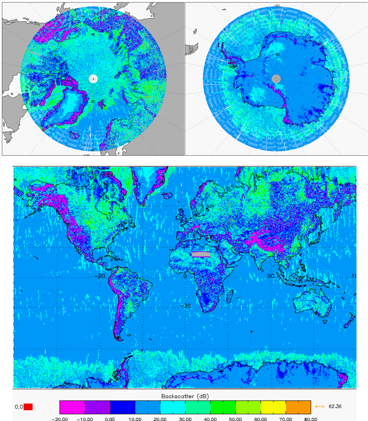
Figure 5-4 Global and Polar plots of Backscatter for cycle 8.
