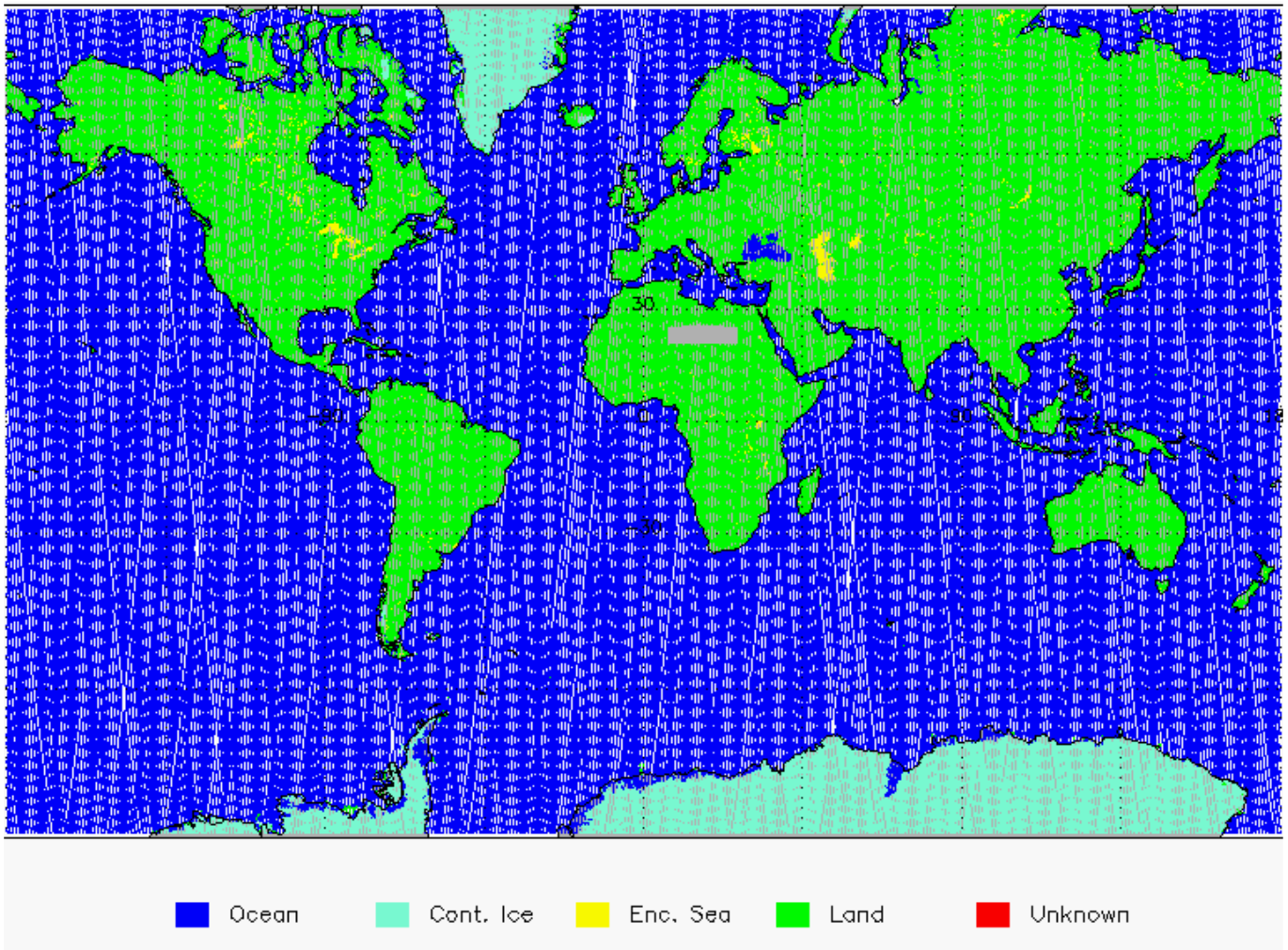
Figure 5-3 Global plot of Surface Type for cycle 8.
