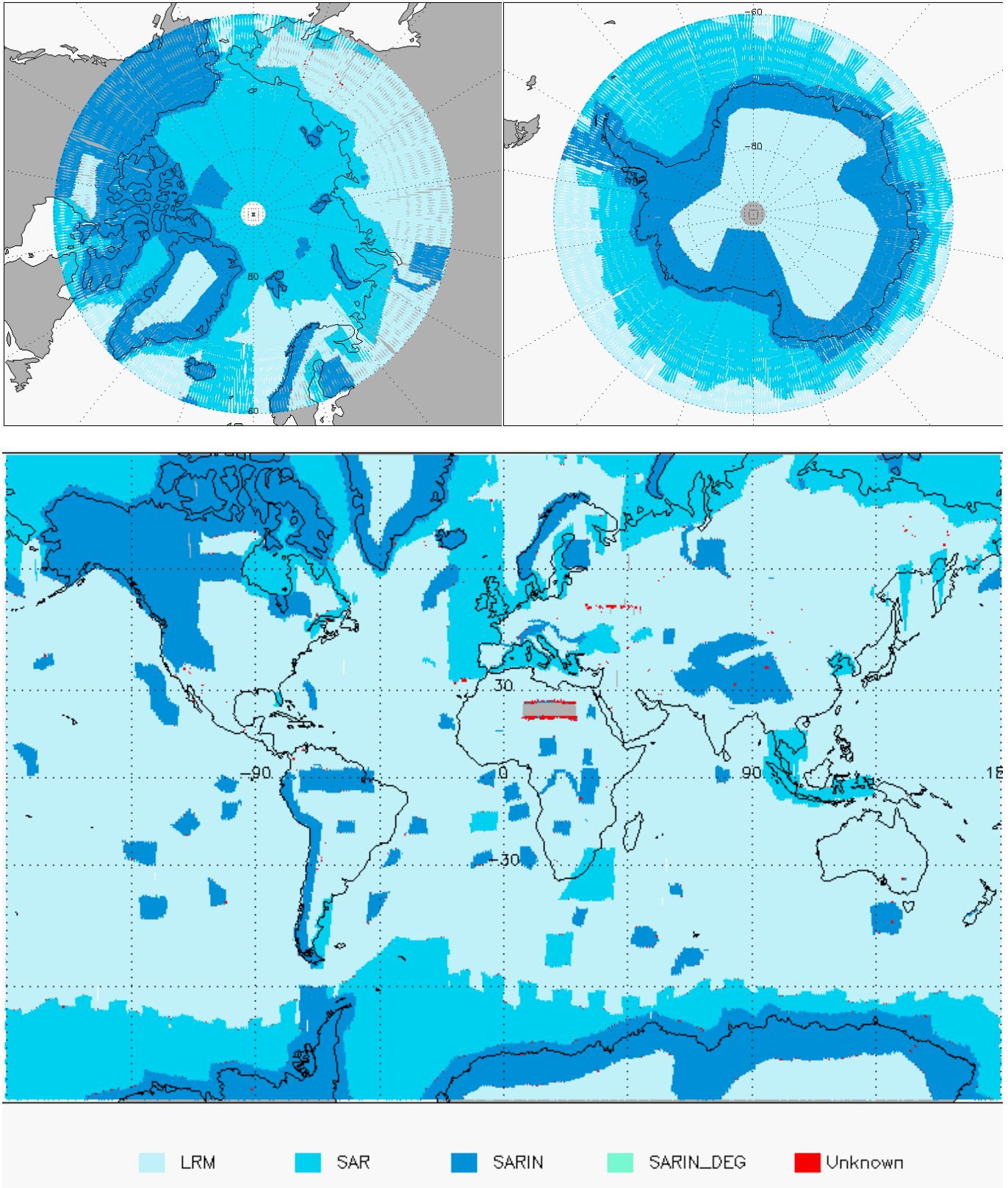
Figure 5-2 Global and Polar plots of SIRAL Modes for cycle 8.
