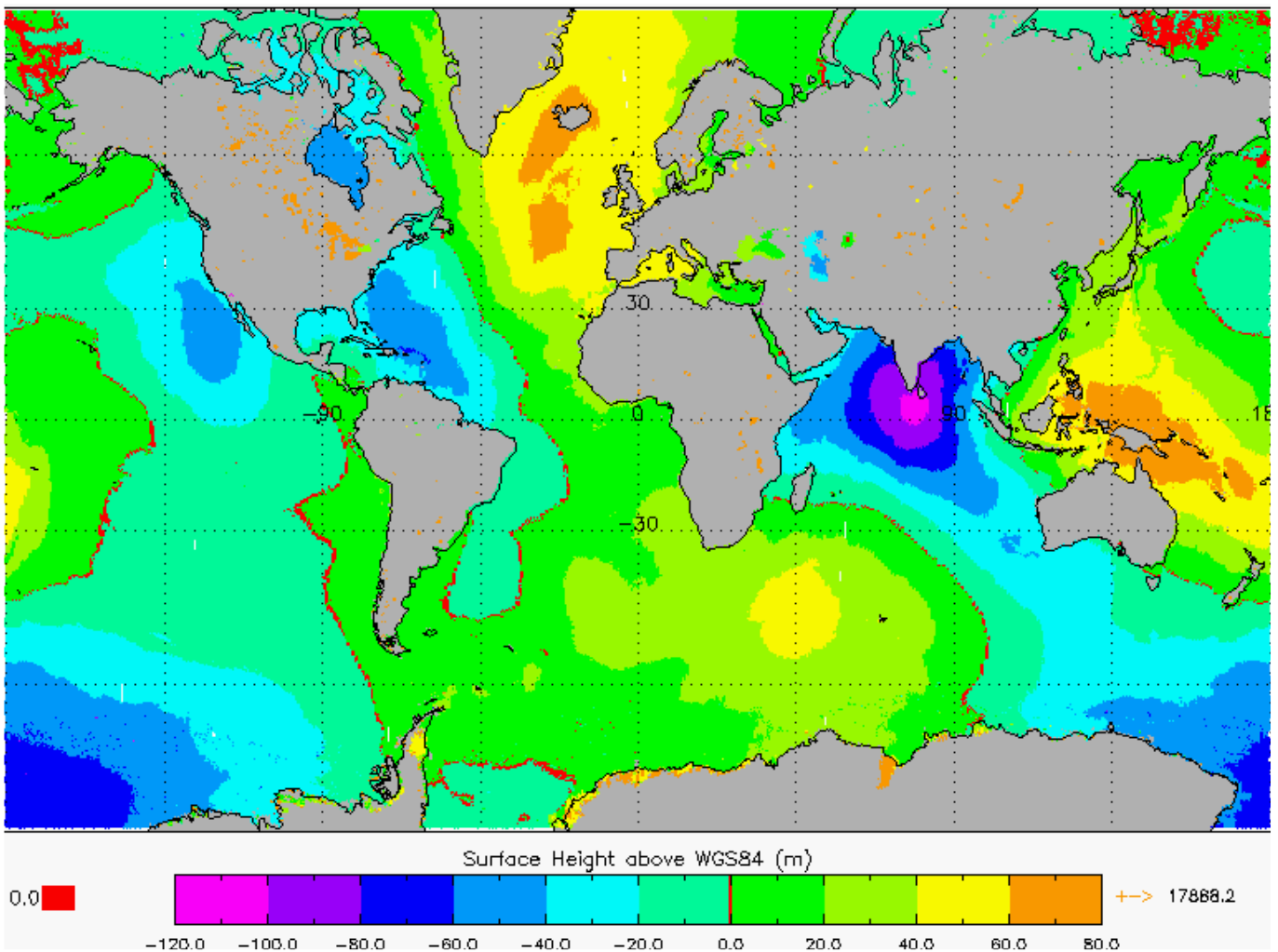
Figure 5-15 Global plots of Sea Surface Height over ocean areas only, for cycle 8.
