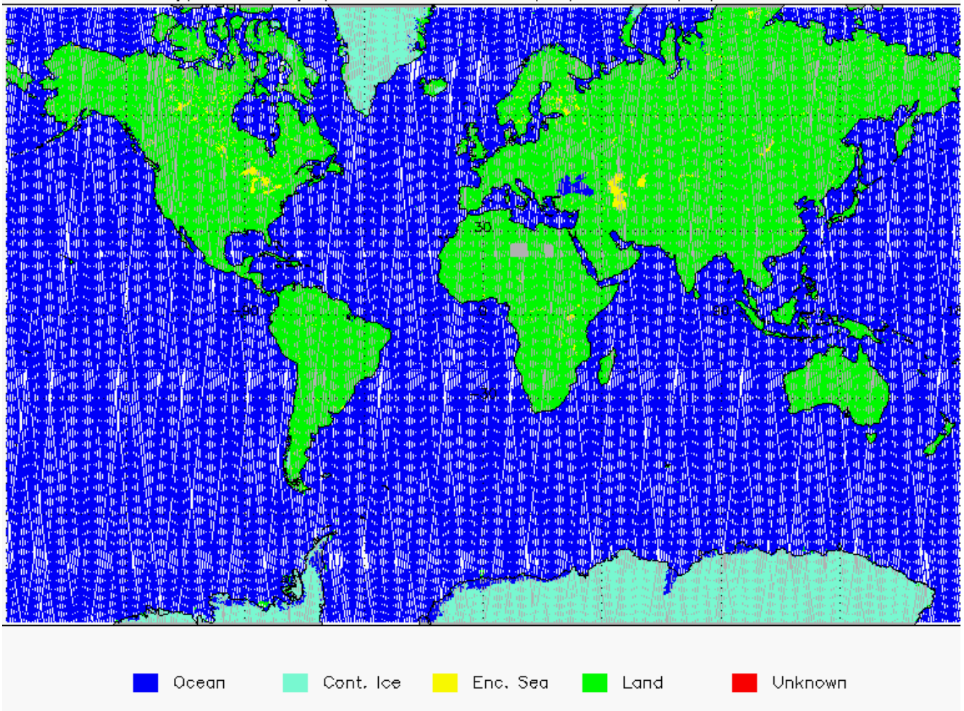
Figure 5-3 Global plot of Surface Type for cycle 5.
