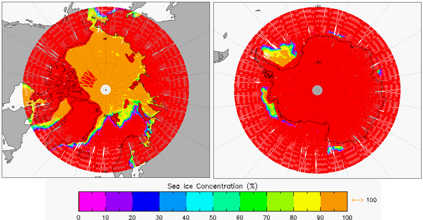
Figure 5-13 Polar plots of Sea Ice Concentration for cycle 5.
