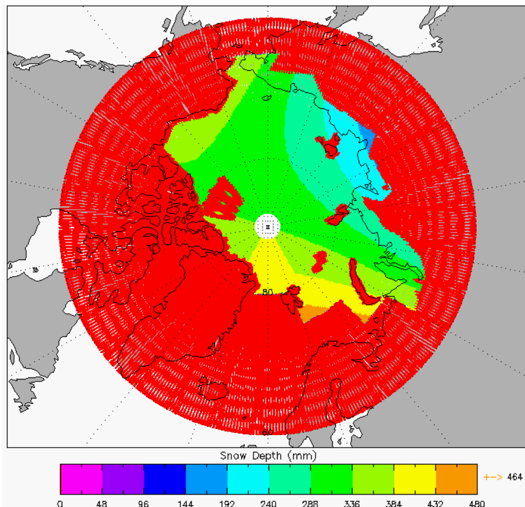
Figure 5-12 Arctic plot of Snow Depth for cycle 5.
