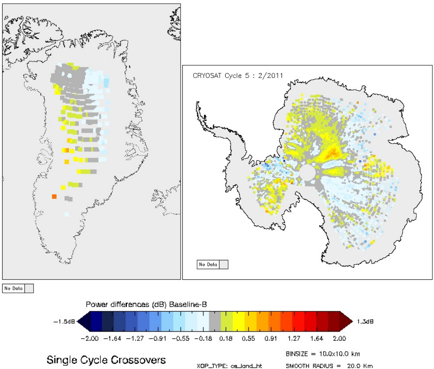
Figure 5-18 Greenland and Antarctica maps of LRM power differences for cycle 5.
