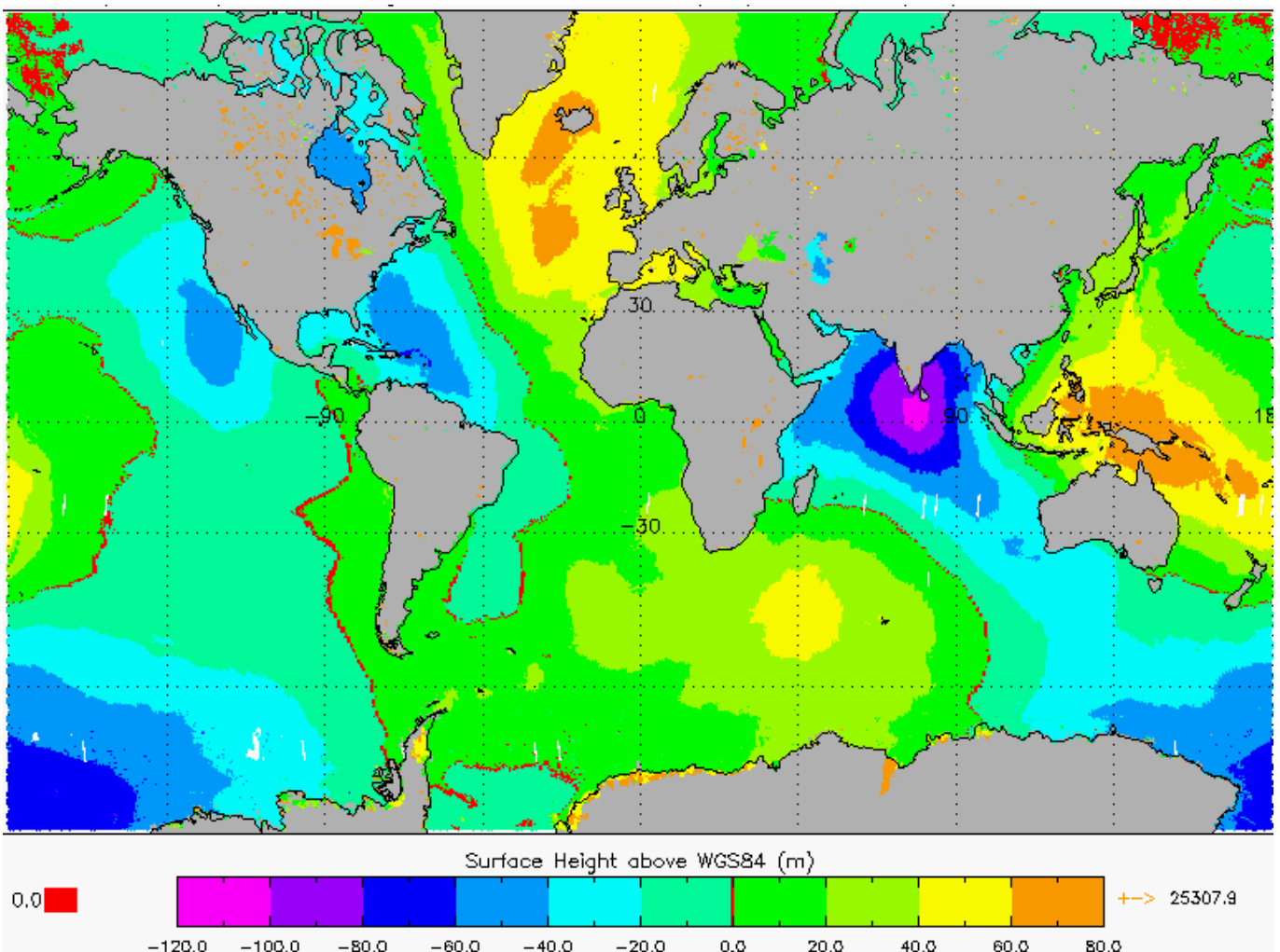
Figure 5-15 Global plots of Sea Surface Height over ocean areas only, for cycle 3.
