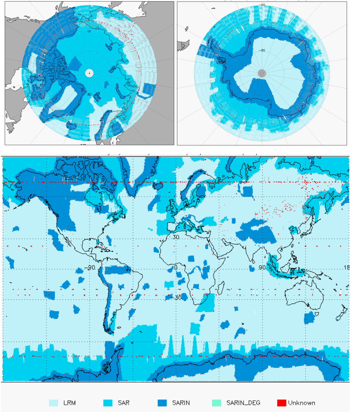
Figure 5-2 Global and Polar plots of SIRAL Modes for cycle 3.
