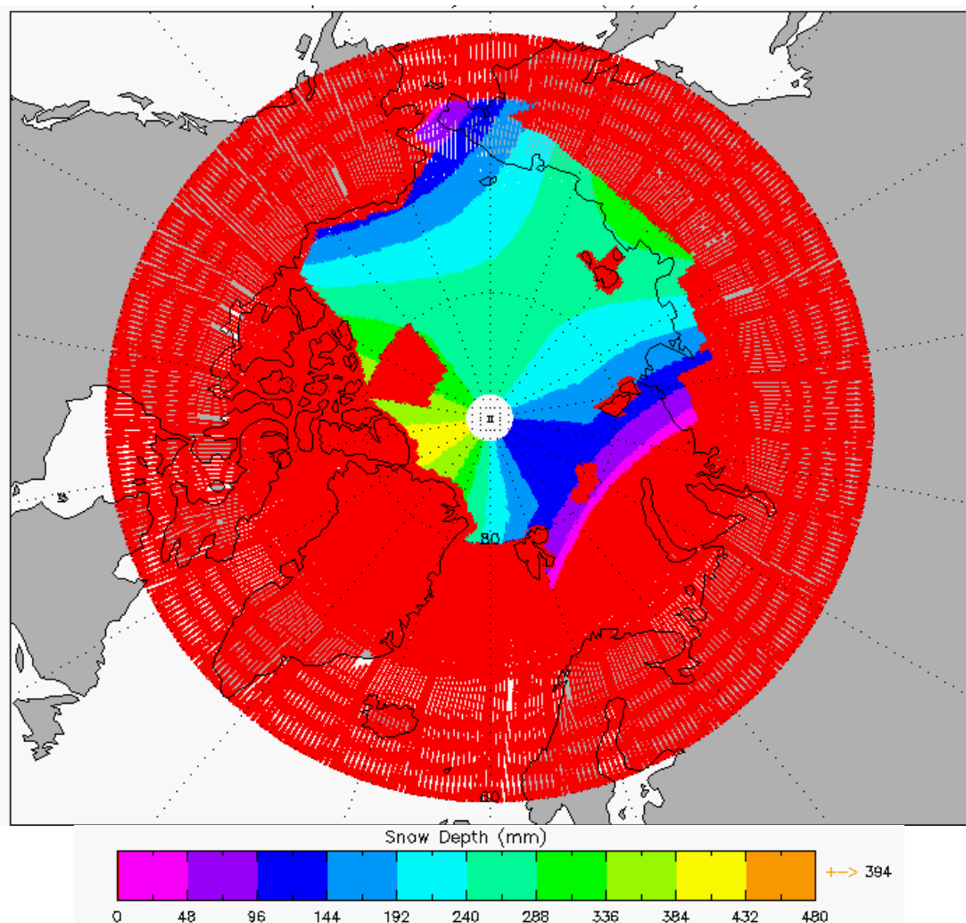
Figure 5-12 Arctic plot of Snow Depth for cycle 3.
