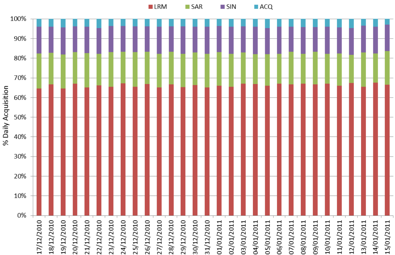
Figure 5-1 Daily percentages of SIRAL modes for cycle 3.
