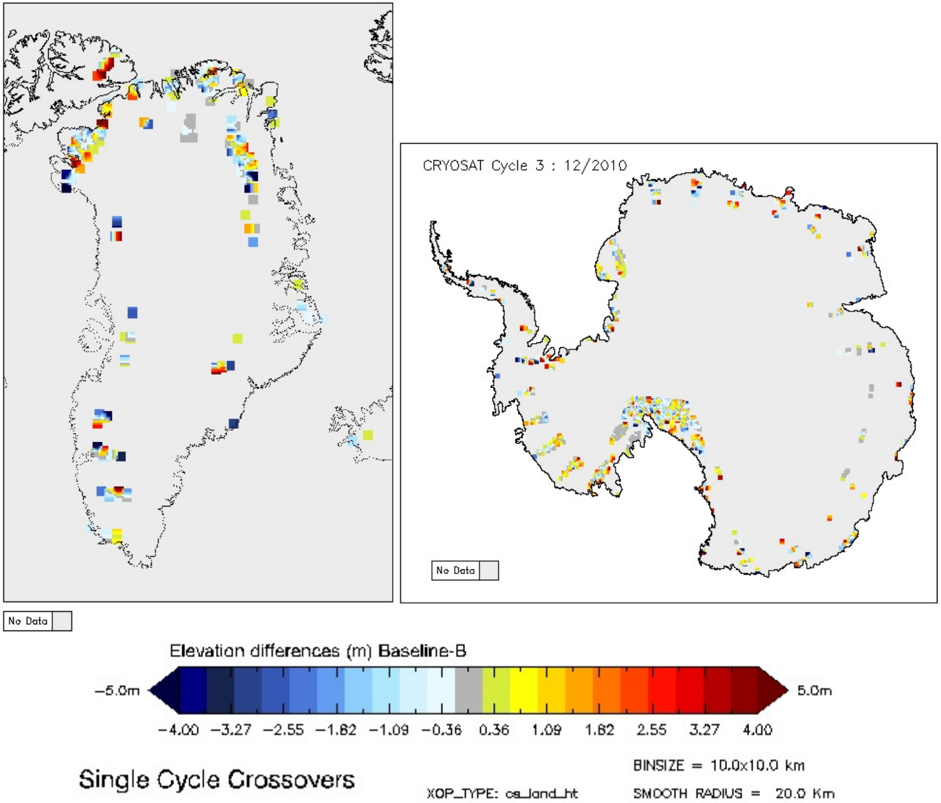
Figure 5-17 Greenland and Antarctica maps of SARIn elevation differences for cycle 3.
