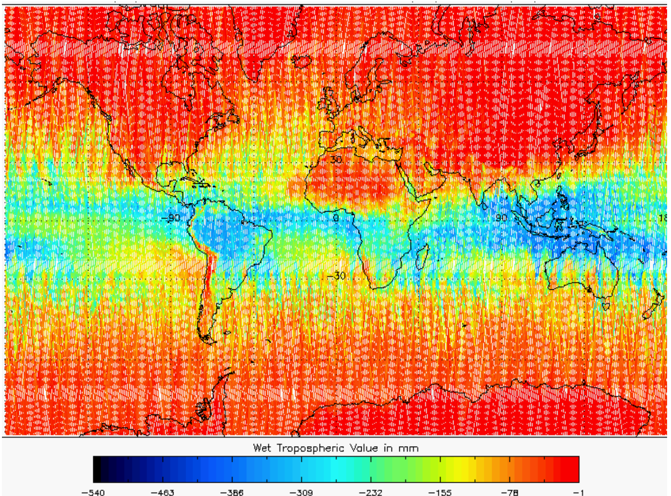
Figure 5-21 Global plot of Wet Tropospheric Correction for cycle 3.
