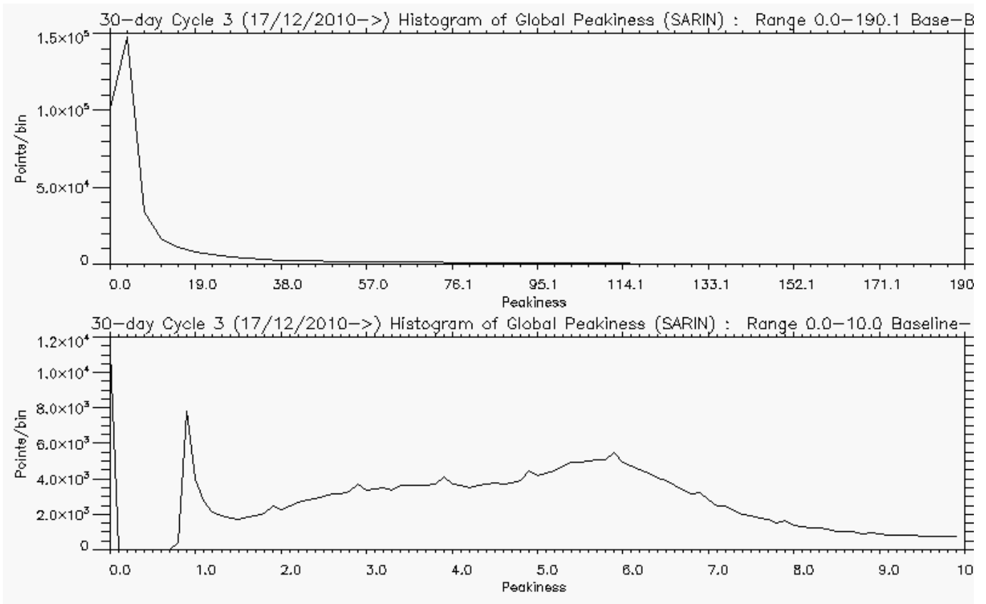
Figure 5-10 Histogram of global Peakiness for SARIn, for cycle 3.
