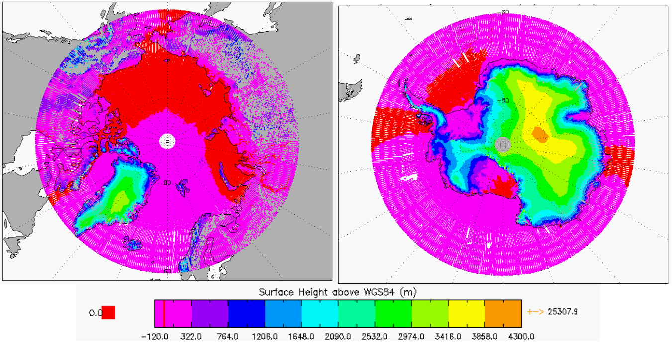
Figure 5-14 Polar plots of Surface Height over land and ocean areas for cycle 3.
