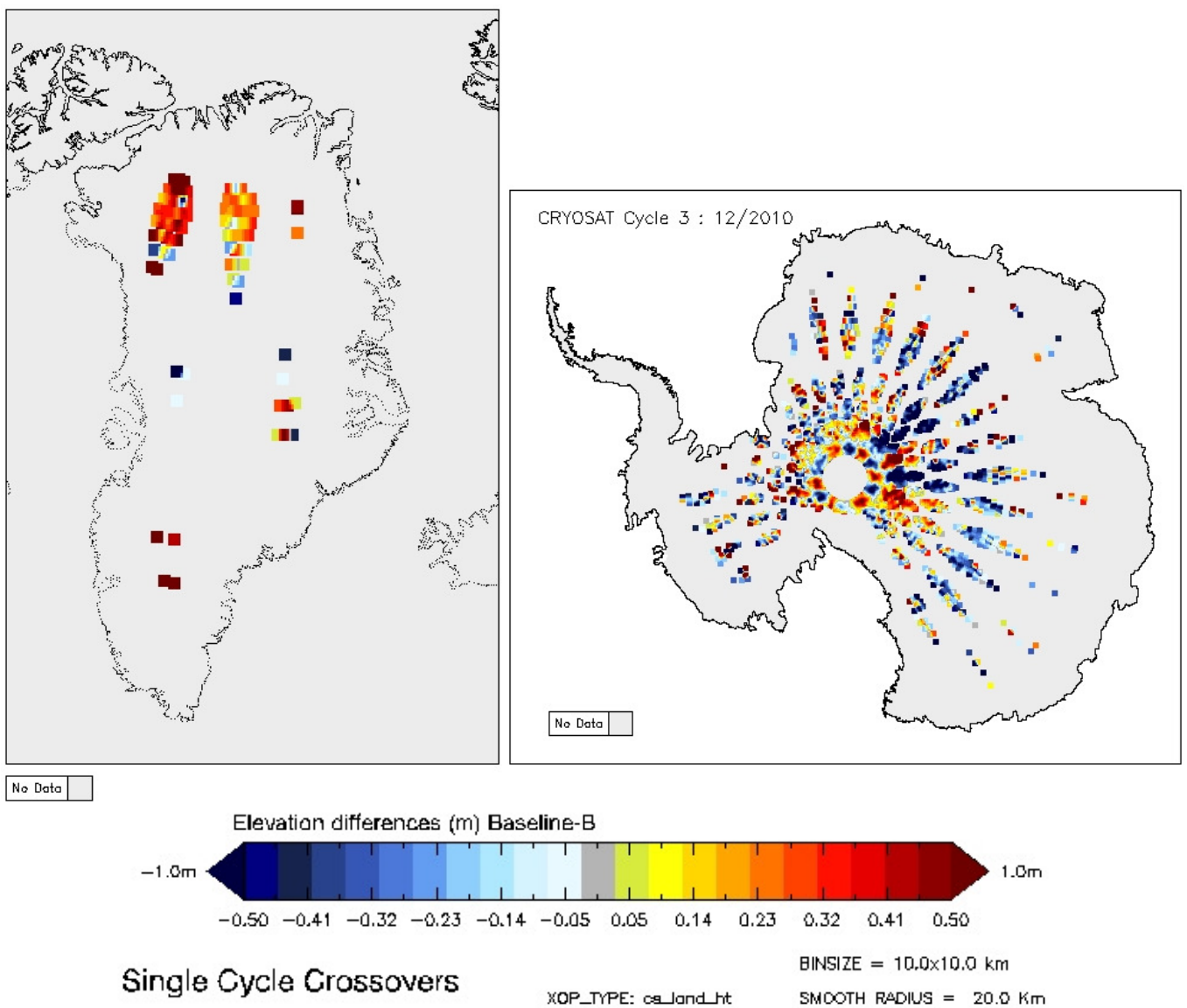
Figure 5-16 Greenland and Antarctica maps of LRM elevation differences for cycle 3.
