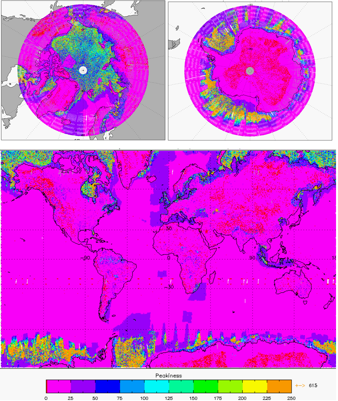
Figure 5-11 Global and Polar plots of Waveform Peakiness for cycle 3.
