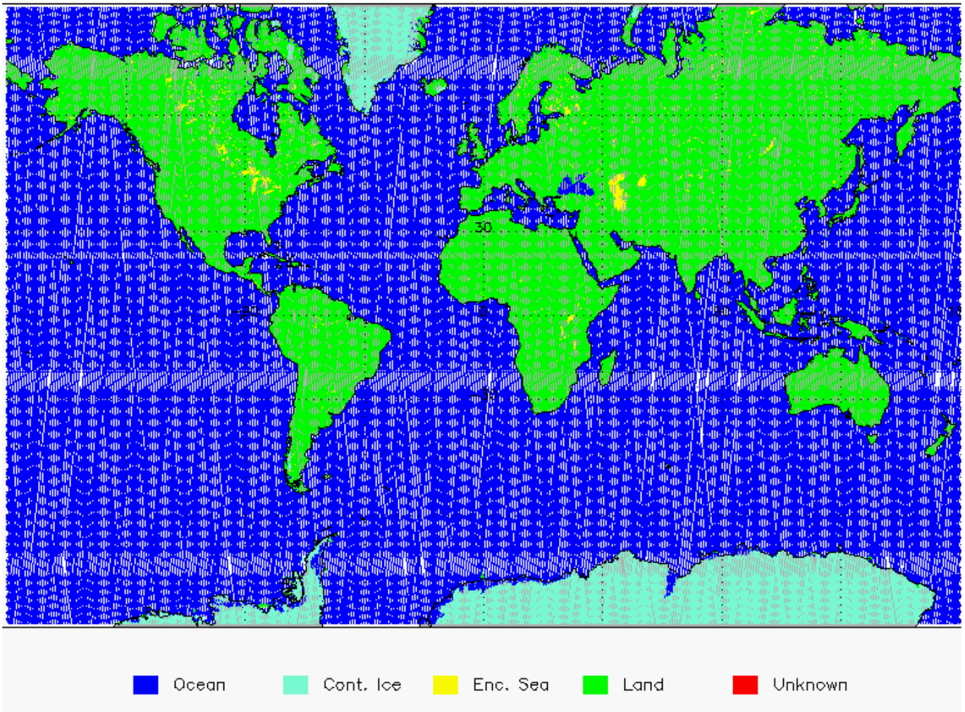
Figure 5-3 Global plot of Surface Type for cycle 3.
