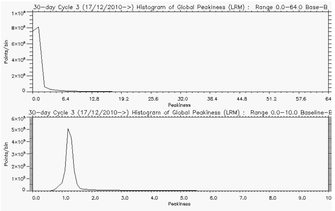
Figure 5-8 Histogram of global Peakiness for LRM, for cycle 3.
