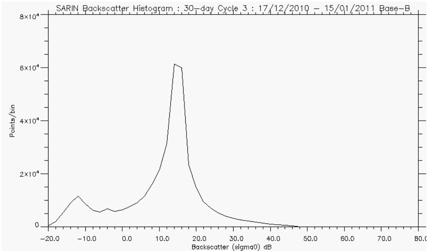
Figure 5-7 Backscatter Histogram for SARIn, cycle 3.
