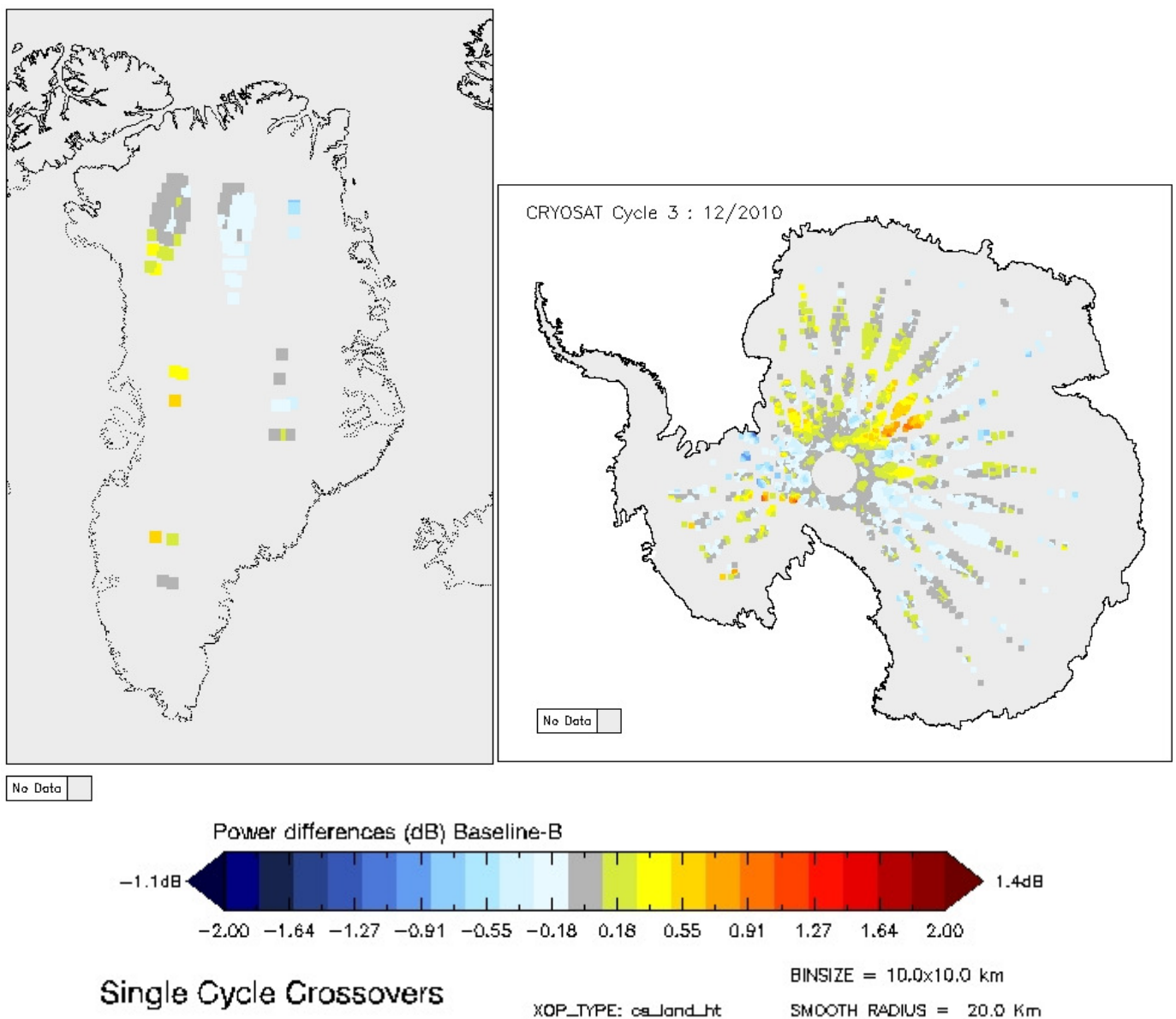
Figure 5-18 Greenland and Antarctica maps of LRM power differences for cycle 3.
