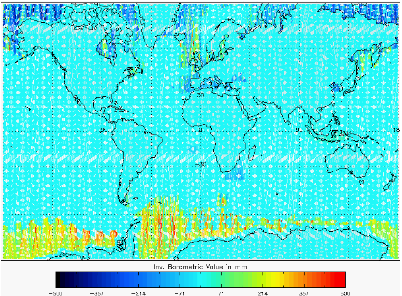
Figure 5-22 Global plot of Inverse Barometric Correction for cycle 3.
