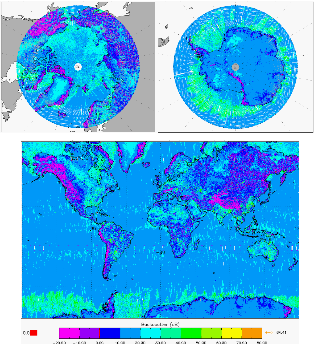
Figure 5-4 Global and Polar plots of Backscatter for cycle 3.
