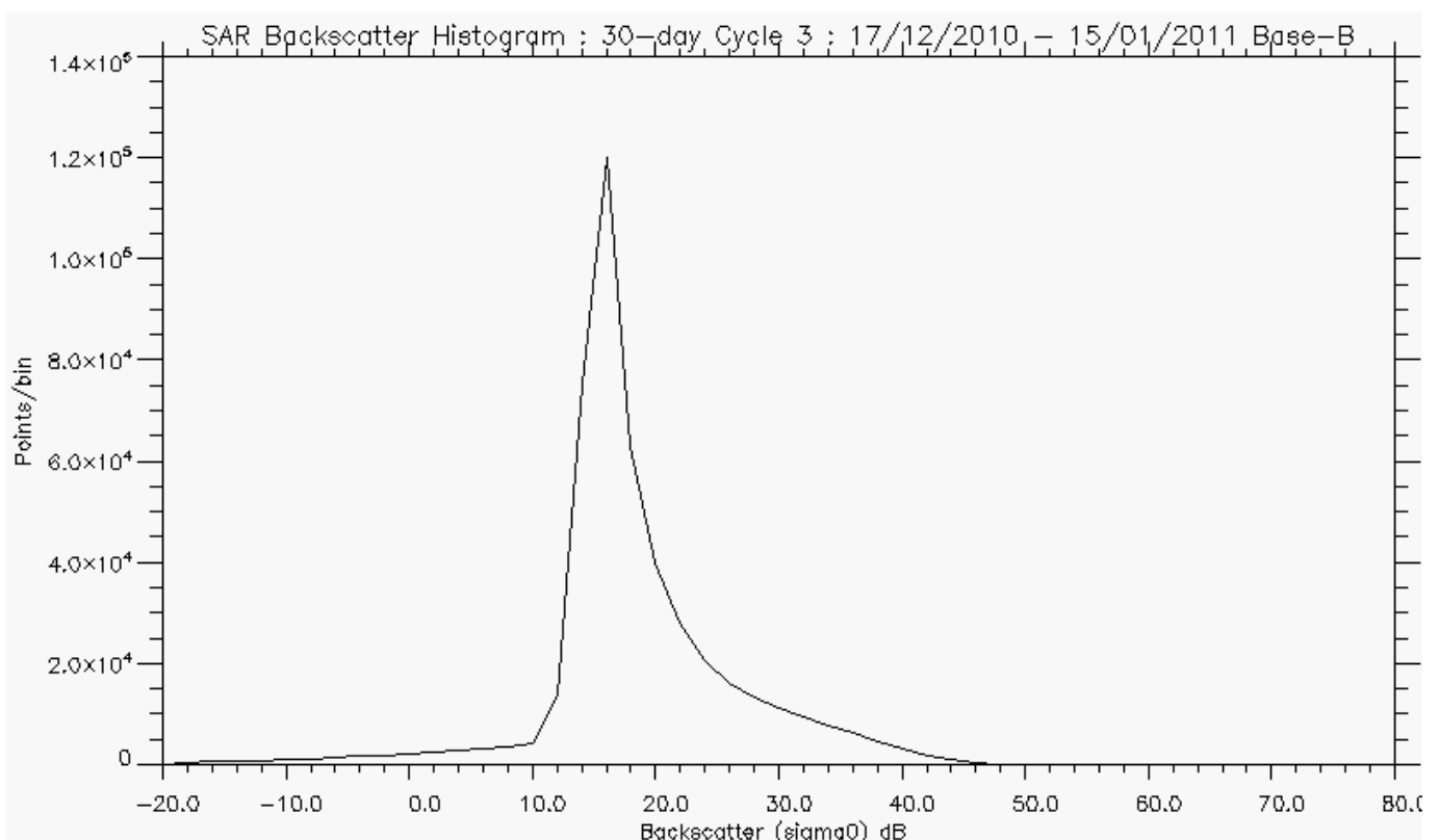
Figure 5-6 Backscatter Histogram for SAR, cycle 3.
