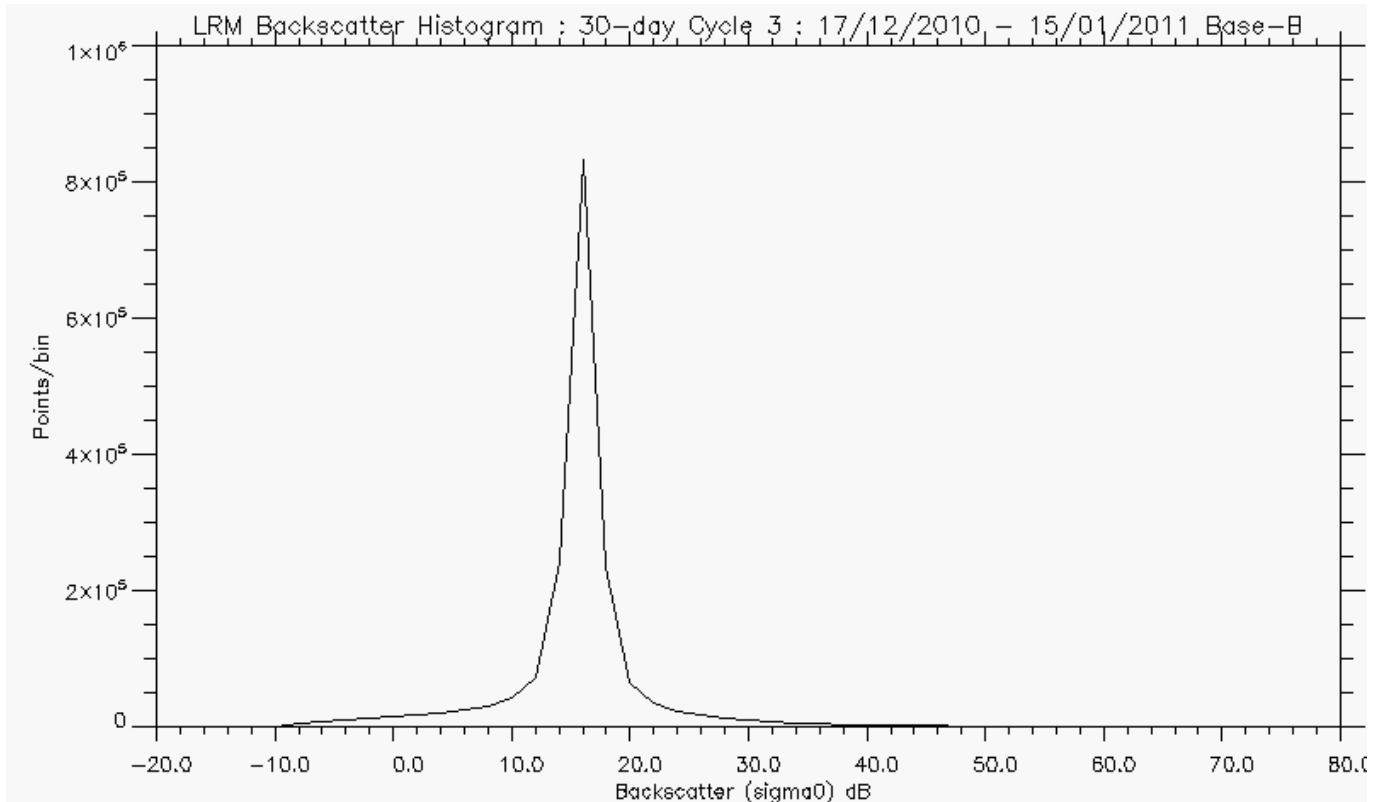
Figure 5-5 Backscatter Histogram for LRM, cycle 3.
