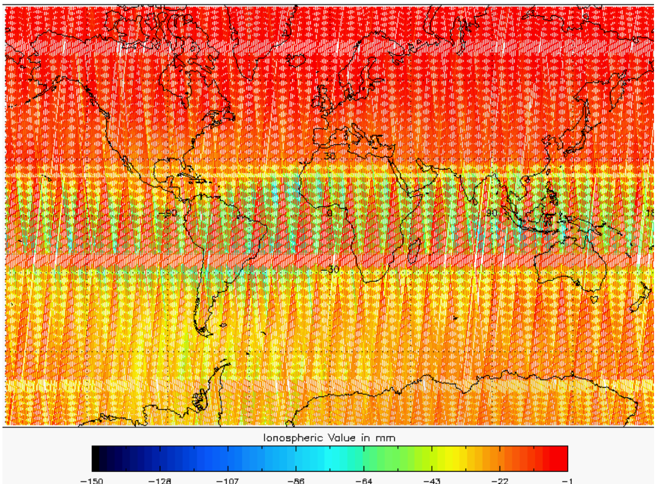
Figure 5-24 Global plot of Ionospheric Correction for cycle 3.
