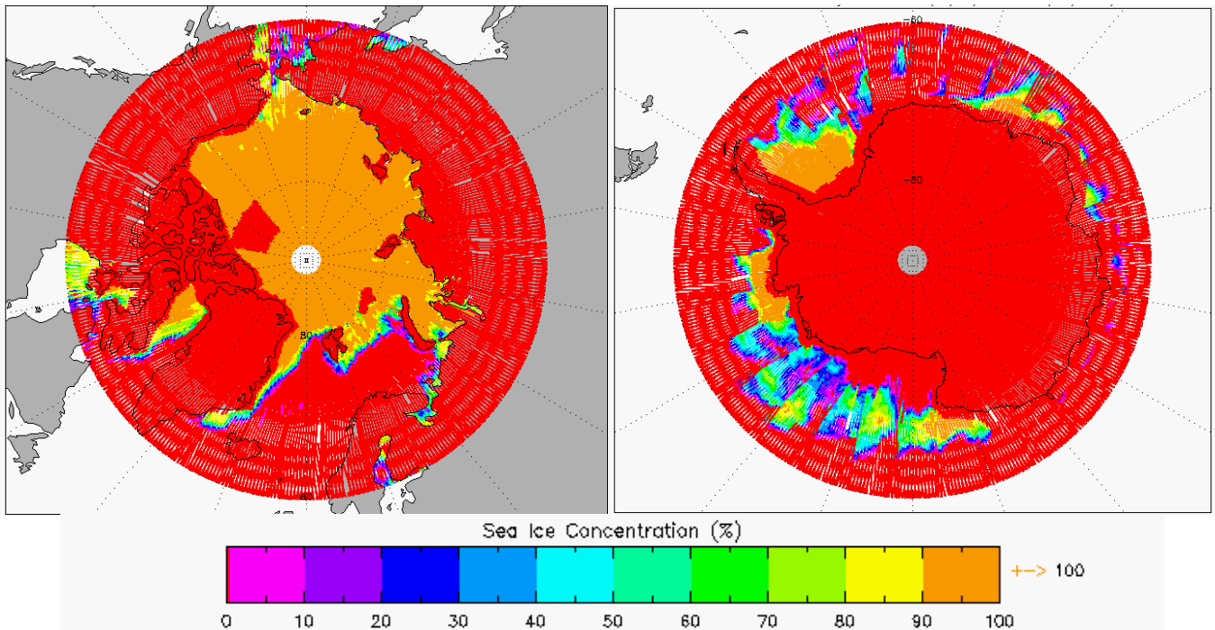
Figure 5-13 Polar plots of Sea Ice Concentration for cycle 3.
