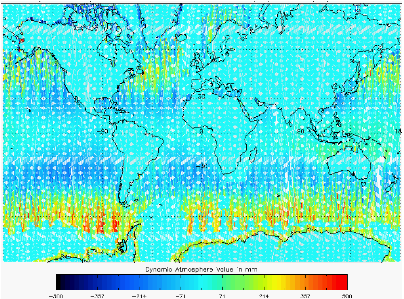
Figure 5-23 Global plot of Dynamic Atmosphere Correction for cycle 3.
