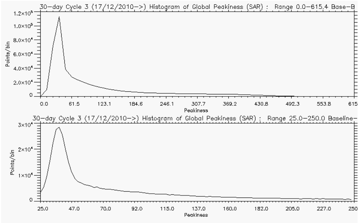
Figure 5-9 Histogram of global Peakiness for SAR, for cycle 3.
