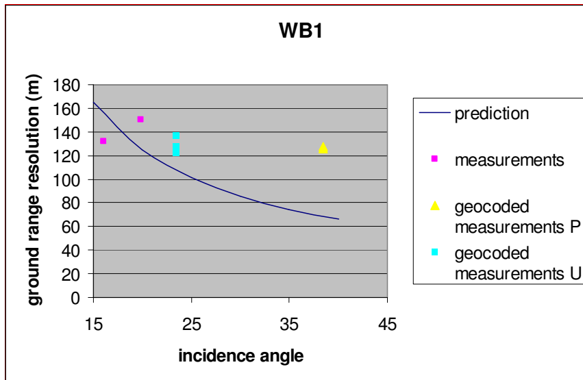
Figure 6.2.1 Ground range resolution for wide swath mode (WB1) data.
