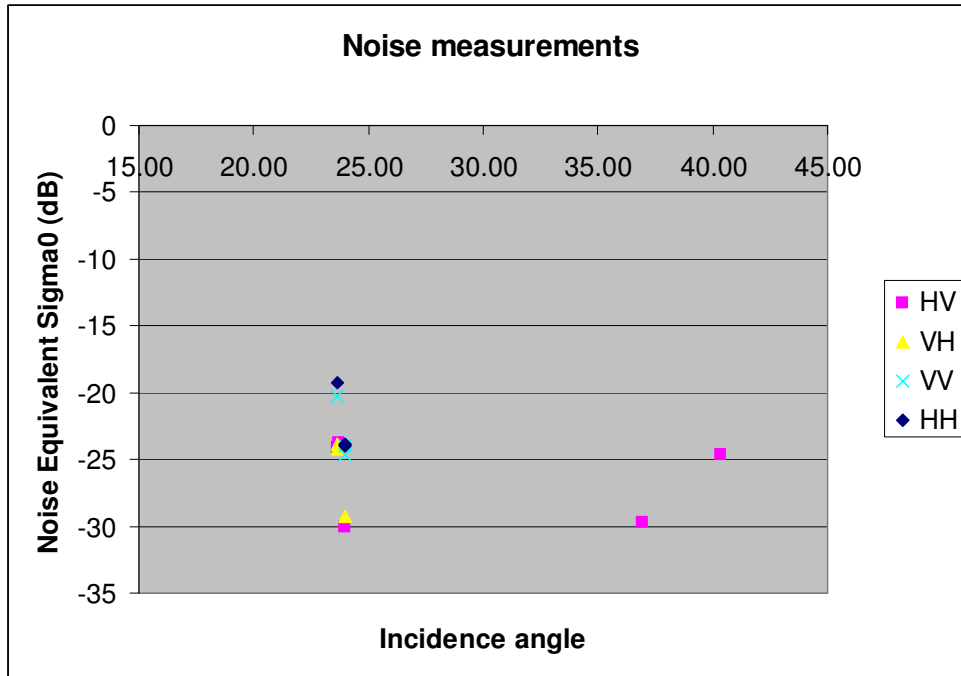
Figure 6.4.1 Measured Noise equivalent Sigma0 variation with polarization and incidence angle
