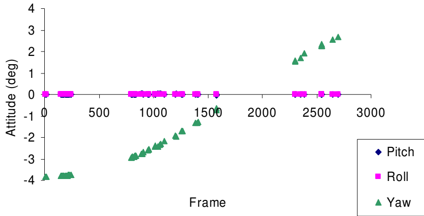
Figure 6-2: Attitude of the satellite as a function of the frame number
