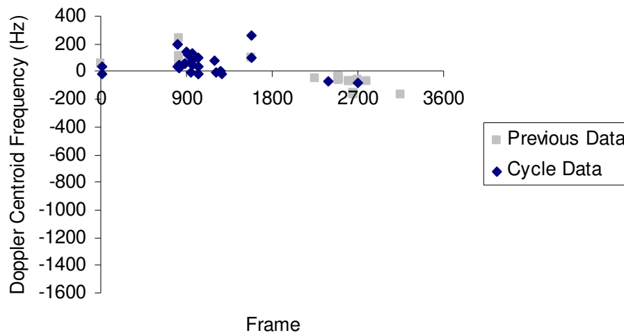
Figure 6-1: Doppler centroid frequency given as a function of the frame
