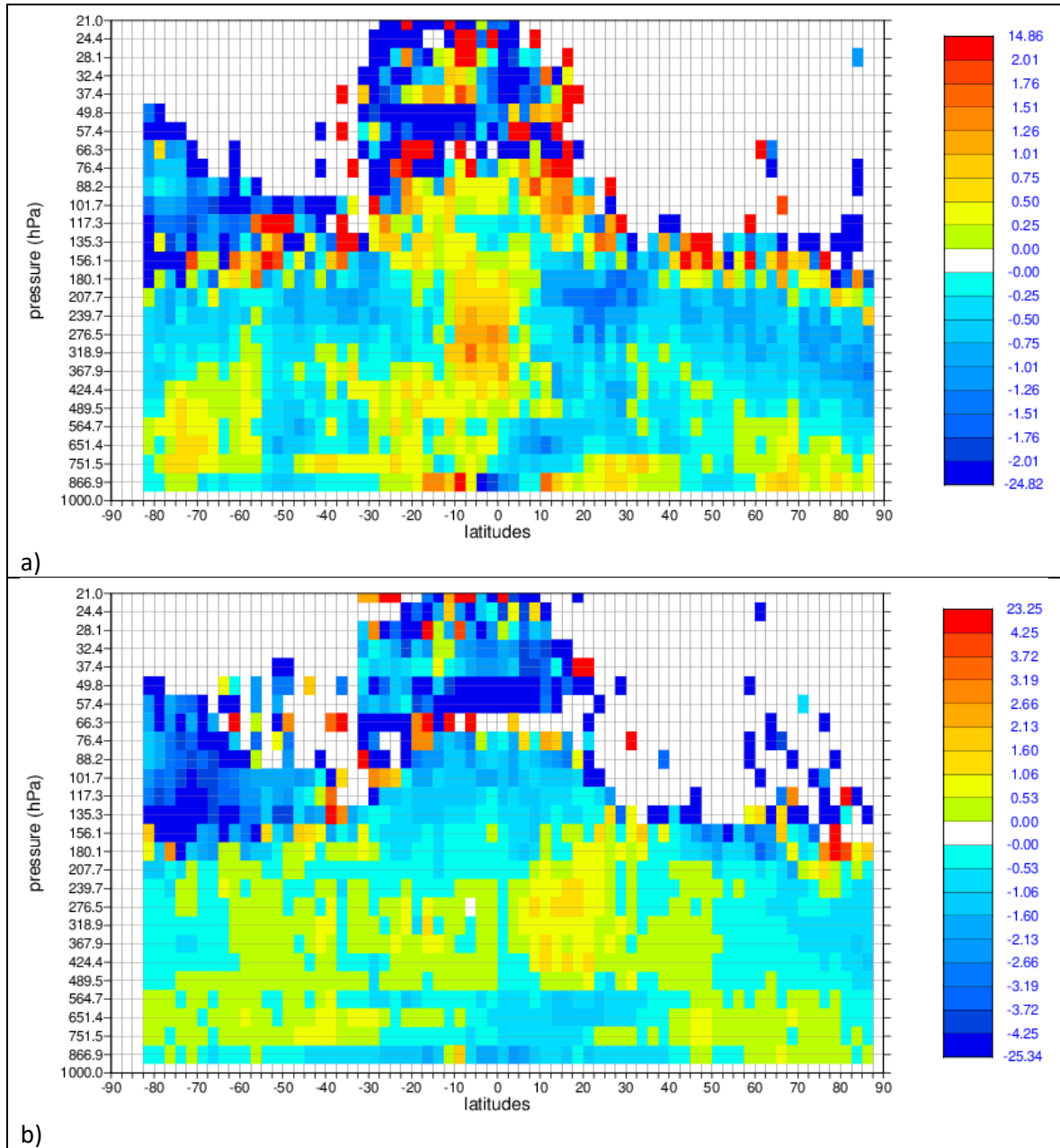
Figure 7. Pressure versus latitude dependence of the L2B Mie-cloudy mean(O-B) for a) ascending and b) descending orbits. Unit: m/s. For the period: 20 February 2023 to 1 April 2023.
