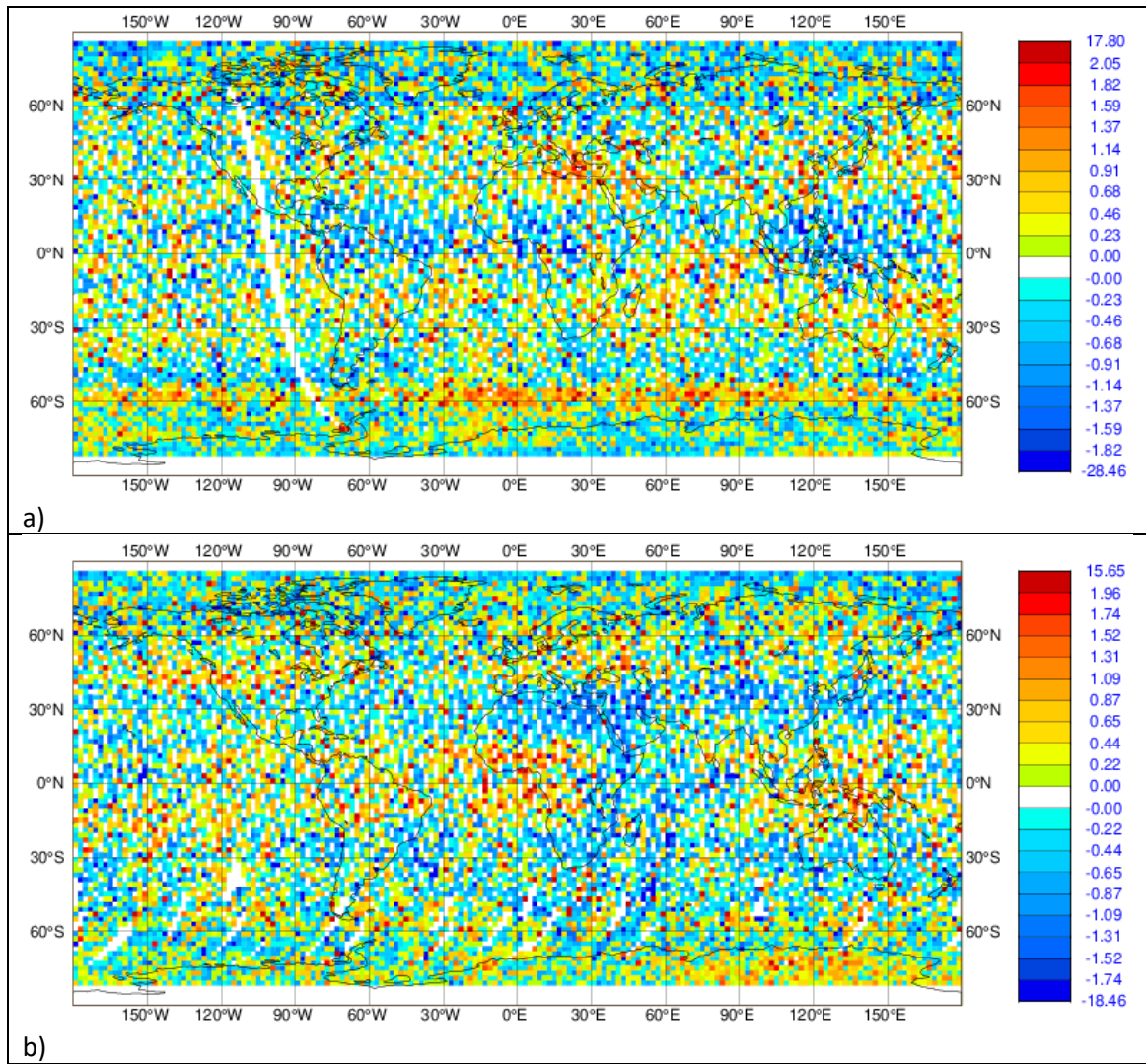
Figure 3. Maps of L2B Rayleigh-clear mean(O-B) for the 0-400 hPa pressure range for a) ascending and b) descending orbit phases. Unit: m/s. For the period: 31 March 2023 to 28 April 2023. These plots are only updated once per week.
