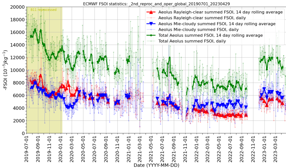
Figure 10. Time-series of the negative of the FSOI of Aeolus L2B HLOS winds with ECMWF reprocessing and ECMWF operations (after 9 January 2020) until 29 April 2023. Therefore, positive values of -FSOI indicate short-range forecast improvement due to assimilating Aeolus. Partitioned into Mie-cloudy (blue), Rayleigh-clear (red) and combined (green). This metric is based on a global dry energy norm. A 2-week rolling average was applied (thicker lines), and periods with reduced data counts, due to special operations were removed from this averaging.
