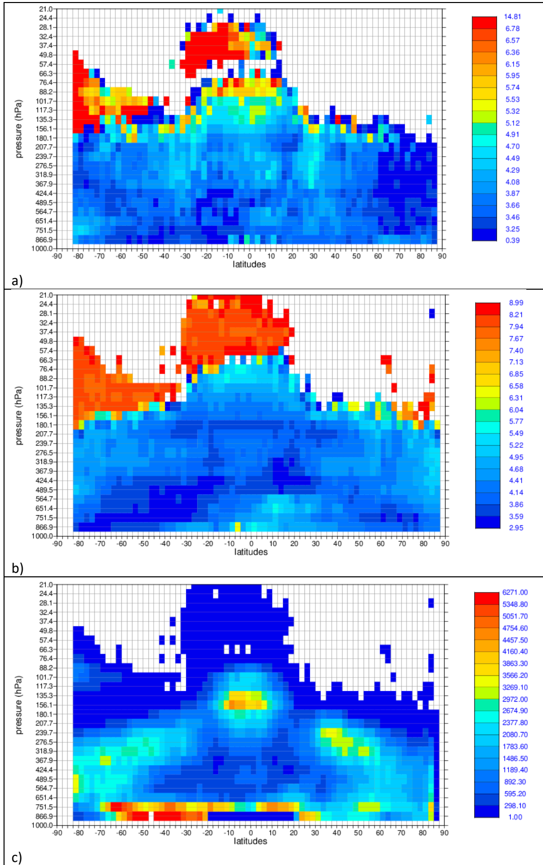
Figure 8. Pressure versus latitude dependence of the ascending L2B Mie-cloudy a) \text{stdev}(\text{O}-\text{B}) m/s, b) assigned observation error in DA (via scaled L2Bp error estimates) and c) number of observations. For the period: 20 March 2023 to 29 April 2023.
