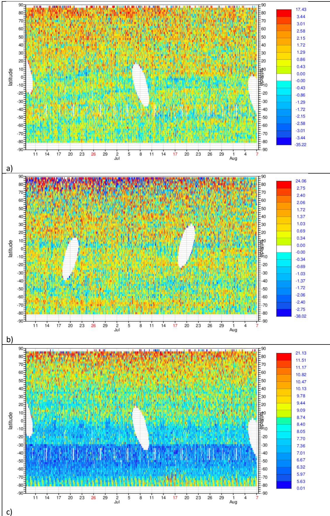
Figure 2. Latitude-time dependence statistics for L2B Rayleigh-clear HLOS winds for the 0-400 hPa pressure range with a) mean(O-B) ascending; b) mean(O-B) descending and c) stdev(O-B) for descending orbit phase. Unit: m/s.
