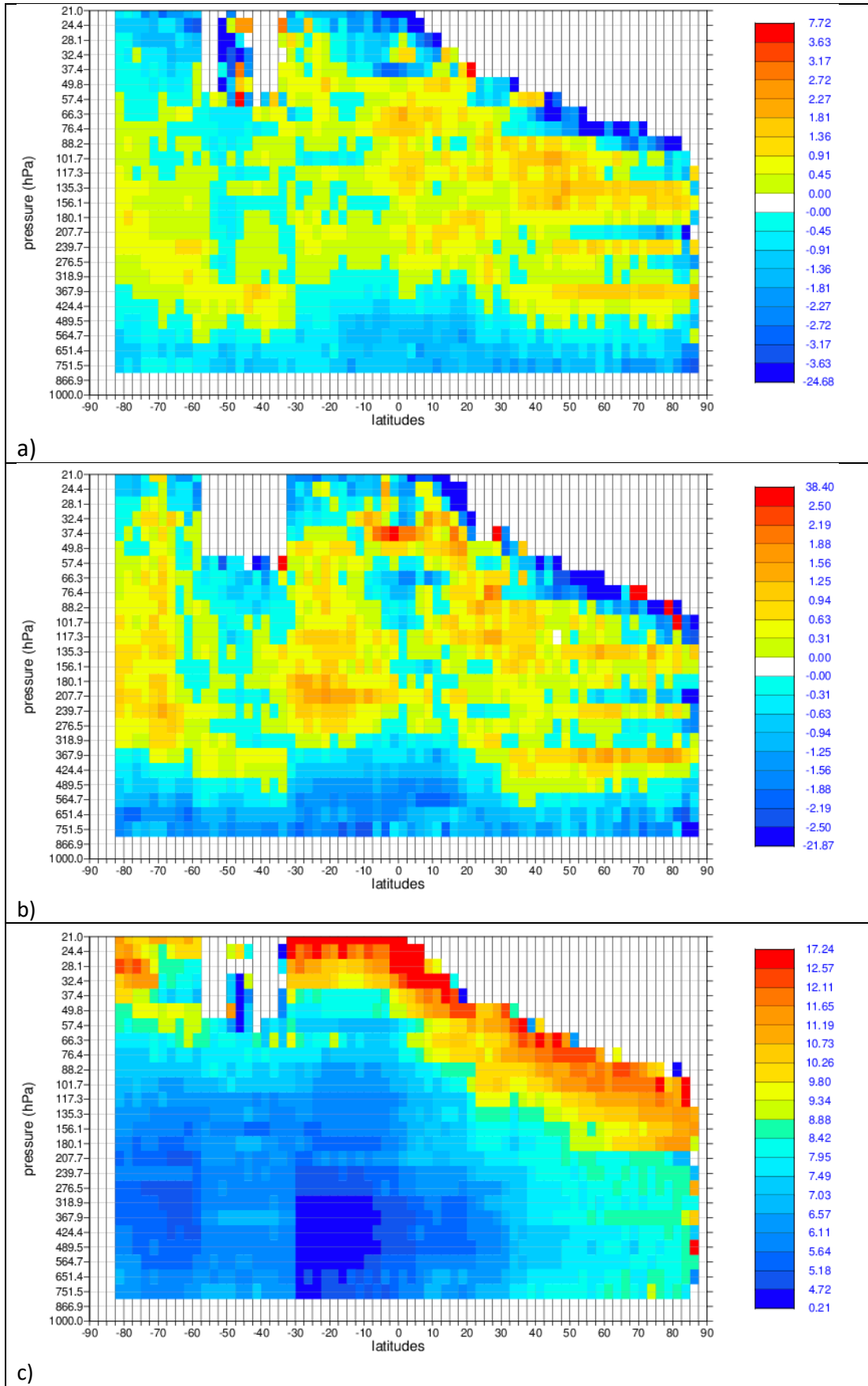
Figure 4. Pressure versus latitude dependence of the L2B Rayleigh-clear mean(O-B) for a) ascending and b) descending orbits. Panel c) is the standard deviation of (O-B) for ascending orbits. Unit: m/s. For the period: 27 June to 6 August 2022.
