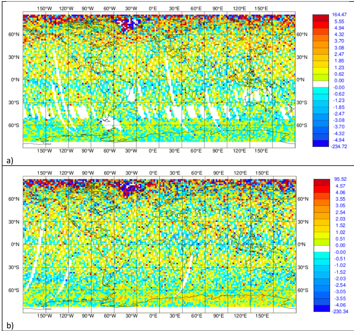
Figure 3. Maps of L2B Rayleigh-clear mean(O-B) for the 0-400 hPa pressure range for a) ascending and b) descending orbit phases. Unit: m/s. For the period: 1 July 2022 to 5 August 2022. These plots are only updated once per week.
