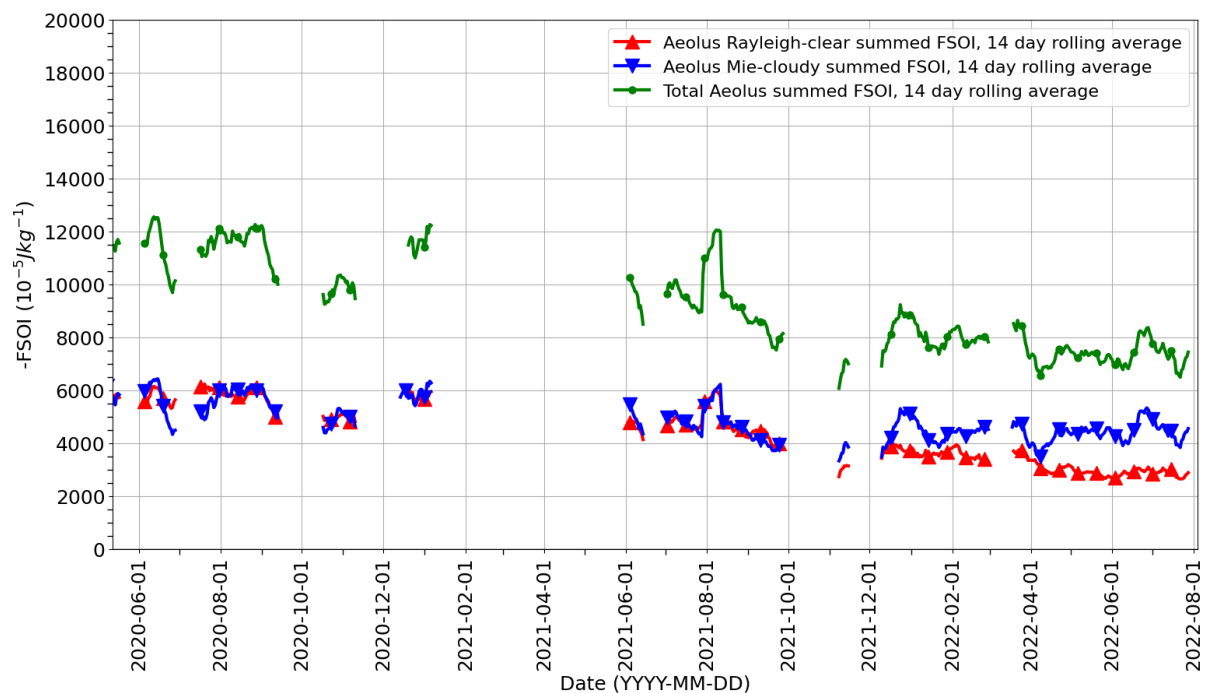
Figure 10. Time-series of the negative of the FSOI of Aeolus L2B HLOS winds in ECMWF operations since the L2B data public release (12 May 2020) until 4 August 2022. Therefore, positive values of -FSOI indicate short-range forecast improvement due to assimilating Aeolus. Partitioned into Mie-cloudy (blue), Rayleigh-clear (red) and combined (green). This metric is based on a global dry energy norm. A 2-week rolling average was applied, and periods with reduced data counts, due to special operations were removed from this averaging
