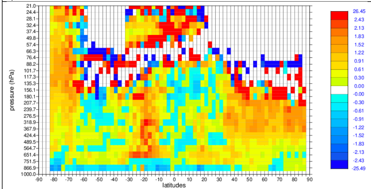
Figure 7. Pressure versus latitude dependence of the L2B Mie-cloudy mean(O-B) for a) ascending and b) descending orbits. Unit: m/s. For the period: 27 June to 6 August 2022.
