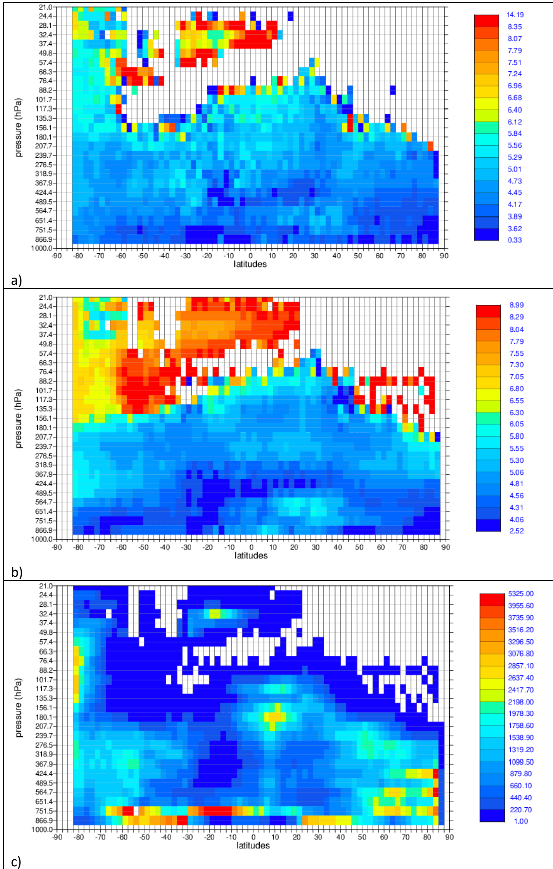
Figure 8. Pressure versus latitude dependence of the ascending L2B Mie-cloudy a) stdev(O-B) m/s, b) assigned observation error in DA (via scaled L2Bp error estimates) and c) number of observations. For the period: 27 June to 6 August 2022.
